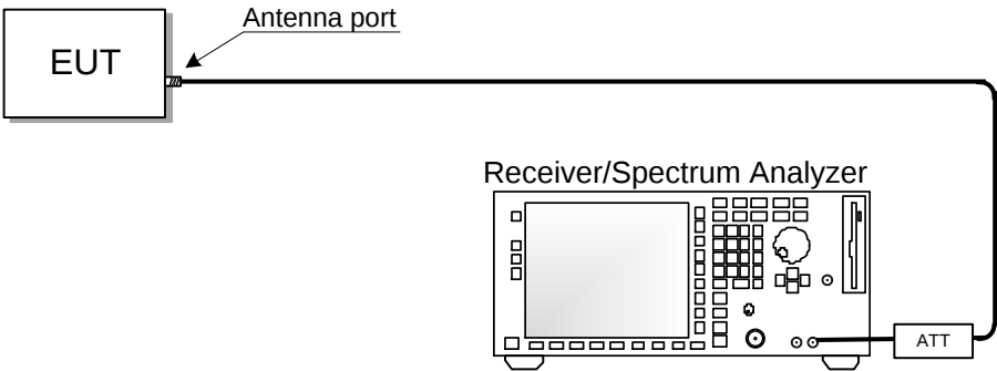
Figure 5.5-2: Antenna port testing block diagram
