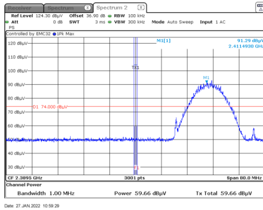
Figure 8.5-7: Sample plot, radiated band edge 802.11b low ch. Peak
