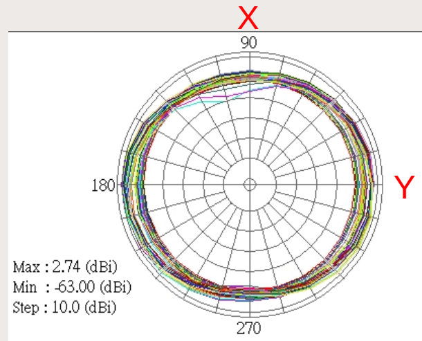
H plane
