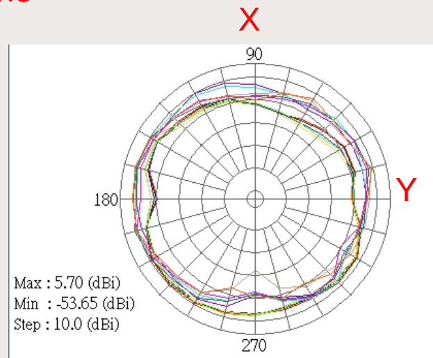
H plane
