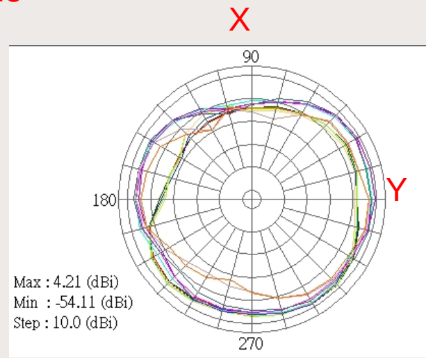
H plane
