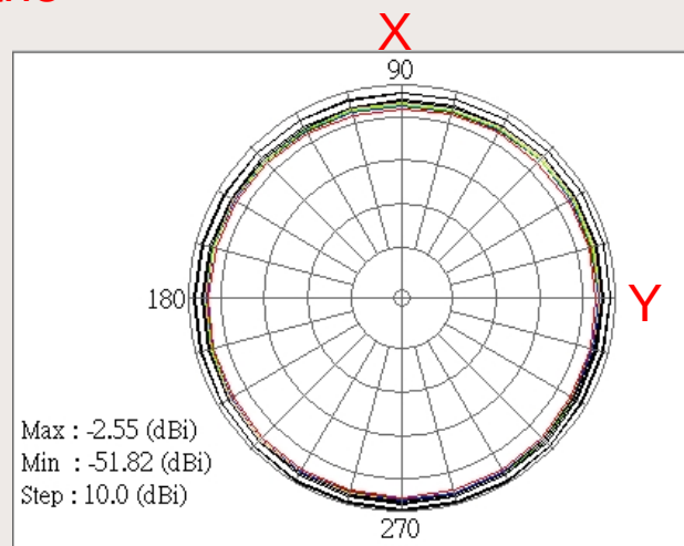
H plane
