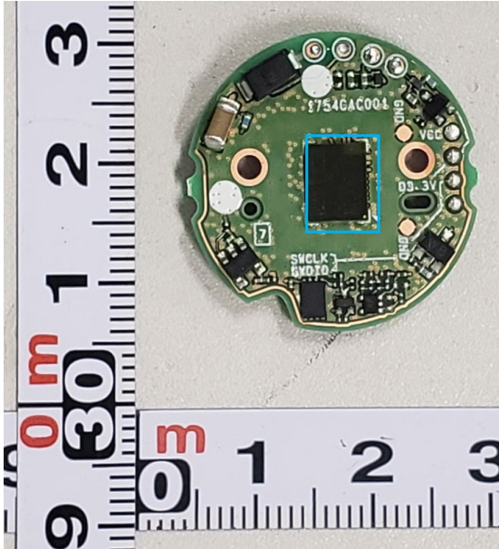
Wireless IC side (Black center IC is wireless IC)
