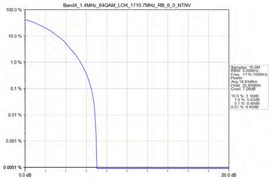
Band4_1.4MHz_64QAM_LCH_1710.7MHz_RB_6_0_NTNV
