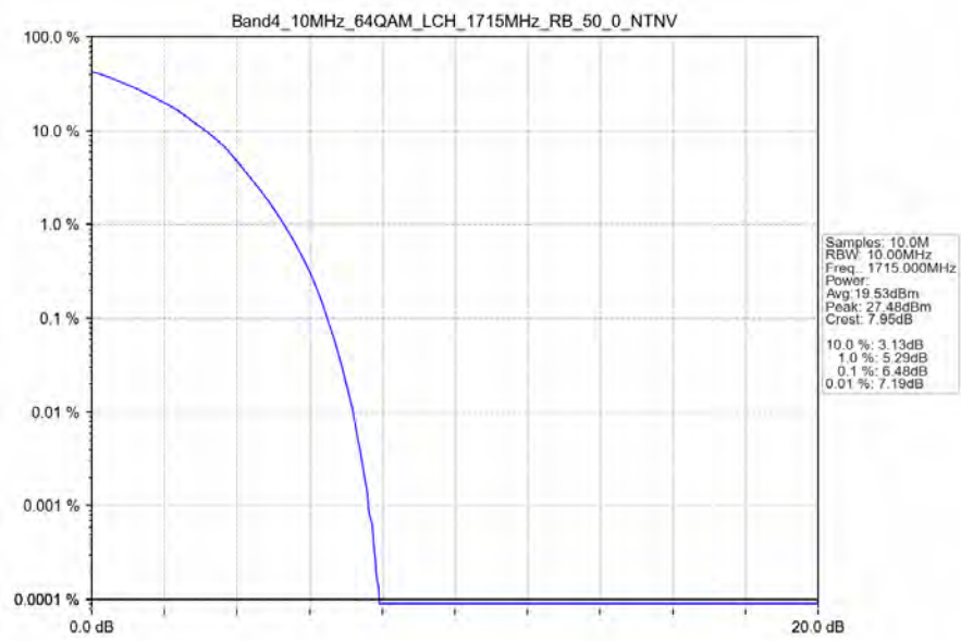
Band4_10MHz_64QAM_LCH_1715MHz_RB_50_0_NTNV
