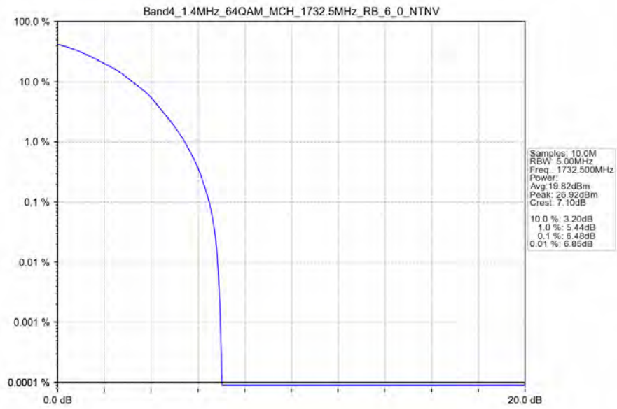
Band4_1.4MHz_64QAM_MCH_1732.5MHz_RB_6_0_NTNV
