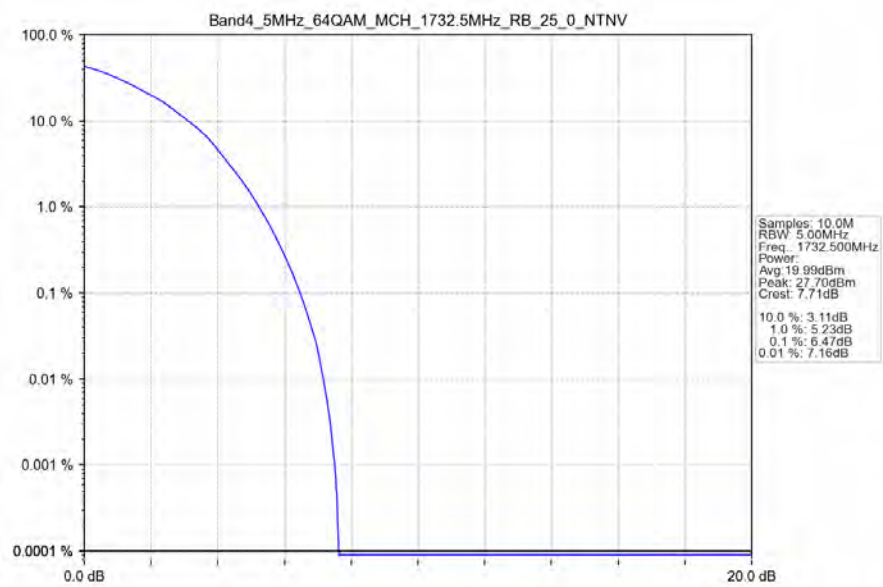
Band4_5MHz_64QAM_MCH_1732.5MHz_RB_25_0_NTNV
