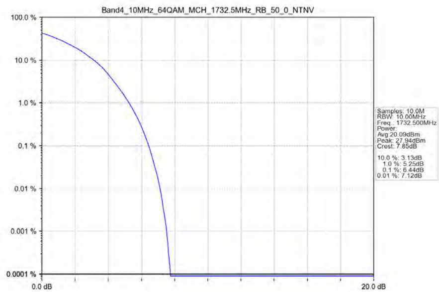
Band4_10MHz_64QAM_MCH_1732.5MHz_RB_50_0_NTNV
