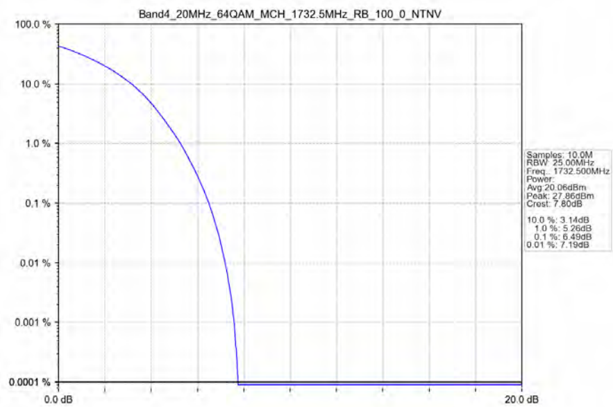
Band4_20MHz_64QAM_MCH_1732.5MHz_RB_100_0_NTNV
