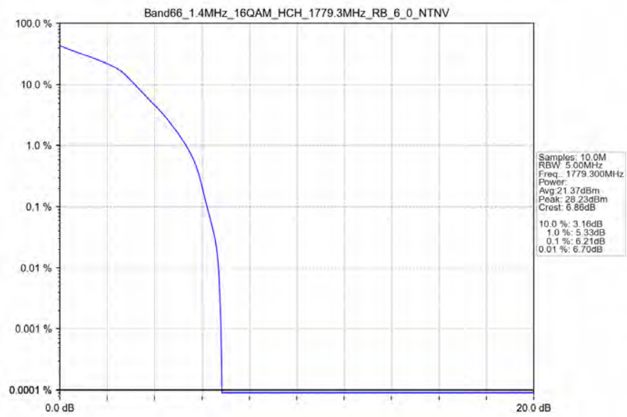
Band66_1.4MHz_16QAM_HCH_1779.3MHz_RB_6_0_NTNV
