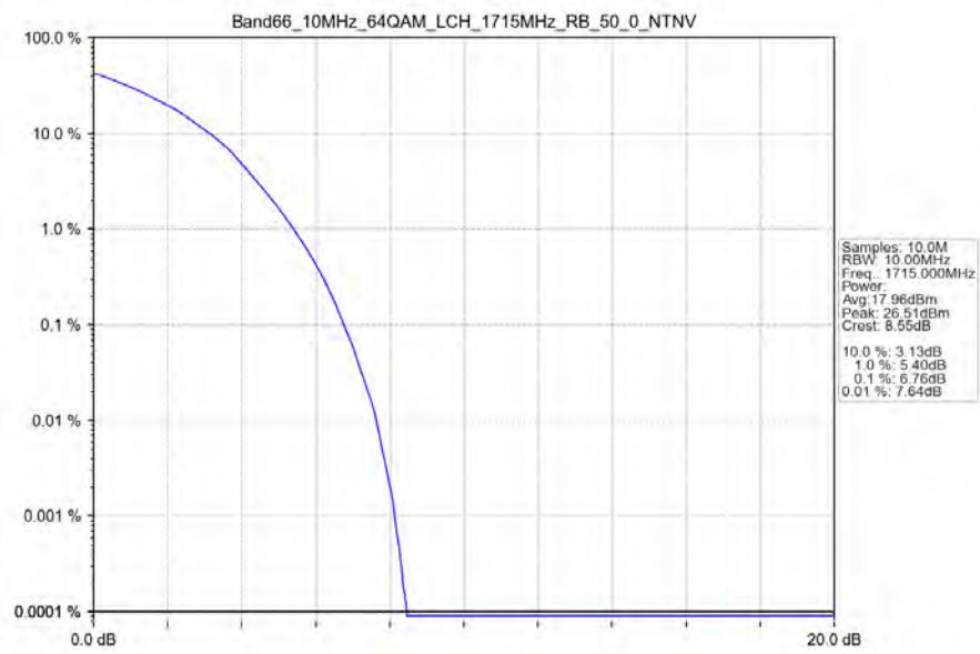
Band66_10MHz_64QAM_LCH_1715MHz_RB_50_0_NTNV
