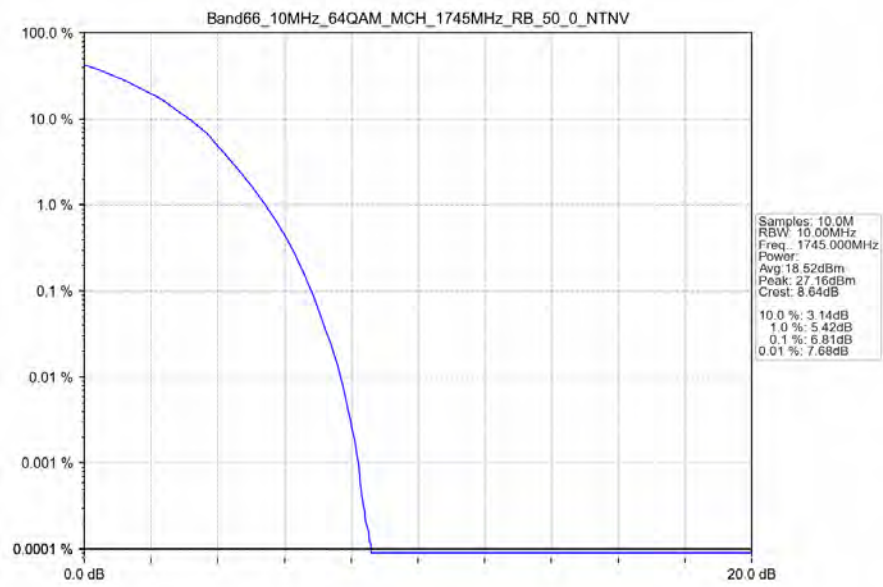
Band66_10MHz_64QAM_MCH_1745MHz_RB_50_0_NTNV
