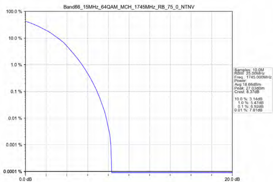
Band66_15MHz_64QAM_MCH_1745MHz_RB_75_0_NTNV
