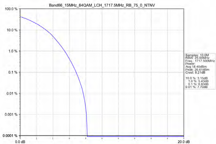
Band66_15MHz_64QAM_LCH_1717.5MHz_RB_75_0_NTNV
