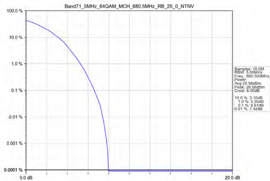
Band71_5MHz_64QAM_MCH_680.5MHz_RB_25_0_NTNV
