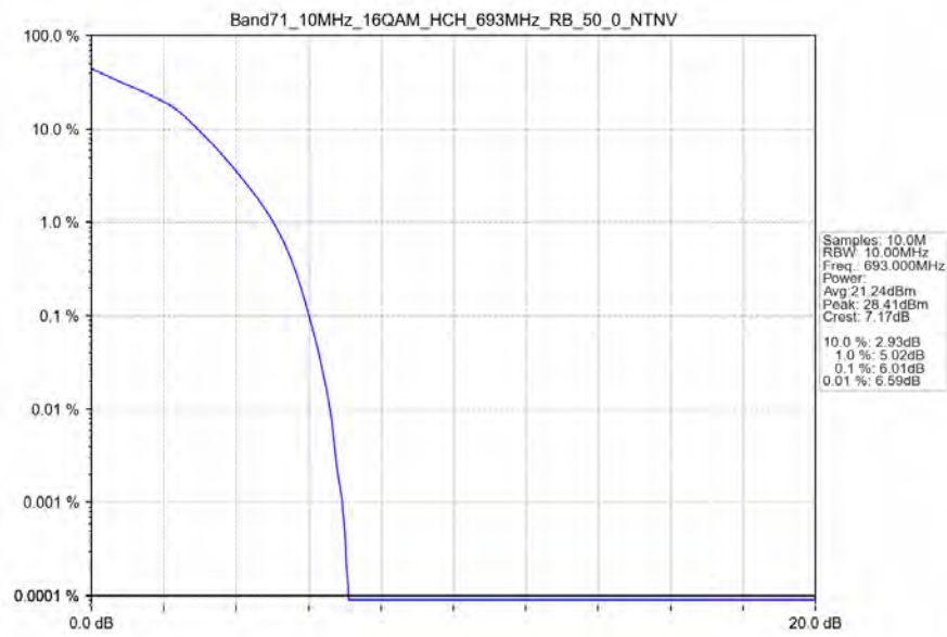
Band71_10MHz_16QAM_HCH_693MHz_RB_50_0_NTNV
