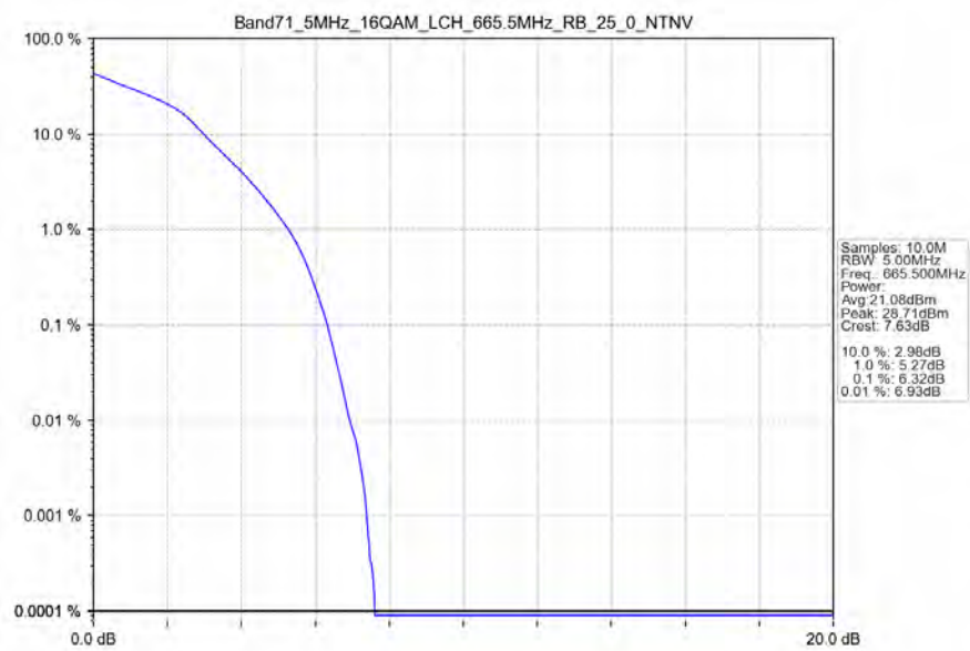
Band71_5MHz_16QAM_LCH_665.5MHz_RB_25_0_NTNV
