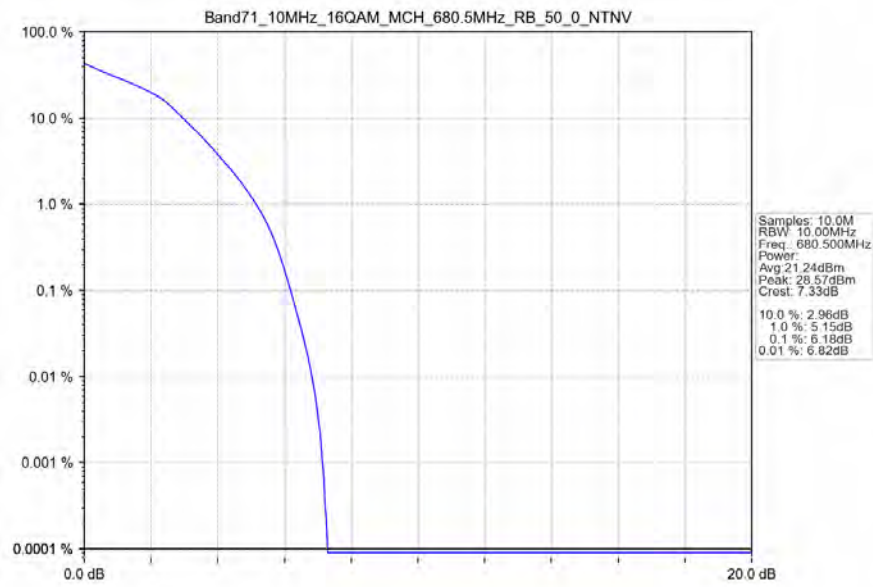
Band71_10MHz_16QAM_MCH_680.5MHz_RB_50_0_NTNV
