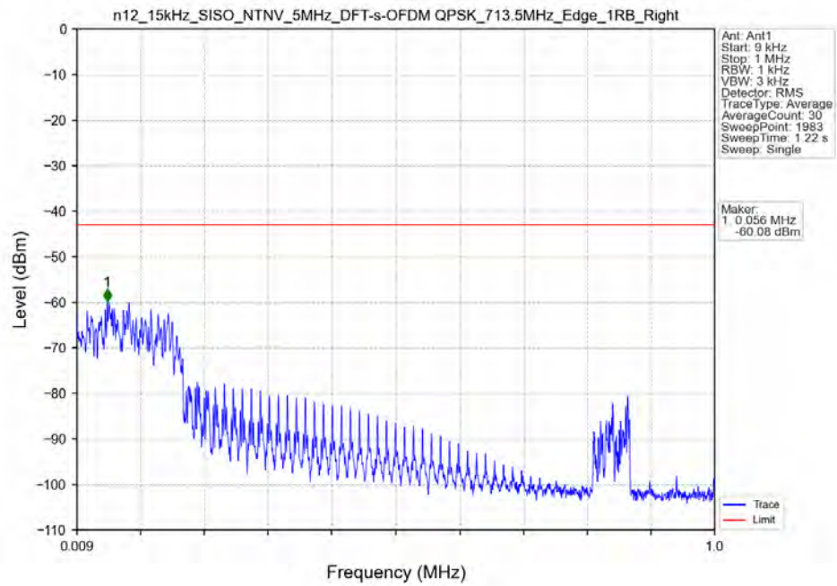
n12_15kHz_SISO_NTNV_5MHz_DFT-s-OFDM_QPSK_713.5MHz_Edge_1RB_Right
