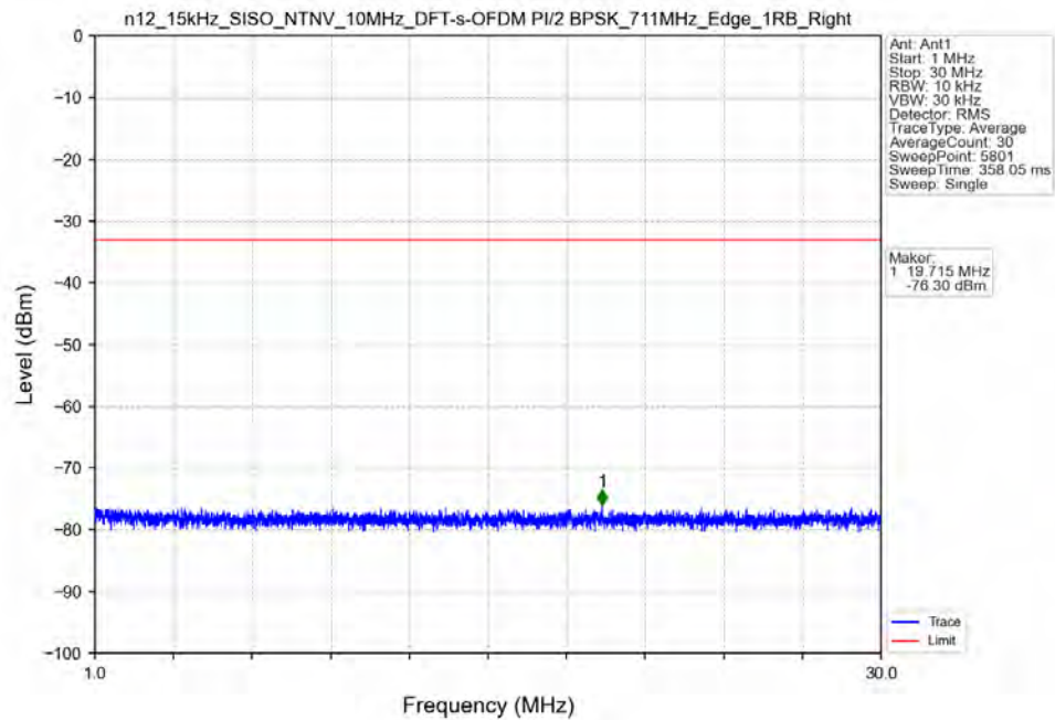
n12_15kHz_SISO_NTNV_10MHz_DFT-s-OFDM PI/2 BPSK_711MHz_Edge_1RB_Right
