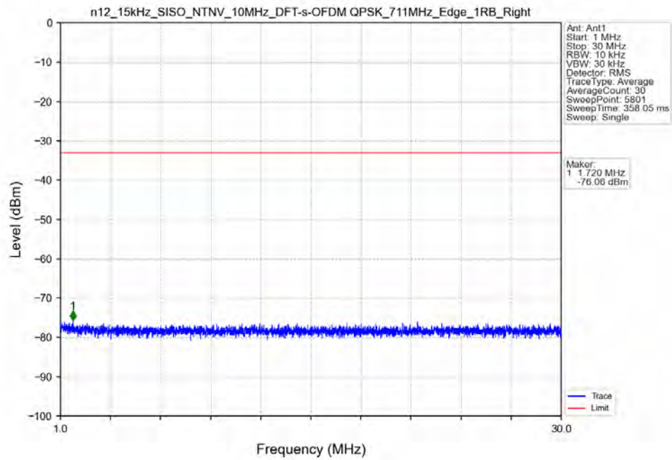
n12_15kHz_SISO_NTNV_10MHz_DFT-s-OFDM QPSK 711MHz_Edge_1RB_Right
