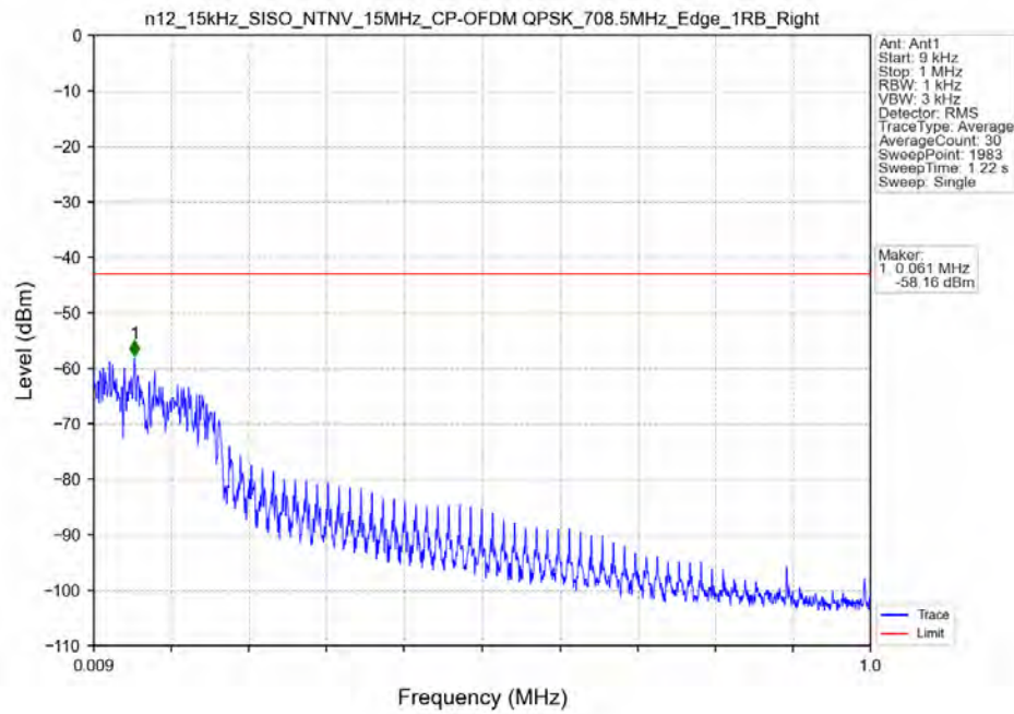
n12_15kHz_SISO_NTNV_15MHz_CP-OFDM_QPSK_708.5MHz_Edge_1RB_Right
