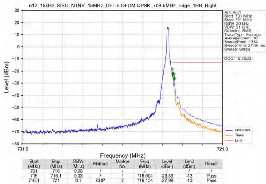
n12_15kHz_SISO_NTNV_15MHz_DFT-s-OFDM_QPSK_708.5MHz_Edge_1RB_Right
