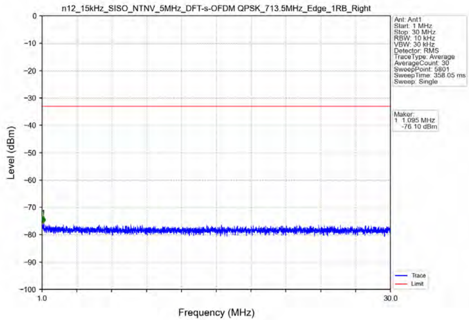
n12_15kHz_SISO_NTNV_5MHz_DFT-s-OFDM_QPSK_713.5MHz_Edge_1RB_Right
