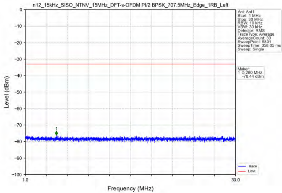
n12_15kHz_SISO_NTNV_15MHz_DFT-s-OFDM_PI/2_BPSK_707.5MHz_Edge_1RB_Left
