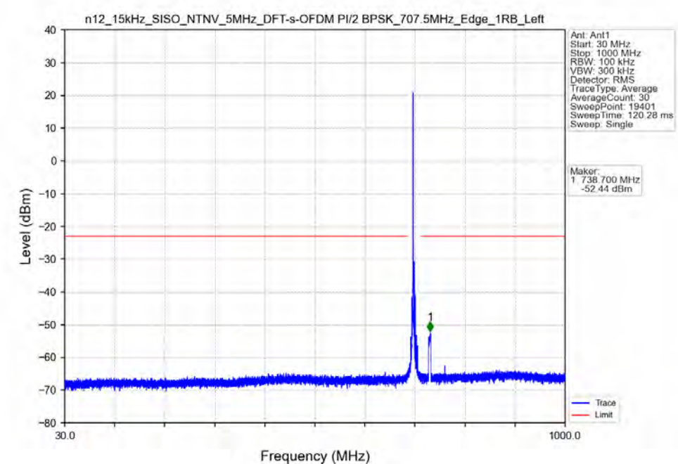
n12_15kHz_SISO_NTNV_5MHz_DFT-s-OFDM_PI/2_BPSK_707.5MHz_Edge_1RB_Left
