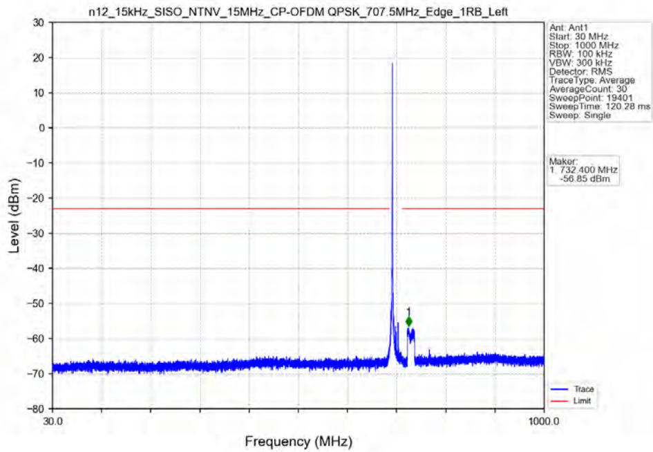
n12_15kHz_SISO_NTNV_15MHz_CP-OFDM_QPSK_707.5MHz_Edge_1RB_Left
