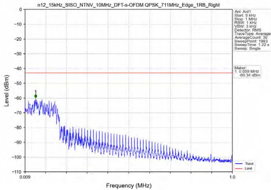
n12_15kHz_SISO_NTNV_10MHz_DFT-s-OFDM QPSK 711MHz_Edge_1RB_Right
