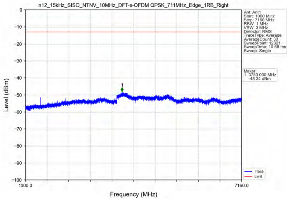
n12_15kHz_SISO_NTNV_10MHz_DFT-s-OFDM_QPSK_711MHz_Edge_1RB_Right
