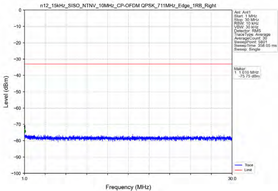
n12_15kHz_SISO_NTNV_10MHz_CP-OFDM_QPSK_711MHz_Edge_1RB_Right
