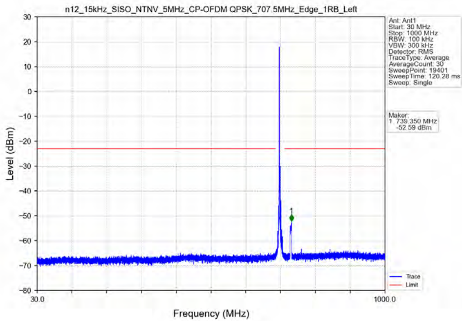
n12_15kHz_SISO_NTNV_5MHz_CP-OFDM_QPSK_707.5MHz_Edge_1RB_Left
