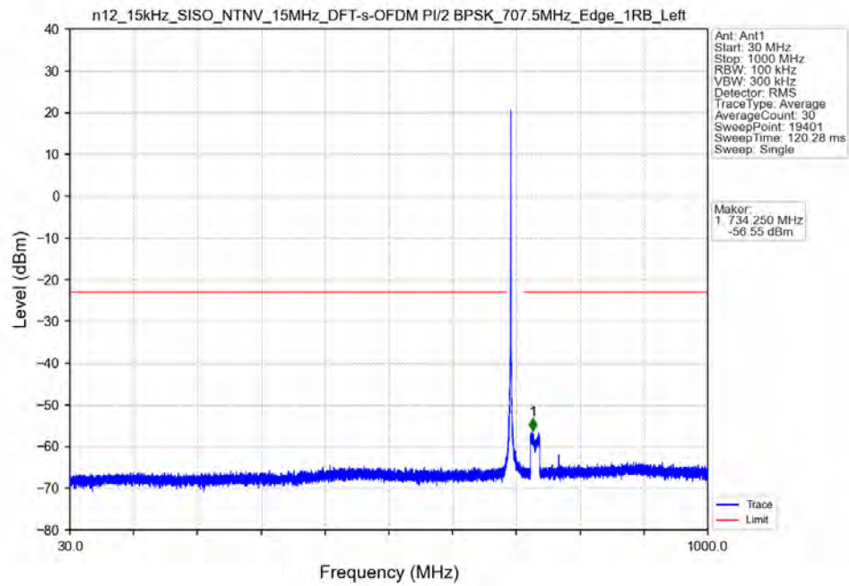
n12_15kHz_SISO_NTNV_15MHz_DFT-s-OFDM_PI/2_BPSK_707.5MHz_Edge_1RB_Left
