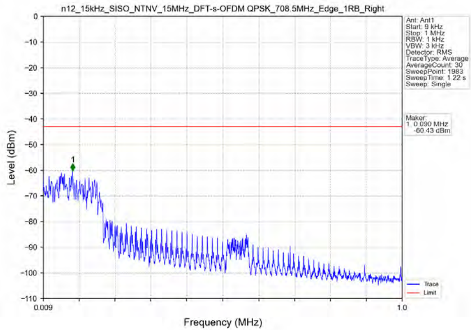
n12_15kHz_SISO_NTNV_15MHz_DFT-s-OFDM_QPSK_708.5MHz_Edge_1RB_Right
