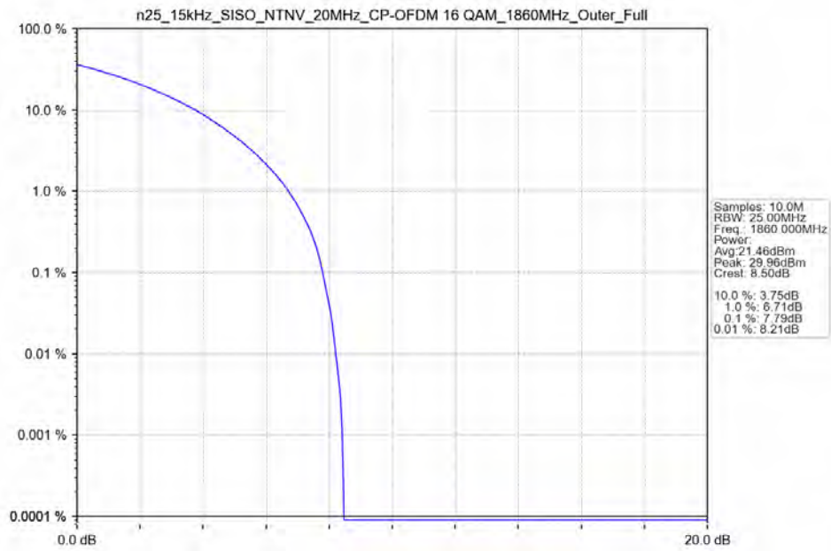
n25_15kHz_SISO_NTNV_20MHz_CP-OFDM 16 QAM_1860MHz_Outer_Full
