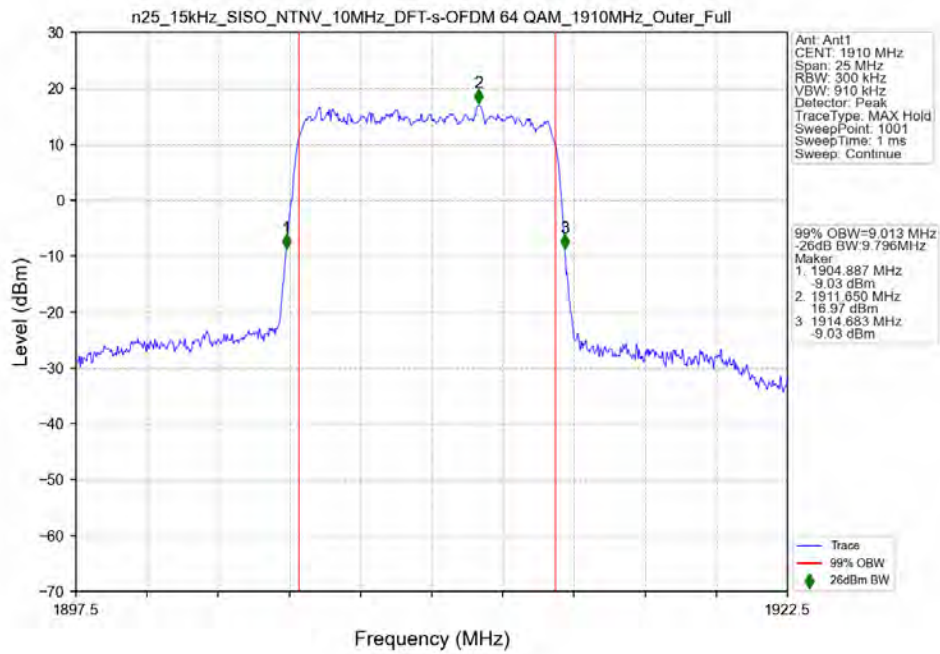
n25_15kHz_SISO_NTNV_10MHz_DFT-s-OFDM_64_QAM_1910MHz_Outer_Full
