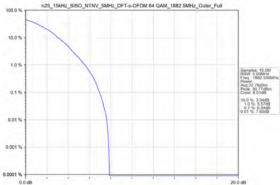
n25_15kHz_SISO_NTNV_5MHz_DFT-s-OFDM_64_QAM_1882.5MHz_Outer_Full
