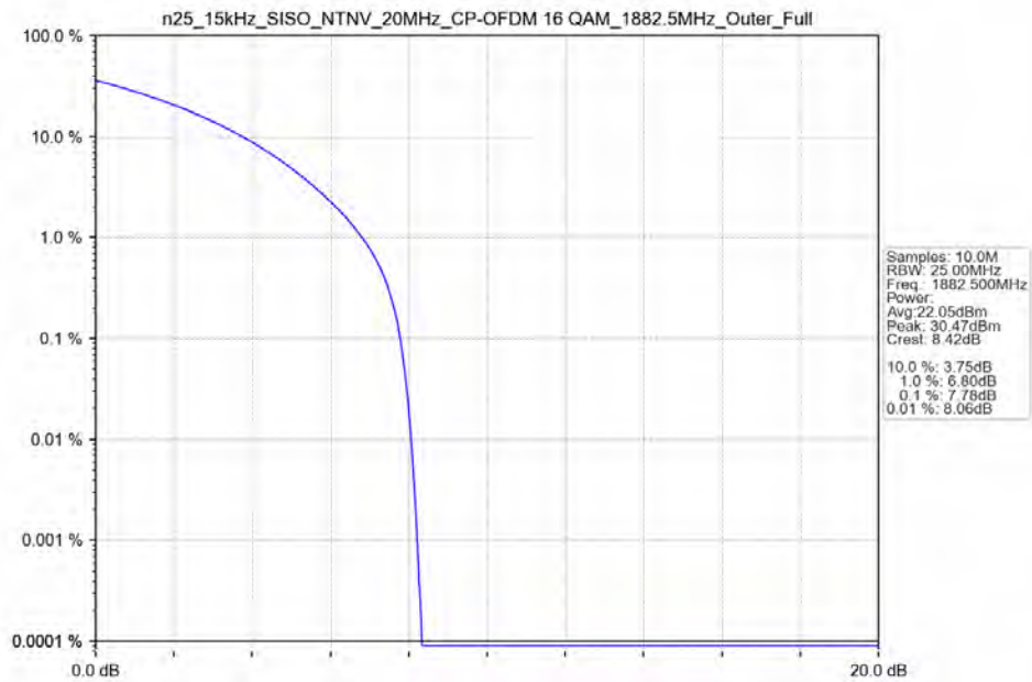
n25_15kHz_SISO_NTNV_20MHz_CP-OFDM 16 QAM_1882.5MHz_Outer_Full
