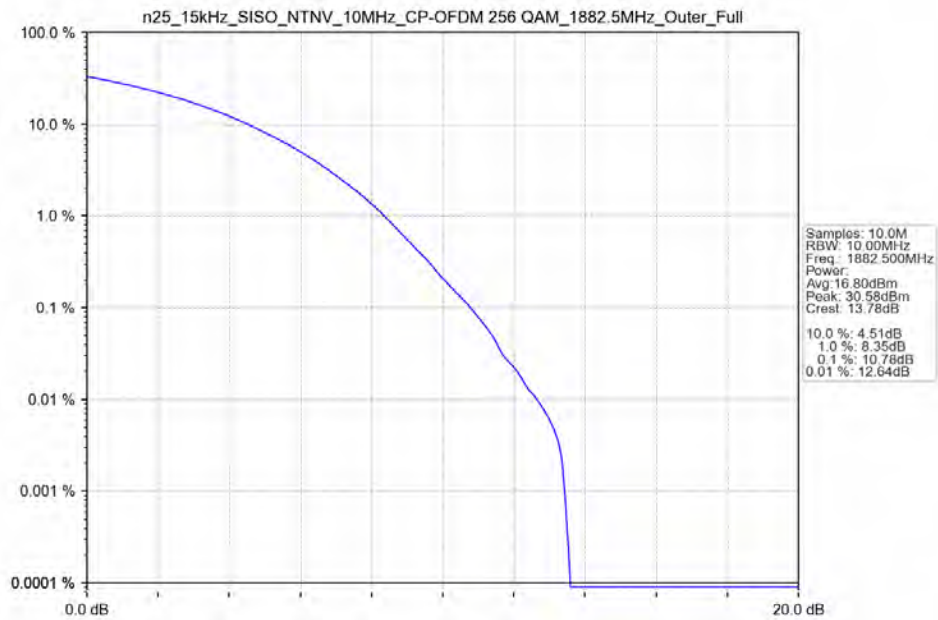
n25_15kHz_SISO_NTNV_10MHz_CP-OFDM 256 QAM_1882.5MHz_Outer_Full
