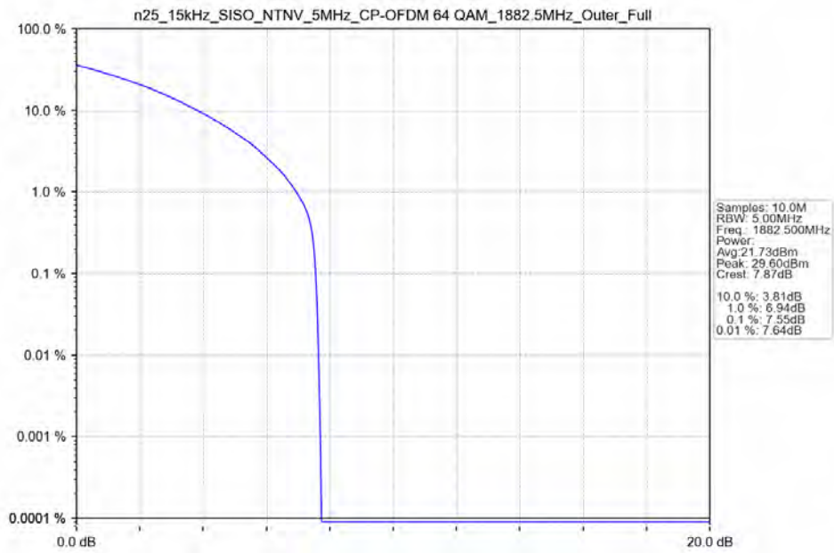
n25_15kHz_SISO_NTNV_5MHz_CP-OFDM 64 QAM_1882.5MHz_Outer_Full
