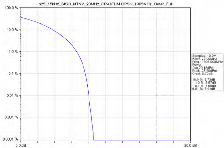
n25_15kHz_SISO_NTNV_20MHz_CP-OFDM_QPSK_1905MHz_Outer_Full
