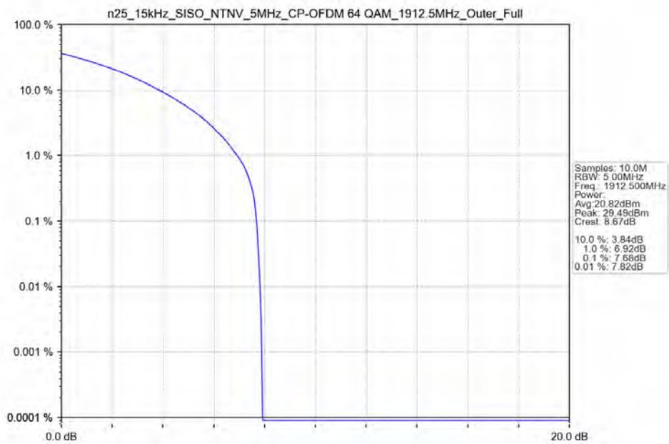
n25_15kHz_SISO_NTNV_5MHz_CP-OFDM 64 QAM_1912.5MHz_Outer_Full
