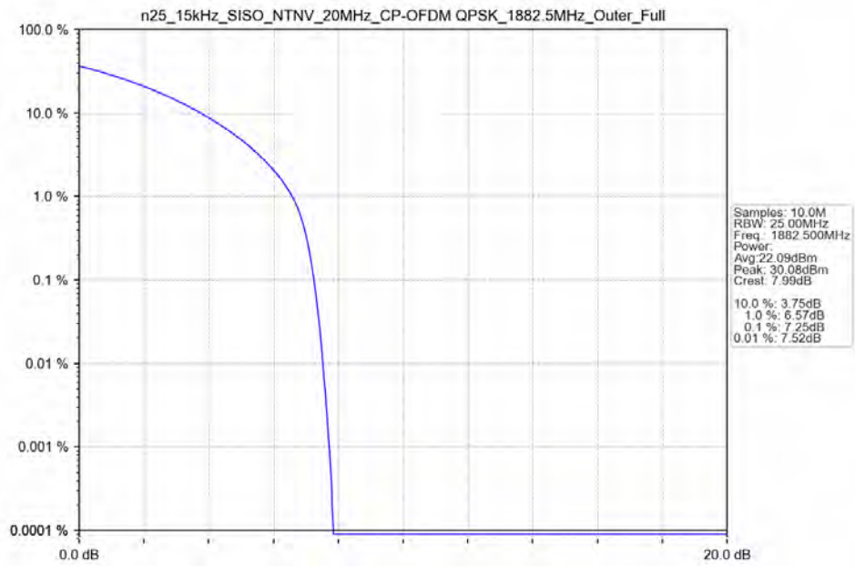
n25_15kHz_SISO_NTNV_20MHz_CP-OFDM_QPSK_1882.5MHz_Outer_Full
