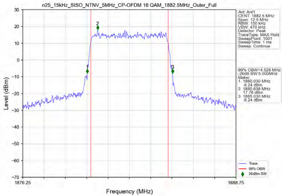
n25_15kHz_SISO_NTNV_5MHz_CP-OFDM_16 QAM_1882.5MHz_Outer_Full
