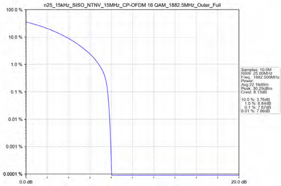
n25_15kHz_SISO_NTNV_15MHz_CP-OFDM 16 QAM_1882.5MHz_Outer_Full
