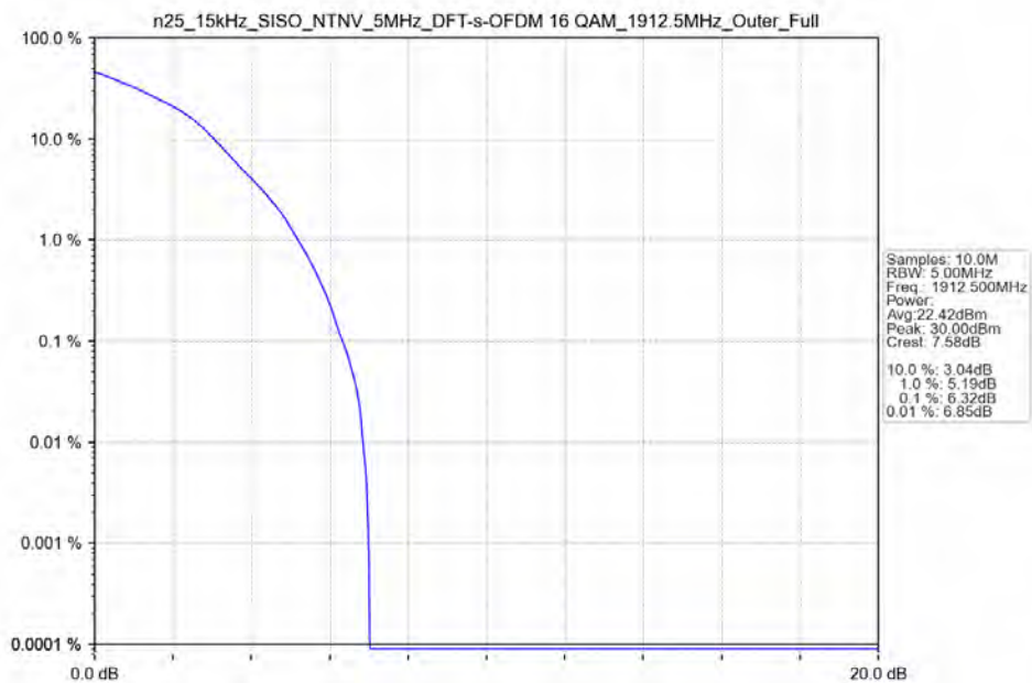
n25_15kHz_SISO_NTNV_5MHz_DFT-s-OFDM_16_QAM_1912.5MHz_Outer_Full
