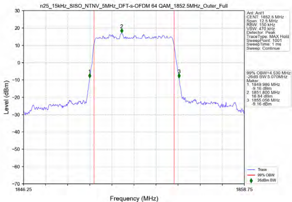
n25_15kHz_SISO_NTNV_5MHz_DFT-s-OFDM_64_QAM_1852.5MHz_Outer_Full
