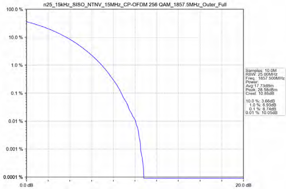
n25_15kHz_SISO_NTNV_15MHz_CP-OFDM_256_QAM_1857.5MHz_Outer_Full
