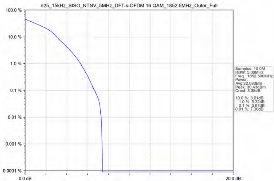
n25_15kHz_SISO_NTNV_5MHz_DFT-s-OFDM_16_QAM_1852.5MHz_Outer_Full
