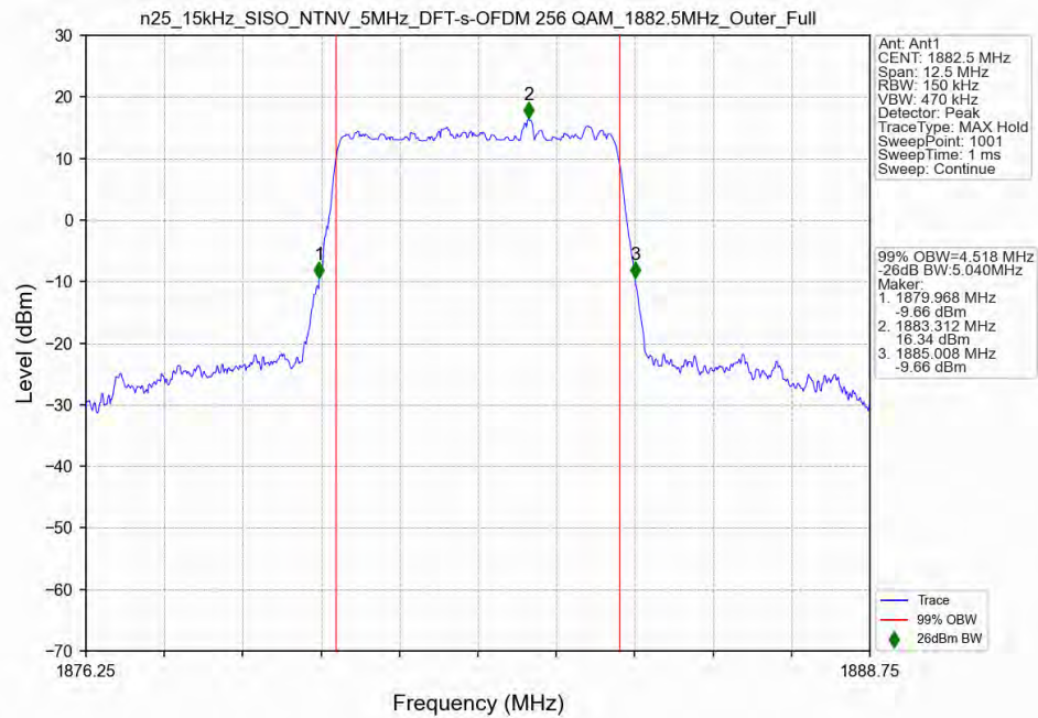
n25_15kHz_SISO_NTNV_5MHz_DFT-s-OFDM_256_QAM_1882.5MHz_Outer_Full
