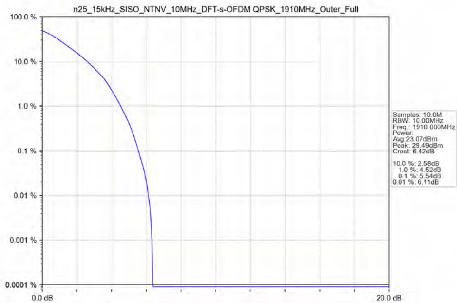
n25_15kHz_SISO_NTNV_10MHz_DFT-s-OFDM_QPSK_1910MHz_Outer_Full
