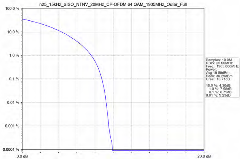
n25_15kHz_SISO_NTNV_20MHz_CP-OFDM 64 QAM_1905MHz_Outer_Full
