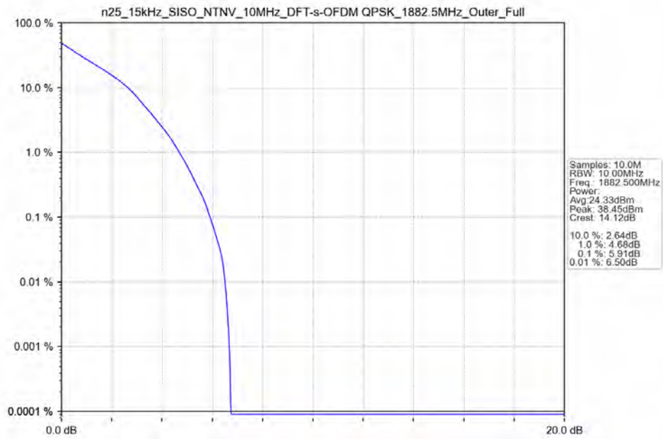
n25_15kHz_SISO_NTNV_10MHz_DFT-s-OFDM_QPSK_1882.5MHz_Outer_Full
