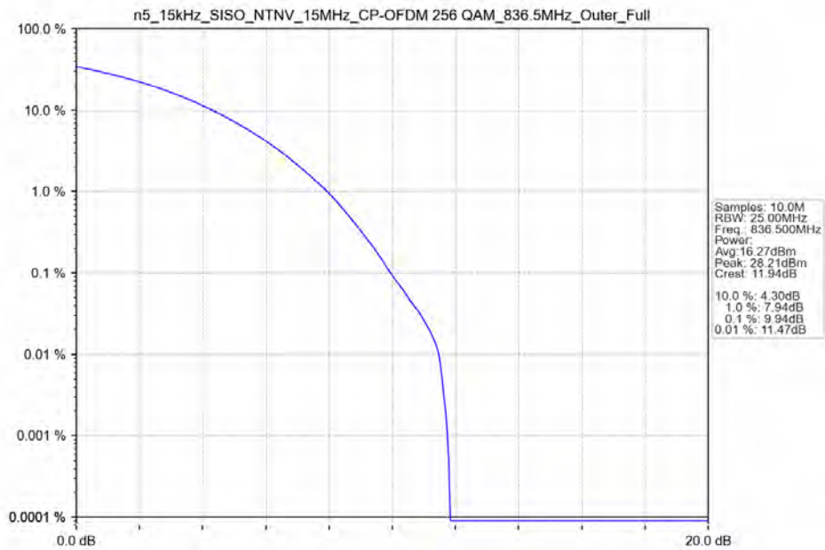
n5_15kHz_SISO_NTNV_15MHz_CP-OFDM_256_QAM_836.5MHz_Outer_Full
