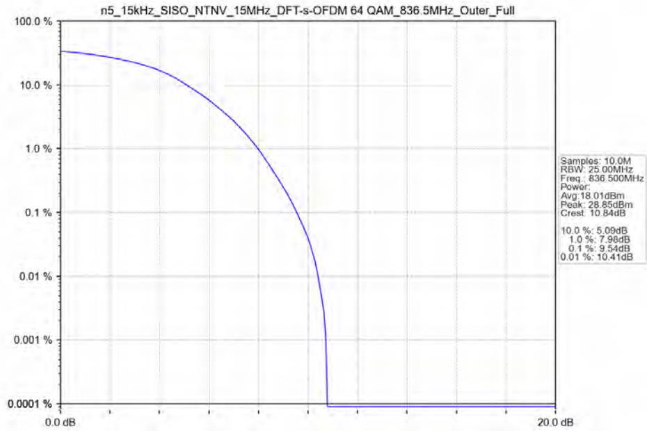
n5_15kHz_SISO_NTNV_15MHz_DFT-s-OFDM_64_QAM_836.5MHz_Outer_Full
