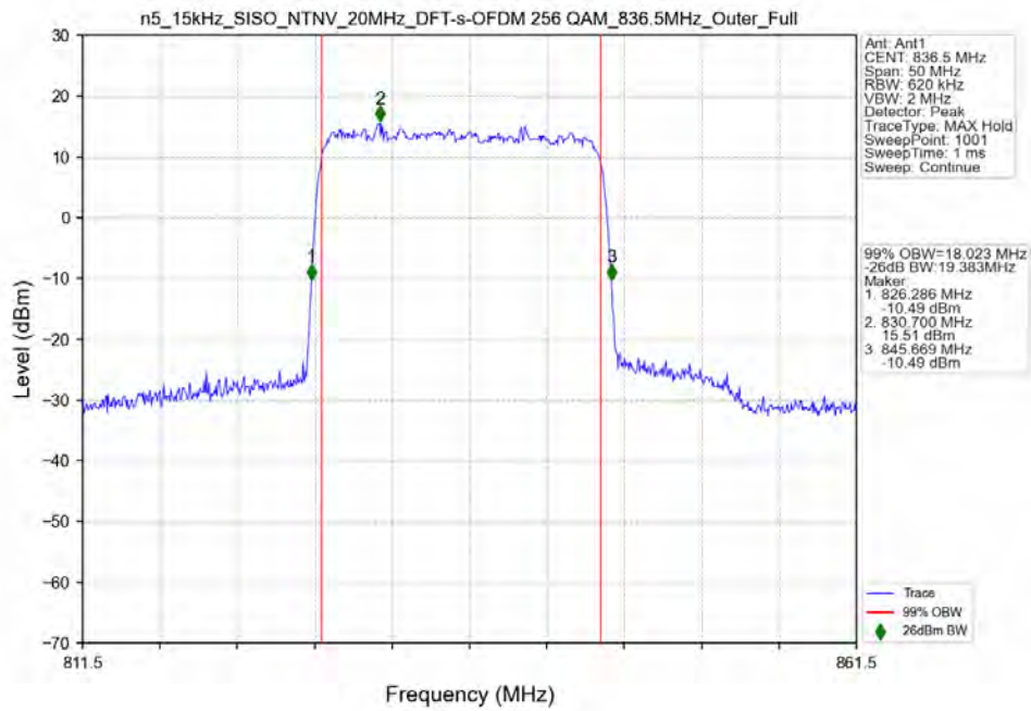
n5_15kHz_SISO_NTNV_20MHz_DFT-s-OFDM_256_QAM_836.5MHz_Outer_Full
