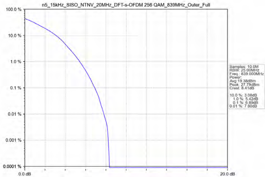
n5_15kHz_SISO_NTNV_20MHz_DFT-s-OFDM 256 QAM_839MHz_Outer_Full
