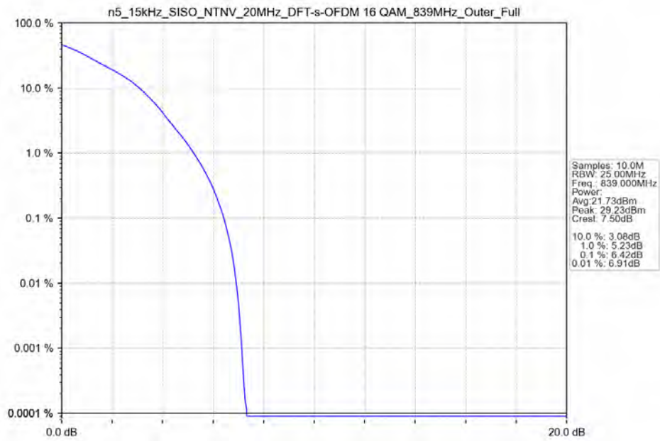
n5_15kHz_SISO_NTNV_20MHz_DFT-s-OFDM_16_QAM_839MHz_Outer_Full
