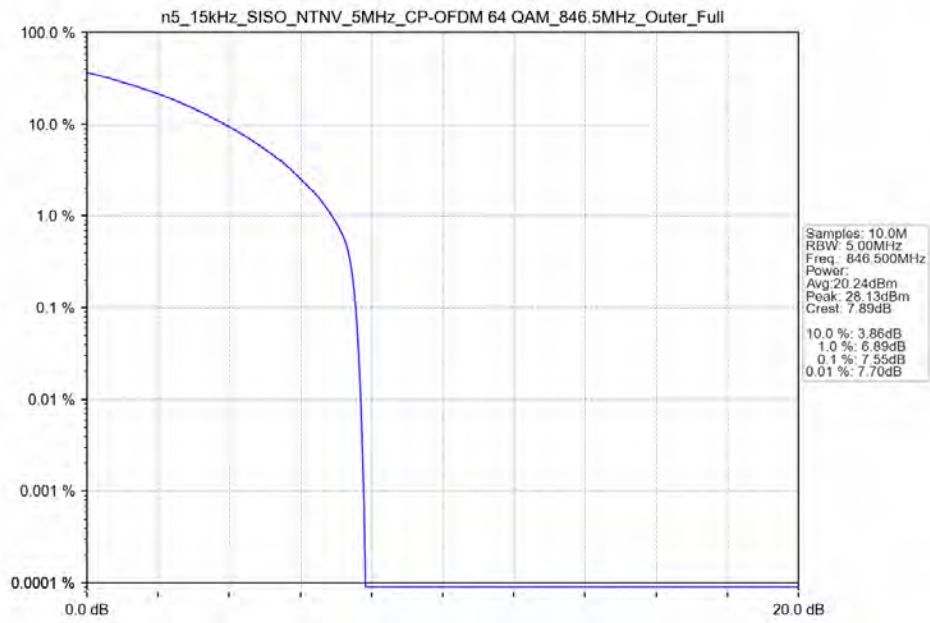
n5_15kHz_SISO_NTNV_5MHz_CP-OFDM 64 QAM_846.5MHz_Outer_Full
