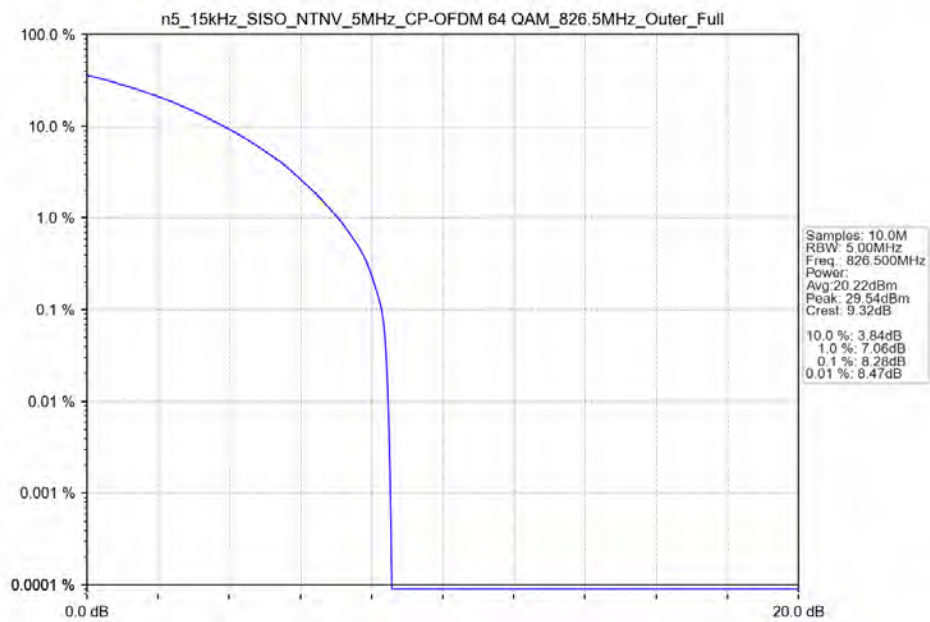
n5_15kHz_SISO_NTNV_5MHz_CP-OFDM 64 QAM_826.5MHz_Outer_Full
