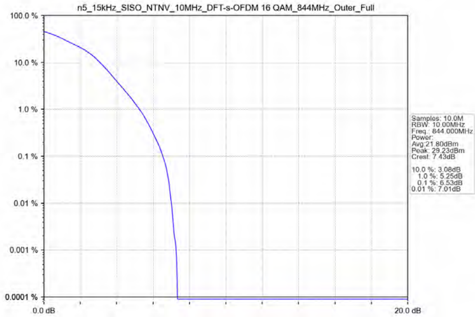
n5_15kHz_SISO_NTNV_10MHz_DFT-s-OFDM_16_QAM_844MHz_Outer_Full
