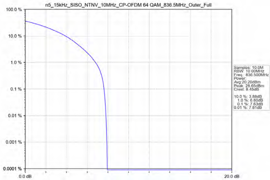
n5_15kHz_SISO_NTNV_10MHz_CP-OFDM 64 QAM_836.5MHz_Outer_Full
