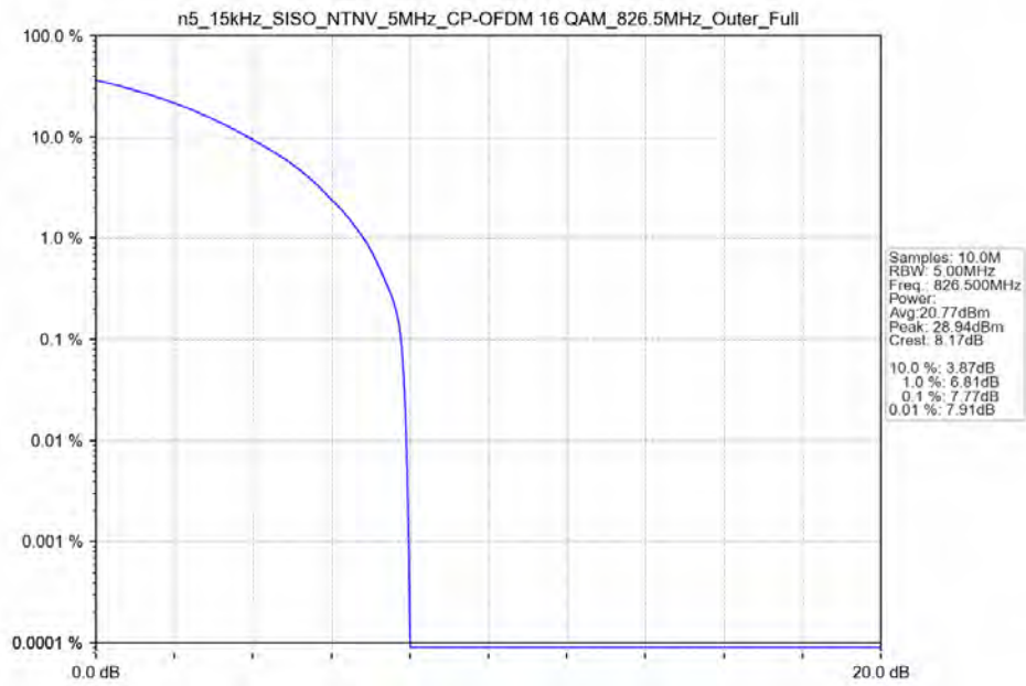
n5_15kHz_SISO_NTNV_5MHz_CP-OFDM 16 QAM_826.5MHz_Outer_Full
