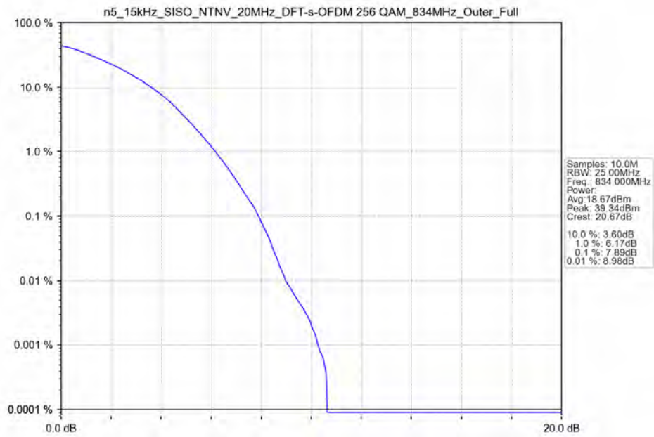
n5_15kHz_SISO_NTNV_20MHz_DFT-s-OFDM_256_QAM_834MHz_Outer_Full
