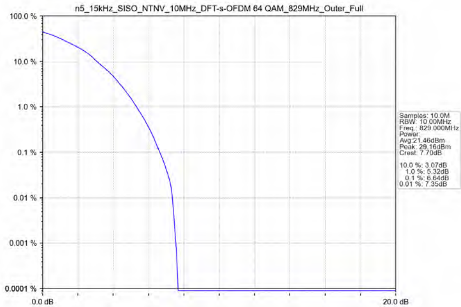
n5_15kHz_SISO_NTNV_10MHz_DFT-s-OFDM_64_QAM_829MHz_Outer_Full
