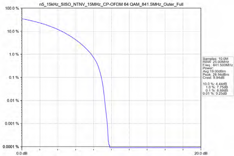
n5_15kHz_SISO_NTNV_15MHz_CP-OFDM 64 QAM_841.5MHz_Outer_Full
