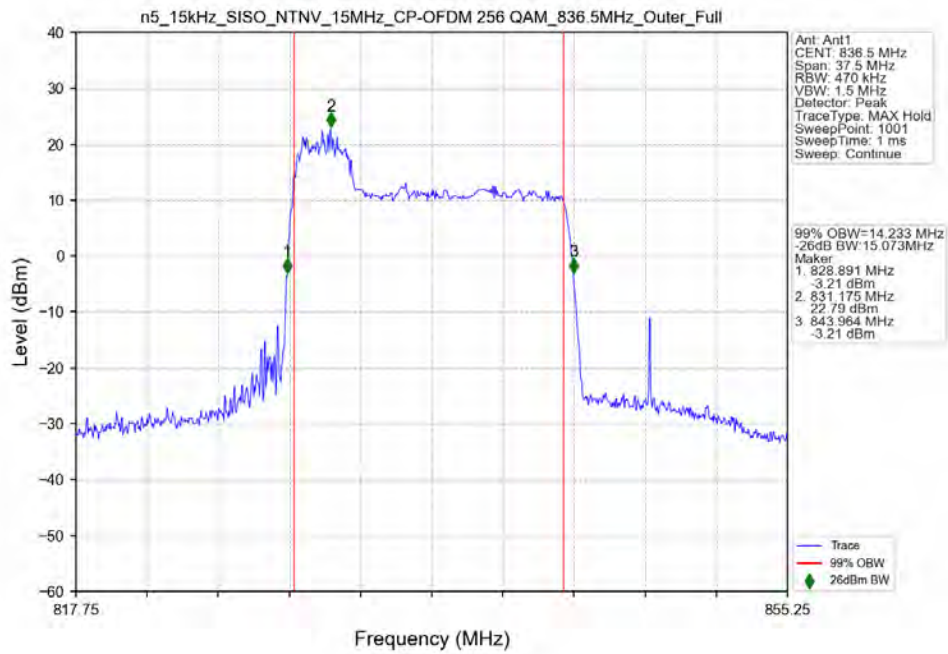
n5_15kHz_SISO_NTNV_15MHz_CP-OFDM_256_QAM_836.5MHz_Outer_Full
