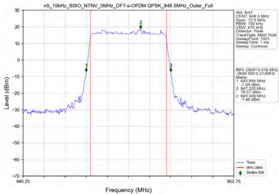
n5_15kHz_SISO_NTNV_5MHz_DFT-s-OFDM QPSK_846.5MHz_Outer_Full
