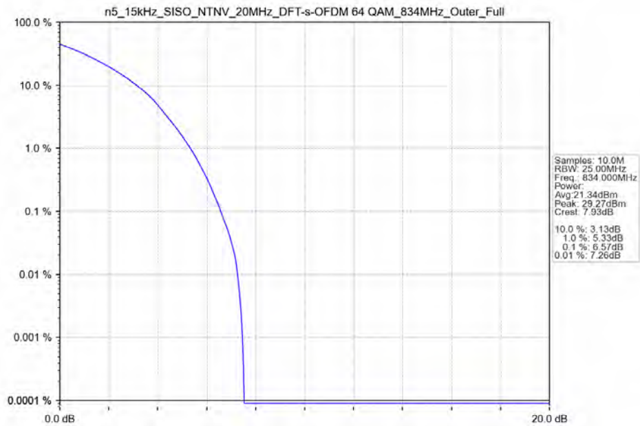
n5_15kHz_SISO_NTNV_20MHz_DFT-s-OFDM_64_QAM_834MHz_Outer_Full
