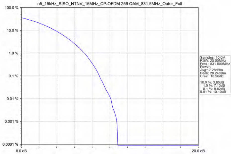
n5_15kHz_SISO_NTNV_15MHz_CP-OFDM_256_QAM_831.5MHz_Outer_Full
