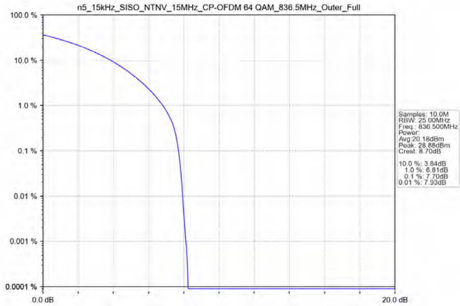
n5_15kHz_SISO_NTNV_15MHz_CP-OFDM 64 QAM_836.5MHz_Outer_Full
