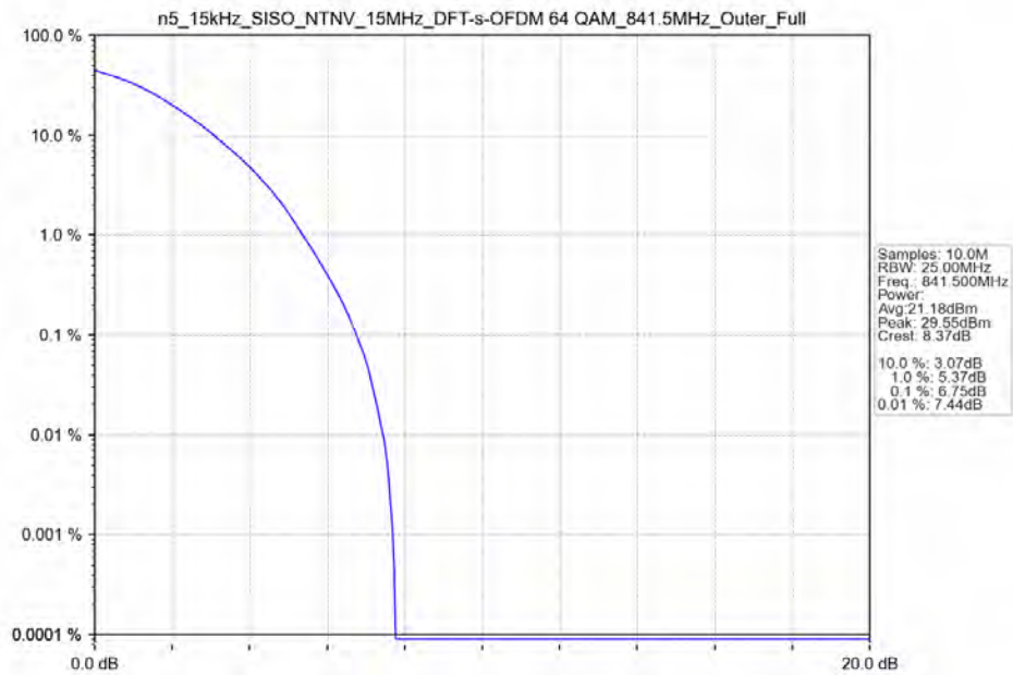
n5_15kHz_SISO_NTNV_15MHz_DFT-s-OFDM_64_QAM_841.5MHz_Outer_Full
