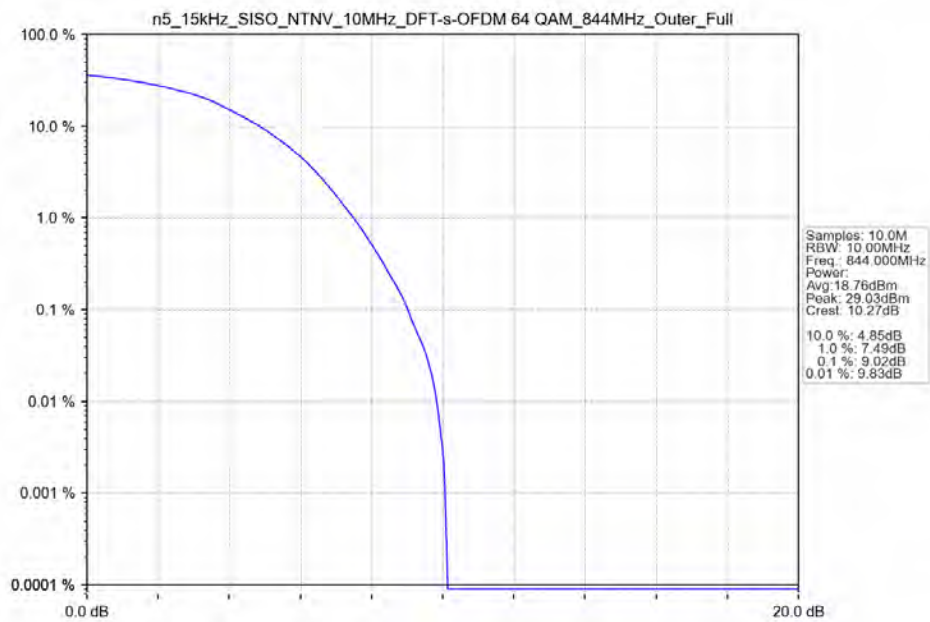
n5_15kHz_SISO_NTNV_10MHz_DFT-s-OFDM 64 QAM_844MHz_Outer_Full
