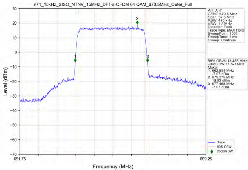
n71_15kHz_SISO_NTNV_15MHz_DFT-s-OFDM 64 QAM_670.5MHz_Outer_Full
