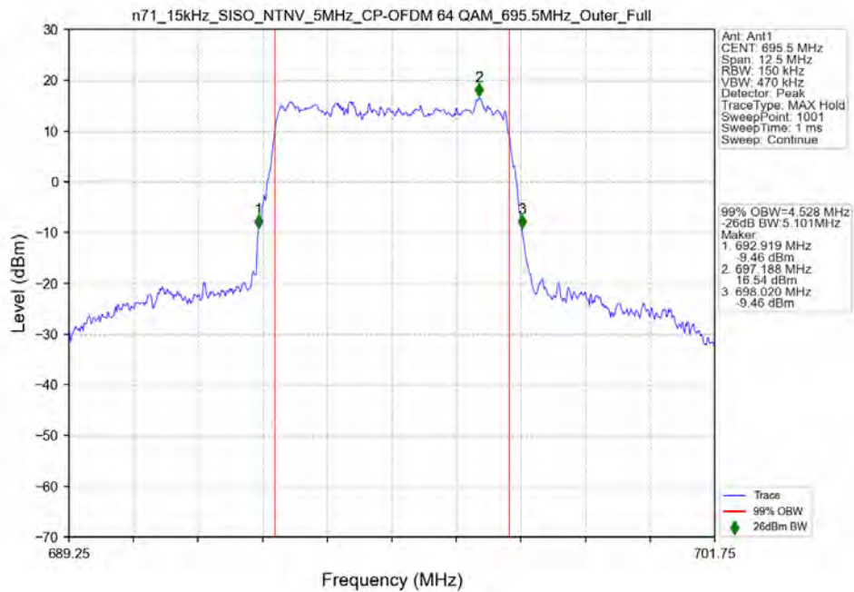
n71_15kHz_SISO_NTNV_5MHz_CP-OFDM 64 QAM 695.5MHz_Outer_Full
