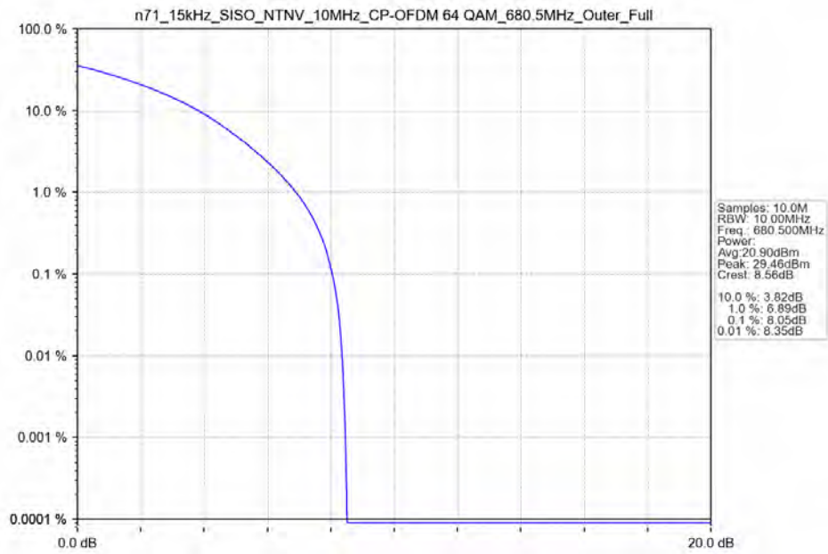
n71_15kHz_SISO_NTNV_10MHz_CP-OFDM 64 QAM_680.5MHz_Outer_Full
