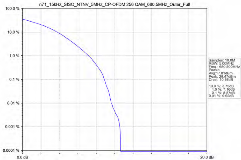
n71_15kHz_SISO_NTNV_5MHz_CP-OFDM 256 QAM_680.5MHz_Outer_Full
