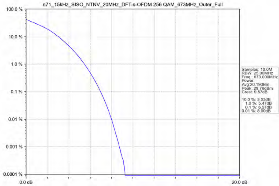
n71_15kHz_SISO_NTNV_20MHz_DFT-s-OFDM_256_QAM_673MHz_Outer_Full
