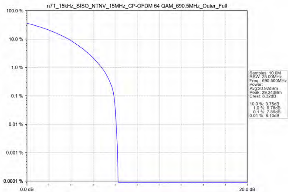
n71_15kHz_SISO_NTNV_15MHz_CP-OFDM 64 QAM_690.5MHz_Outer_Full
