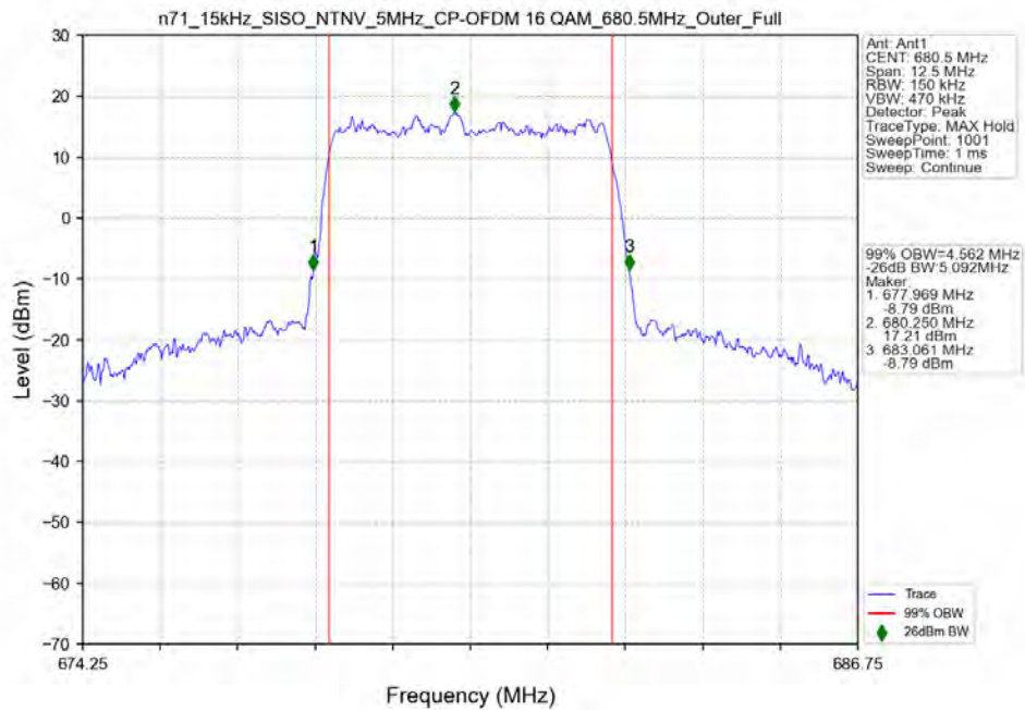
n71_15kHz_SISO_NTNV_5MHz_CP-OFDM 16 QAM 680.5MHz_Outer_Full
