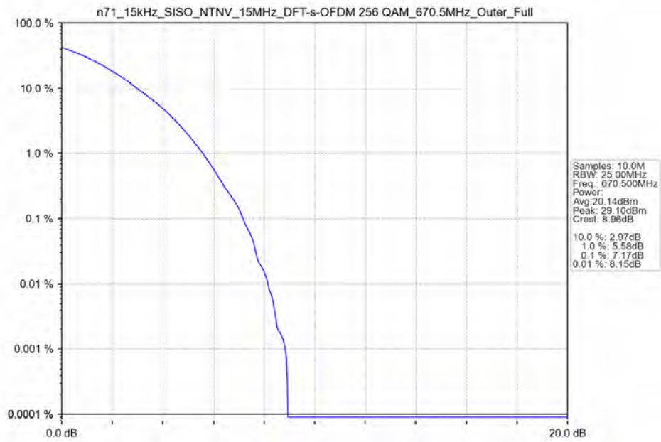
n71_15kHz_SISO_NTNV_15MHz_DFT-s-OFDM_256_QAM_670.5MHz_Outer_Full
