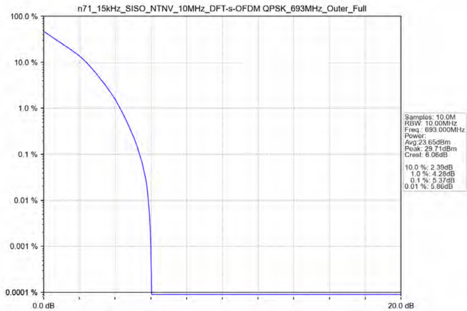
n71_15kHz_SISO_NTNV_10MHz_DFT-s-OFDM_QPSK_693MHz_Outer_Full
