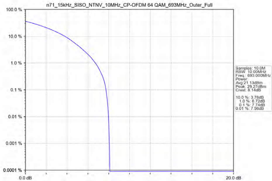
n71_15kHz_SISO_NTNV_10MHz_CP-OFDM 64 QAM_693MHz_Outer_Full
