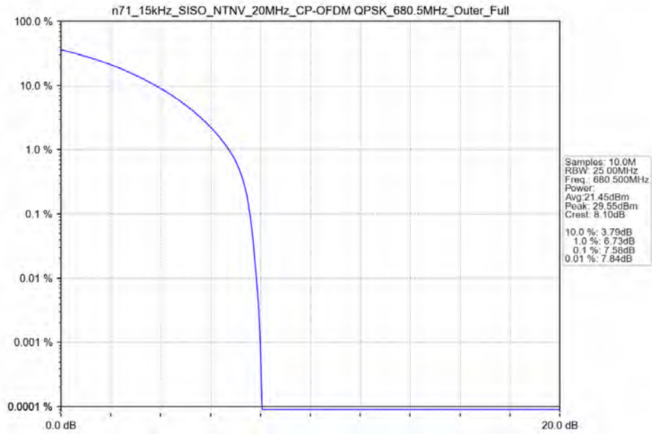
n71_15kHz_SISO_NTNV_20MHz_CP-OFDM_QPSK_680.5MHz_Outer_Full
