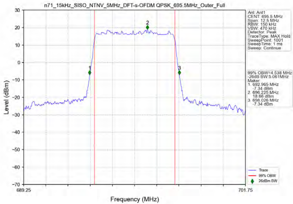
n71_15kHz_SISO_NTNV_5MHz_DFT-s-OFDM_QPSK_695.5MHz_Outer_Full
