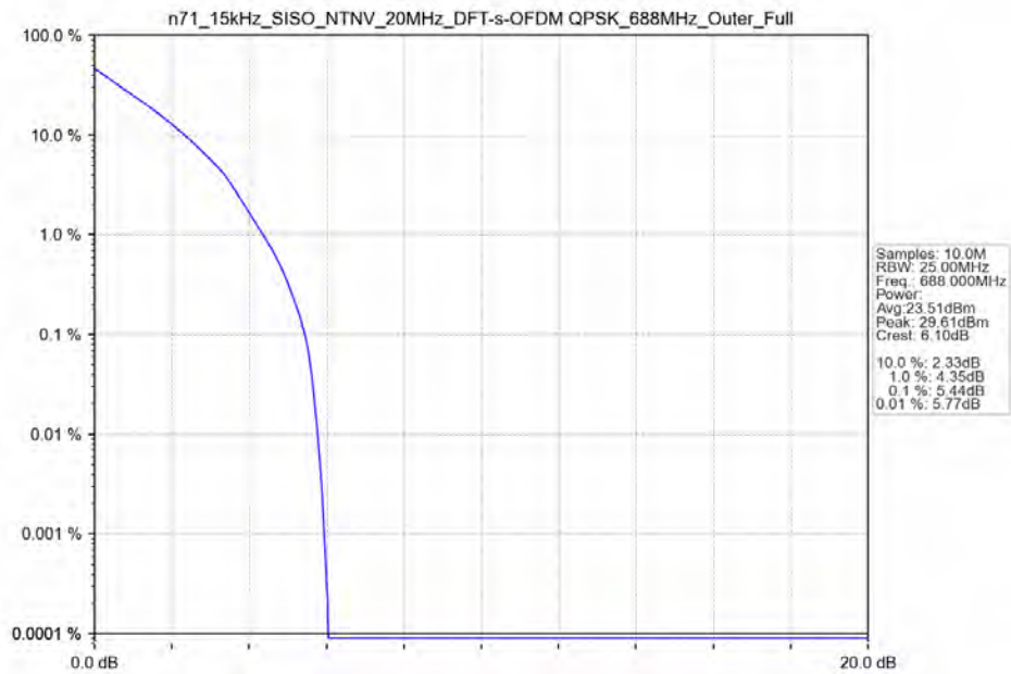
n71_15kHz_SISO_NTNV_20MHz_DFT-s-OFDM_QPSK_688MHz_Outer_Full
