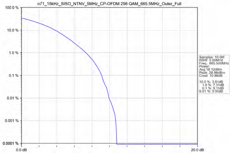
n71_15kHz_SISO_NTNV_5MHz_CP-OFDM 256 QAM_665.5MHz_Outer_Full
