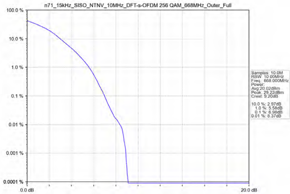
n71_15kHz_SISO_NTNV_10MHz_DFT-s-OFDM_256_QAM_668MHz_Outer_Full
