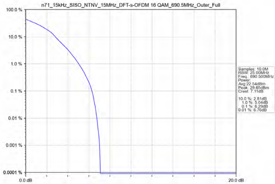
n71_15kHz_SISO_NTNV_15MHz_DFT-s-OFDM_16_QAM_690.5MHz_Outer_Full
