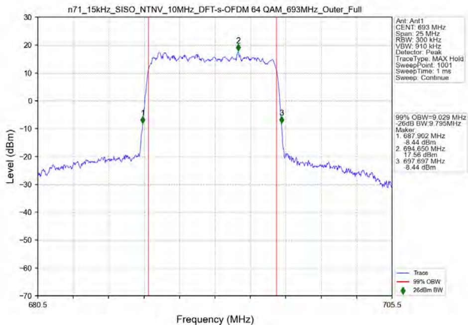
n71_15kHz_SISO_NTNV_10MHz_DFT-s-OFDM_64_QAM_693MHz_Outer_Full
