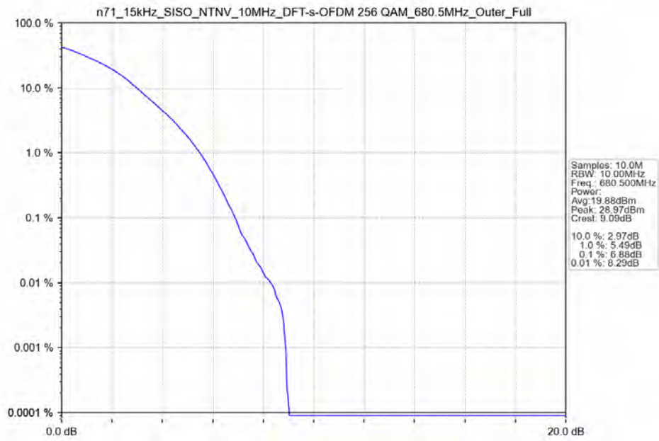
n71_15kHz_SISO_NTNV_10MHz_DFT-s-OFDM_256_QAM_680.5MHz_Outer_Full
