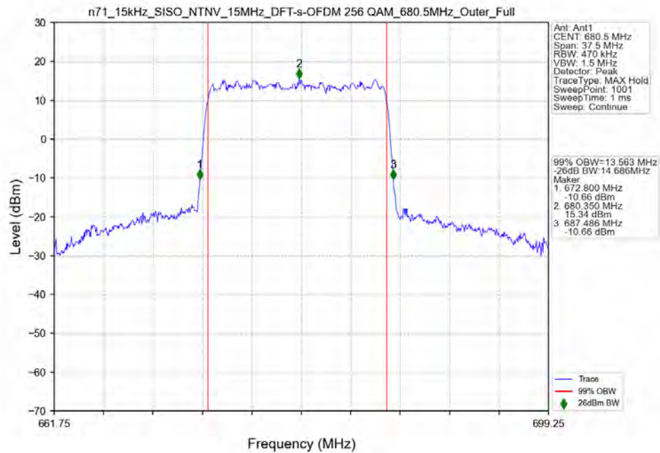
n71_15kHz_SISO_NTNV_15MHz_DFT-s-OFDM_256_QAM_680.5MHz_Outer_Full
