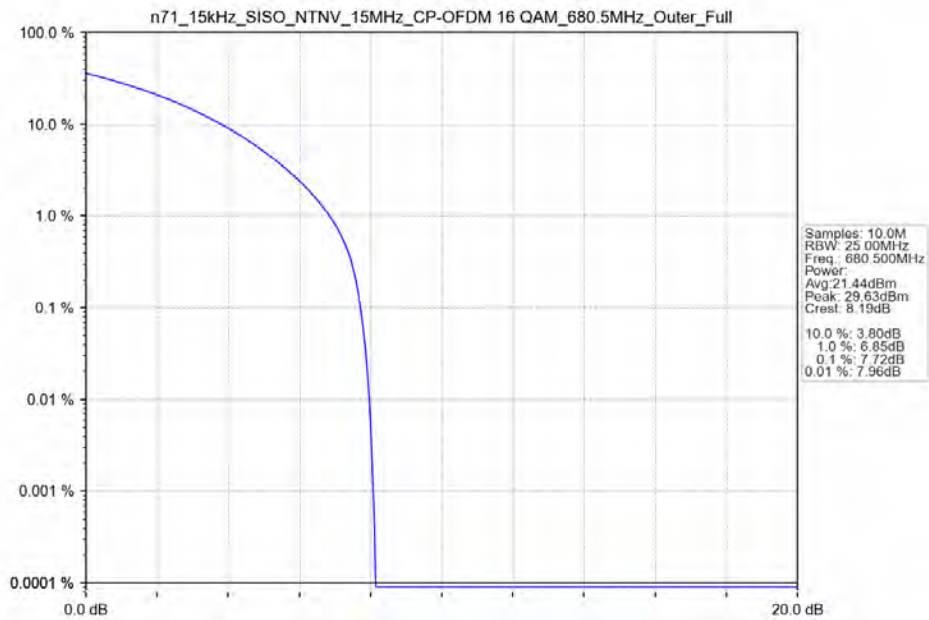
n71_15kHz_SISO_NTNV_15MHz_CP-OFDM_16_QAM_680.5MHz_Outer_Full
