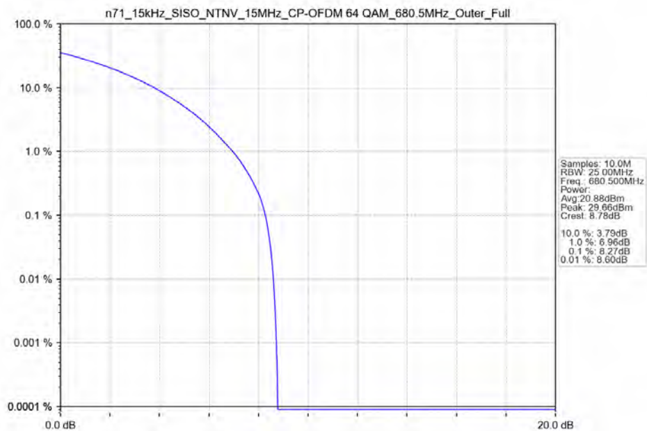
n71_15kHz_SISO_NTNV_15MHz_CP-OFDM 64 QAM_680.5MHz_Outer_Full
