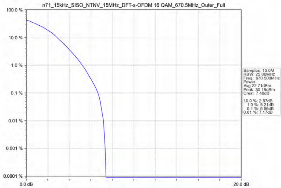
n71_15kHz_SISO_NTNV_15MHz_DFT-s-OFDM_16_QAM_670.5MHz_Outer_Full
