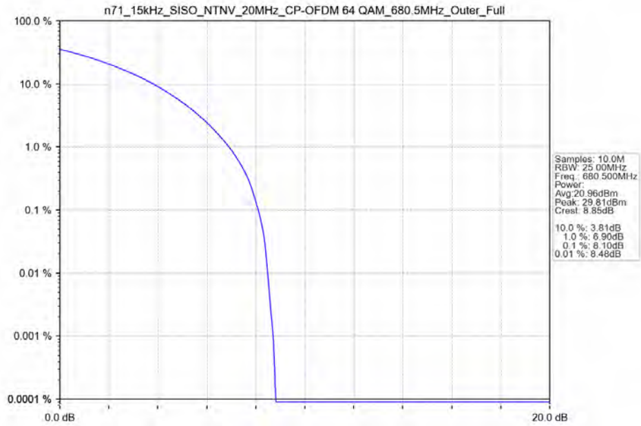
n71_15kHz_SISO_NTNV_20MHz_CP-OFDM 64 QAM_680.5MHz_Outer_Full
