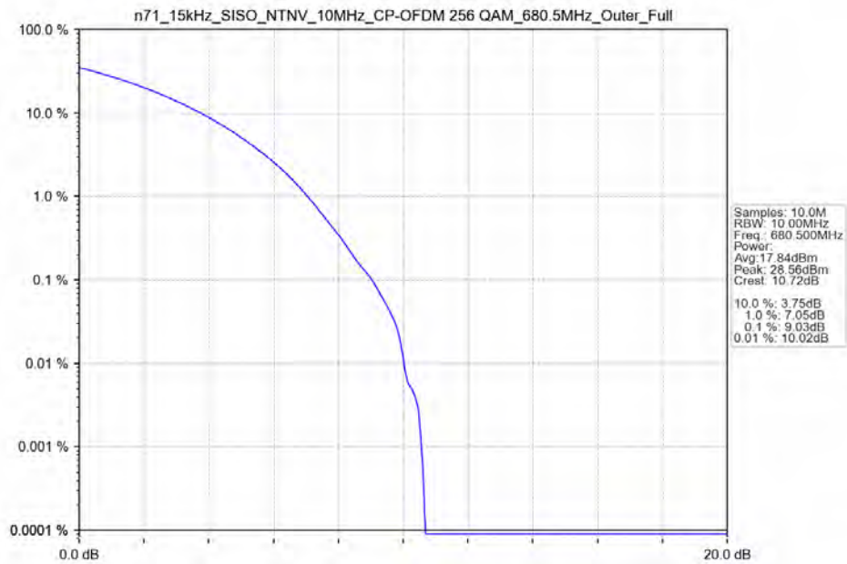
n71_15kHz_SISO_NTNV_10MHz_CP-OFDM 256 QAM_680.5MHz_Outer_Full
