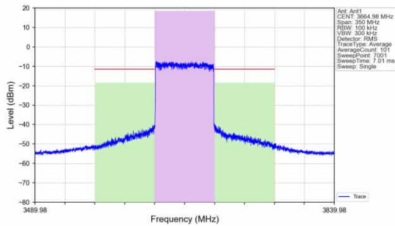
n78d_30kHz_SISO_NTNV_70MHz_CP-OFDM QPSK_3664.98MHz_Outer_Full_Ant1
