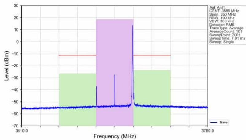
n78d_30kHz_SISO_NTNV_70MHz_CP-OFDM QPSK_3585MHz_Edge_1RB_Right_Ant1
