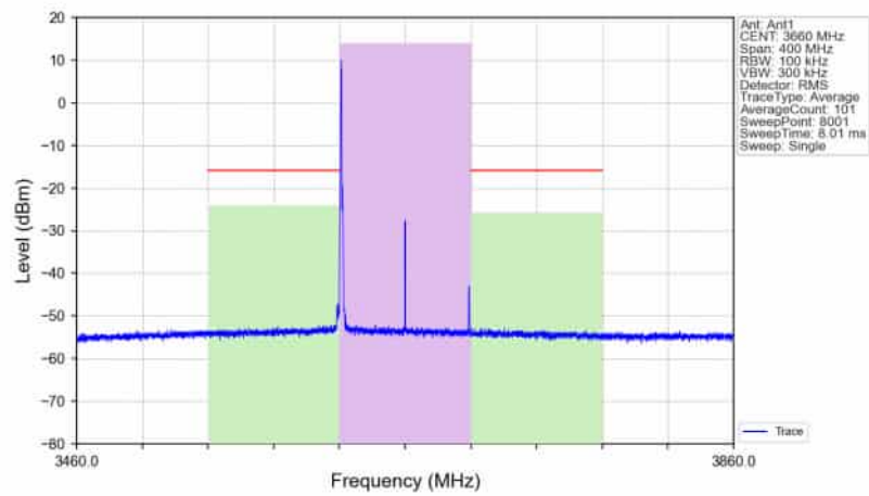
n78d_30kHz_SISO_NTNV_80MHz_CP-OFDM_256_QAM_3660MHz_Edge_1RB_Left_Ant1
