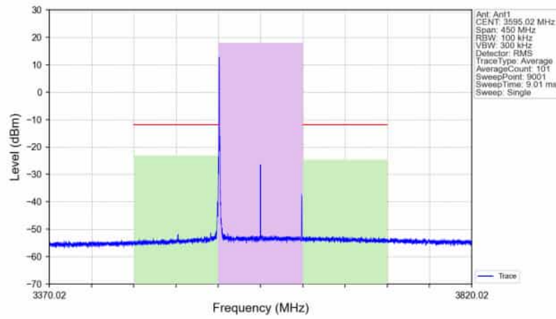
n78d_30kHz_SISO_NTNV_90MHz_DFT-s-OFDM_64_QAM_3595.02MHz_Edge_1RB_Left_Ant1
