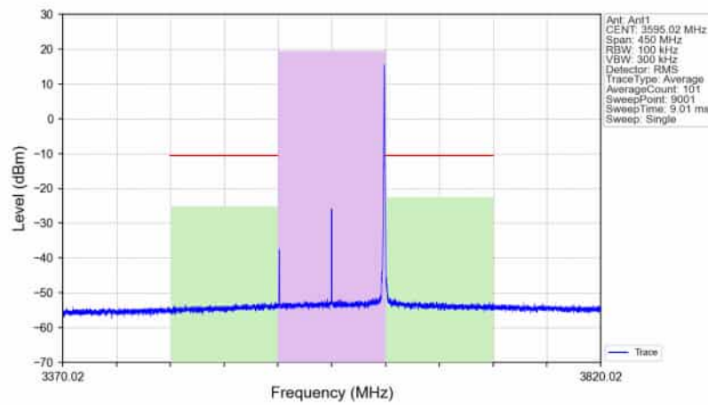
n78d_30kHz_SISO_NTNV_90MHz_DFT-s-OFDM_64_QAM_3595.02MHz_Edge_1RB_Right_Ant1
