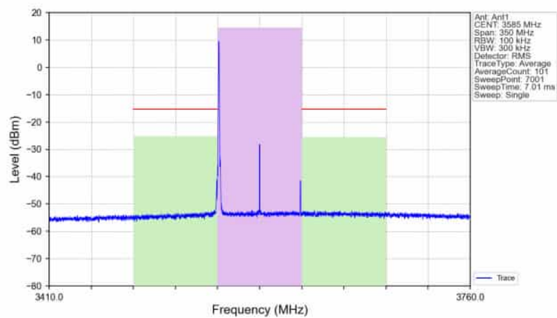
n78d_30kHz_SISO_NTNV_70MHz_CP-OFDM_256_QAM_3585MHz_Edge_1RB_Left_Ant1
