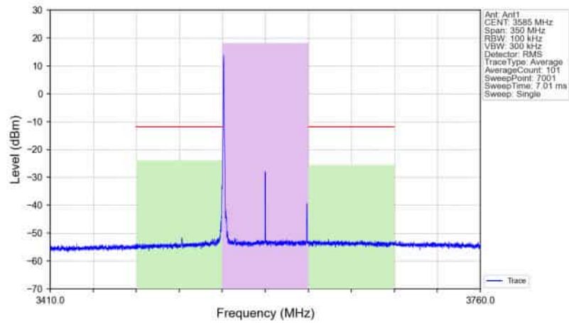
n78d_30kHz_SISO_NTNV_70MHz_CP-OFDM QPSK_3585MHz_Edge_1RB_Left_Ant1
