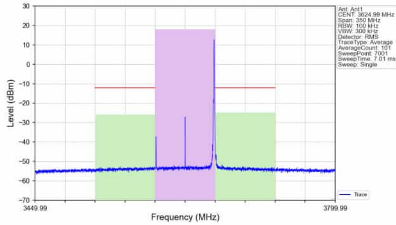
n78d_30kHz_SISO_NTNV_70MHz_CP-OFDM QPSK_3624.99MHz_Edge_1RB_Right_Ant1
