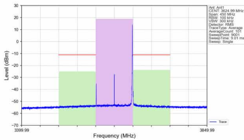
n78d_30kHz_SISO_NTNV_90MHz_DFT-s-OFDM_16_QAM_3624.99MHz_Edge_1RB_Right_Ant1
