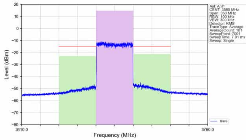
n78d_30kHz_SISO_NTNV_70MHz_CP-OFDM_256_QAM_3585MHz_Outer_Full_Ant1
