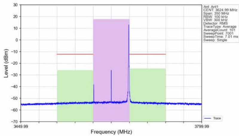
n78d_30kHz_SISO_NTNV_70MHz_CP-OFDM_16_QAM_3624.99MHz_Edge_1RB_Right_Ant1
