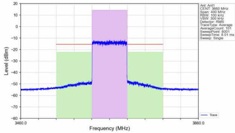
n78d_30kHz_SISO_NTNV_80MHz_CP-OFDM_256_QAM_3660MHz_Outer_Full_Ant1
