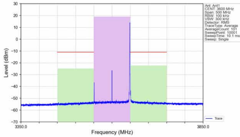
n78d_30kHz_SISO_NTNV_100MHz_CP-OFDM 16 QAM_3600MHz_Edge_Right_Ant1
