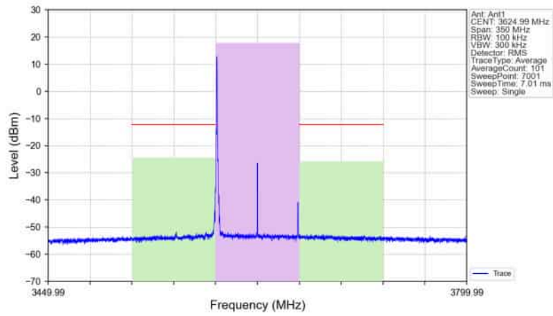
n78d_30kHz_SISO_NTNV_70MHz_CP-OFDM_16_QAM_3624.99MHz_Edge_1RB_Left_Ant1
