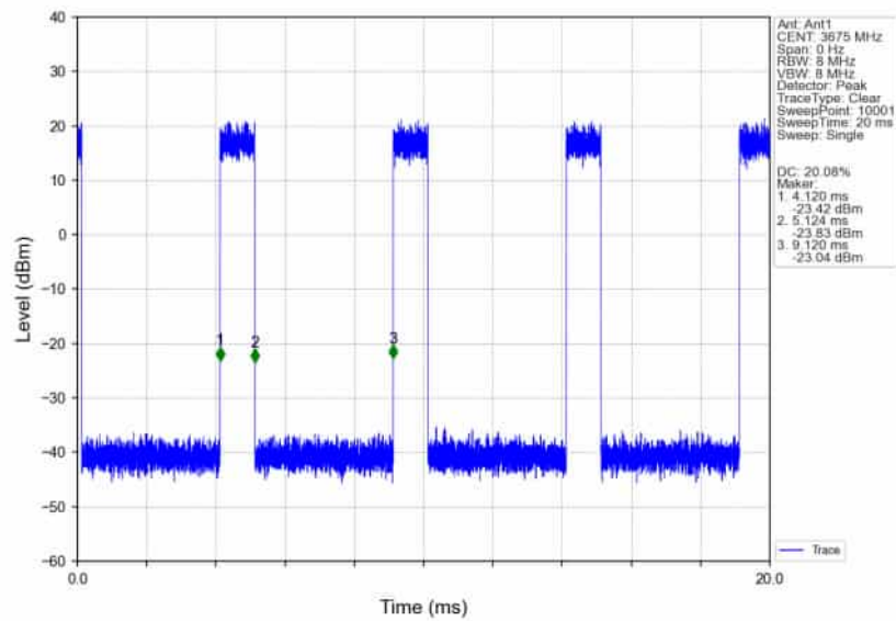
n78d_30kHz_SISO_NTNV_50MHz_CP-OFDM_256_QAM_3675MHz_Inner_Full_Ant1
