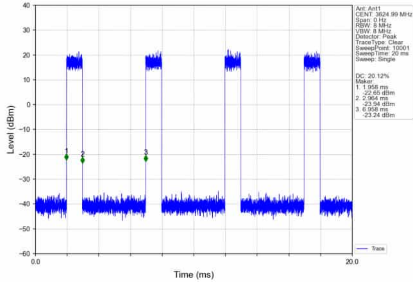
n78d_30kHz_SISO_NTNV_50MHz_CP-OFDM QPSK_3624.99MHz_Inner_Full_Ant1
