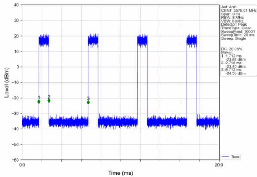
n78d_30kHz_SISO_NTNV_50MHz_CP-OFDM_256_QAM_3575.01MHz_Inner_Full_Ant1
