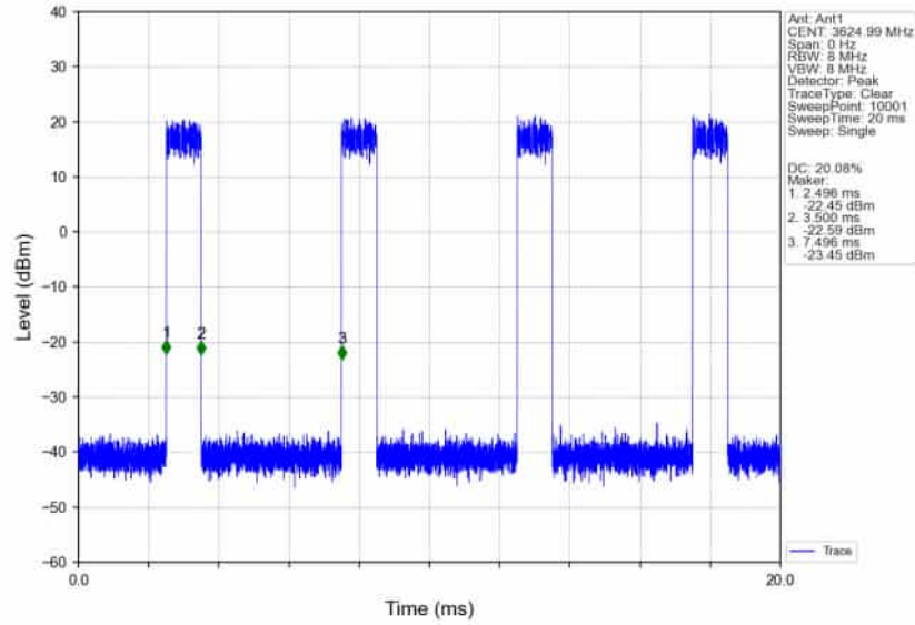
n78d_30kHz_SISO_NTNV_60MHz_DFT-s-OFDM_16_QAM_3624.99MHz_Inner_Full_Ant1
