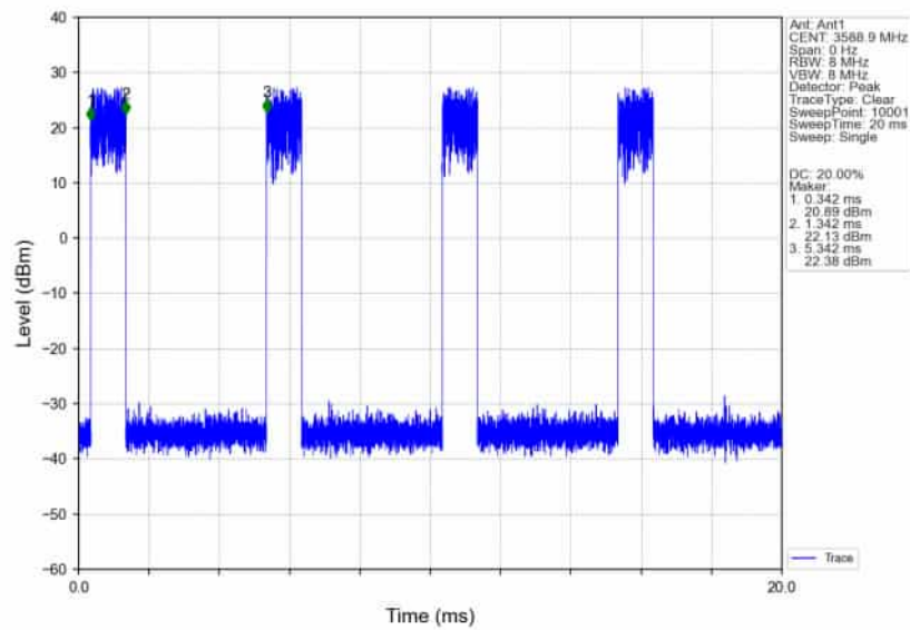
n78d_30kHz_SISO_NTNV_40MHz_CP-OFDM_QPSK_3570MHz_Edge_1RB_Right_Ant1
