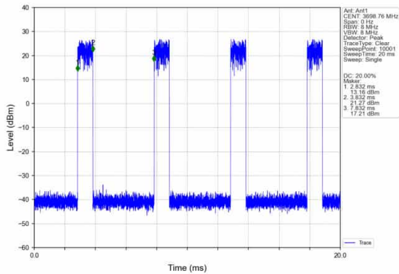
n78d_30kHz_SISO_NTNV_50MHz_DFT-s-OFDM_16_QAM_3675MHz_Edge_1RB_Right_Ant1
