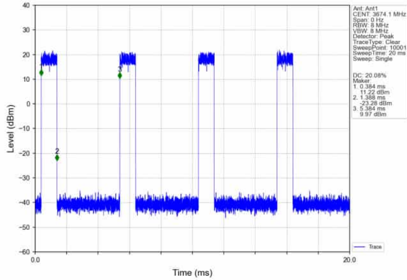
n78d_30kHz_SISO_NTNV_50MHz_DFT-s-OFDM 16 QAM 3675MHz_Inner_Full_Ant1
