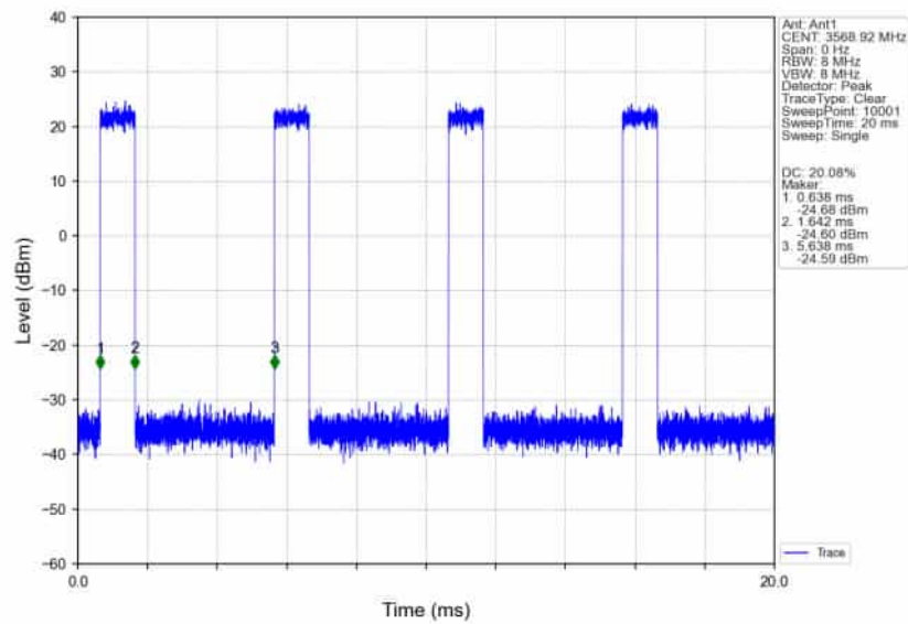
n78d_30kHz_SISO_NTNV_40MHz_DFT-s-OFDM_QPSK_3570MHz_Inner_Full_Ant1
