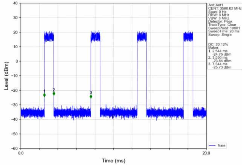
n78d_30kHz_SISO_NTNV_60MHz_DFT-s-OFDM_64_QAM_3580.02MHz_Inner_Full_Ant1
