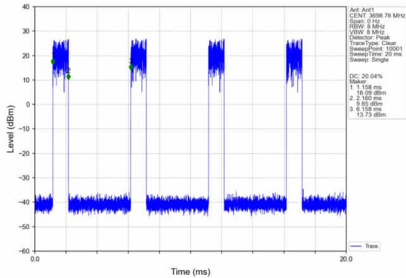
n78d_30kHz_SISO_NTNV_50MHz_CP-OFDM_64_QAM_3675MHz_Edge_1RB_Right_Ant1
