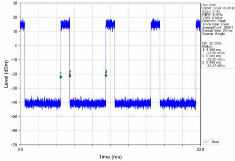
n78d_30kHz_SISO_NTNV_40MHz_CP-OFDM_256_QAM_3624.99MHz_Inner_Full_Ant1
