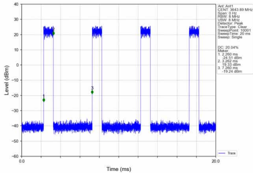
n78d_30kHz_SISO_NTNV_40MHz_DFT-s-OFDM_QPSK_3624.99MHz_Edge_1RB_Right_Ant1
