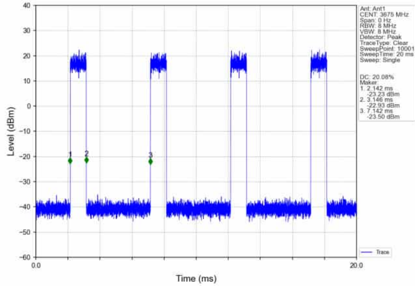
n78d_30kHz_SISO_NTNV_50MHz_CP-OFDM 64 QAM_3675MHz_Inner_Full_Ant1
