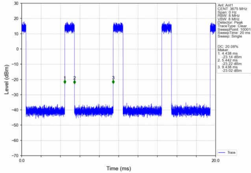
n78d_30kHz_SISO_NTNV_50MHz_CP-OFDM_256_QAM_3675MHz_Inner_Full_Ant1
