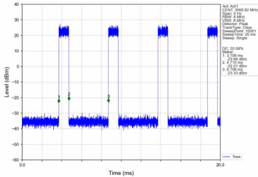
n78d_30kHz_SISO_NTNV_40MHz_CP-OFDM_16_QAM_3570MHz_Inner_Full_Ant1
