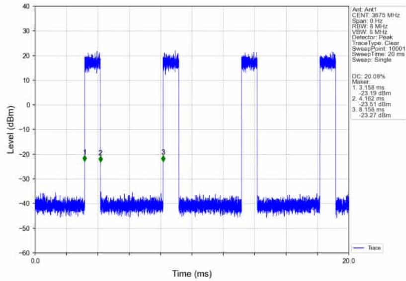
n78d_30kHz_SISO_NTNV_50MHz_CP-OFDM_QPSK_3675MHz_Inner_Full_Ant1
