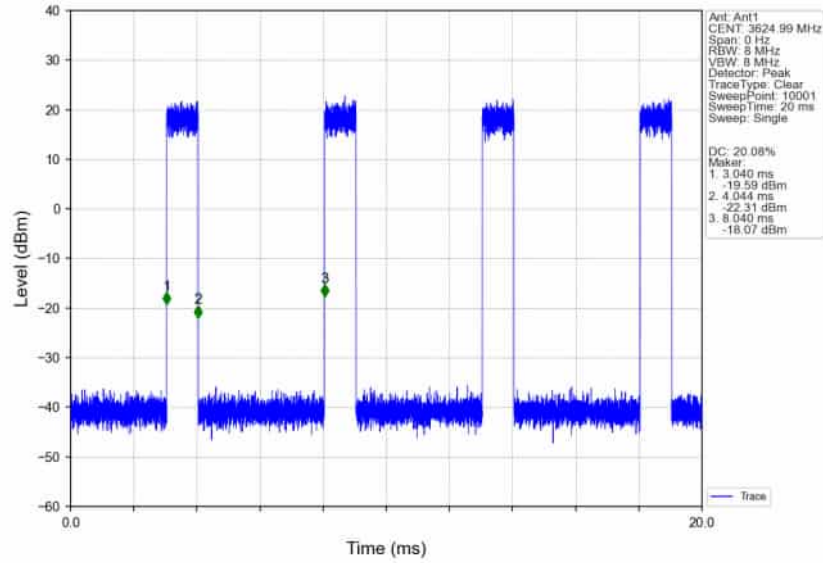
n78d_30kHz_SISO_NTNV_40MHz_CP-OFDM 16 QAM 3624.99MHz_Inner_Full_Ant1
