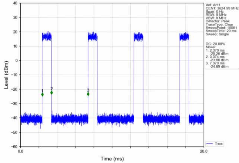
n78d_30kHz_SISO_NTNV_60MHz_DFT-s-OFDM_PI/2_BPSK_3624.99MHz_Inner_Full_Ant1
