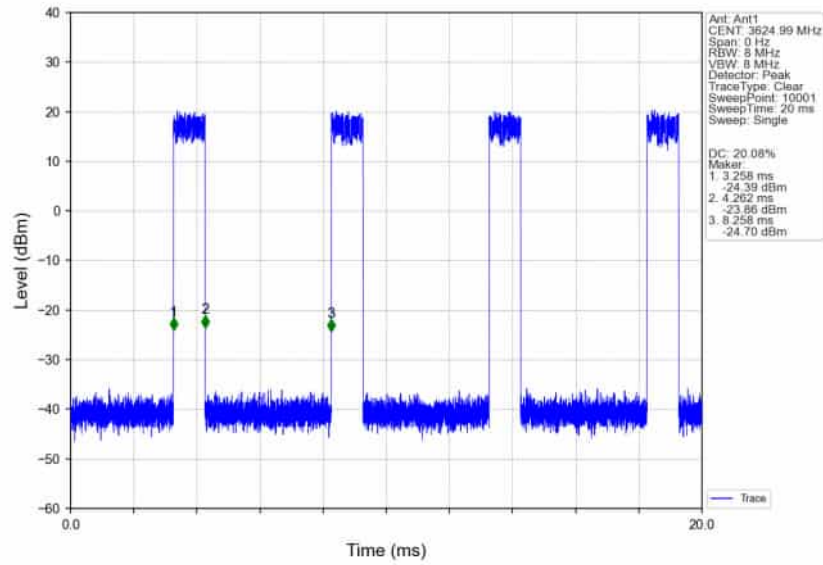
n78d_30kHz_SISO_NTNV_60MHz_DFT-s-OFDM_QPSK_3624.99MHz_Inner_Full_Ant1
