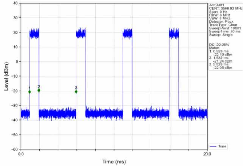
n78d_30kHz_SISO_NTNV_40MHz_DFT-s-OFDM 64 QAM 3570MHz_Inner_Full_Ant1
