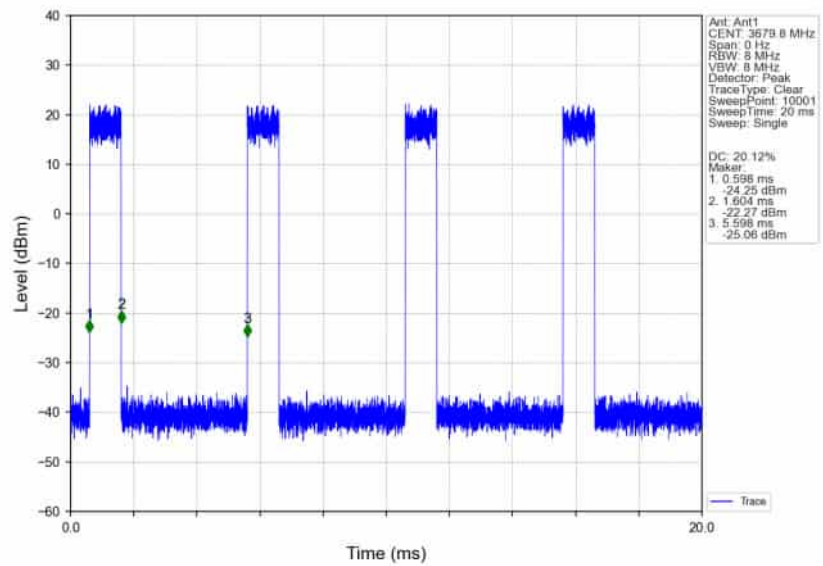
n78d_30kHz_SISO_NTNV_40MHz_CP-OFDM_256_QAM_3679.98MHz_Inner_Full_Ant1
