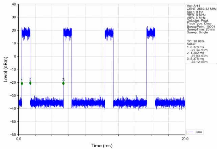
n78d_30kHz_SISO_NTNV_40MHz_CP-OFDM_256_QAM_3570MHz_Inner_Full_Ant1
