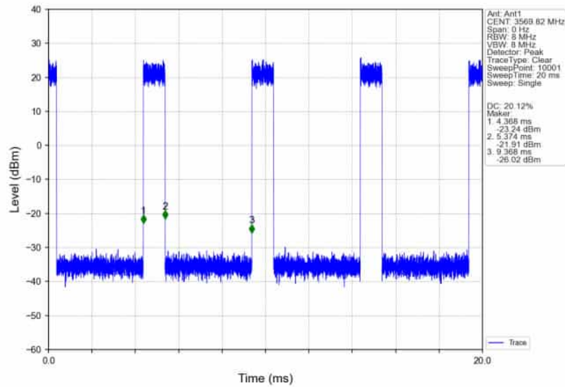
n78d_30kHz_SISO_NTNV_40MHz_CP-OFDM 64 QAM 3570MHz_Inner_Full_Ant1
