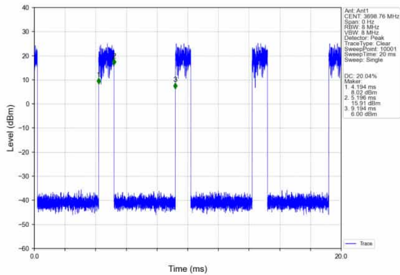
n78d_30kHz_SISO_NTNV_50MHz_DFT-s-OFDM_256_QAM_3675MHz_Edge_1RB_Right_Ant1
