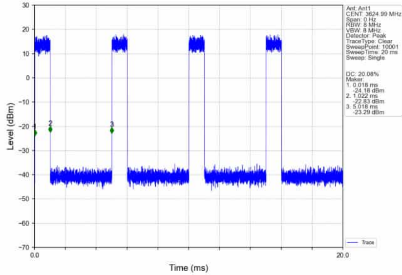
n78d_30kHz_SISO_NTNV_50MHz_CP-OFDM_256_QAM_3624.99MHz_Inner_Full_Ant1
