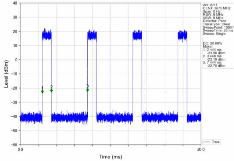
n78d_30kHz_SISO_NTNV_50MHz_CP-OFDM_16_QAM_3675MHz_Inner_Full_Ant1
