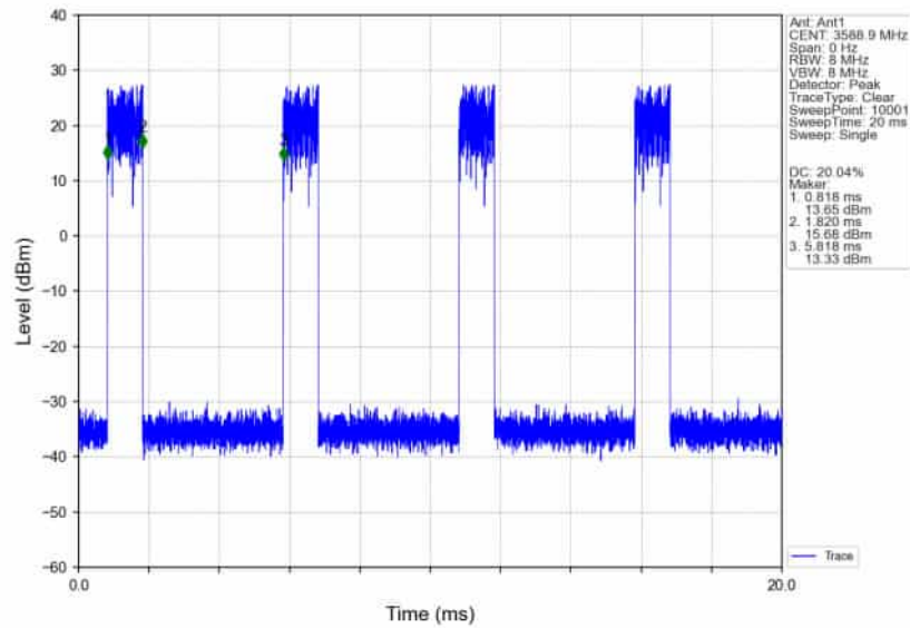
n78d_30kHz_SISO_NTNV_40MHz_CP-OFDM_64_QAM_3570MHz_Edge_1RB_Right_Ant1
