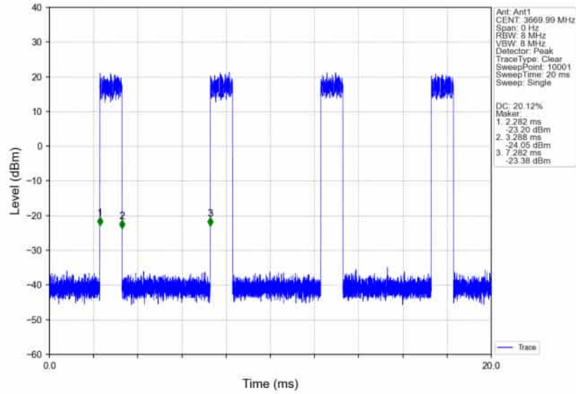
n78d_30kHz_SISO_NTNV_60MHz_DFT-s-OFDM_16_QAM_3669.99MHz_Inner_Full_Ant1
