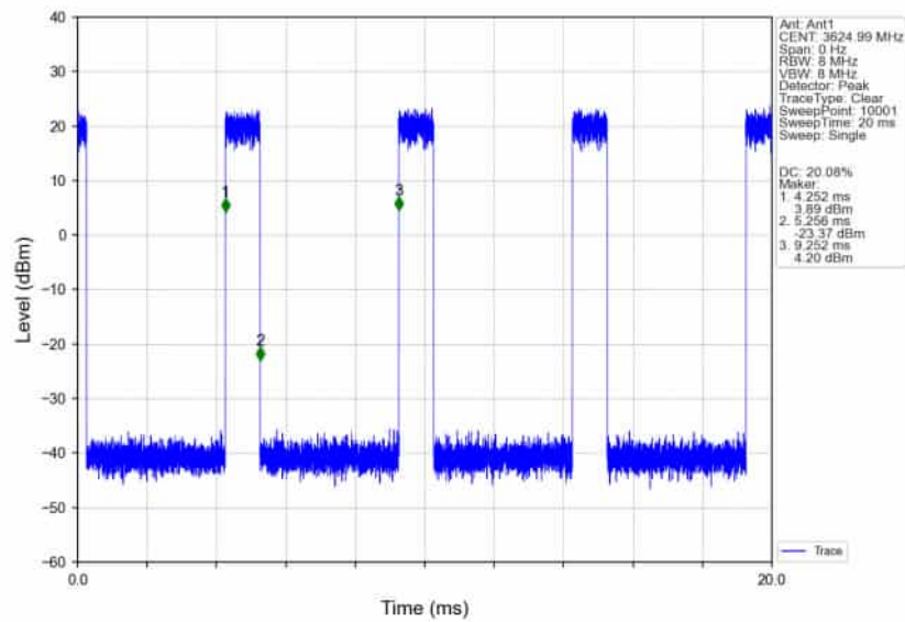
n78d_30kHz_SISO_NTNV_50MHz_CP-OFDM 64 QAM 3624.99MHz_Inner_Full_Ant1
