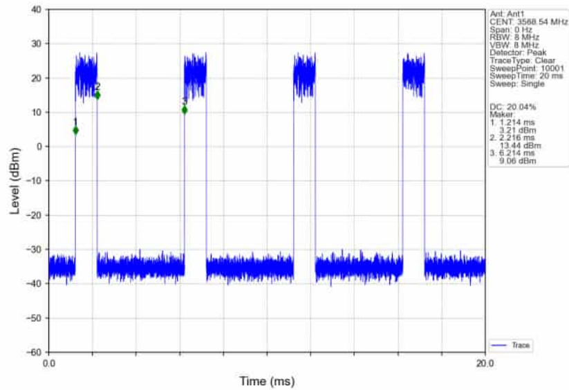
n78d_30kHz_SISO_NTNV_40MHz_DFT-s-OFDM_64_QAM_3570MHz_Inner_1RB_Right_Ant1
