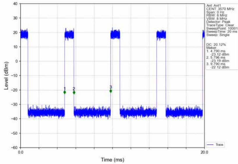
n78d_30kHz_SISO_NTNV_40MHz_CP-OFDM_QPSK_3570MHz_Inner_Full_Ant1
