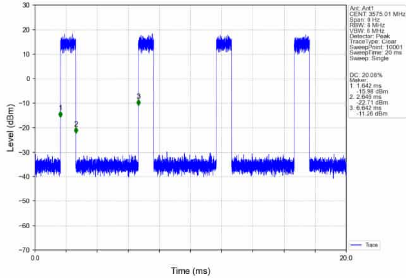
n78d_30kHz_SISO_NTNV_50MHz_CP-OFDM_256_QAM_3575.01MHz_Inner_Full_Ant1
