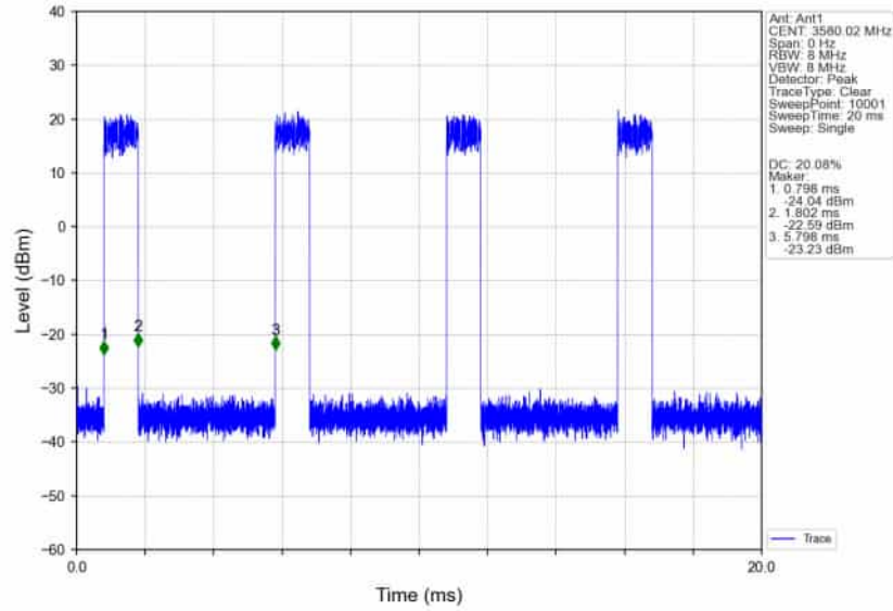
n78d_30kHz_SISO_NTNV_60MHz_DFT-s-OFDM_16_QAM_3580.02MHz_Inner_Full_Ant1
