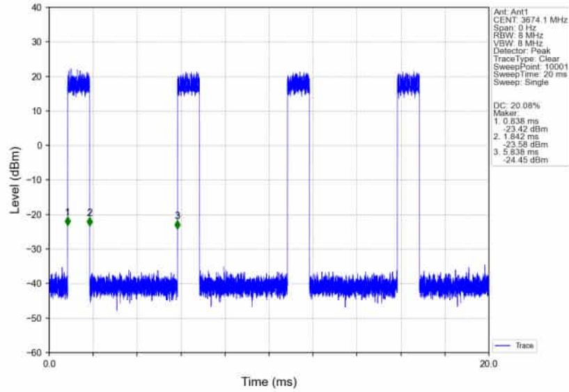
n78d_30kHz_SISO_NTNV_50MHz_DFT-s-OFDM 64 QAM 3675MHz_Inner_Full_Ant1
