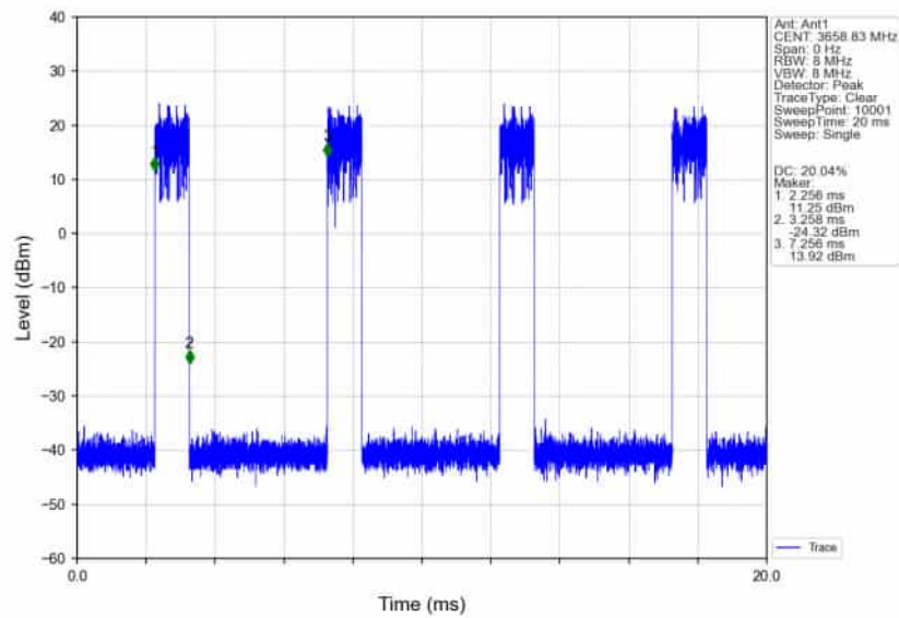
n78d_30kHz_SISO_NTNV_70MHz_CP-OFDM_256_QAM_3624.99MHz_Edge_1RB_Right_Ant1
