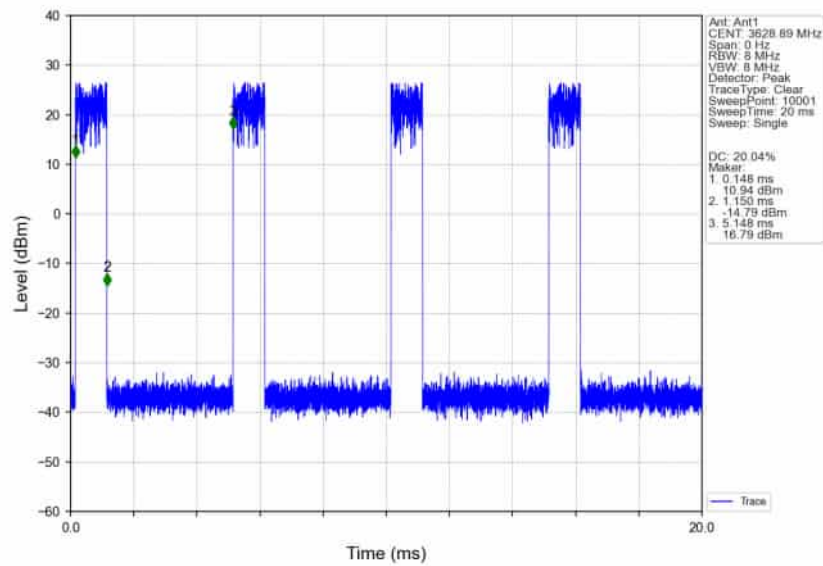
n78d_30kHz_SISO_NTNV_80MHz_DFT-s-OFDM_16_QAM_3590.01MHz_Edge_1RB_Right_Ant1
