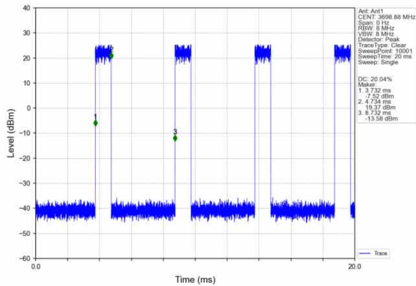
n78d_30kHz_SISO_NTNV_80MHz_DFT-s-OFDM_QPSK_3660MHz_Edge_1RB_Right_Ant1
