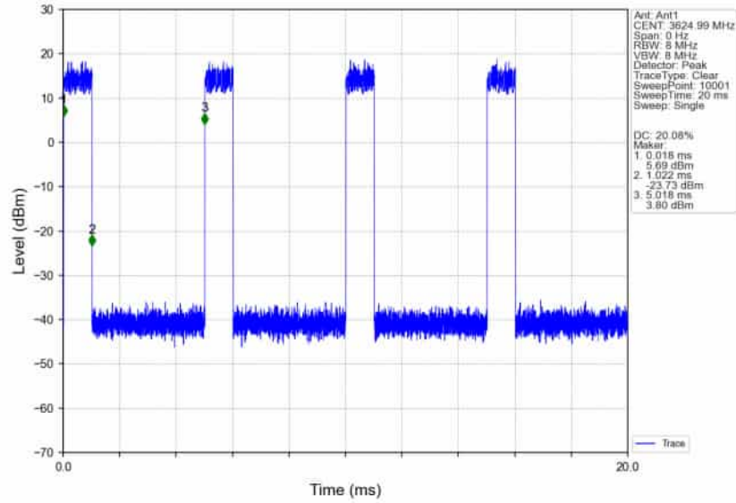
n78d_30kHz_SISO_NTNV_60MHz_DFT-s-OFDM_256_QAM_3624.99MHz_Inner_Full_Ant1
