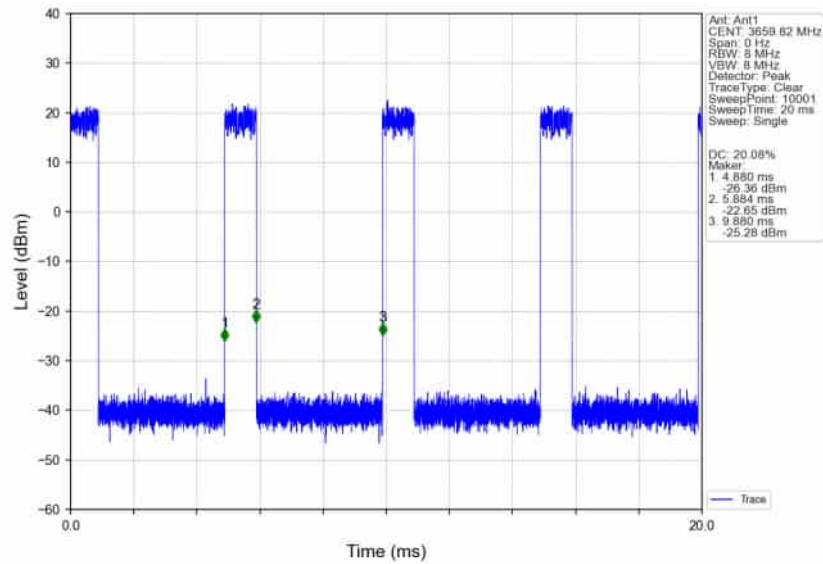
n78d_30kHz_SISO_NTNV_80MHz_DFT-s-OFDM_QPSK_3660MHz_Inner_Full_Ant1
