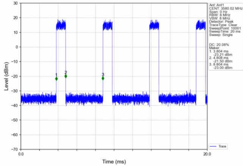
n78d_30kHz_SISO_NTNV_60MHz_DFT-s-OFDM_256_QAM_3580.02MHz_Inner_Full_Ant1
