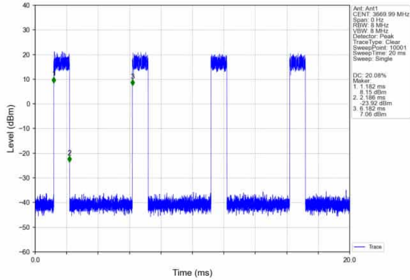
n78d_30kHz_SISO_NTNV_60MHz_DFT-s-OFDM_64_QAM_3669.99MHz_Inner_Full_Ant1
