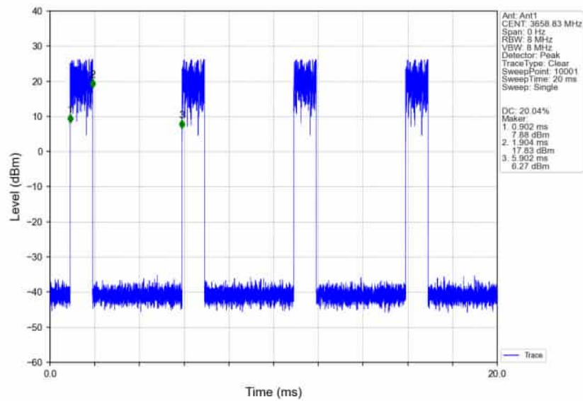
n78d_30kHz_SISO_NTNV_70MHz_CP-OFDM_64_QAM_3624.99MHz_Edge_1RB_Right_Ant1
