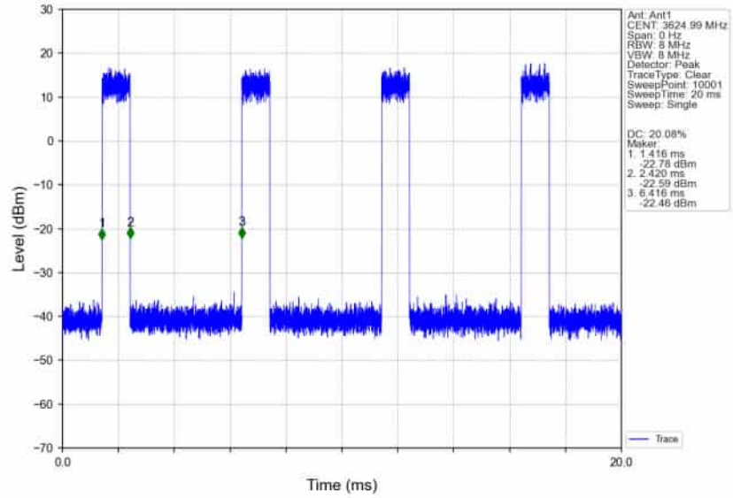
n78d_30kHz_SISO_NTNV_60MHz_CP-OFDM_256_QAM_3624.99MHz_Inner_Full_Ant1
