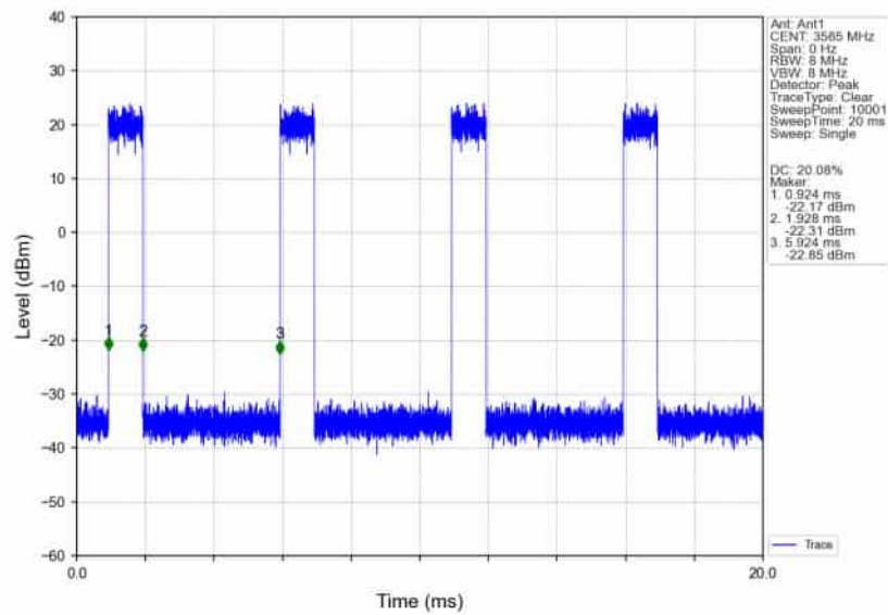
n78d_30kHz_SISO_NTNV_70MHz_CP-OFDM_16_QAM_3585MHz_Inner_Full_Ant1
