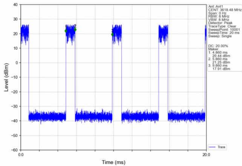
n78d_30kHz_SISO_NTNV_70MHz_DFT-s-OFDM_16_QAM_3585MHz_Inner_1RB_Right_Ant1
