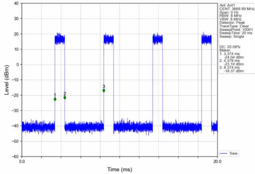
n78d_30kHz_SISO_NTNV_60MHz_CP-OFDM_QPSK_3669.99MHz_Inner_Full_Ant1
