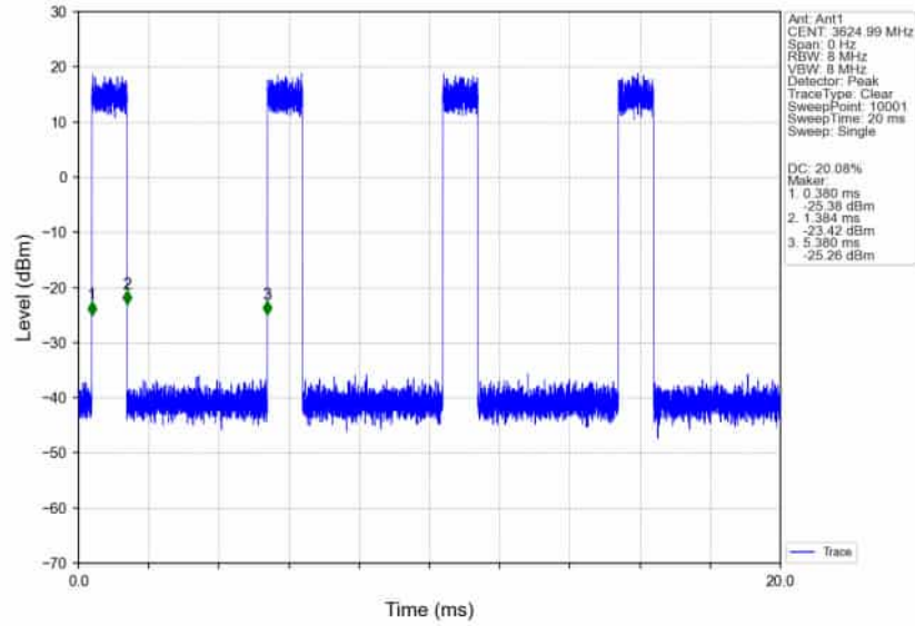
n78d_30kHz_SISO_NTNV_80MHz_CP-OFDM_QPSK_3624.99MHz_Inner_Full_Ant1
