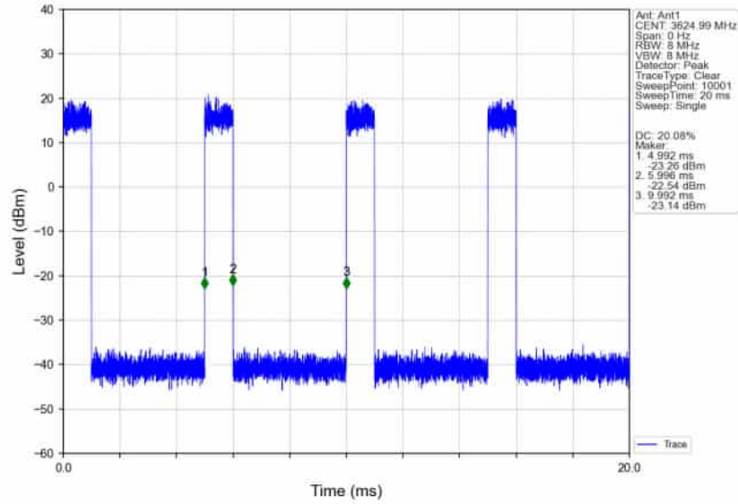
n78d_30kHz_SISO_NTNV_70MHz_CP-OFDM QPSK_3624.99MHz_Inner_Full_Ant1
