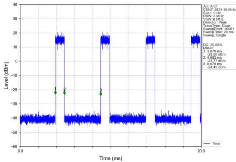
n78d_30kHz_SISO_NTNV_70MHz_CP-OFDM_256_QAM_3624.99MHz_Inner_Full_Ant1
