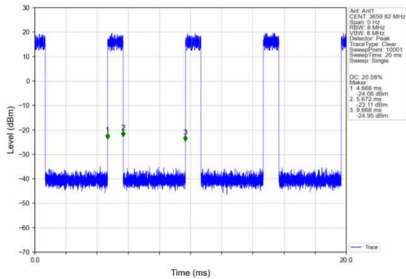
n78d_30kHz_SISO_NTNV_80MHz_DFT-s-OFDM_256_QAM_3660MHz_Inner_Full_Ant1
