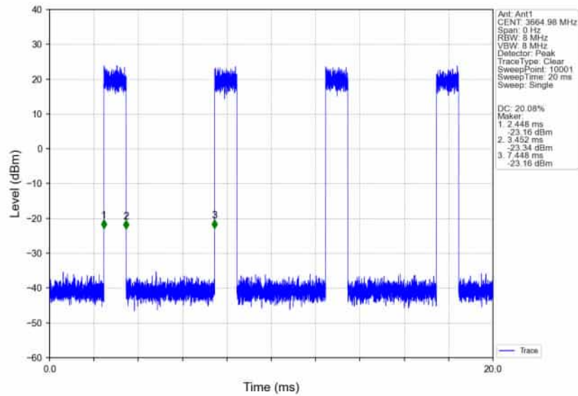
n78d_30kHz_SISO_NTNV_70MHz_CP-OFDM_QPSK_3664.98MHz_Inner_Full_Ant1
