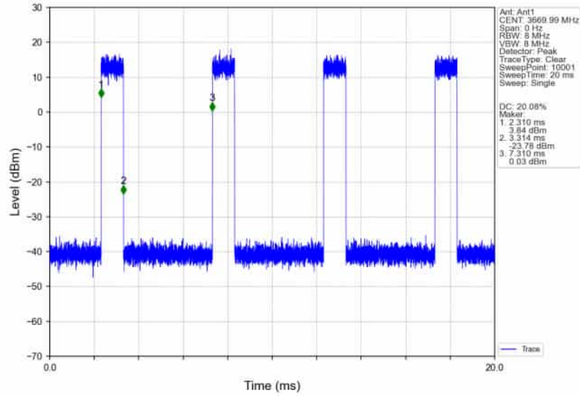
n78d_30kHz_SISO_NTNV_60MHz_CP-OFDM_256_QAM_3669.99MHz_Inner_Full_Ant1
