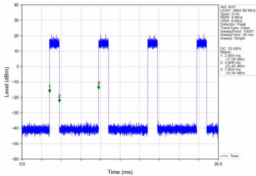
n78d_30kHz_SISO_NTNV_70MHz_CP-OFDM_256_QAM_3664.98MHz_Inner_Full_Ant1
