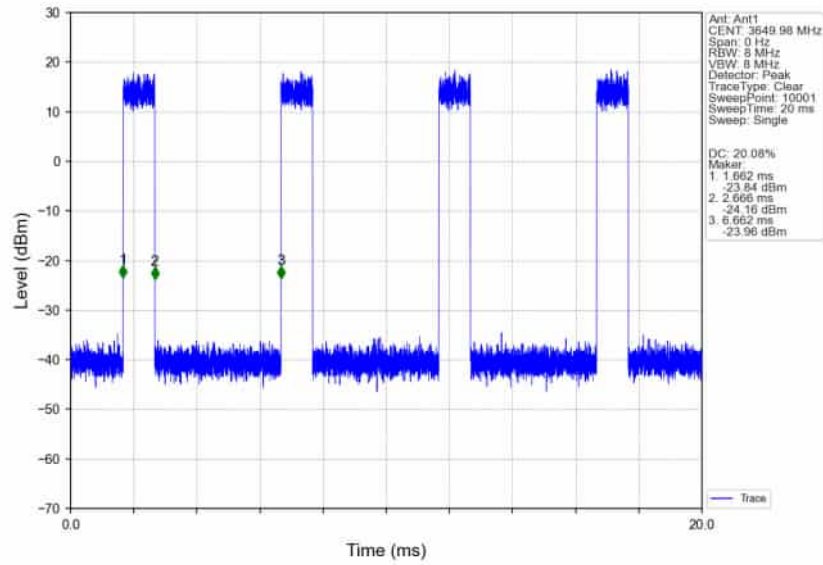
n78d_30kHz_SISO_NTNV_100MHz_CP-OFDM_QPSK_3649.98MHz_Inner_Full_Ant1
