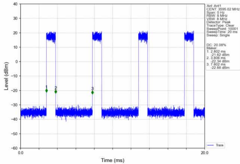
n78d_30kHz_SISO_NTNV_90MHz_CP-OFDM 64 QAM 3595.02MHz_Inner_Full_Ant1
