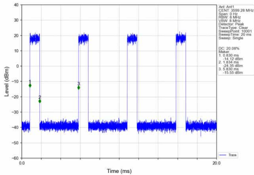
n78d_30kHz_SISO_NTNV_100MHz_DFT-s-OFDM_QPSK_3600MHz_Inner_Full_Ant1
