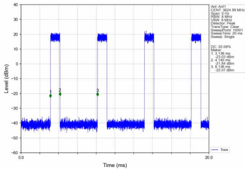
n78d_30kHz_SISO_NTNV_100MHz_CP-OFDM_16_QAM_3624.99MHz_Inner_Full_Ant1
