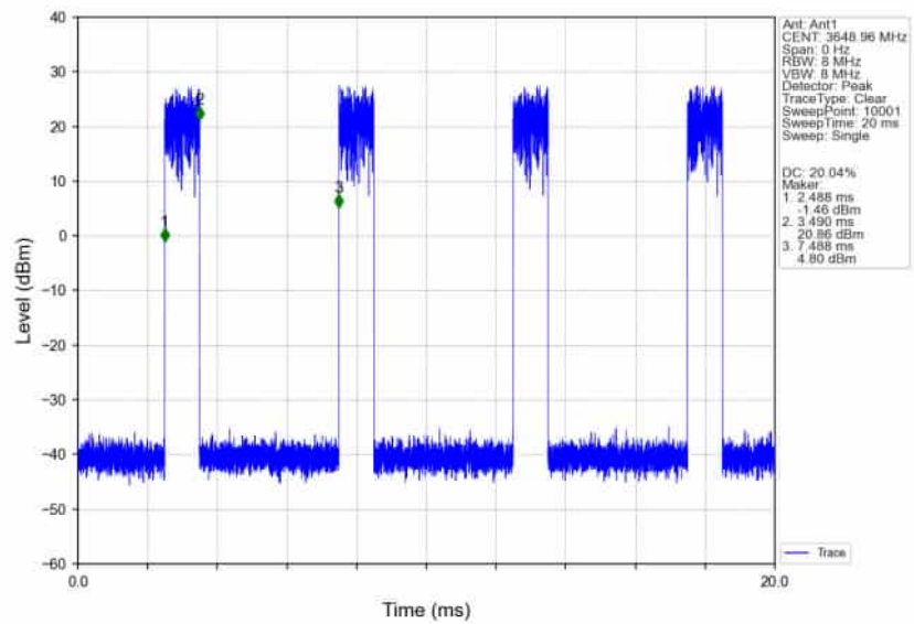
n78d_30kHz_SISO_NTNV_100MHz_CP-OFDM_16_QAM_3600MHz_Edge_1RB_Right_Ant1
