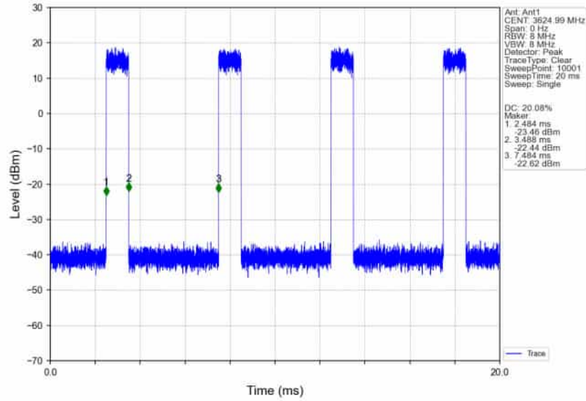
n78d_30kHz_SISO_NTNV_80MHz_CP-OFDM 16 QAM 3624.99MHz_Inner_Full_Ant1
