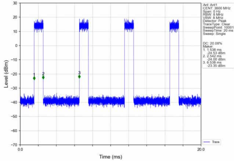
n78d_30kHz_SISO_NTNV_100MHz_CP-OFDM_16 QAM_3600MHz_Inner_Full_Ant1
