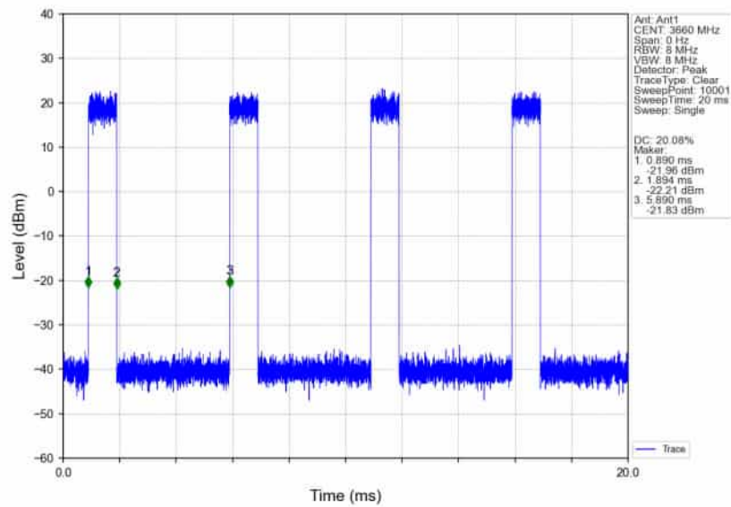
n78d_30kHz_SISO_NTNV_80MHz_CP-OFDM_16_QAM_3660MHz_Inner_Full_Ant1
