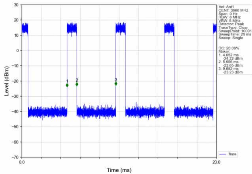
n78d_30kHz_SISO_NTNV_80MHz_CP-OFDM_256_QAM_3660MHz_Inner_Full_Ant1
