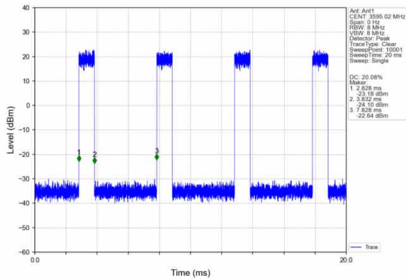
n78d_30kHz_SISO_NTNV_90MHz_CP-OFDM_QPSK_3595.02MHz_Inner_Full_Ant1
