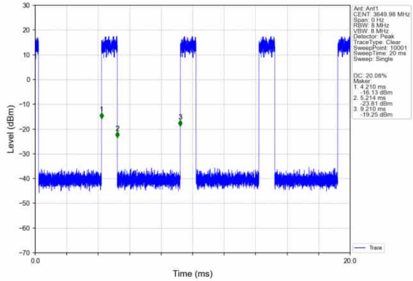
n78d_30kHz_SISO_NTNV_100MHz_CP-OFDM 64 QAM_3649.98MHz_Inner_Full_Ant1
