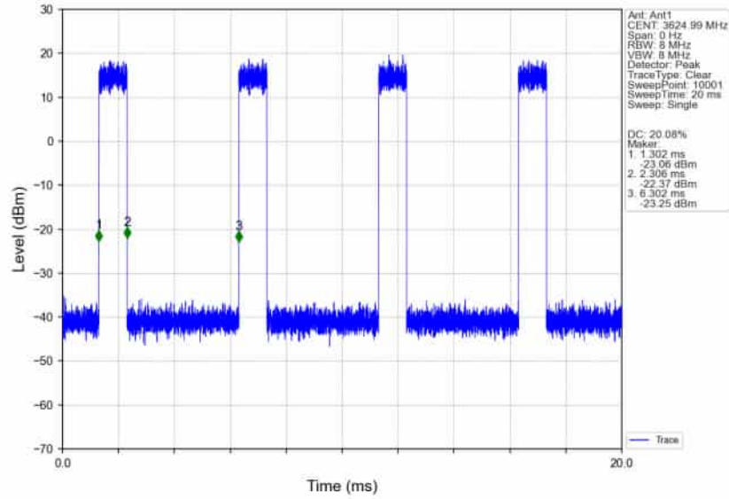
n78d_30kHz_SISO_NTNV_80MHz_CP-OFDM 64 QAM 3624.99MHz_Inner_Full_Ant1
