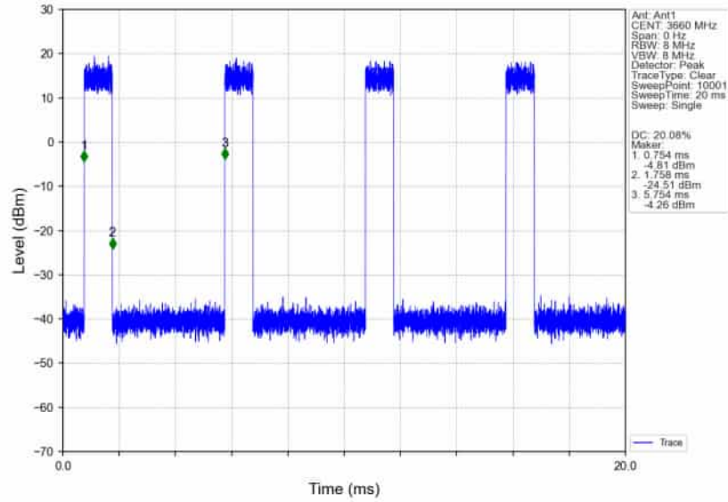
n78d_30kHz_SISO_NTNV_80MHz_CP-OFDM 64 QAM 3660MHz_Inner_Full_Ant1
