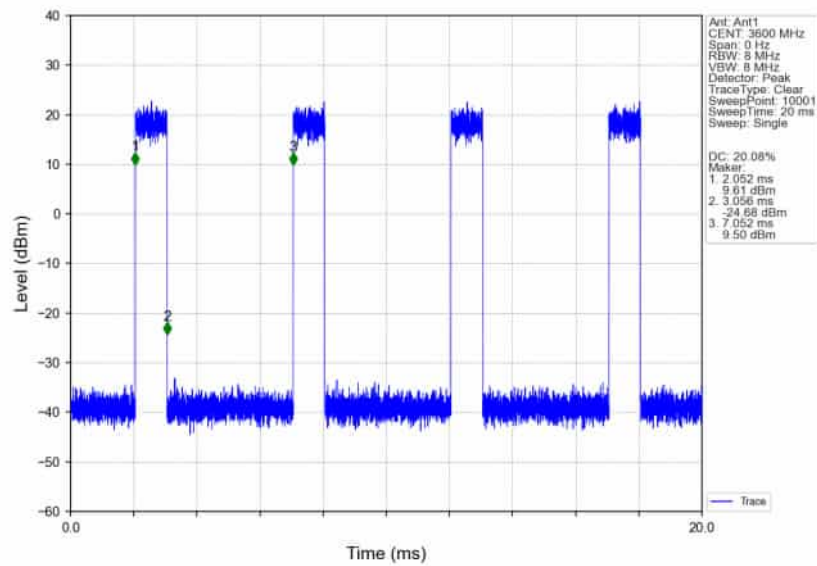
n78d_30kHz_SISO_NTNV_100MHz_CP-OFDM_QPSK_3600MHz_Inner_Full_Ant1
