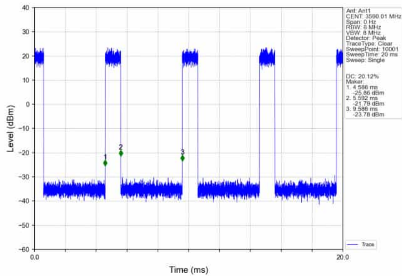
n78d_30kHz_SISO_NTNV_80MHz_CP-OFDM 16 QAM 3590.01MHz_Inner_Full_Ant1
