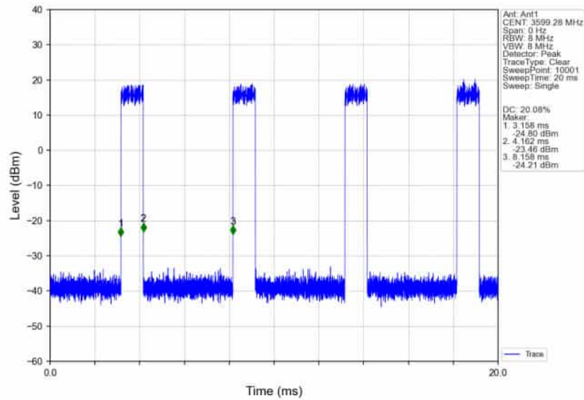
n78d_30kHz_SISO_NTNV_100MHz_DFT-s-OFDM_256_QAM_3600MHz_Inner_Full_Ant1
