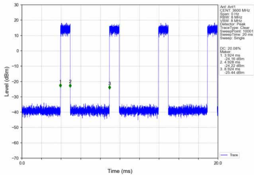
n78d_30kHz_SISO_NTNV_100MHz_CP-OFDM 256 QAM 3600MHz_Inner_Full_Ant1
