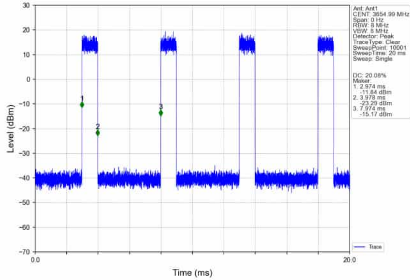
n78d_30kHz_SISO_NTNV_90MHz_CP-OFDM 64 QAM 3654.99MHz_Inner_Full_Ant1
