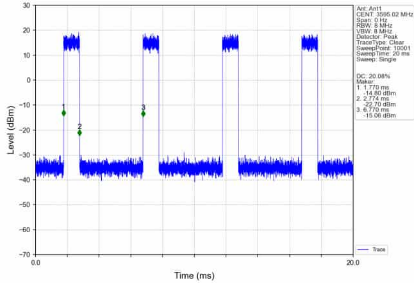
n78d_30kHz_SISO_NTNV_90MHz_CP-OFDM 16 QAM 3595.02MHz_Inner_Full_Ant1
