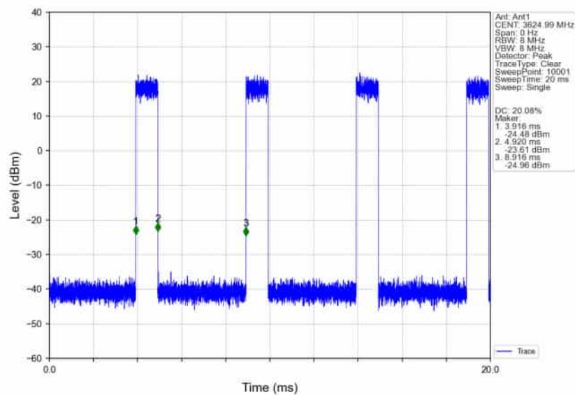
n78d_30kHz_SISO_NTNV_100MHz_CP-OFDM_QPSK_3624.99MHz_Inner_Full_Ant1
