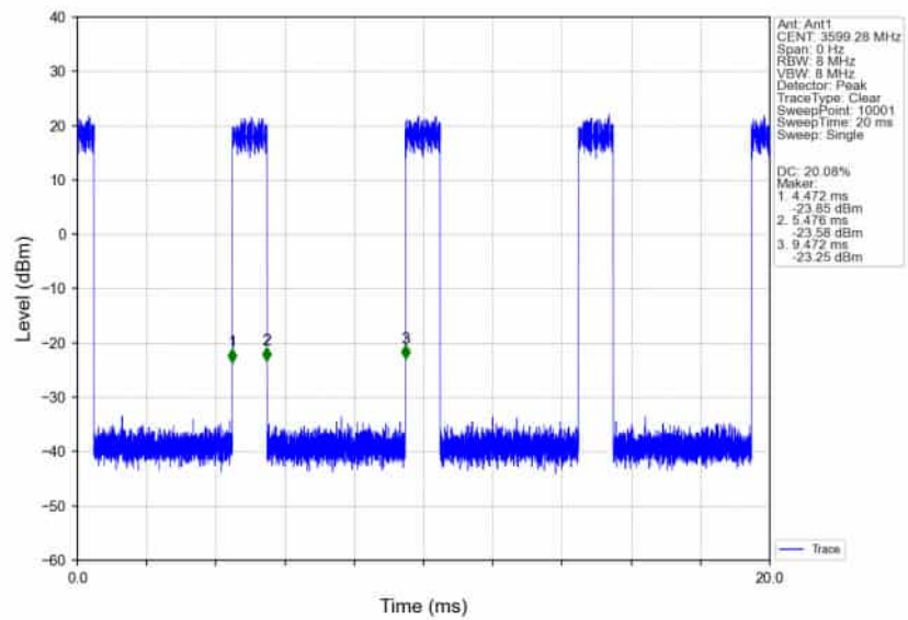
n78d_30kHz_SISO_NTNV_100MHz_DFT-s-OFDM_16_QAM_3600MHz_Inner_Full_Ant1
