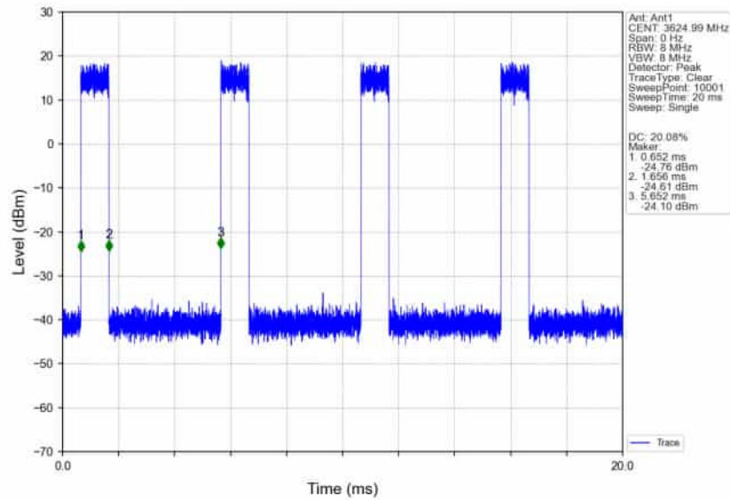
n78d_30kHz_SISO_NTNV_80MHz_CP-OFDM_256_QAM_3624.99MHz_Inner_Full_Ant1
