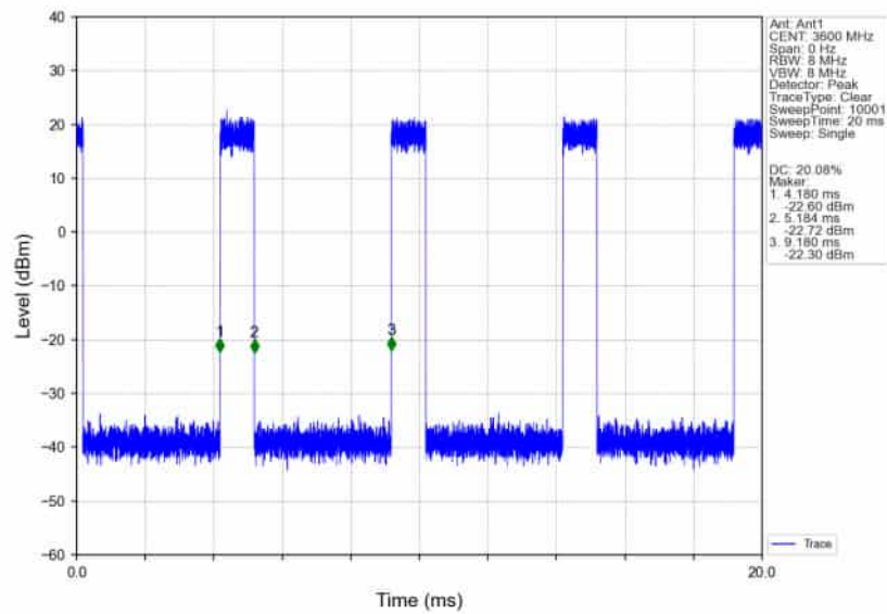
n78d_30kHz_SISO_NTNV_100MHz_CP-OFDM_16 QAM_3600MHz_Inner_Full_Ant1
