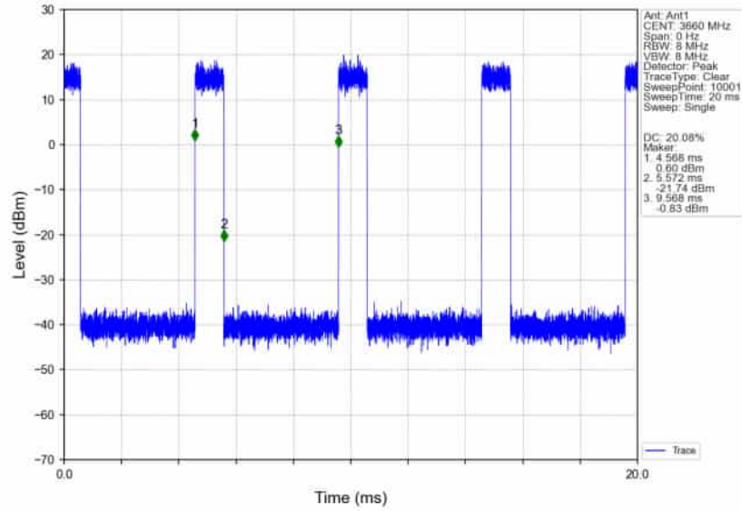
n78d_30kHz_SISO_NTNV_80MHz_CP-OFDM_16_QAM_3660MHz_Inner_Full_Ant1
