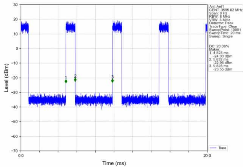
n78d_30kHz_SISO_NTNV_90MHz_CP-OFDM_256_QAM_3595.02MHz_Inner_Full_Ant1
