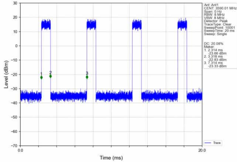
n78d_30kHz_SISO_NTNV_80MHz_CP-OFDM 64 QAM 3590.01MHz_Inner_Full_Ant1
