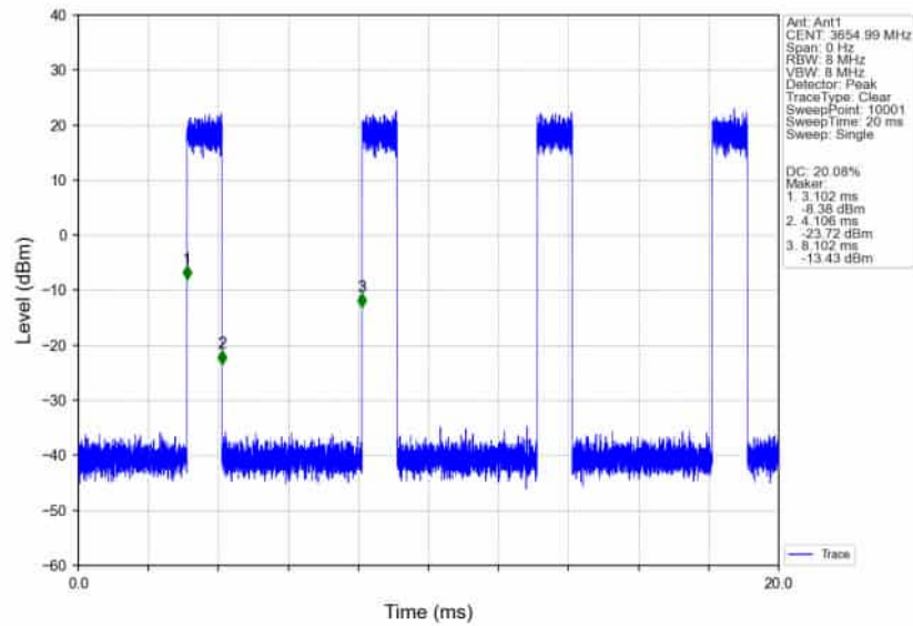
n78d_30kHz_SISO_NTNV_90MHz_CP-OFDM QPSK_3654.99MHz_Inner_Full_Ant1
