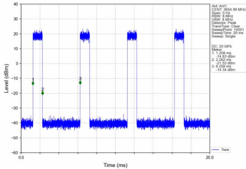
n78d_30kHz_SISO_NTNV_90MHz_CP-OFDM 16 QAM 3654.99MHz_Inner_Full_Ant1
