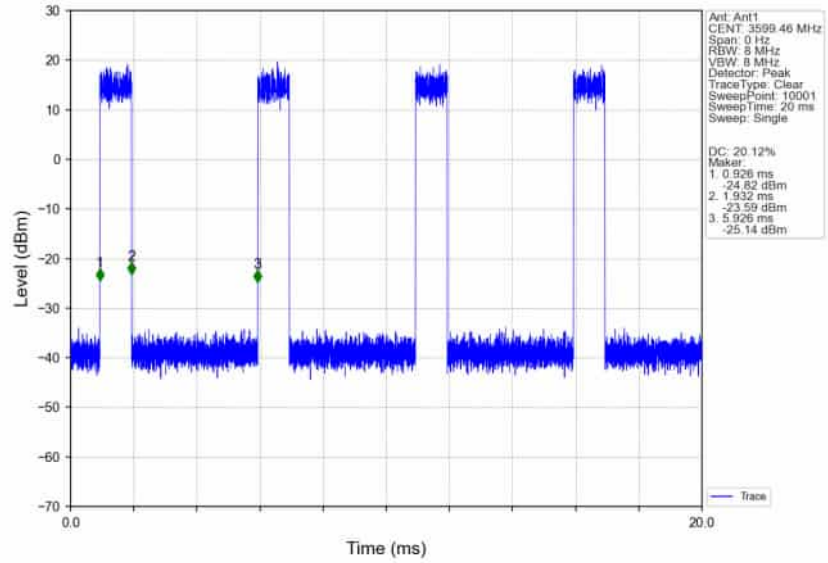
n78d_30kHz_SISO_NTNV_100MHz_DFT-s-OFDM_64_QAM_3600MHz_Inner_Full_Ant1
