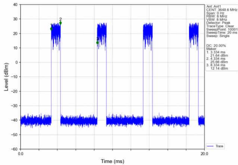
n78d_30kHz_SISO_NTNV_100MHz_CP-OFDM_16_QAM_3600MHz_Inner_1RB_Right_Ant1
