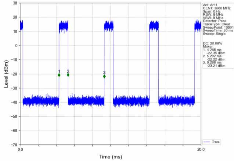
n78d_30kHz_SISO_NTNV_100MHz_CP-OFDM 64 QAM_3600MHz_Inner_Full_Ant1
