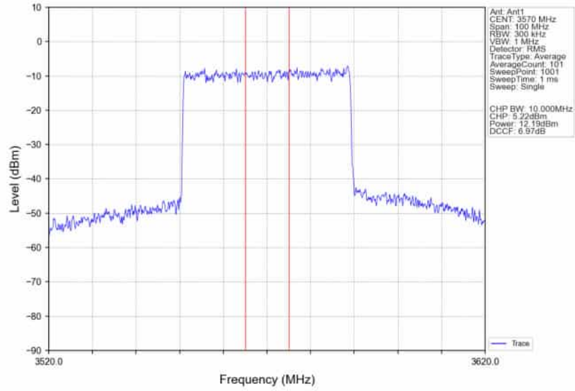
n78d_30kHz_SISO_NTNV_40MHz_CP-OFDM 16 QAM 3570MHz_Inner_Full_Ant1
