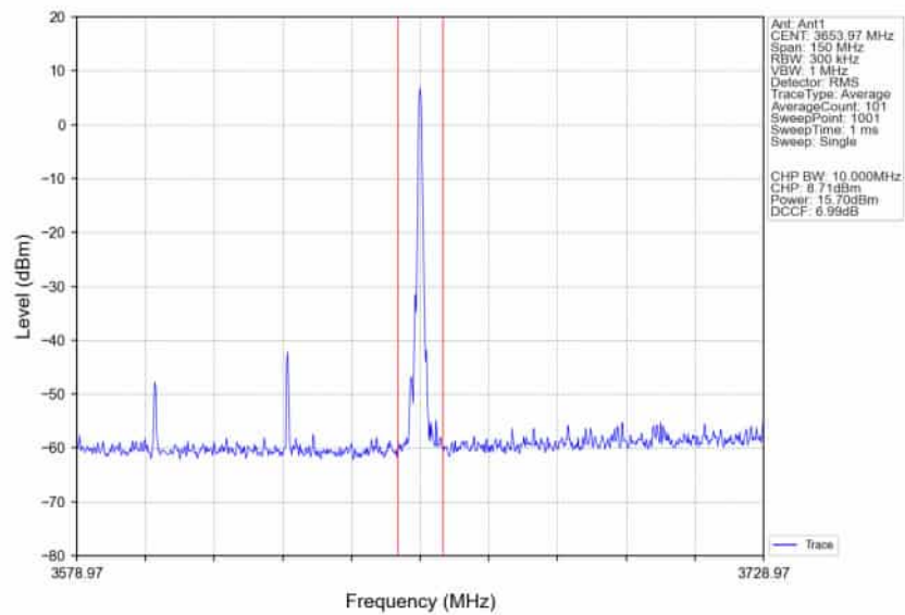
n78d_30kHz_SISO_NTNV_60MHz_DFT-s-OFDM_256_QAM_3624.99MHz_Edge_1RB_Right_Ant1
