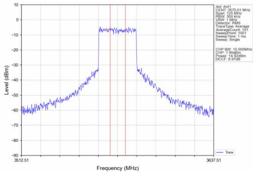
n78d_30kHz_SISO_NTNV_50MHz_CP-OFDM_QPSK_3575.01MHz_Inner_Full_Ant1
