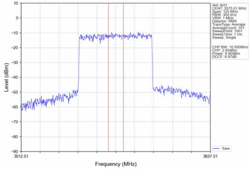
n78d_30kHz_SISO_NTNV_50MHz_CP-OFDM_QPSK_3575.01MHz_Inner_Full_Ant1
