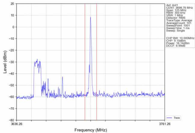
n78d_30kHz_SISO_NTNV_50MHz_CP-OFDM_16_QAM_3675MHz_Edge_1RB_Right_Ant1
