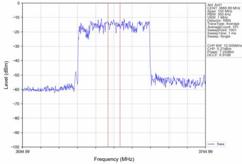
n78d_30kHz_SISO_NTNV_60MHz_DFT-s-OFDM_QPSK_3669.99MHz_Inner_Full_Ant1
