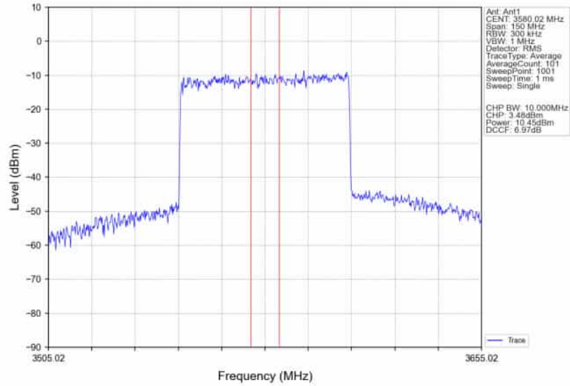
n78d_30kHz_SISO_NTNV_60MHz_CP-OFDM_QPSK_3580.02MHz_Inner_Full_Ant1
