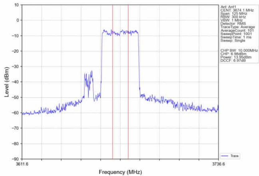
n78d_30kHz_SISO_NTNV_50MHz_DFT-s-OFDM_256_QAM_3675MHz_Inner_Full_Ant1
