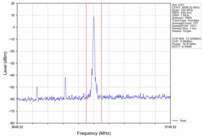
n78d_30kHz_SISO_NTNV_40MHz_DFT-s-OFDM_256_QAM_3679.98MHz_Inner_1RB_Right_Ant1
