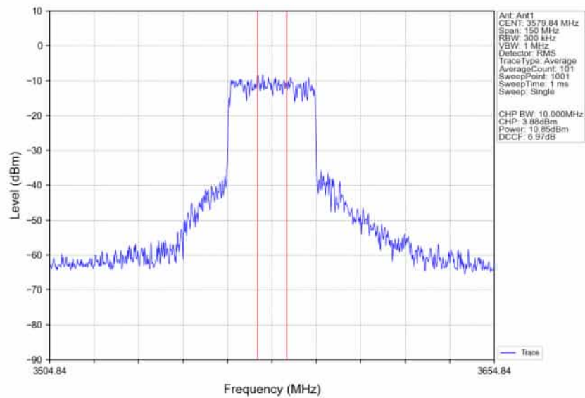
n78d_30kHz_SISO_NTNV_60MHz_CP-OFDM_QPSK_3580.02MHz_Inner_Full_Ant1
