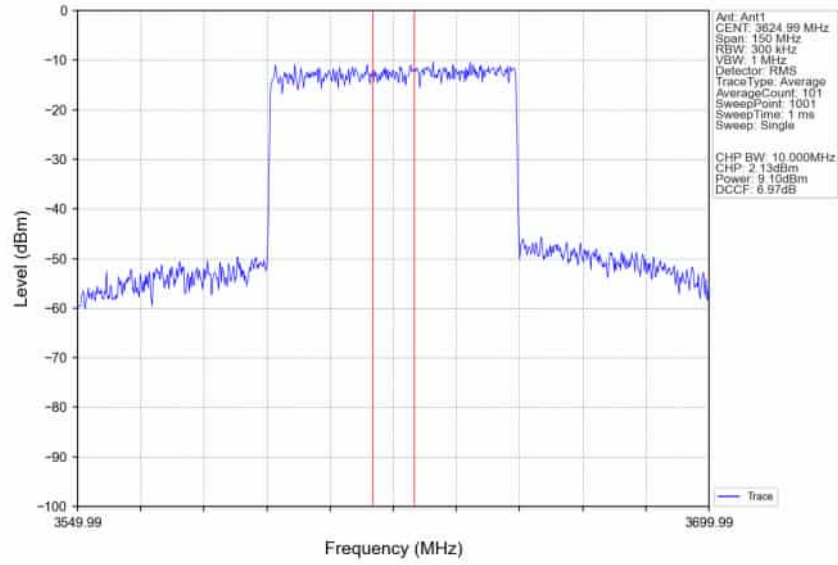
n78d_30kHz_SISO_NTNV_60MHz_CP-OFDM_QPSK_3624.99MHz_Inner_Full_Ant1
