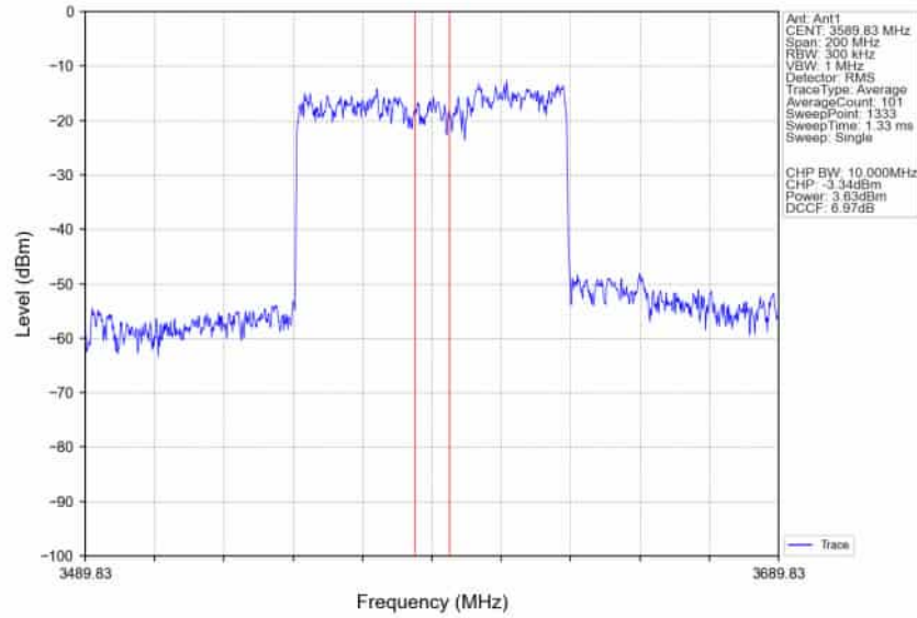
n78d_30kHz_SISO_NTNV_80MHz_DFT-s-OFDM_256_QAM_3590.01MHz_Inner_Full_Ant1
