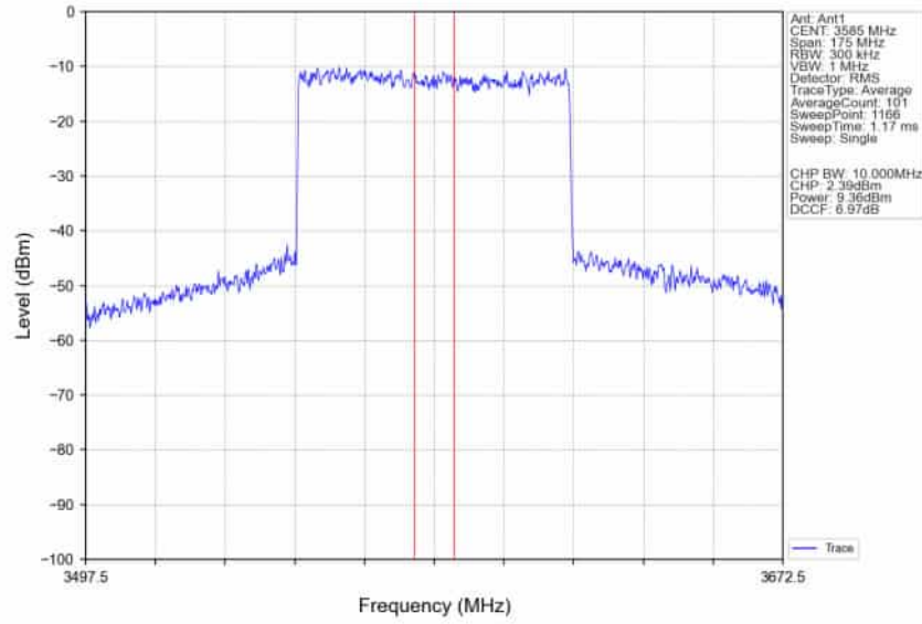
n78d_30kHz_SISO_NTNV_70MHz_CP-OFDM 64 QAM_3585MHz_Inner_Full_Ant1
