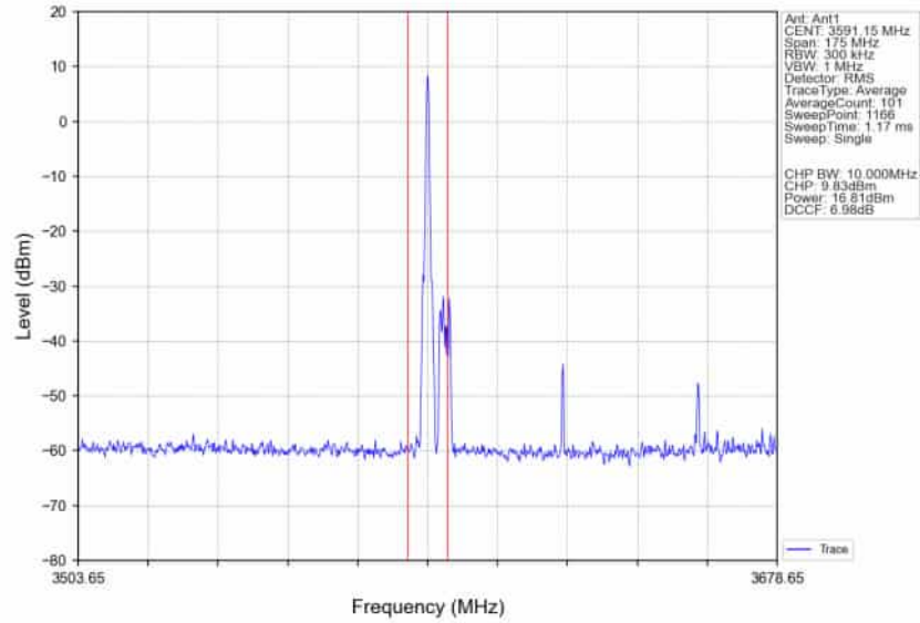
n78d_30kHz_SISO_NTNV_70MHz_CP-OFDM_16_QAM_3624.99MHz_Edge_1RB_Right_Ant1
