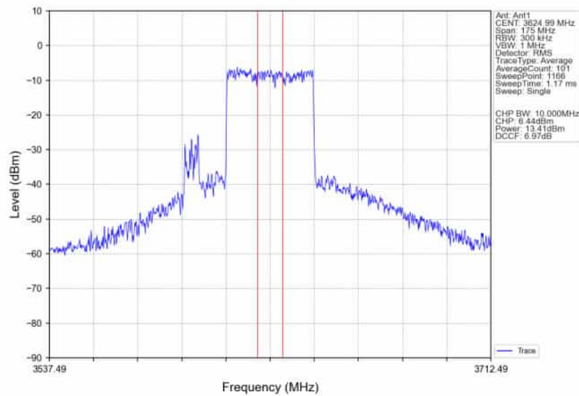
n78d_30kHz_SISO_NTNV_70MHz_CP-OFDM_QPSK_3624.99MHz_Inner_Full_Ant1
