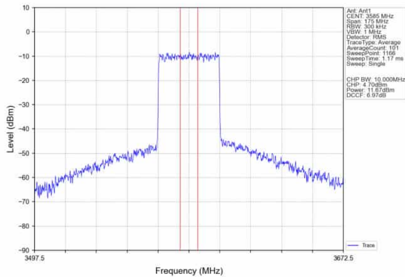
n78d_30kHz_SISO_NTNV_70MHz_CP-OFDM 64 QAM_3585MHz_Inner_Full_Ant1
