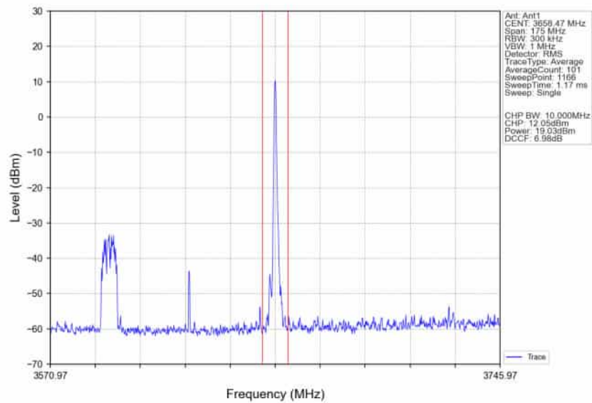
n78d_30kHz_SISO_NTNV_70MHz_CP-OFDM 16 QAM 3624.99MHz_Inner_1RB_Right_Ant1
