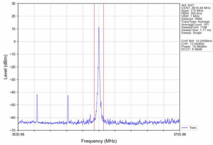
n78d_30kHz_SISO_NTNV_70MHz_DFT-s-OFDM_QPSK_3585MHz_Inner_1RB_Right_Ant1
