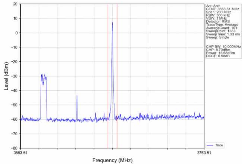
n78d_30kHz_SISO_NTNV_80MHz_DFT-s-OFDM_256_QAM_3624.99MHz_Inner_1RB_Right_Ant1
