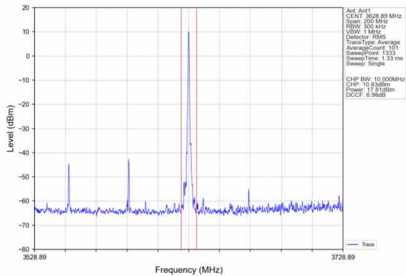
n78d_30kHz_SISO_NTNV_80MHz_CP-OFDM 64 QAM_3590.01MHz_Edge_1RB_Right_Ant1
