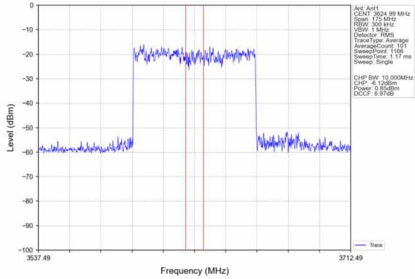
n78d_30kHz_SISO_NTNV_70MHz_CP-OFDM_256_QAM_3624.99MHz_Inner_Full_Ant1
