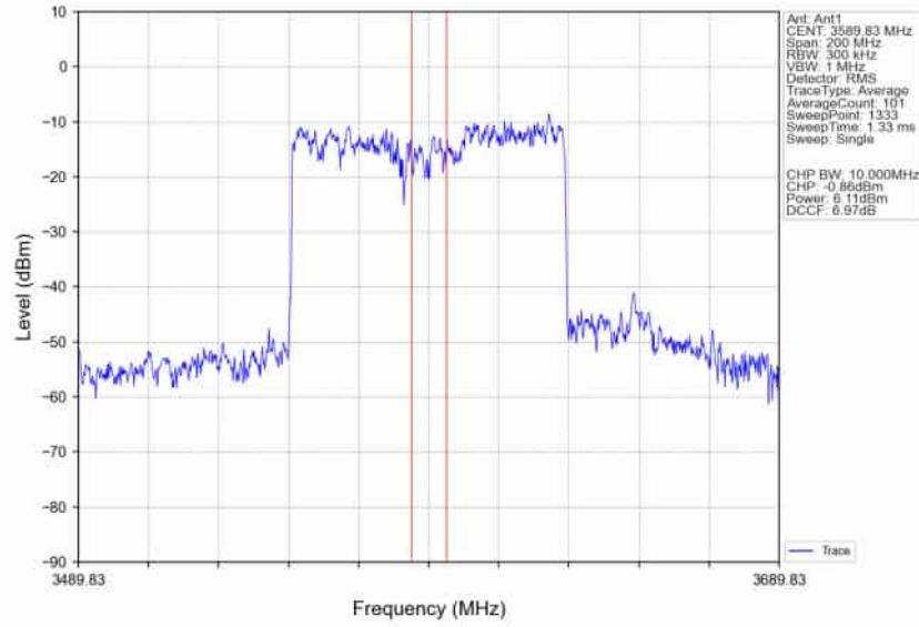
n78d_30kHz_SISO_NTNV_80MHz_DFT-s-OFDM_QPSK_3590.01MHz_Inner_Full_Ant1
