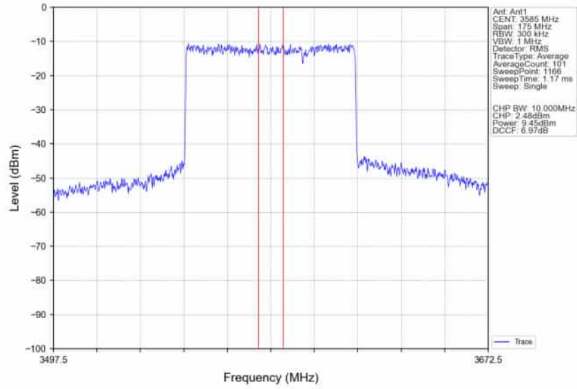
n78d_30kHz_SISO_NTNV_70MHz_CP-OFDM_QPSK_3585MHz_Inner_Full_Ant1
