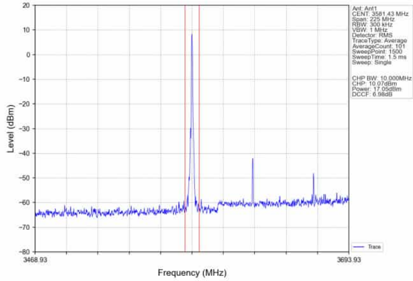
n78d_30kHz_SISO_NTNV_90MHz_DFT-s-OFDM_256_QAM_3624.99MHz_Inner_1RB_Right_Ant1
