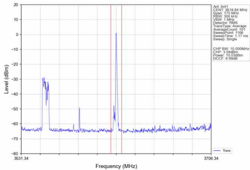
n78d_30kHz_SISO_NTNV_70MHz_CP-OFDM_64_QAM_3585MHz_Edge_1RB_Right_Ant1
