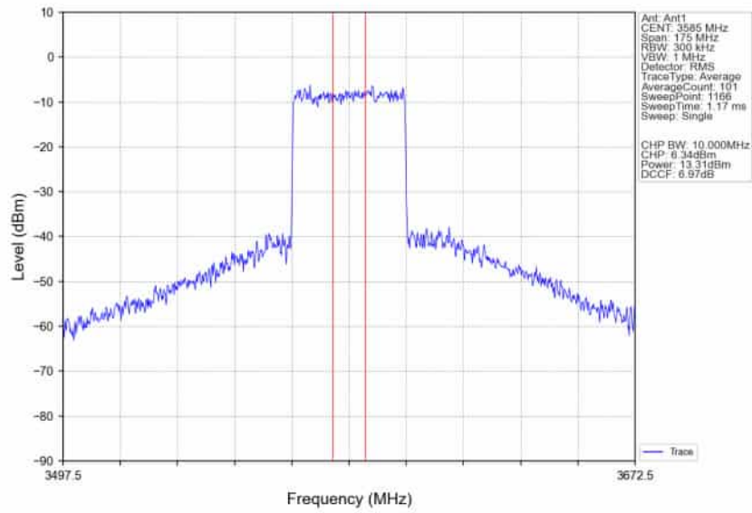
n78d_30kHz_SISO_NTNV_70MHz_CP-OFDM_QPSK_3585MHz_Inner_Full_Ant1
