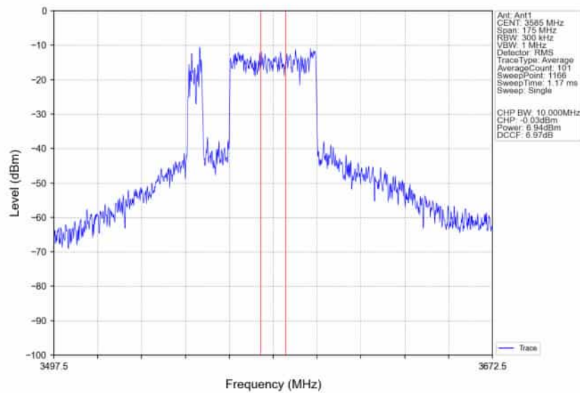
n78d_30kHz_SISO_NTNV_70MHz_CP-OFDM 16 QAM 3585MHz_Inner_Full_Ant1
