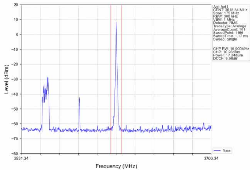
n78d_30kHz_SISO_NTNV_70MHz_DFT-s-OFDM_256_QAM_3585MHz_Edge_1RB_Right_Ant1
