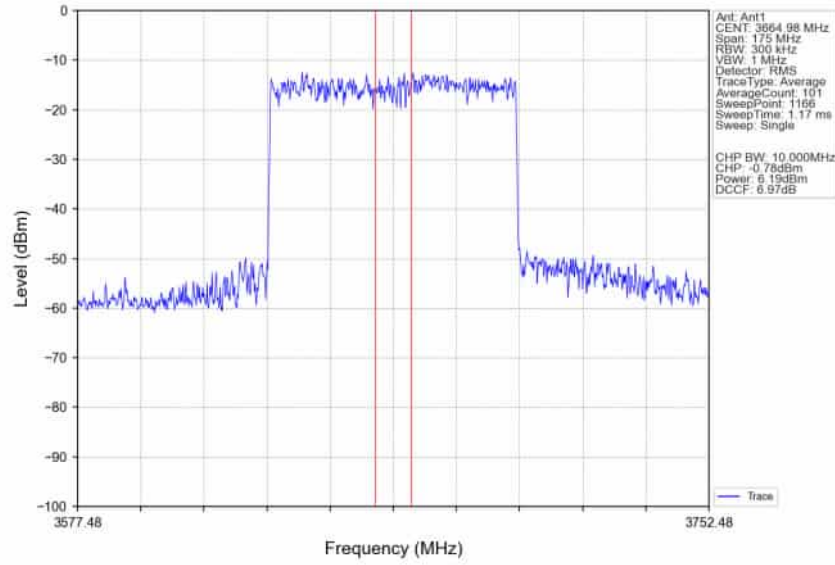
n78d_30kHz_SISO_NTNV_70MHz_CP-OFDM 16 QAM 3664.98MHz_Inner_Full_Ant1
