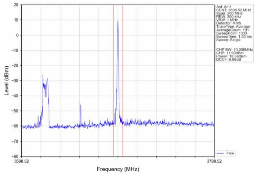
n78d_30kHz_SISO_NTNV_80MHz_DFT-s-OFDM_QPSK_3660MHz_Inner_1RB_Right_Ant1
