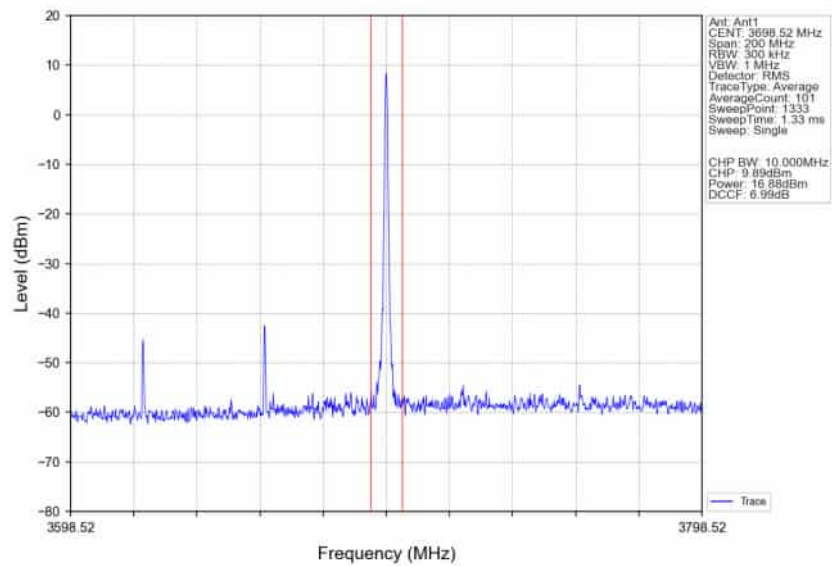
n78d_30kHz_SISO_NTNV_80MHz_DFT-s-OFDM 256 QAM_3660MHz_Inner_1RB_Right_Ant1
