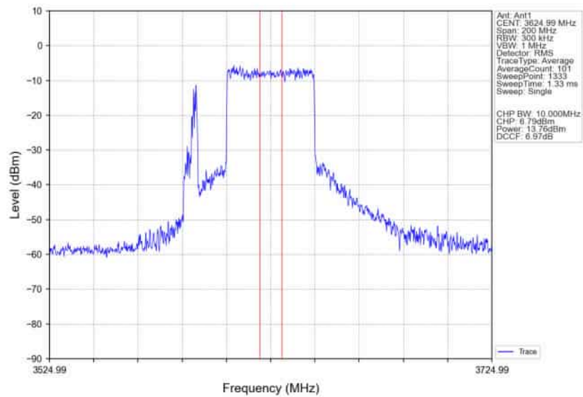
n78d_30kHz_SISO_NTNV_80MHz_CP-OFDM_QPSK_3624.99MHz_Inner_Full_Ant1
