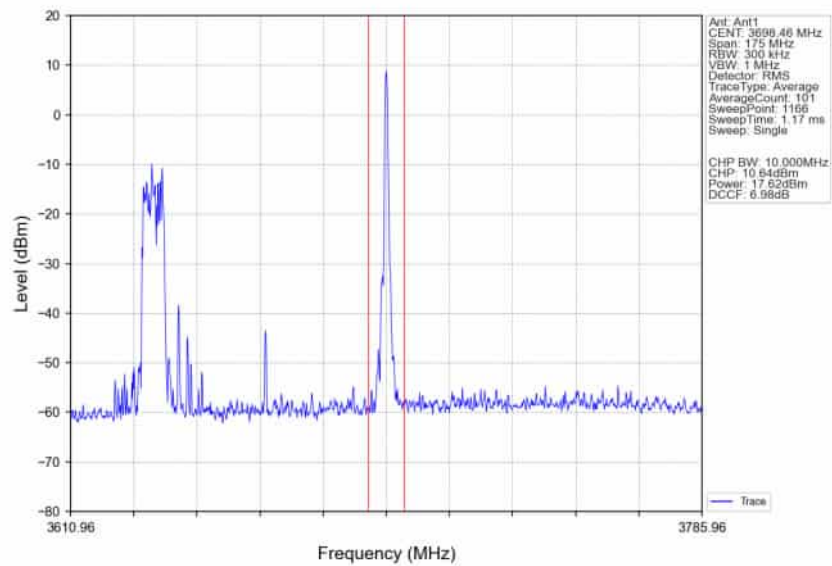
n78d_30kHz_SISO_NTNV_70MHz_CP-OFDM 64 QAM_3664.98MHz_Inner_1RB_Right_Ant1
