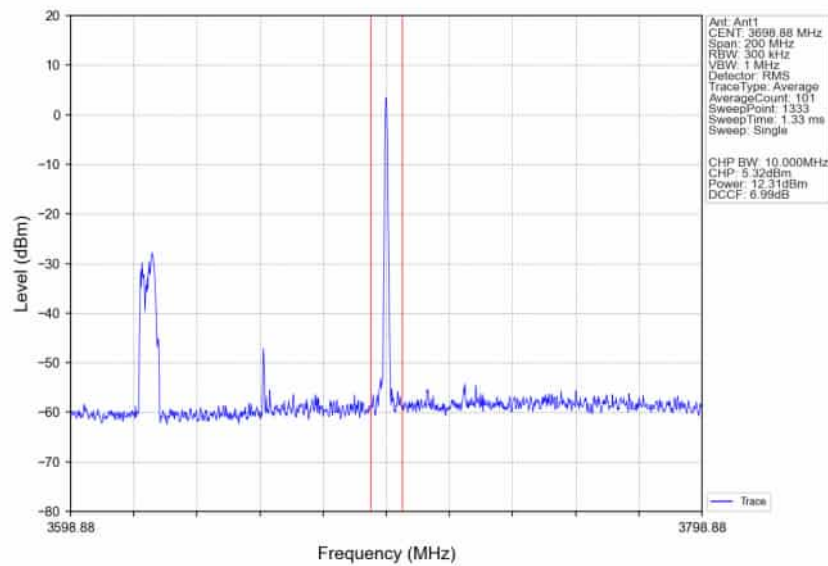
n78d_30kHz_SISO_NTNV_80MHz_DFT-s-OFDM_256_QAM_3660MHz_Edge_1RB_Right_Ant1
