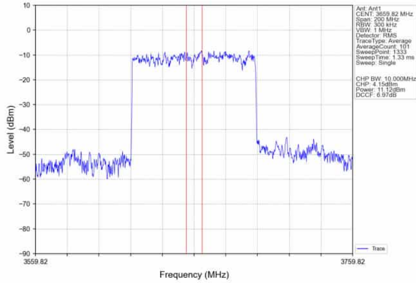
n78d_30kHz_SISO_NTNV_80MHz_DFT-s-OFDM PI/2 BPSK_3660MHz_Inner_Full_Ant1
