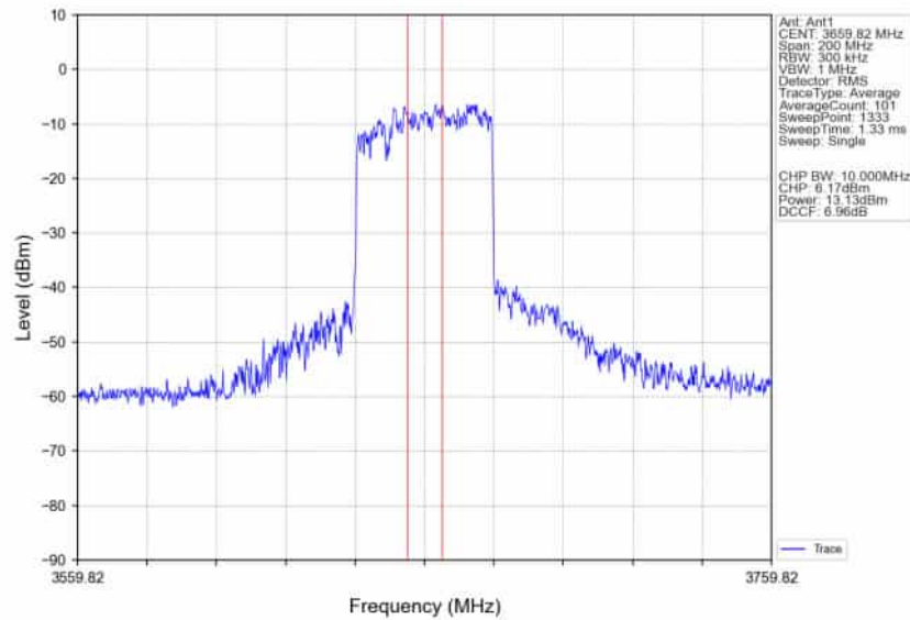
n78d_30kHz_SISO_NTNV_80MHz_DFT-s-OFDM 16 QAM 3660MHz_Inner_Full_Ant1
