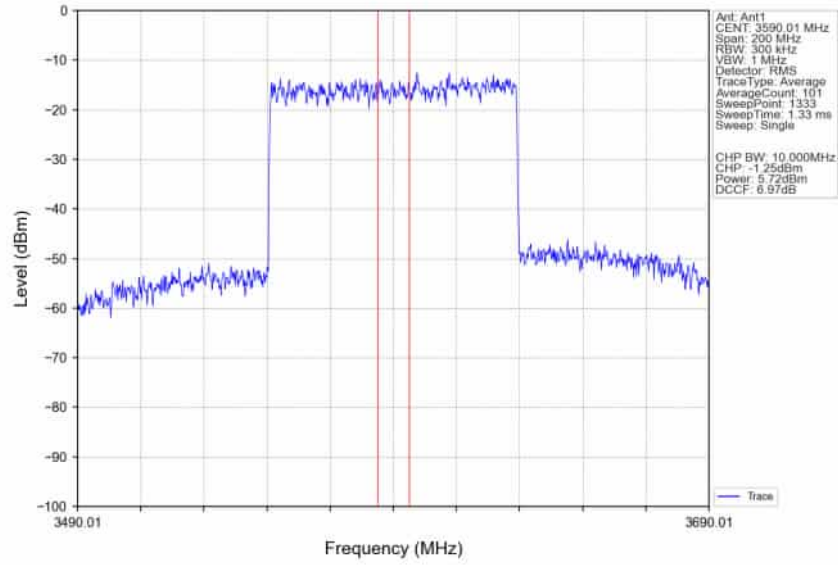
n78d_30kHz_SISO_NTNV_80MHz_CP-OFDM_QPSK_3590.01MHz_Inner_Full_Ant1
