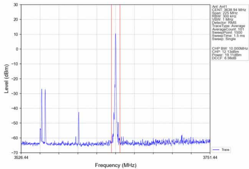
n78d_30kHz_SISO_NTNV_90MHz_DFT-s-OFDM_QPSK_3595.02MHz_Edge_1RB_Right_Ant1
