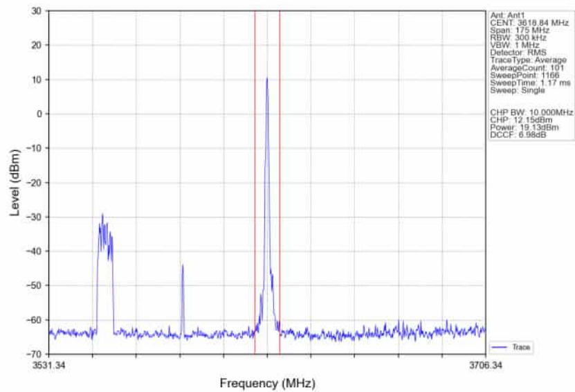
n78d_30kHz_SISO_NTNV_70MHz_DFT-s-OFDM_16_QAM_3585MHz_Edge_1RB_Right_Ant1
