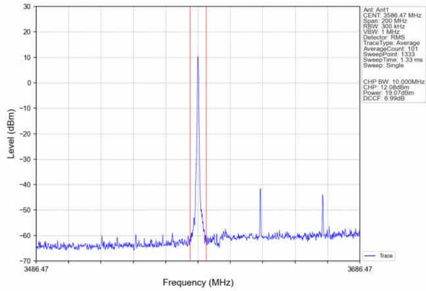
n78d_30kHz_SISO_NTNV_80MHz_DFT-s-OFDM_64_QAM_3624.99MHz_Inner_1RB_Right_Ant1
