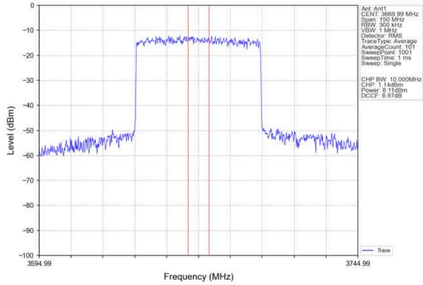
n78d_30kHz_SISO_NTNV_60MHz_CP-OFDM_256_QAM_3669.99MHz_Inner_Full_Ant1
