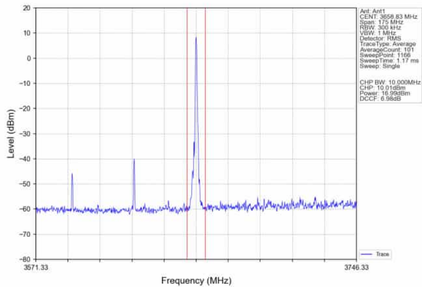
n78d_30kHz_SISO_NTNV_70MHz_CP-OFDM_256_QAM_3624.99MHz_Edge_1RB_Right_Ant1
