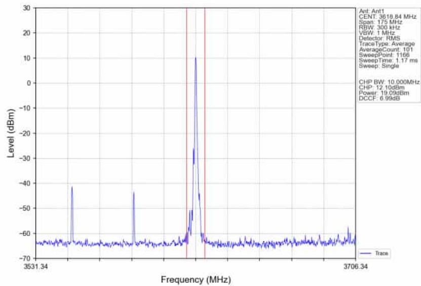
n78d_30kHz_SISO_NTNV_70MHz_DFT-s-OFDM_QPSK_3585MHz_Edge_1RB_Right_Ant1
