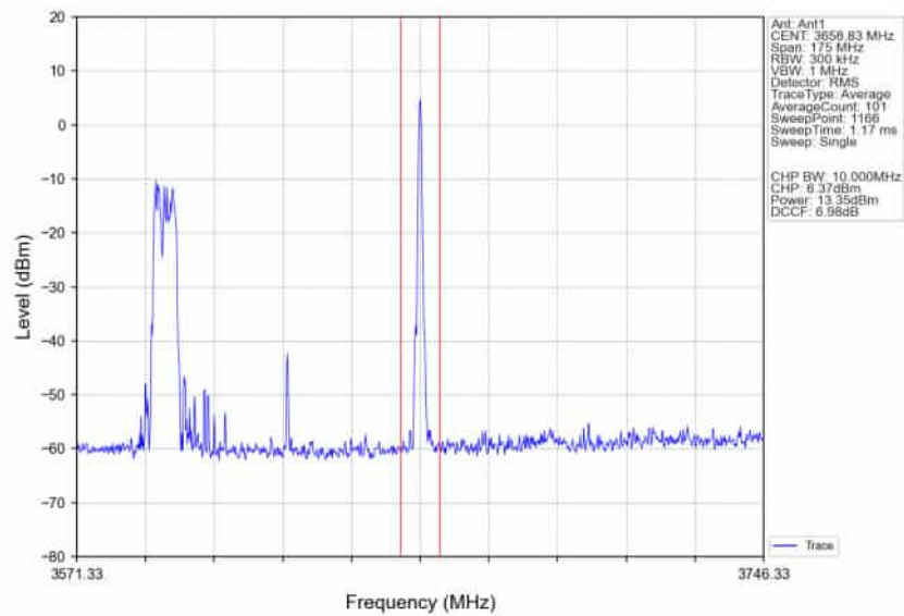
n78d_30kHz_SISO_NTNV_70MHz_CP-OFDM 64 QAM_3624.99MHz_Edge_1RB_Right_Ant1
