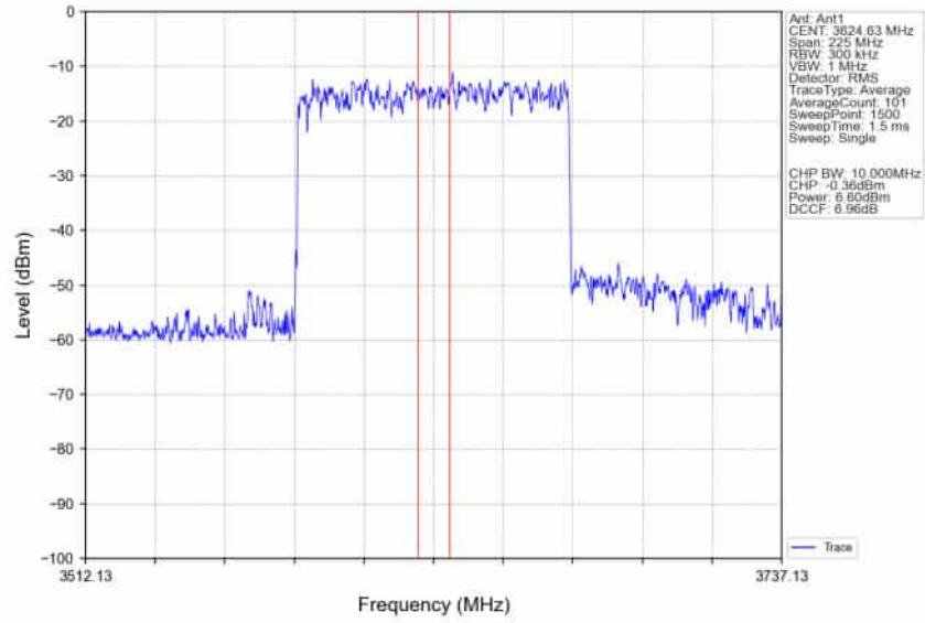
n78d_30kHz_SISO_NTNV_90MHz_DFT-s-OFDM_64_QAM_3624.99MHz_Inner_Full_Ant1
