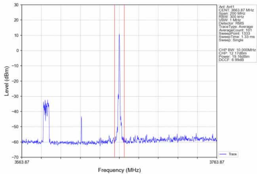
n78d_30kHz_SISO_NTNV_80MHz_CP-OFDM_16_QAM_3624.99MHz_Edge_1RB_Right_Ant1
