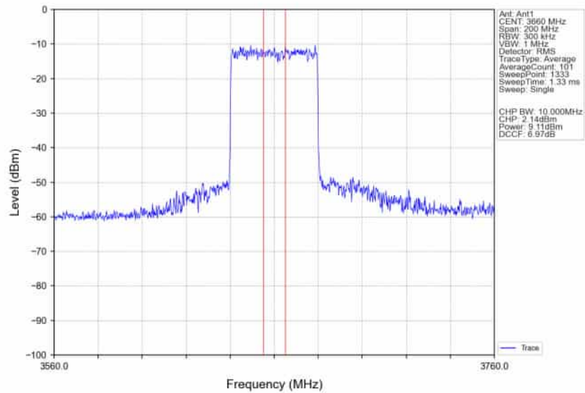
n78d_30kHz_SISO_NTNV_80MHz_CP-OFDM_256_QAM_3660MHz_Inner_Full_Ant1
