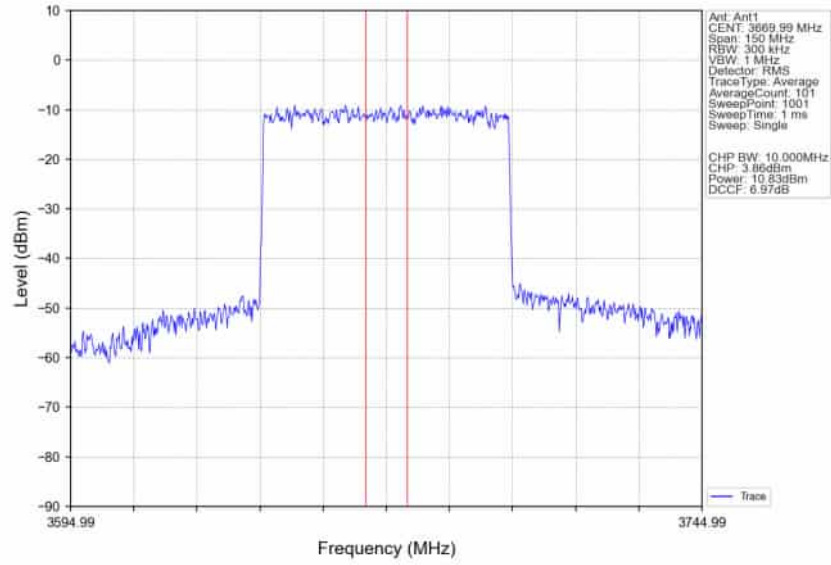
n78d_30kHz_SISO_NTNV_60MHz_CP-OFDM 64 QAM 3669.99MHz_Inner_Full_Ant1
