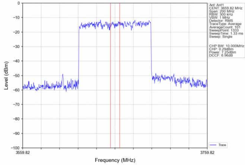
n78d_30kHz_SISO_NTNV_80MHz_DFT-s-OFDM_256_QAM_3660MHz_Inner_Full_Ant1
