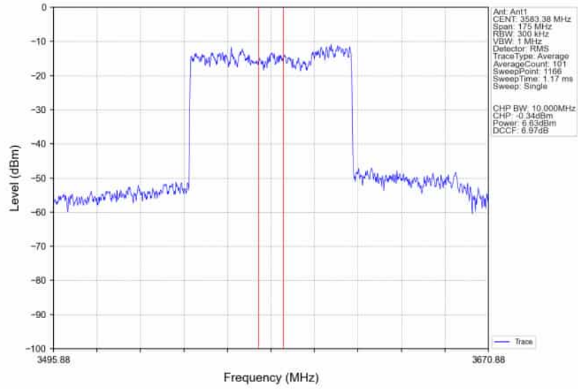
n78d_30kHz_SISO_NTNV_70MHz_DFT-s-OFDM_256_QAM_3585MHz_Inner_Full_Ant1
