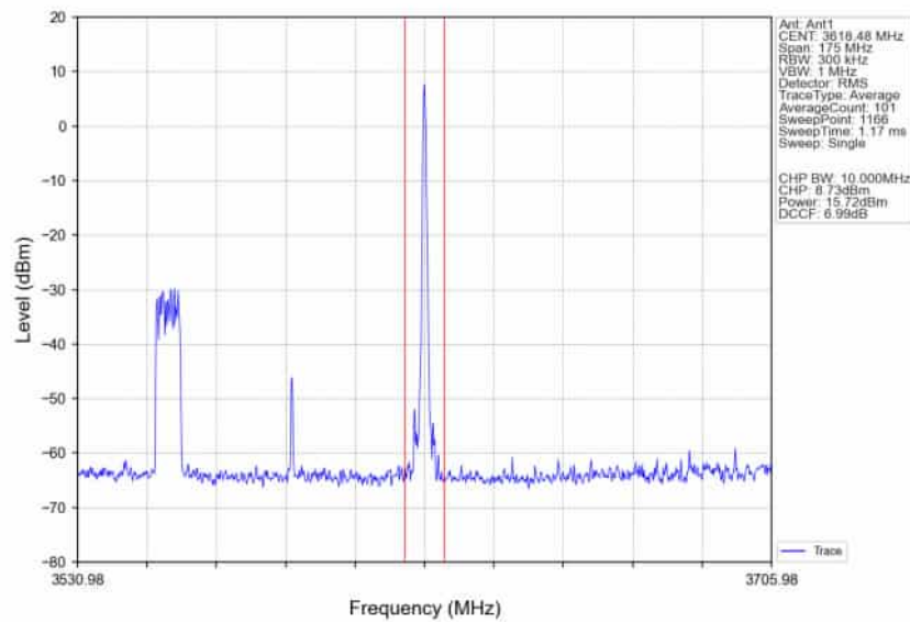
n78d_30kHz_SISO_NTNV_70MHz_DFT-s-OFDM_16_QAM_3585MHz_Inner_1RB_Right_Ant1
