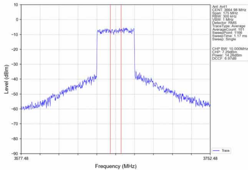
n78d_30kHz_SISO_NTNV_70MHz_CP-OFDM_QPSK_3664.98MHz_Inner_Full_Ant1
