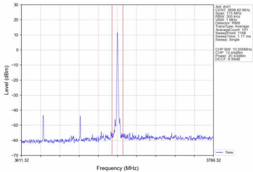
n78d_30kHz_SISO_NTNV_70MHz_DFT-s-OFDM_QPSK_3664.98MHz_Edge_1RB_Right_Ant1
