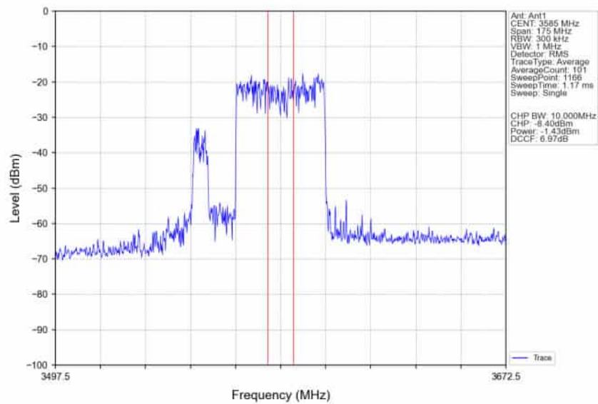
n78d_30kHz_SISO_NTNV_70MHz_CP-OFDM_256_QAM_3585MHz_Inner_Full_Ant1
