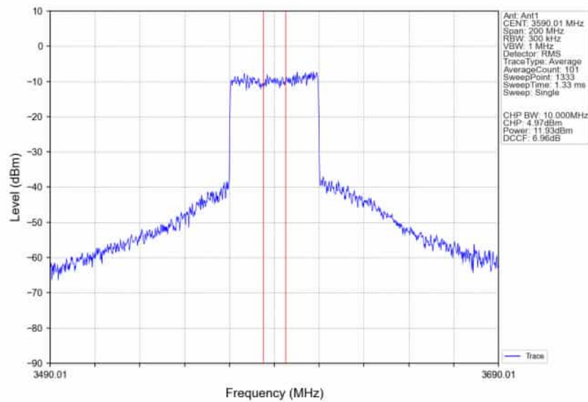
n78d_30kHz_SISO_NTNV_80MHz_CP-OFDM 16 QAM 3590.01MHz_Inner_Full_Ant1
