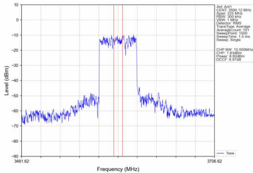
n78d_30kHz_SISO_NTNV_90MHz_DFT-s-OFDM_QPSK_3595.02MHz_Inner_Full_Ant1
