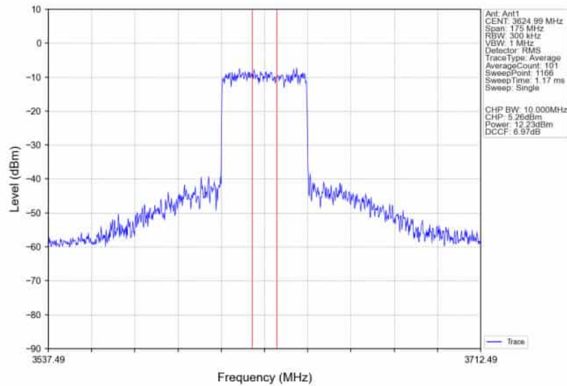
n78d_30kHz_SISO_NTNV_70MHz_CP-OFDM 16 QAM 3624.99MHz_Inner_Full_Ant1
