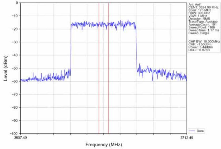
n78d_30kHz_SISO_NTNV_70MHz_CP-OFDM 64 QAM 3624.99MHz_Inner_Full_Ant1
