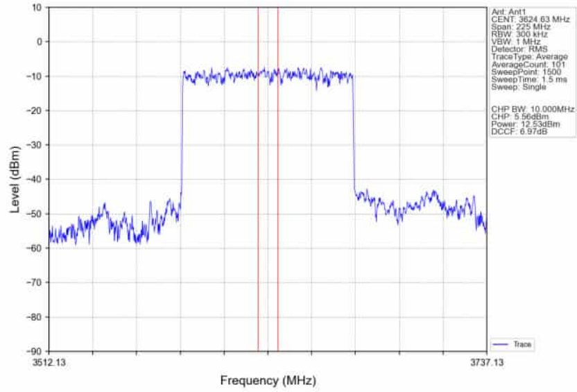
n78d_30kHz_SISO_NTNV_90MHz_DFT-s-OFDM PI/2 BPSK_3624.99MHz_Inner_Full_Ant1
