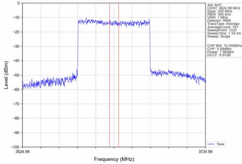
n78d_30kHz_SISO_NTNV_80MHz_CP-OFDM 64 QAM 3624.99MHz_Inner_Full_Ant1
