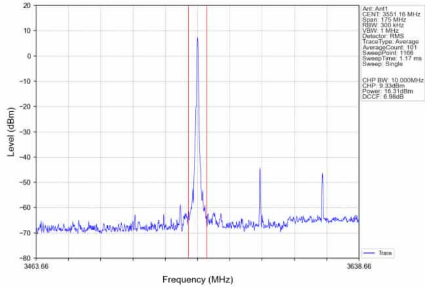
n78d_30kHz_SISO_NTNV_70MHz_CP-OFDM_64_QAM_3585MHz_Edge_1RB_Right_Ant1
