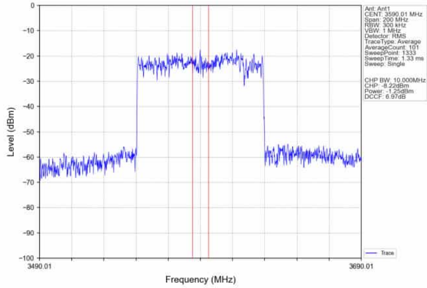
n78d_30kHz_SISO_NTNV_80MHz_CP-OFDM_256_QAM_3590.01MHz_Inner_Full_Ant1
