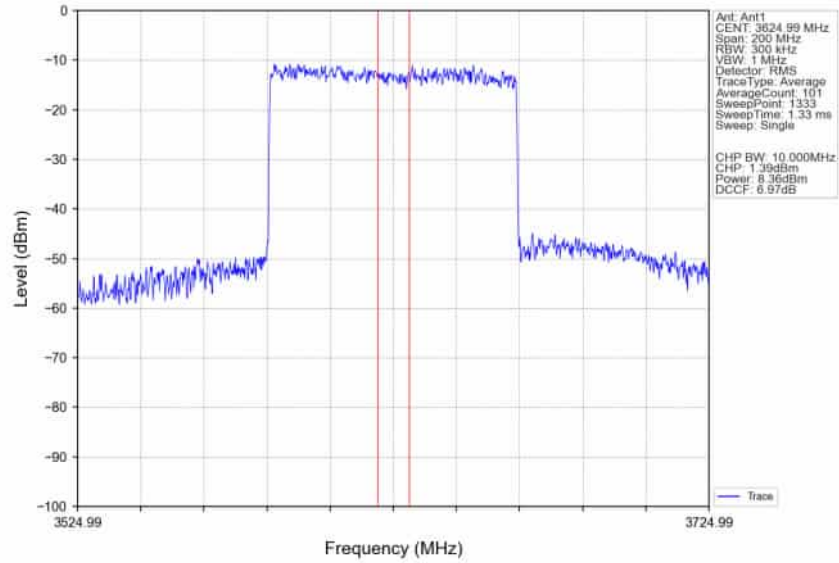
n78d_30kHz_SISO_NTNV_80MHz_CP-OFDM_QPSK_3624.99MHz_Inner_Full_Ant1
