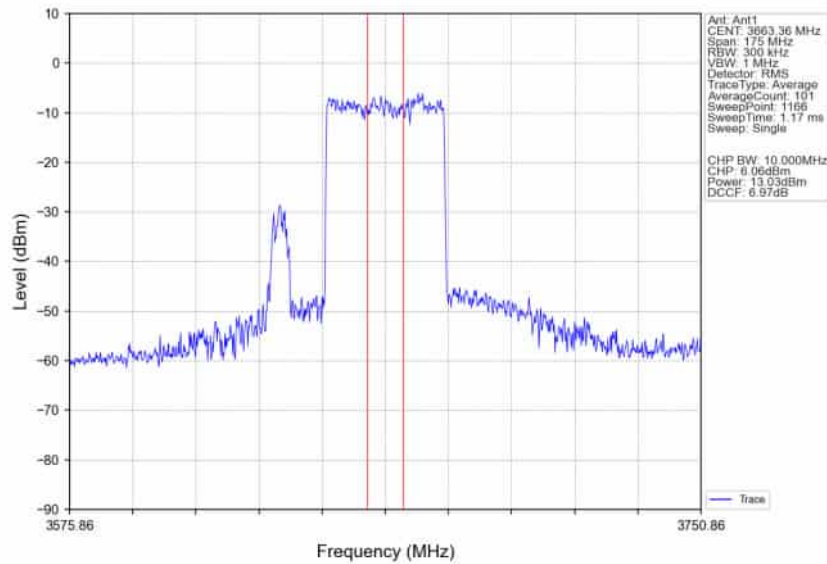
n78d_30kHz_SISO_NTNV_70MHz_DFT-s-OFDM_64_QAM_3664.98MHz_Inner_Full_Ant1
