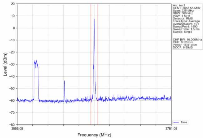
n78d_30kHz_SISO_NTNV_90MHz_DFT-s-OFDM 64 QAM_3624.99MHz_Inner_1RB_Right_Ant1
