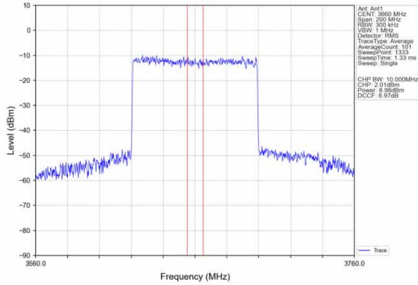
n78d_30kHz_SISO_NTNV_80MHz_CP-OFDM 64 QAM 3660MHz_Inner_Full_Ant1
