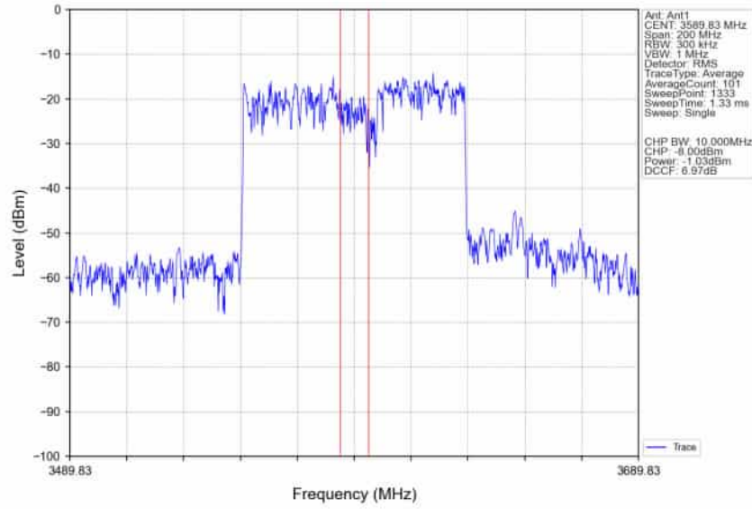
n78d_30kHz_SISO_NTNV_80MHz_DFT-s-OFDM_16_QAM_3590.01MHz_Inner_Full_Ant1
