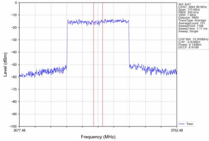
n78d_30kHz_SISO_NTNV_70MHz_CP-OFDM_256_QAM_3664.98MHz_Inner_Full_Ant1
