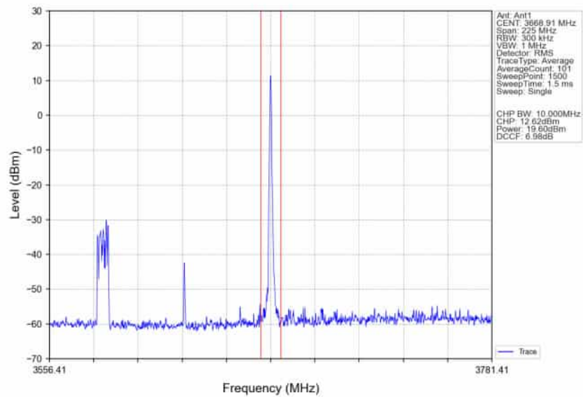
n78d_30kHz_SISO_NTNV_90MHz_DFT-s-OFDM_64_QAM_3624.99MHz_Edge_1RB_Right_Ant1
