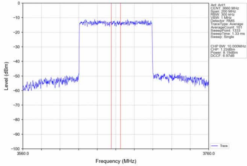
n78d_30kHz_SISO_NTNV_80MHz_CP-OFDM 16 QAM 3660MHz_Inner_Full_Ant1
