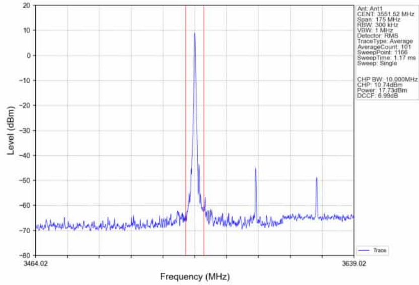
n78d_30kHz_SISO_NTNV_70MHz_CP-OFDM_QPSK_3585MHz_Inner_1RB_Right_Ant1
