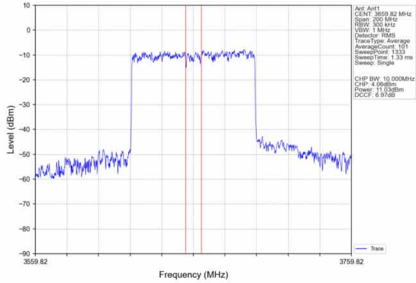
n78d_30kHz_SISO_NTNV_80MHz_DFT-s-OFDM_QPSK_3660MHz_Inner_Full_Ant1
