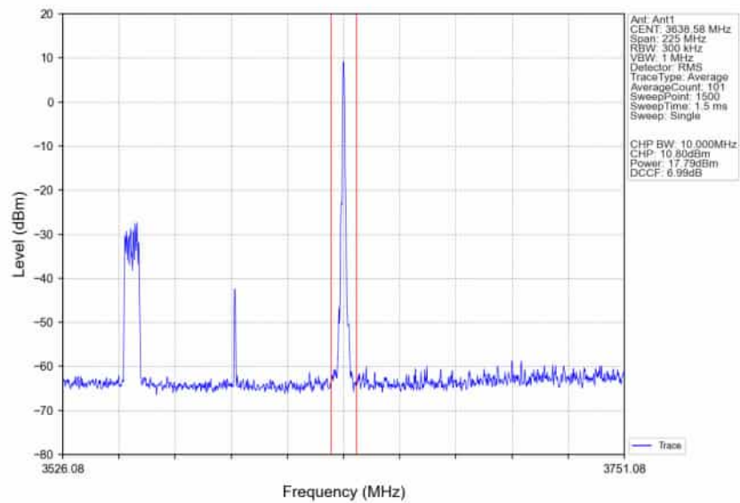
n78d_30kHz_SISO_NTNV_90MHz_DFT-s-OFDM_256_QAM_3595.02MHz_Inner_1RB_Right_Ant1
