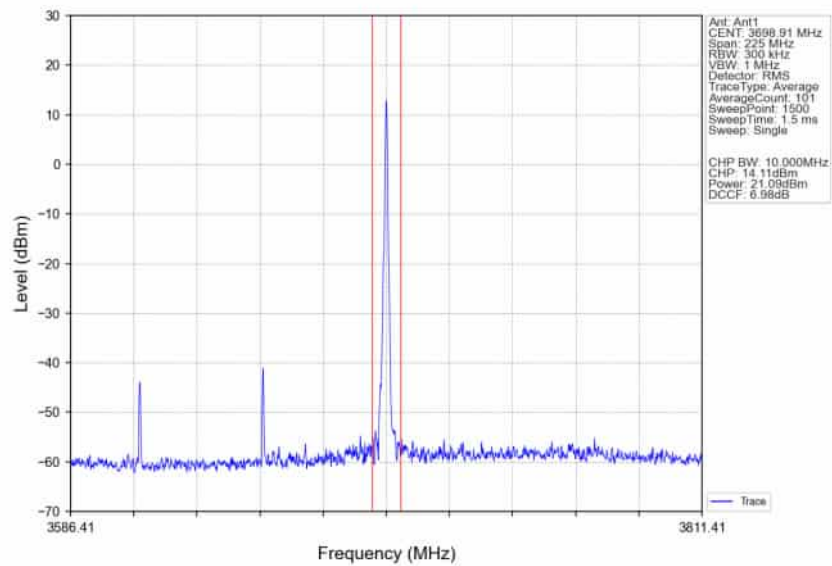
n78d_30kHz_SISO_NTNV_90MHz_DFT-s-OFDM_16_QAM_3654.99MHz_Edge_1RB_Right_Ant1
