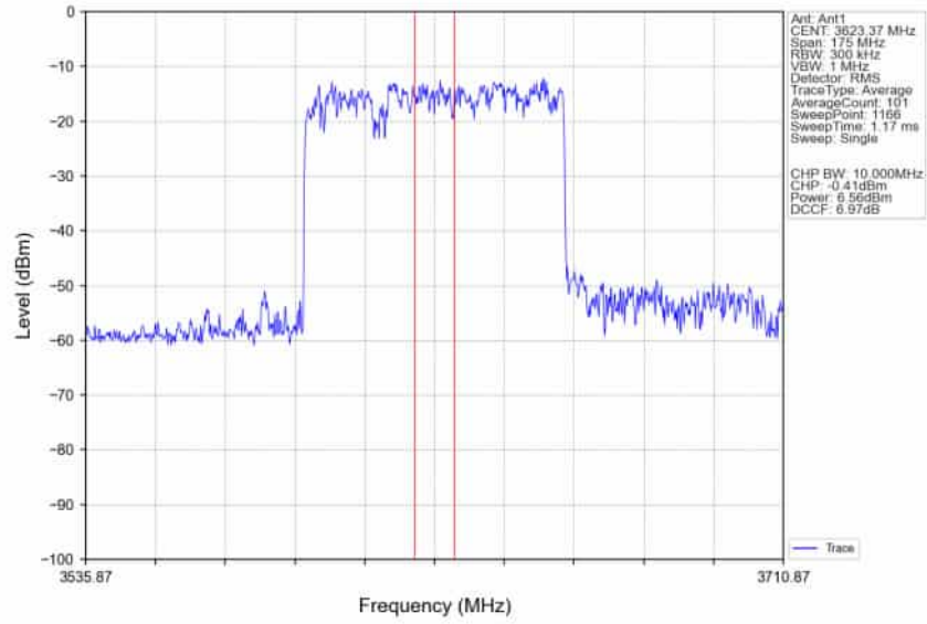
n78d_30kHz_SISO_NTNV_70MHz_DFT-s-OFDM_64_QAM_3624.99MHz_Inner_Full_Ant1
