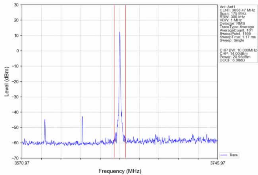
n78d_30kHz_SISO_NTNV_70MHz_CP-OFDM_QPSK_3624.99MHz_Inner_1RB_Right_Ant1
