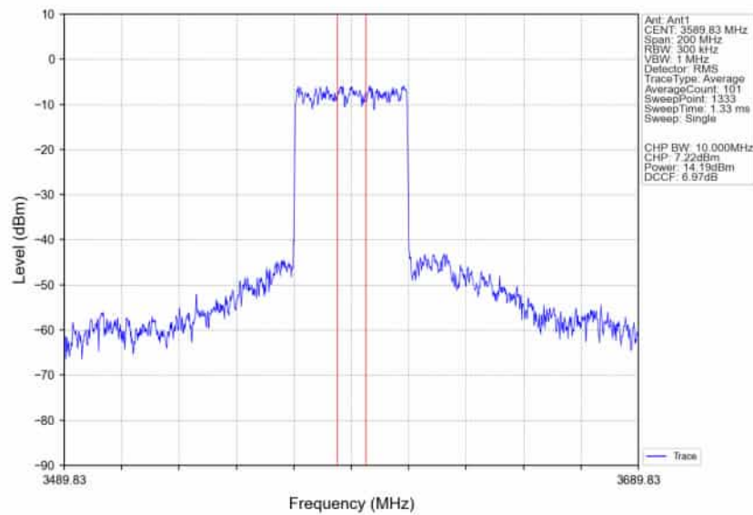
n78d_30kHz_SISO_NTNV_80MHz_DFT-s-OFDM_QPSK_3590.01MHz_Inner_Full_Ant1
