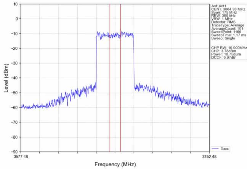
n78d_30kHz_SISO_NTNV_70MHz_CP-OFDM 64 QAM 3664.98MHz_Inner_Full_Ant1
