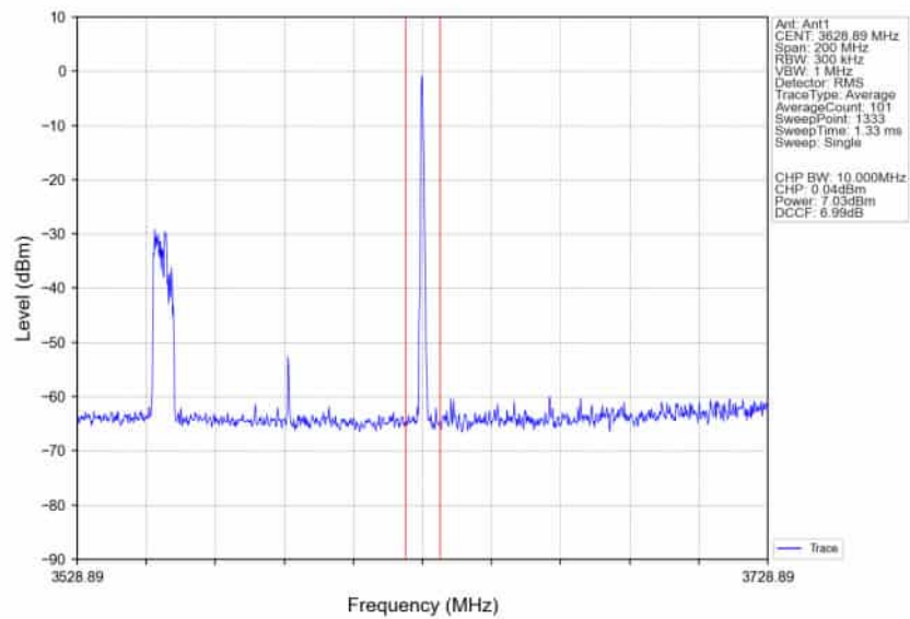
n78d_30kHz_SISO_NTNV_80MHz_DFT-s-OFDM_QPSK_3590.01MHz_Edge_1RB_Right_Ant1
