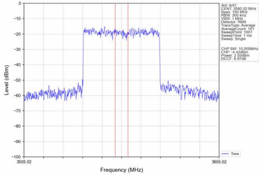
n78d_30kHz_SISO_NTNV_60MHz_CP-OFDM_256_QAM_3580.02MHz_Inner_Full_Ant1
