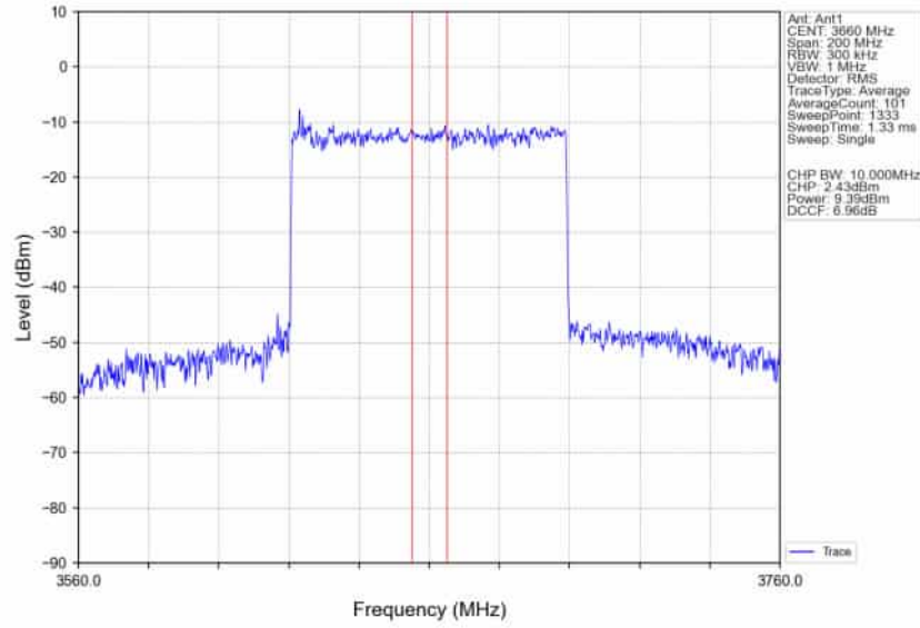
n78d_30kHz_SISO_NTNV_80MHz_CP-OFDM QPSK_3660MHz_Inner_Full_Ant1
