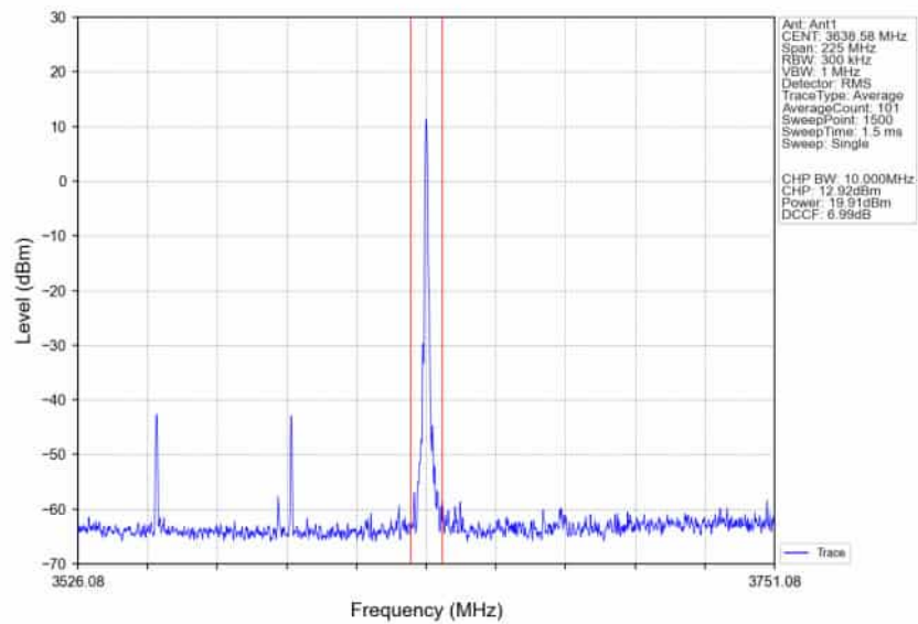
n78d_30kHz_SISO_NTNV_90MHz_DFT-s-OFDM_16_QAM_3595.02MHz_Inner_1RB_Right_Ant1
