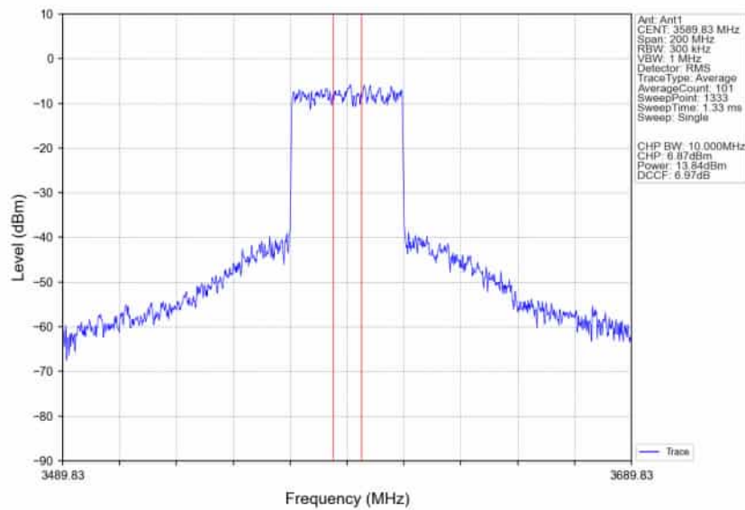
n78d_30kHz_SISO_NTNV_80MHz_DFT-s-OFDM_16_QAM_3590.01MHz_Inner_Full_Ant1
