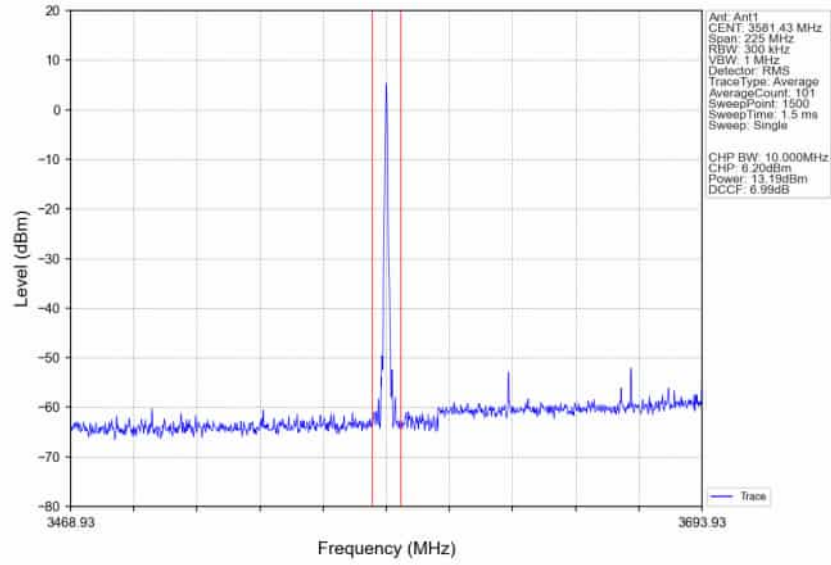
n78d_30kHz_SISO_NTNV_90MHz_DFT-s-OFDM PI/2 BPSK_3624.99MHz_Inner_1RB_Right_Ant1
