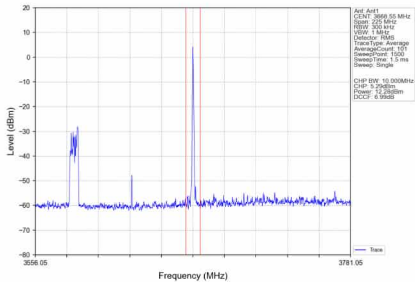
n78d_30kHz_SISO_NTNV_90MHz_DFT-s-OFDM_256_QAM_3624.99MHz_Inner_1RB_Right_Ant1
