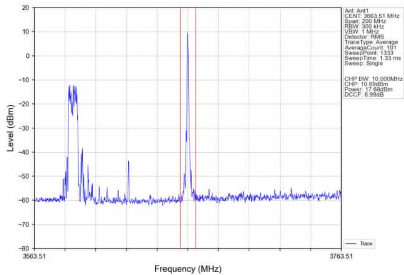
n78d_30kHz_SISO_NTNV_80MHz_CP-OFDM_16_QAM_3624.99MHz_Inner_1RB_Right_Ant1
