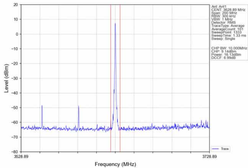
n78d_30kHz_SISO_NTNV_80MHz_CP-OFDM_QPSK_3590.01MHz_Edge_1RB_Right_Ant1
