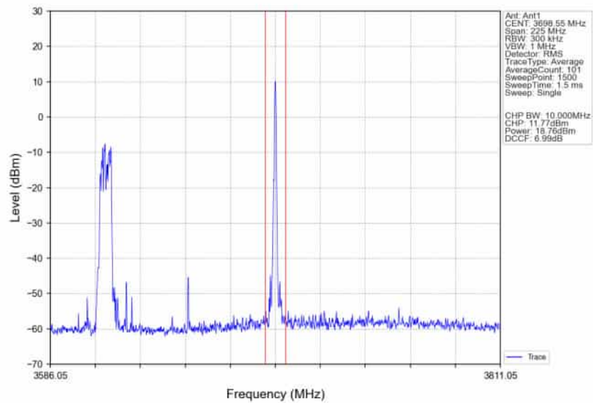
n78d_30kHz_SISO_NTNV_90MHz_DFT-s-OFDM_QPSK_3654.99MHz_Inner_1RB_Right_Ant1
