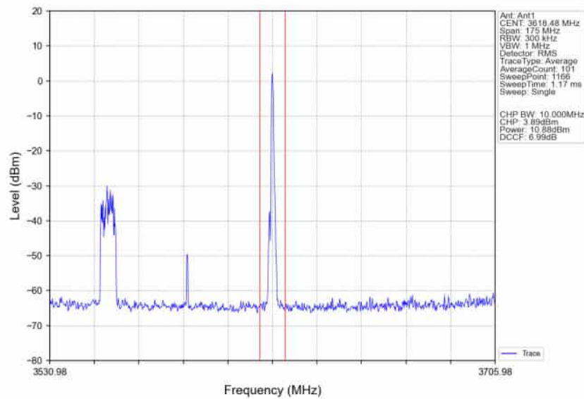
n78d_30kHz_SISO_NTNV_70MHz_CP-OFDM 64 QAM_3585MHz_Inner_1RB_Right_Ant1
