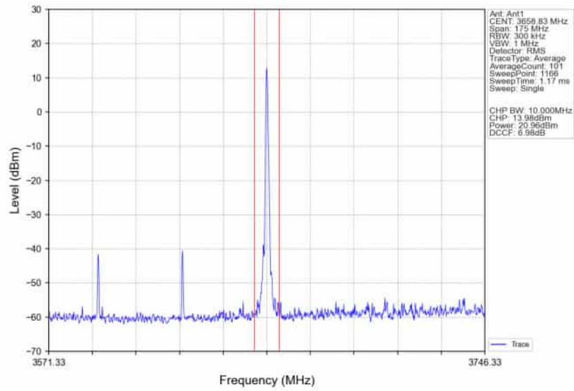
n78d_30kHz_SISO_NTNV_70MHz_DFT-s-OFDM_QPSK_3624.99MHz_Edge_1RB_Right_Ant1
