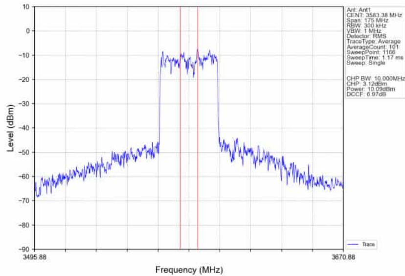
n78d_30kHz_SISO_NTNV_70MHz_DFT-s-OFDM 16 QAM 3585MHz_Inner_Full_Ant1
