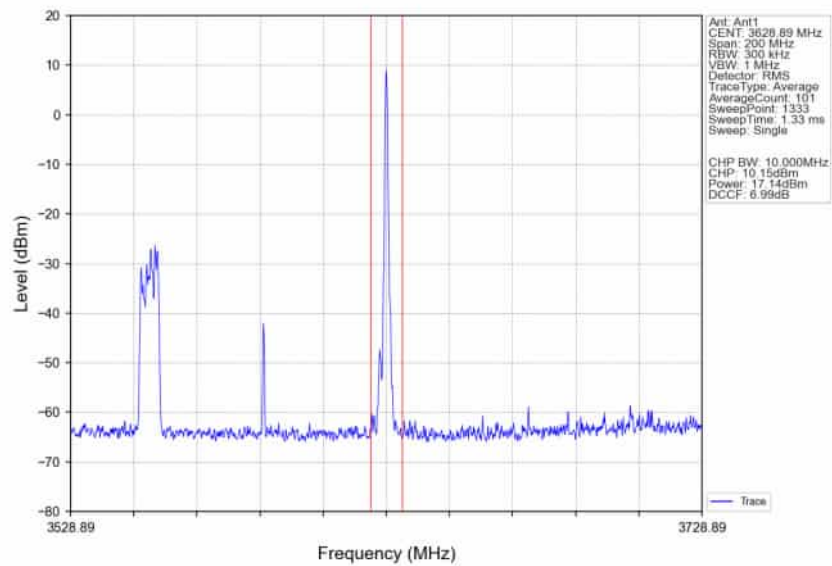
n78d_30kHz_SISO_NTNV_80MHz_DFT-s-OFDM_256_QAM_3590.01MHz_Edge_1RB_Right_Ant1
