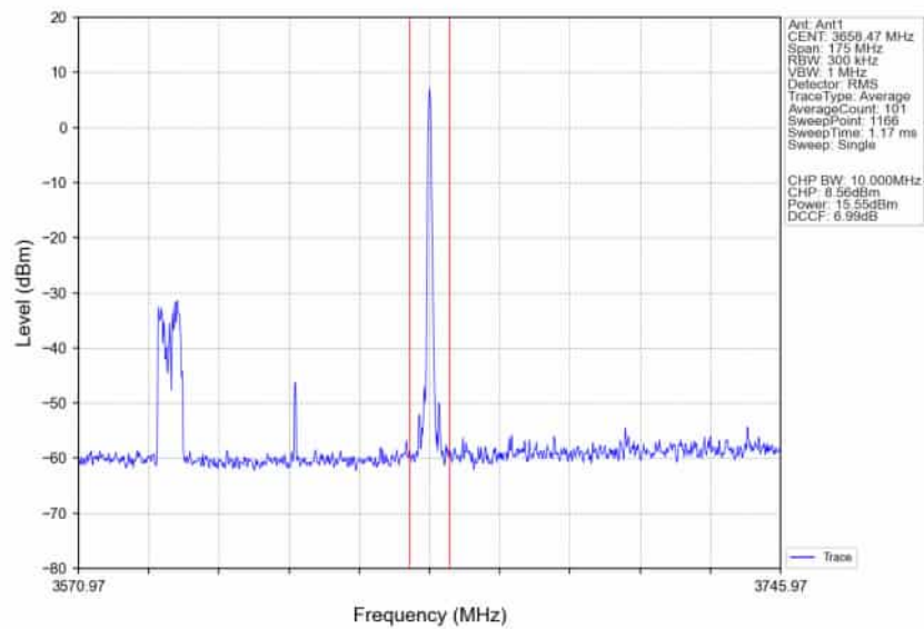
n78d_30kHz_SISO_NTNV_70MHz_DFT-s-OFDM_QPSK_3624.99MHz_Inner_1RB_Right_Ant1
