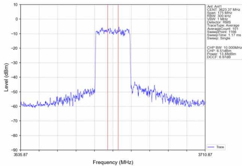
n78d_30kHz_SISO_NTNV_70MHz_DFT-s-OFDM_16_QAM_3624.99MHz_Inner_Full_Ant1
