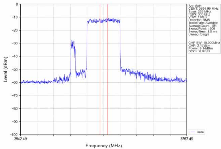
n78d_30kHz_SISO_NTNV_90MHz_CP-OFDM_256_QAM_3654.99MHz_Inner_Full_Ant1
