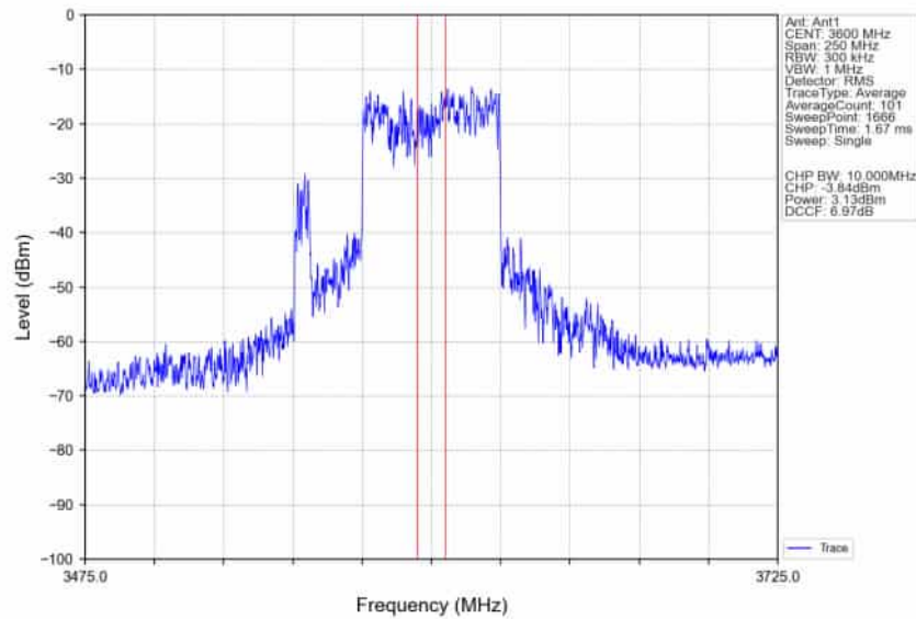
n78d_30kHz_SISO_NTNV_100MHz_CP-OFDM QPSK_3600MHz_Inner_Full_Ant1
