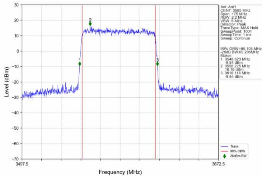
n78d_30kHz_SISO_NTNV_70MHz_DFT-s-OFDM 64 QAM_3585MHz_Outer_Full_Ant1
