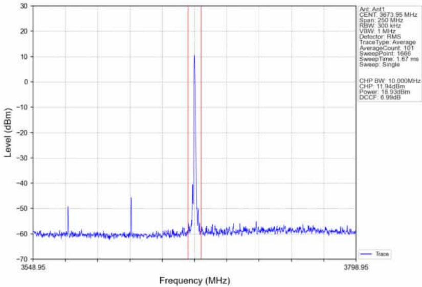
n78d_30kHz_SISO_NTNV_100MHz_DFT-s-OFDM_PI/2_BPSK_3624.99MHz_Edge_1RB_Right_Ant1
