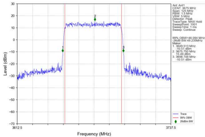
n78d_30kHz_SISO_NTNV_50MHz_DFT-s-OFDM_64_QAM_3675MHz_Outer_Full_Ant1
