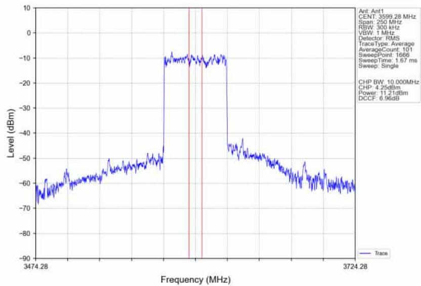
n78d_30kHz_SISO_NTNV_100MHz_DFT-s-OFDM_64_QAM_3600MHz_Inner_Full_Ant1
