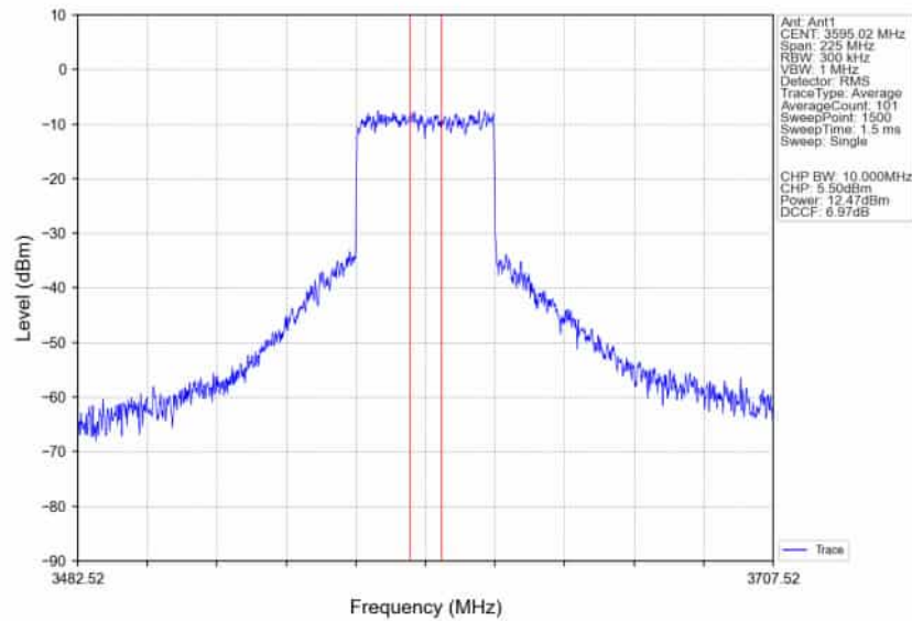
n78d_30kHz_SISO_NTNV_90MHz_CP-OFDM_QPSK_3595.02MHz_Inner_Full_Ant1
