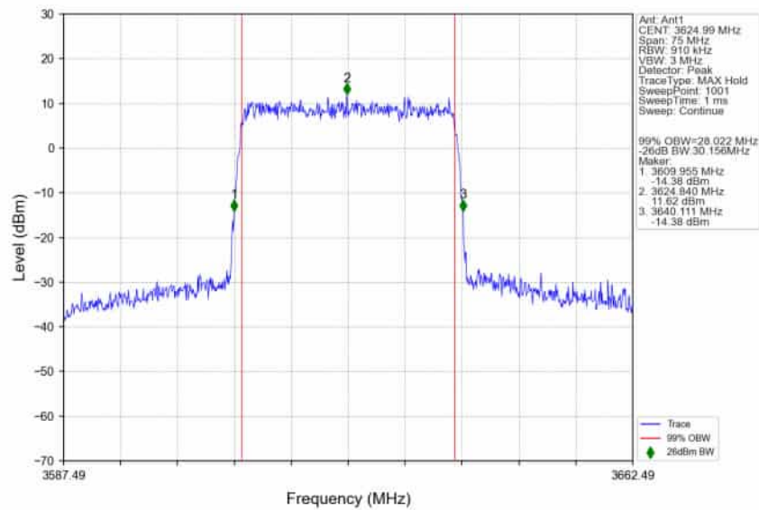
n78d_30kHz_SISO_NTNV_30MHz_CP-OFDM_256_QAM_3624.99MHz_Outer_Full_Ant1
