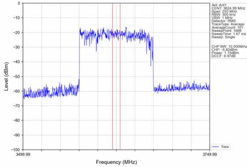
n78d_30kHz_SISO_NTNV_100MHz_CP-OFDM 16 QAM_3624.99MHz_Inner_Full_Ant1
