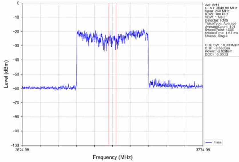
n78d_30kHz_SISO_NTNV_100MHz_CP-OFDM_256_QAM_3649.98MHz_Inner_Full_Ant1
