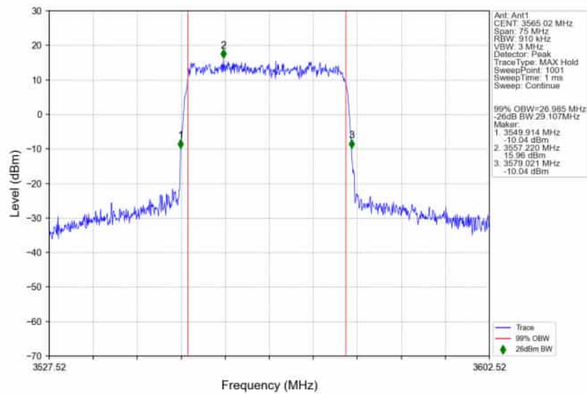
n78d_30kHz_SISO_NTNV_30MHz_DFT-s-OFDM_64_QAM_3565.02MHz_Outer_Full_Ant1
