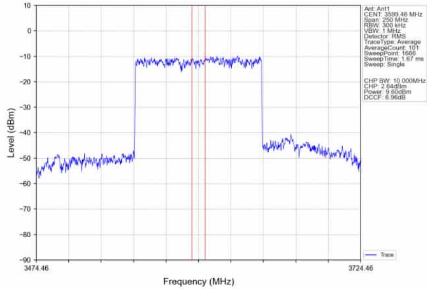
n78d_30kHz_SISO_NTNV_100MHz_DFT-s-OFDM QPSK_3600MHz_Inner_Full_Ant1
