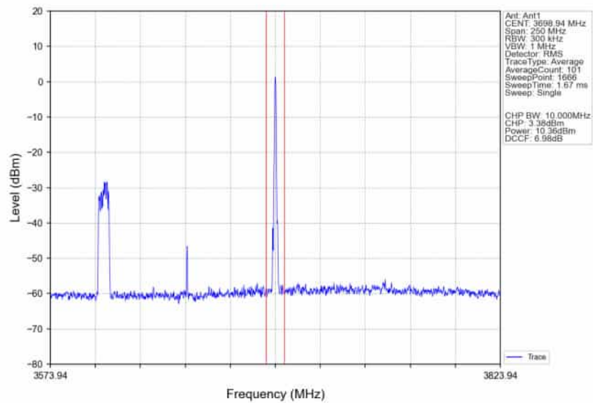
n78d_30kHz_SISO_NTNV_100MHz_DFT-s-OFDM_64_QAM_3649.98MHz_Edge_1RB_Right_Ant1
