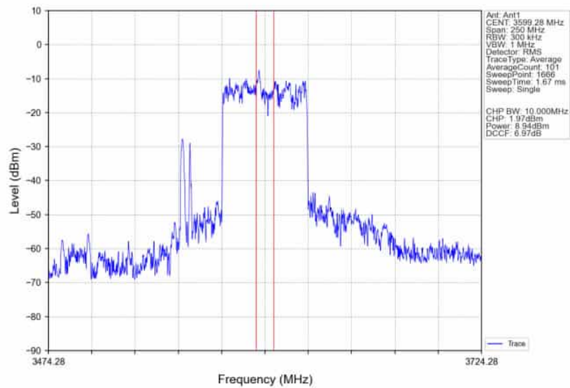
n78d_30kHz_SISO_NTNV_100MHz_DFT-s-OFDM QPSK_3600MHz_Inner_Full_Ant1
