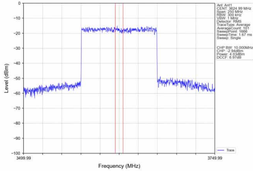
n78d_30kHz_SISO_NTNV_100MHz_CP-OFDM_256_QAM_3624.99MHz_Inner_Full_Ant1
