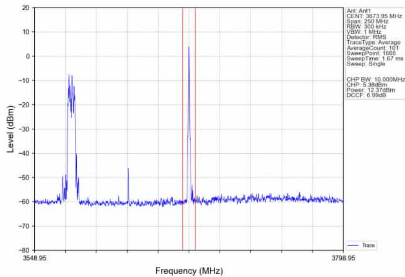
n78d_30kHz_SISO_NTNV_100MHz_CP-OFDM 256 QAM_3624.99MHz_Edge_1RB_Right_Ant1
