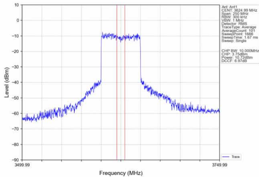
n78d_30kHz_SISO_NTNV_100MHz_CP-OFDM 16 QAM_3624.99MHz_Inner_Full_Ant1
