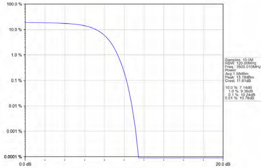
n78e 30kHz SISO NTN 100MHz DFT-s-OFDM 64 QAM 3500.01MHz Outer Full Ant1
