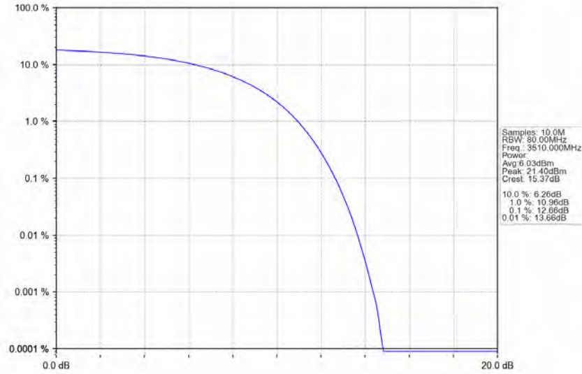
n78e 30kHz SISO NTN 80MHz DFT-s-OFDM 16 QAM 3510MHz Outer Full Ant1
