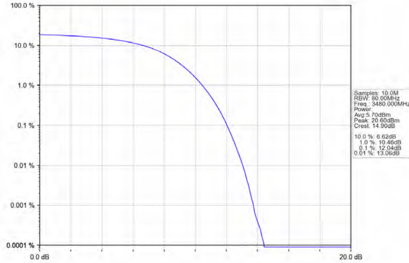
n78e_30kHz_SISO_NTNV_60MHz_DFT-s-OFDM_16_QAM_3480MHz_Outer_Full_Ant1
