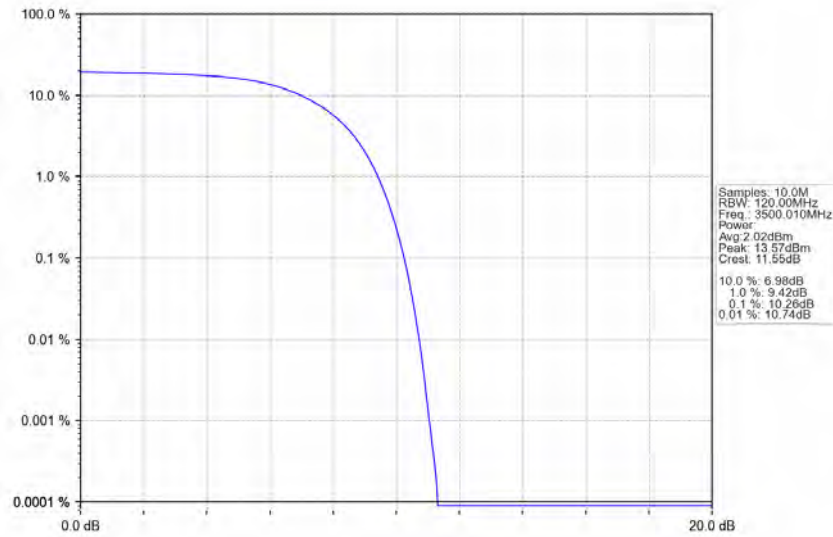
n78e_30kHz_SISO_NTNV_90MHz_CP-OFDM_256_QAM_3500.01MHz_Outer_Full_Ant1
