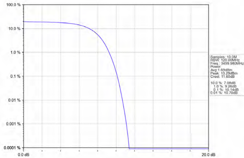
n78e 30kHz SISO NTN 100MHz DFT-s-OFDM 64 QAM 3499.98MHz Outer Full Ant1
