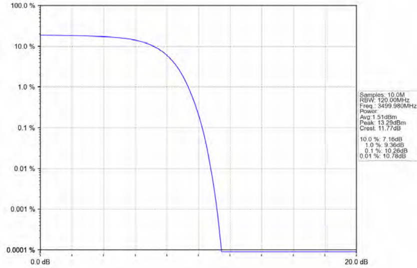
n78e 30kHz SISO NTN 100MHz DFT-s-OFDM 16 QAM 3499.98MHz Outer Full Ant1
