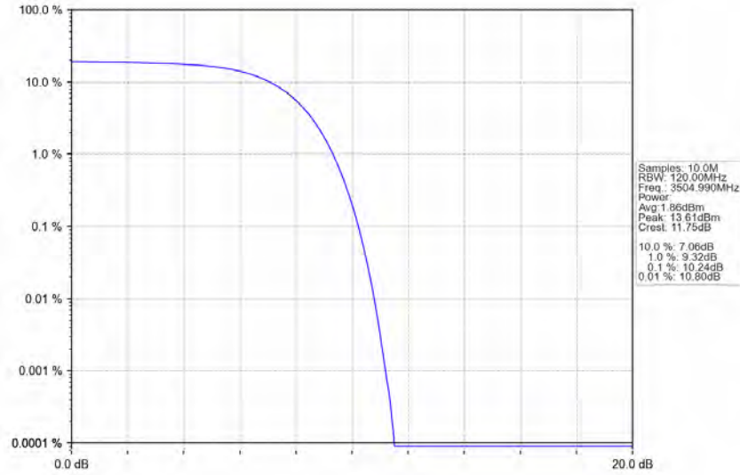
n78e_30kHz_SISO_NTNV_90MHz_CP-OFDM_16_QAM_3504.99MHz_Outer_Full_Ant1
