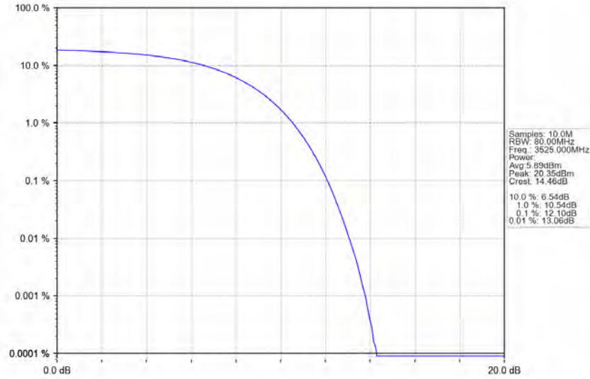
n78e 30kHz SISO NTN 50MHz CP-OFDM 16 QAM 3525MHz Outer Full Ant1
