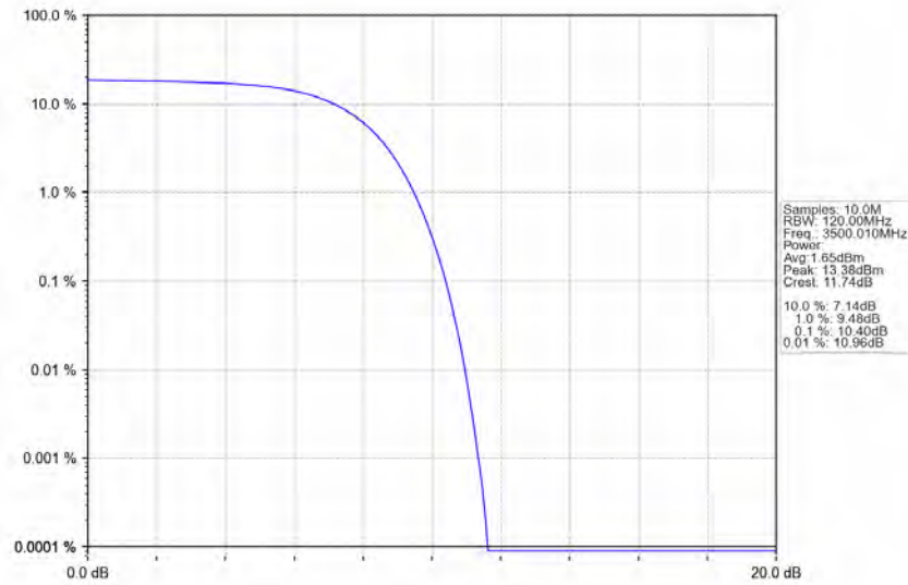
n78e 30kHz SISO NTN 90MHz CP-OFDM 16 QAM 3500.01MHz Outer Full Ant1
