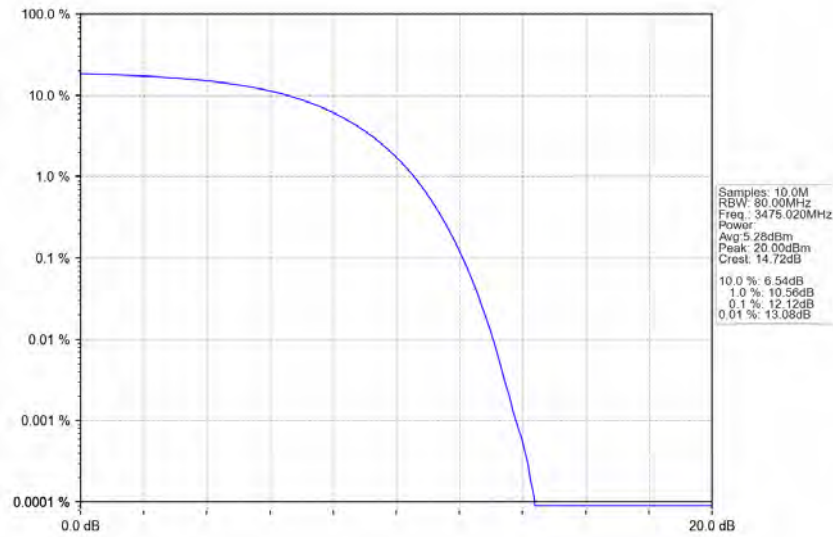
n78e 30kHz SISO NTN 50MHz CP-OFDM 64 QAM 3475.02MHz Outer Full Ant1
