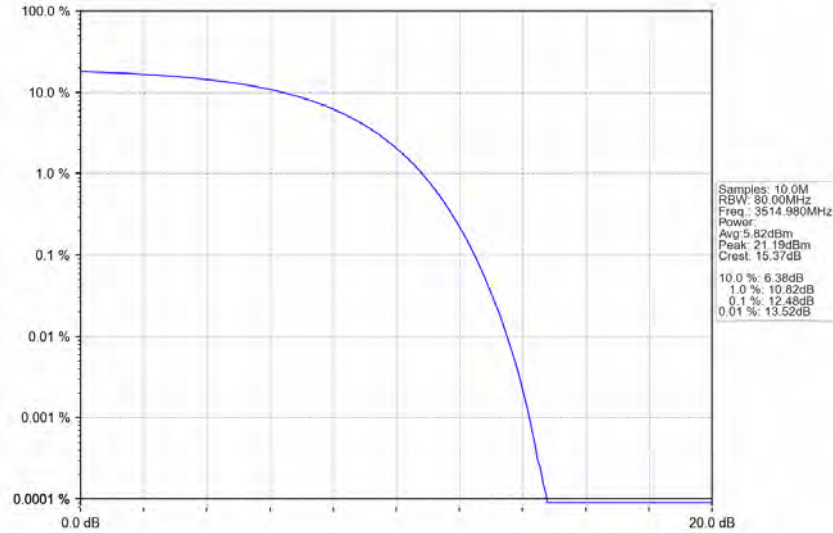
n78e 30kHz SISO NTN 70MHz CP-OFDM 16 QAM 3514.98MHz Outer Full Ant1
