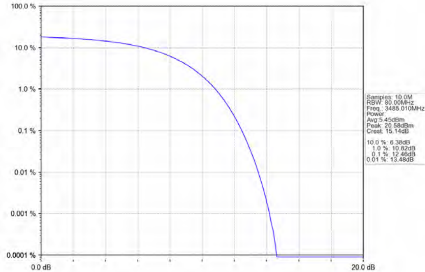
n78e 30kHz SISO NTN 70MHz CP-OFDM 64 QAM 3485.01MHz Outer Full Ant1
