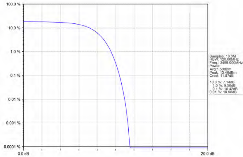
n78e_30kHz_SISO_NTNV_90MHz_CP-OFDM_64_QAM_3495MHz_Outer_Full_Ant1
