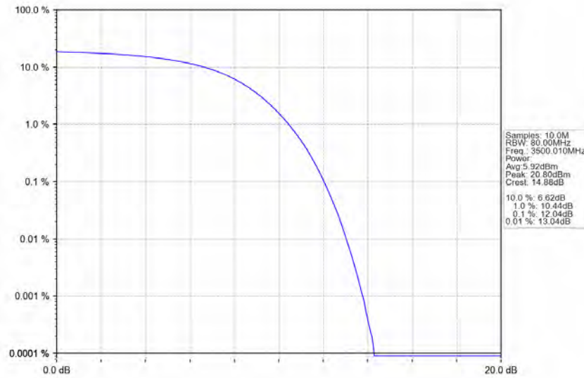
n78e_30kHz_SISO_NTNV_60MHz_DFT-s-OFDM_16_QAM_3500.01MHz_Outer_Full_Ant1
