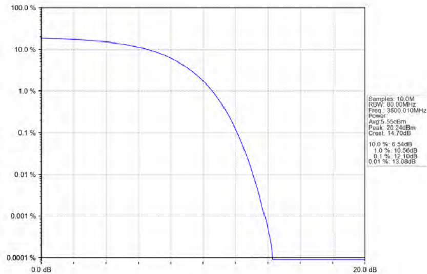
n78e_30kHz_SISO_NTNV_50MHz_CP-OFDM_64_QAM_3500.01MHz_Outer_Full_Ant1
