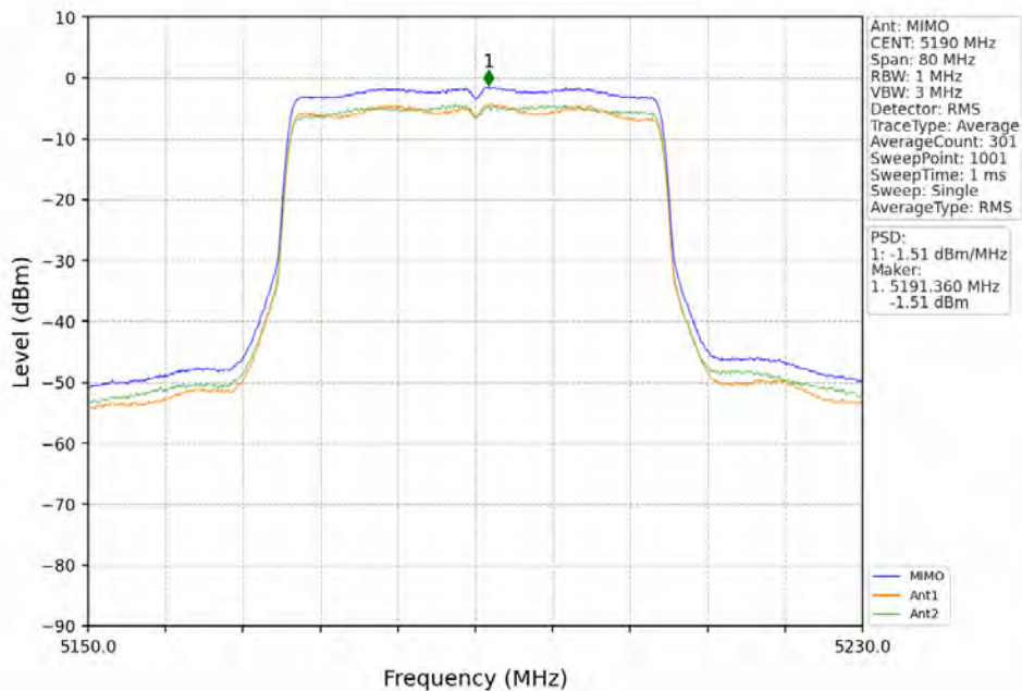
802.11ax(HEW40)_LCH_5190MHz_RU484_Left_MIMO_NTNV
