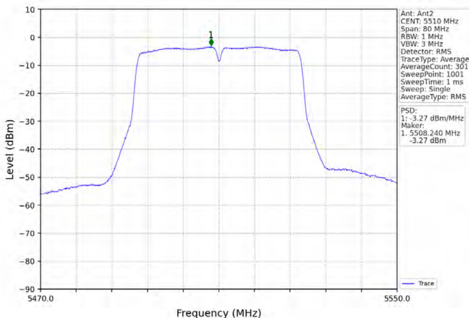
802.11ac(VHT40)_LCH_5510MHz_MIMO_NTNV
