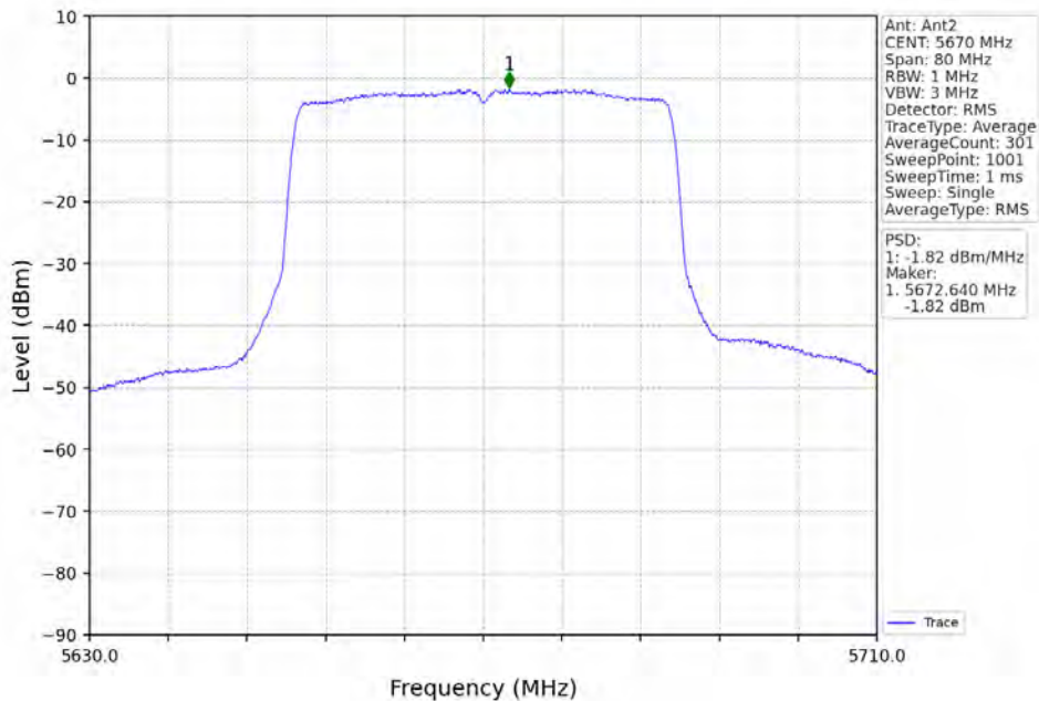
802.11ax(HEW40)_HCH_5670MHz_RU484_Left_MIMO_NTNV
