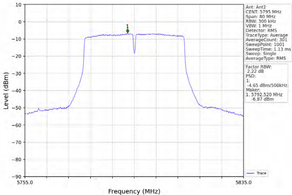
802.11ac(VHT40)_HCH_5795MHz_MIMO_NTNV
