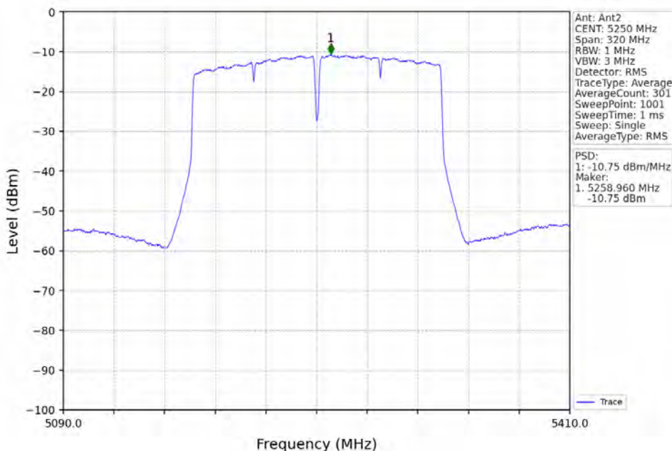
802.11ac(VHT160)_MCH_5250MHz_MIMO_NTNV
