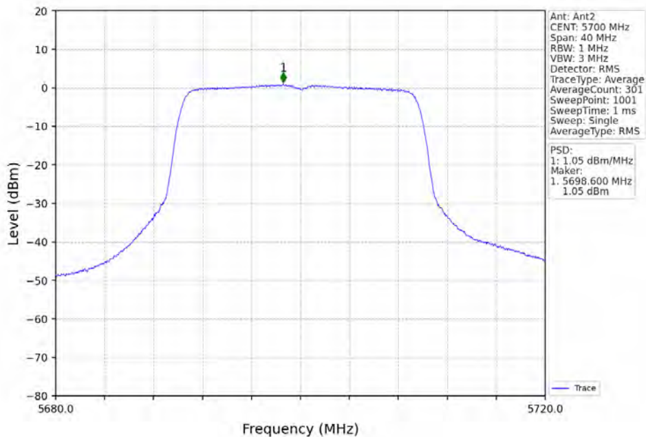
802.11ax(HEW20)_HCH_5700MHz_RU242_Left_Ant2_NTNV
