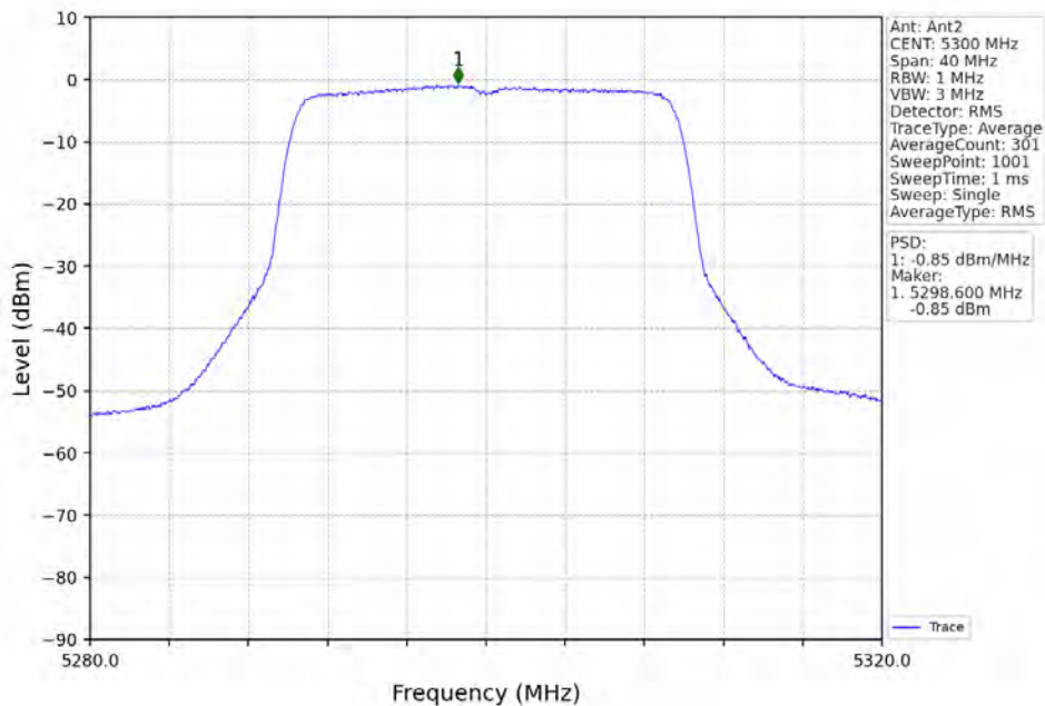
802.11ax(HEW20)_MCH_5300MHz_RU242_Left_Ant2_NTNV
