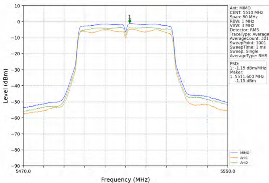
802.11ac(VHT40)_LCH_5510MHz_MIMO_NTNV
