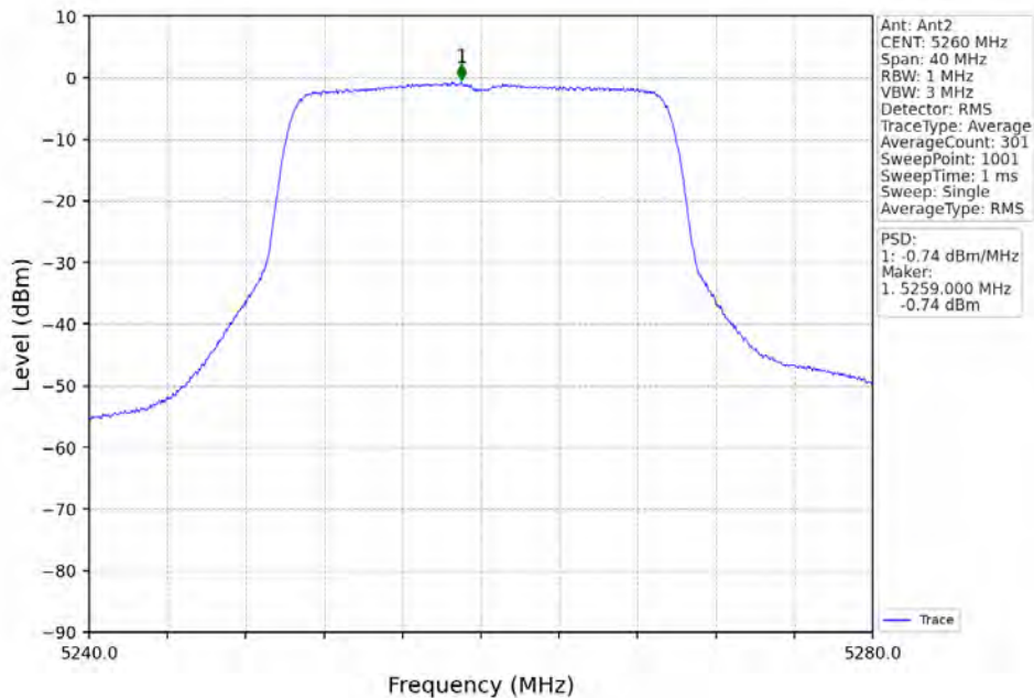
802.11ax(HEW20)_LCH_5260MHz_RU242_Left_MIMO_NTNV
