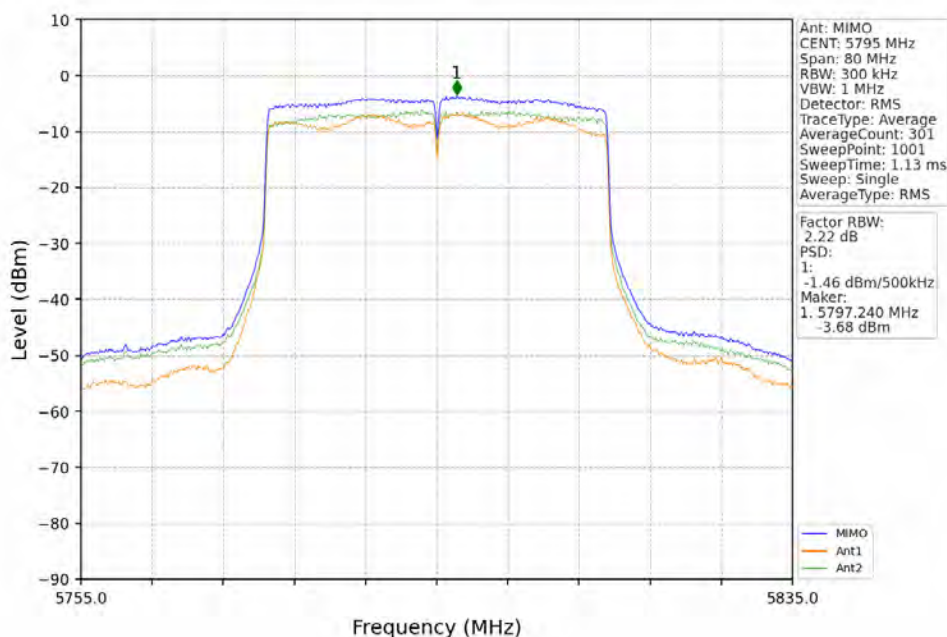
802.11ax(HEW40)_HCH_5795MHz_RU484_Left_MIMO_NTNV
