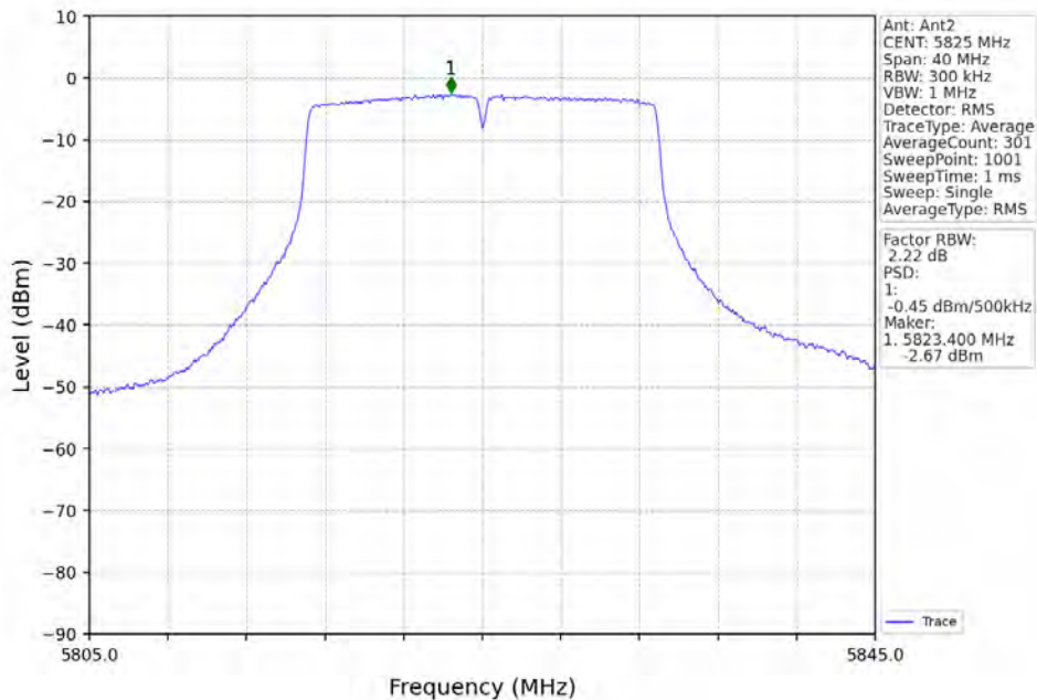
802.11ac(VHT20)_HCH_5825MHz_MIMO_NTNV
