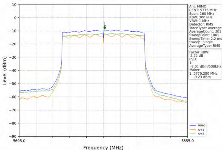
802.11ax(HEW80)_MCH_5775MHz_RU996_Left_MIMO_NTNV
