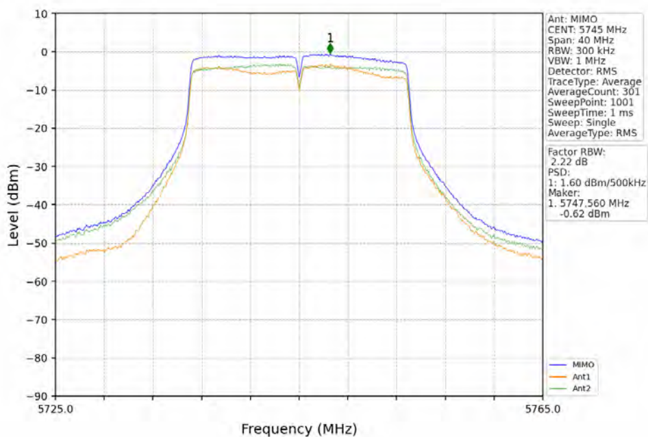
802.11ac(VHT20)_LCH_5745MHz_MIMO_NTNV
