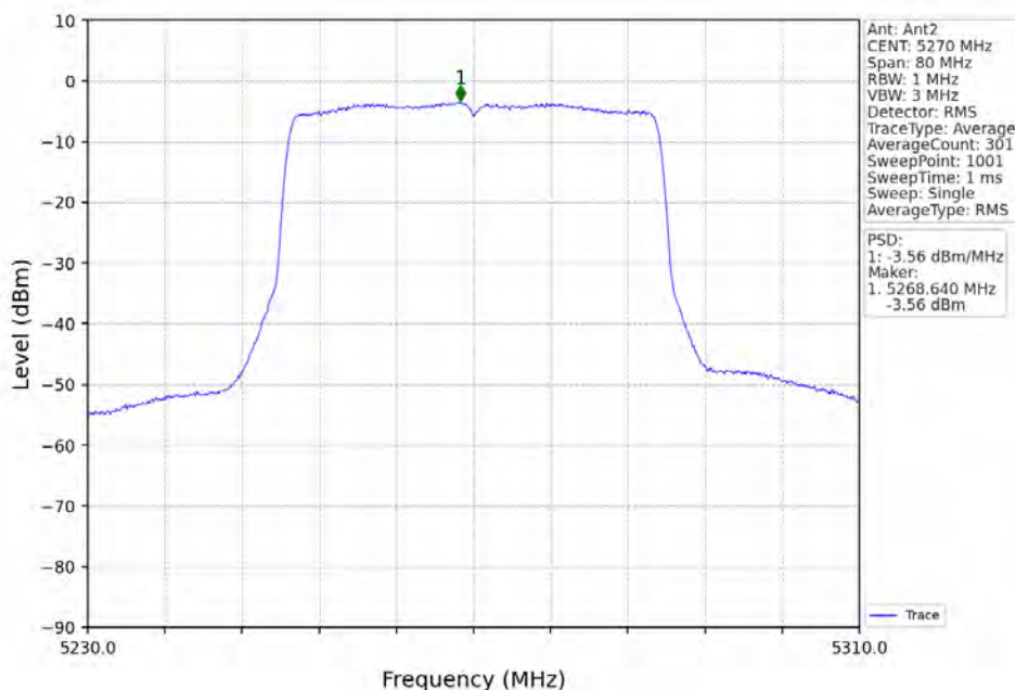
802.11ax(HEW40)_LCH_5270MHz_RU484_Left_MIMO_NTNV
