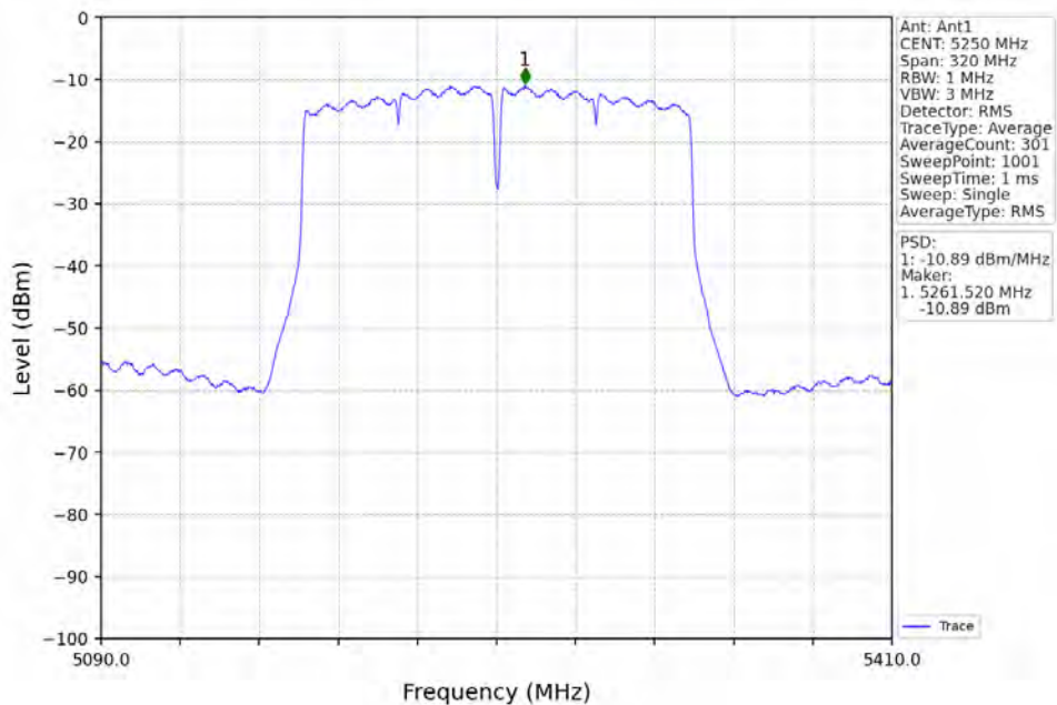
802.11ac(VHT160)_MCH_5250MHz_Ant1_NTNV
