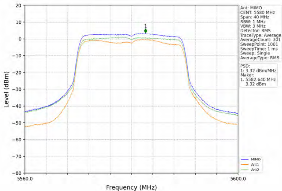
802.11ax(HEW20)_MCH_5580MHz_RU242_Left_MIMO_NTNV
