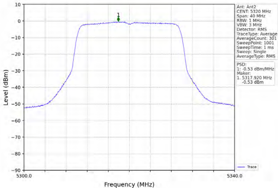
802.11ax(HEW20)_HCH_5320MHz_RU242_Left_MIMO_NTNV
