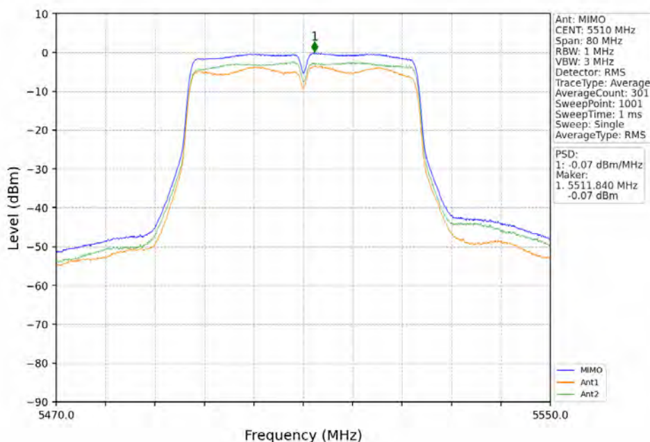
802.11n(HT40)_LCH_5510MHz_MIMO_NTNV
