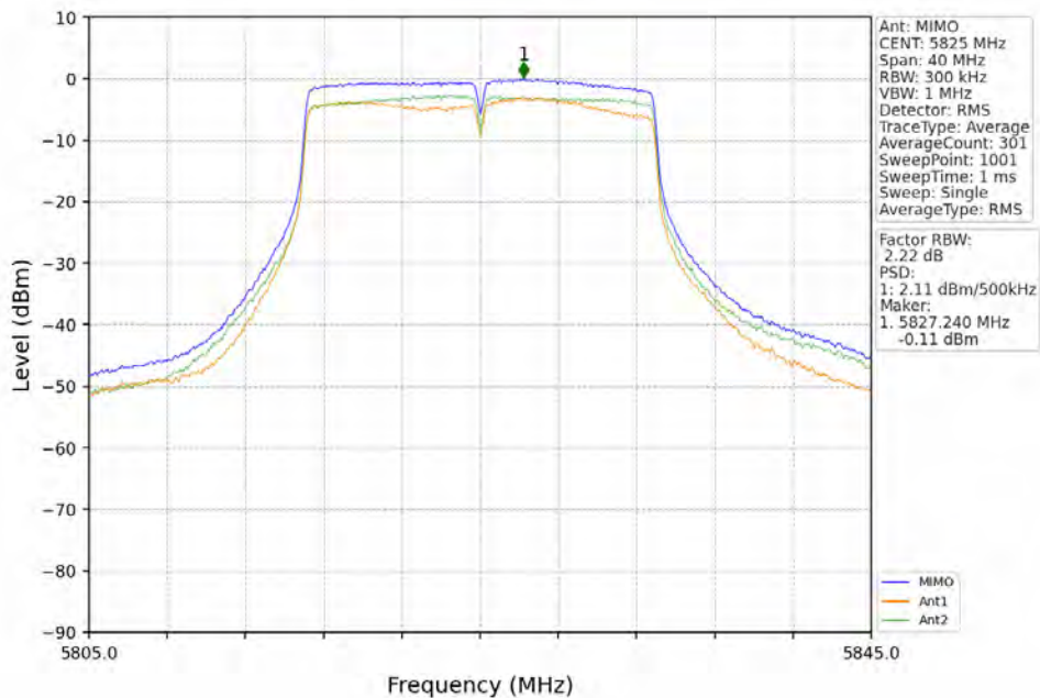
802.11ac(VHT20)_HCH_5825MHz_MIMO_NTNV
