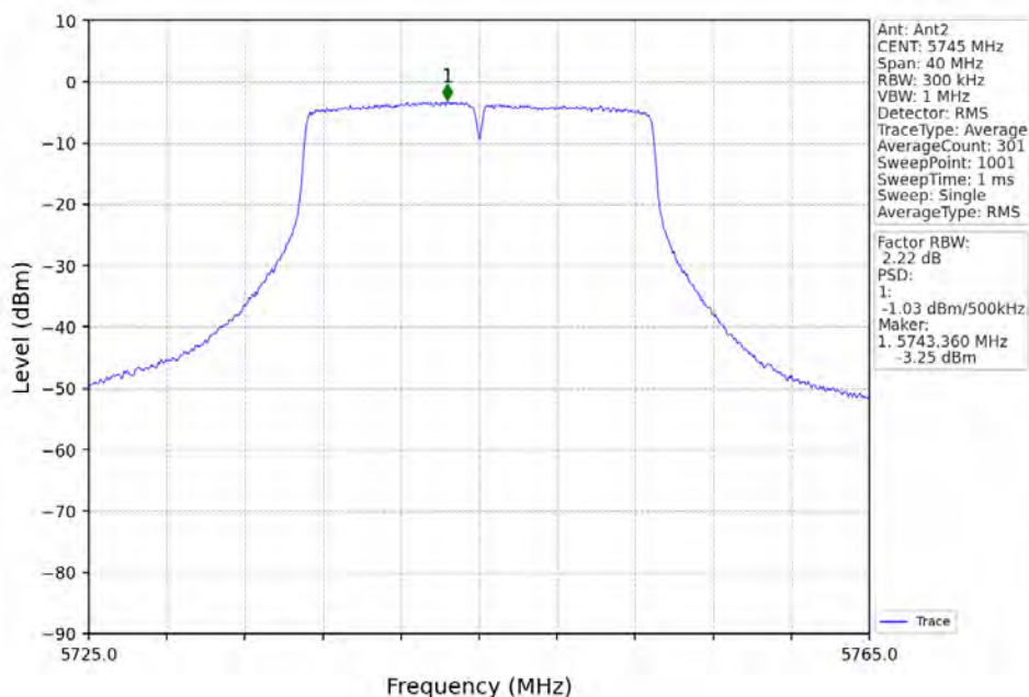
802.11ac(VHT20)_LCH_5745MHz_MIMO_NTNV
