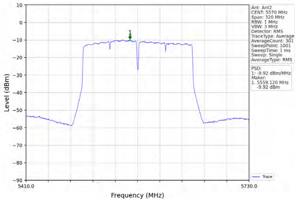
802.11ac(VHT160)_MCH_5570MHz_Ant2_NTNV
