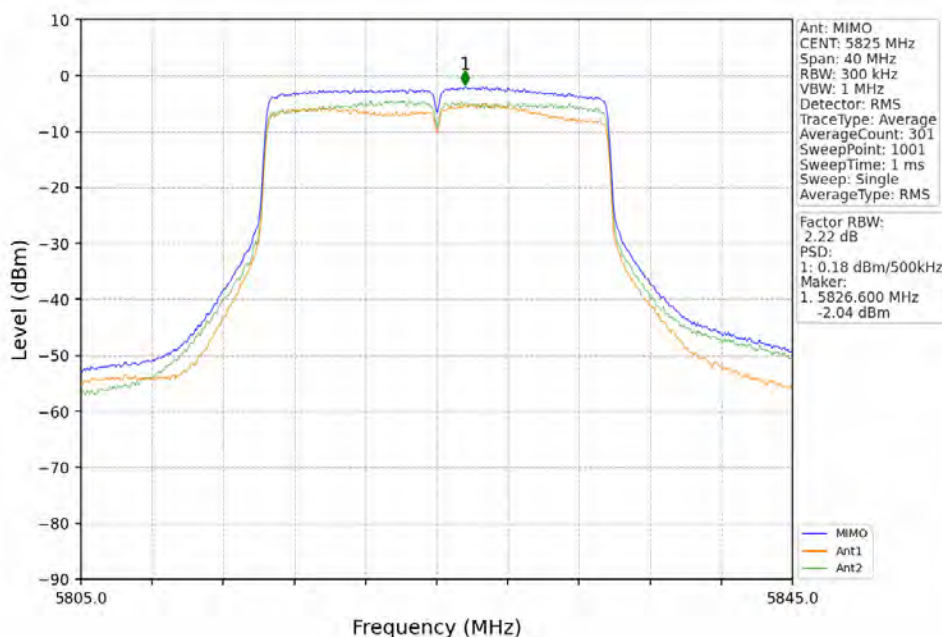
802.11ax(HEW20)_HCH_5825MHz_RU242_Left_MIMO_NTNV
