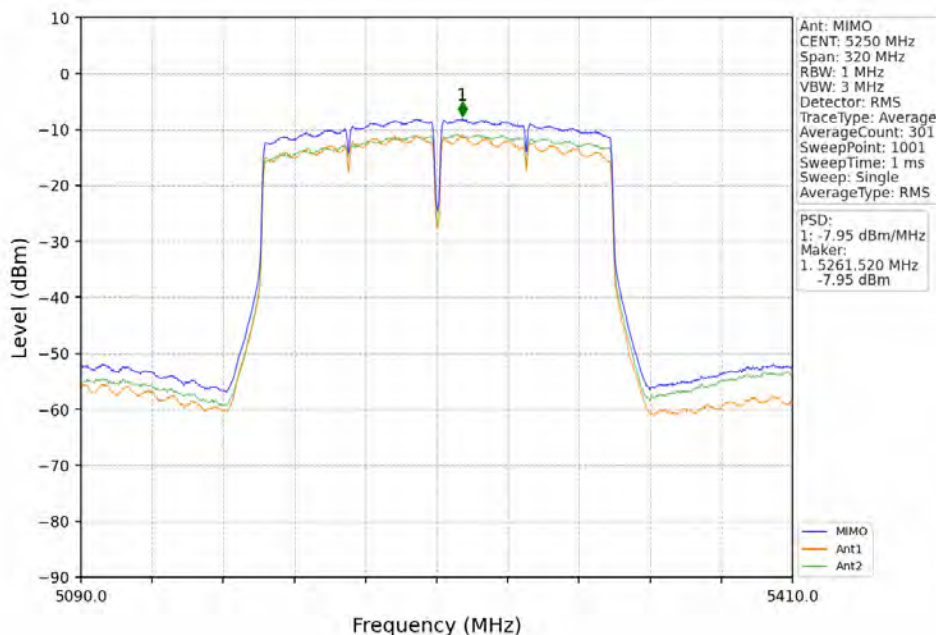
802.11ac(VHT160)_MCH_5250MHz_MIMO_NTNV
