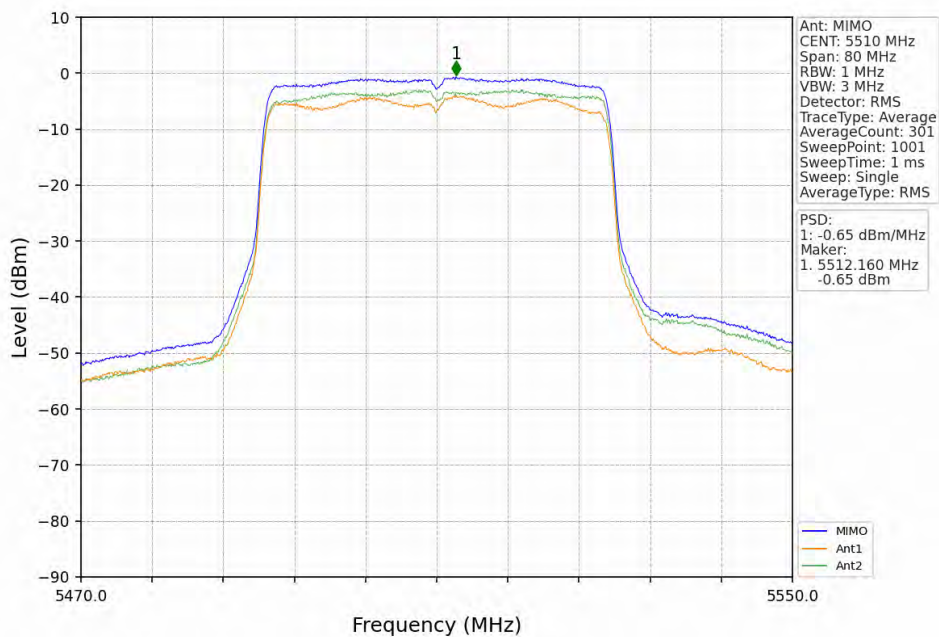
802.11ax(HEW40)_LCH_5510MHz_RU484_Left_MIMO_NTNV
