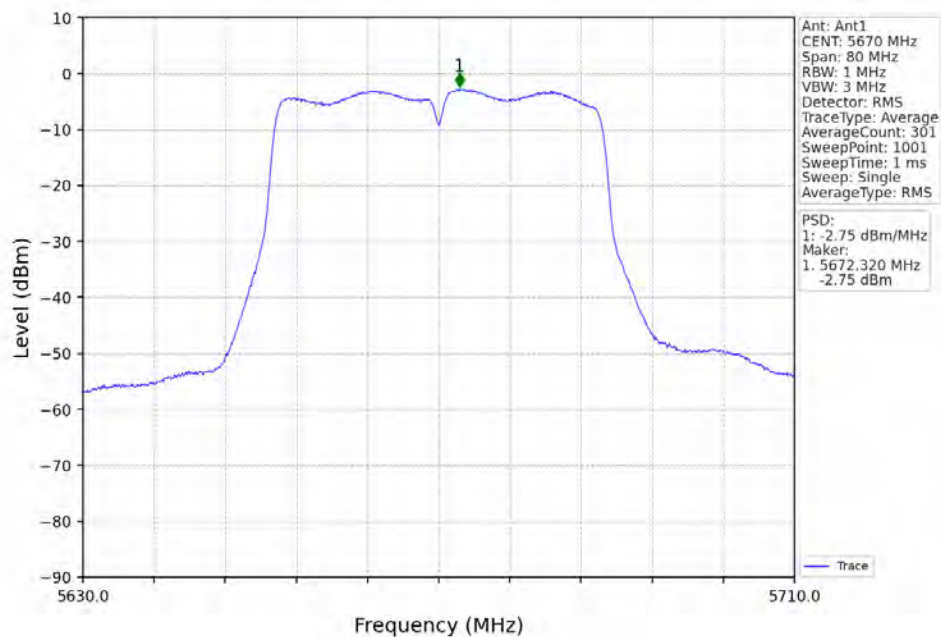
802.11n(HT40)_HCH_5670MHz_Ant1_NTNV
