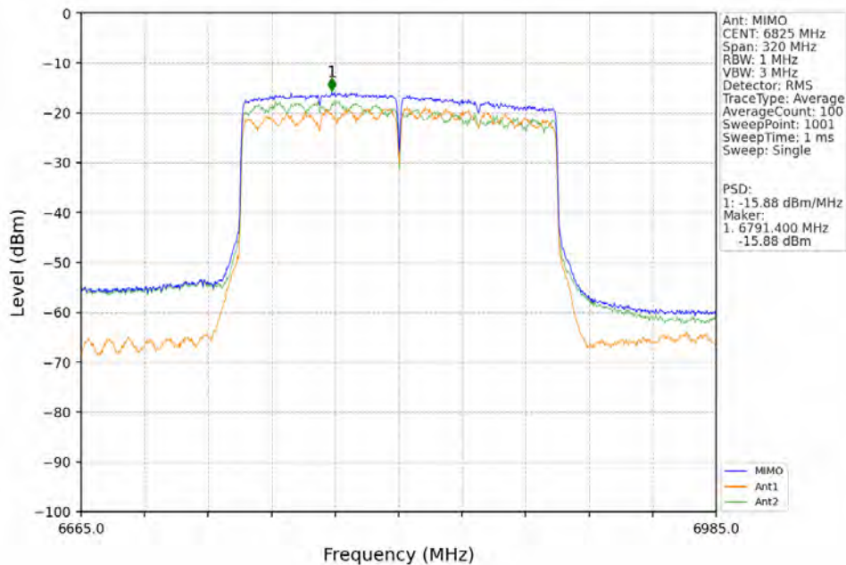
802.11ax(HEW160)_HCH_6825MHz_2xRU996_Left_MIMO_NTNV
