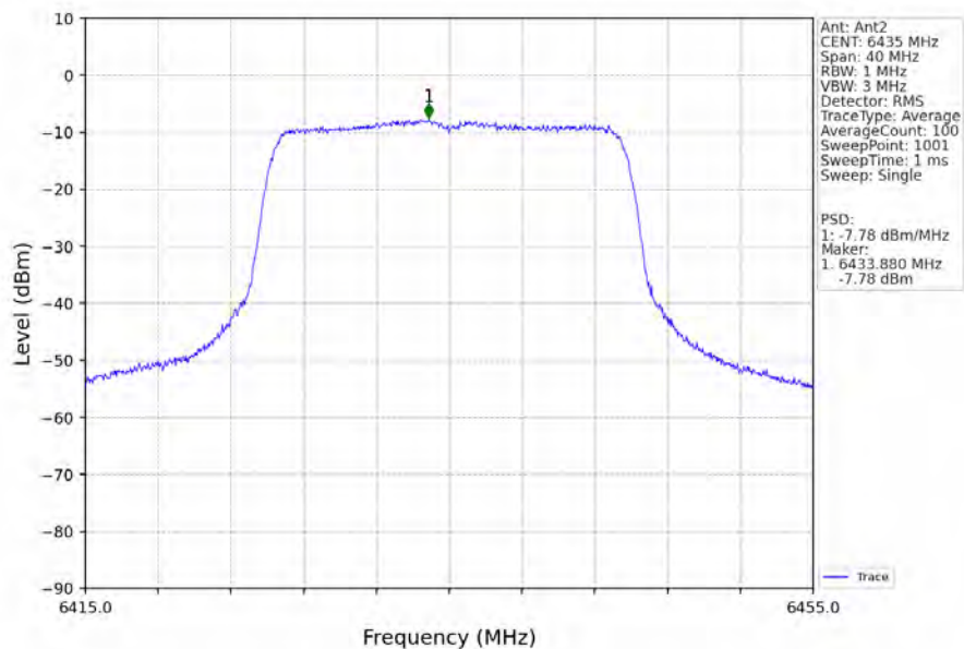
802.11ax(HEW20)_LCH_6435MHz_RU242_Left_Ant2_NTNV
