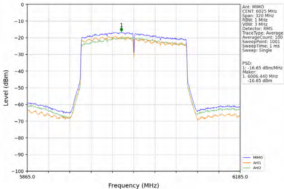
802.11ax(HEW160)_LCH_6025MHz_2xRU996_Left_MIMO_NTNV
