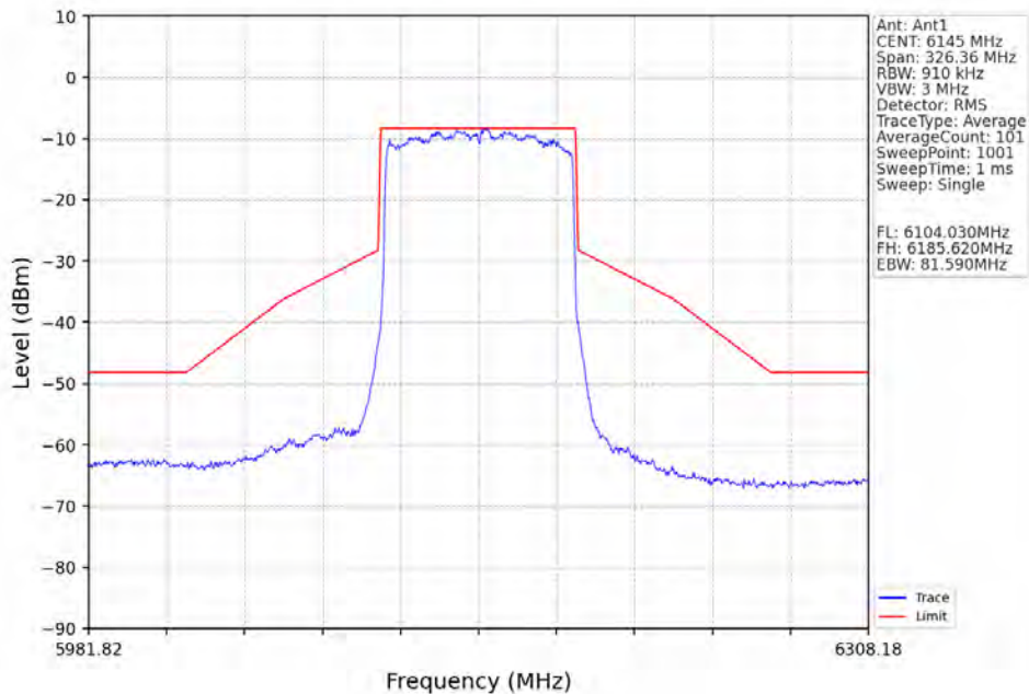
802.11ax(HEW80)_MCH_6145MHz_RU996_Left_Ant1_NTNV
