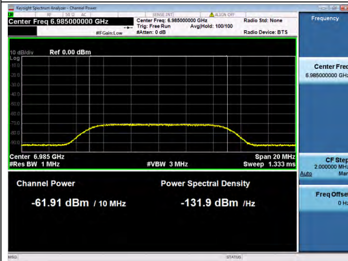
11AX160SISO-Ant 1-6985-Center-6985-Minimal
