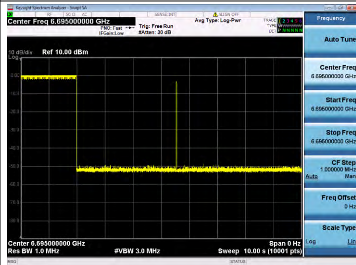
11AX20SISO-Ant 1-6695-Center-6695-Minimal
