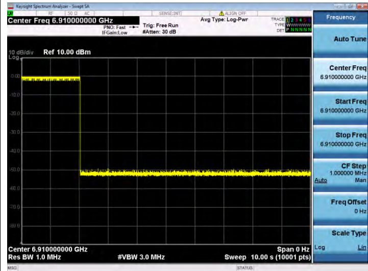
11AX160SISO-Ant 1-6985-Center-6910-Minimal
