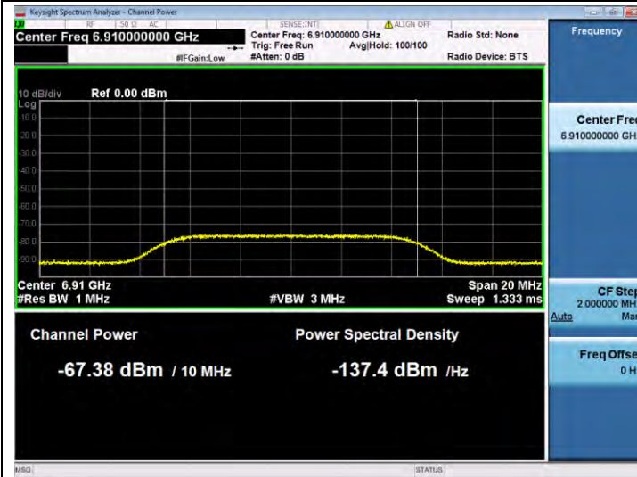
11AX160SISO-Ant 1-6985-Center-6910-Minimal
