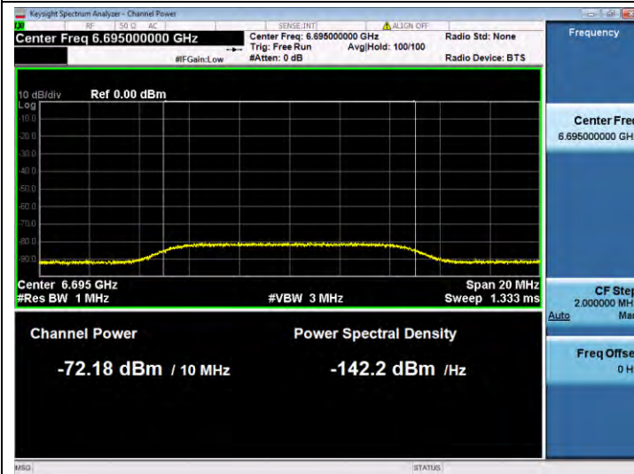
11AX20SISO-Ant 1-6695-Center-6695-Minimal
