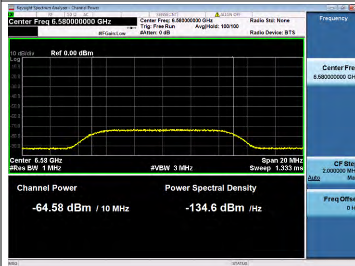
11AX160SISO-Ant 1-6505-Center-6580-Minimal
