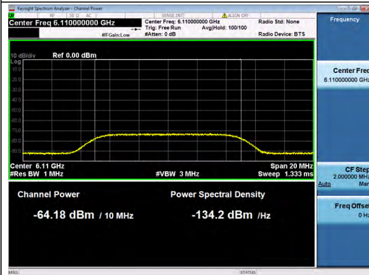
11AX160SISO-Ant 1-6185-Center-6110-Minimal
