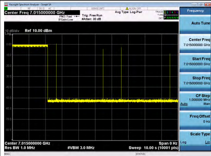
11AX20SISO-Ant 1-7015-Center-7015-Minimal
