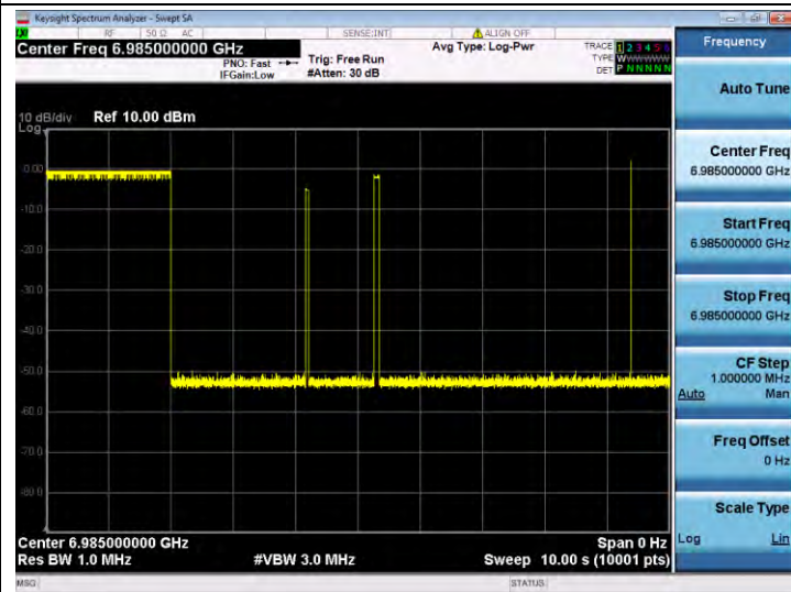
11AX160SISO-Ant 1-6985-Center-6985-Minimal
