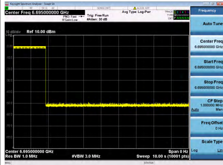
11AX20SISO-Ant 1-6695-Center-6695-Minimal
