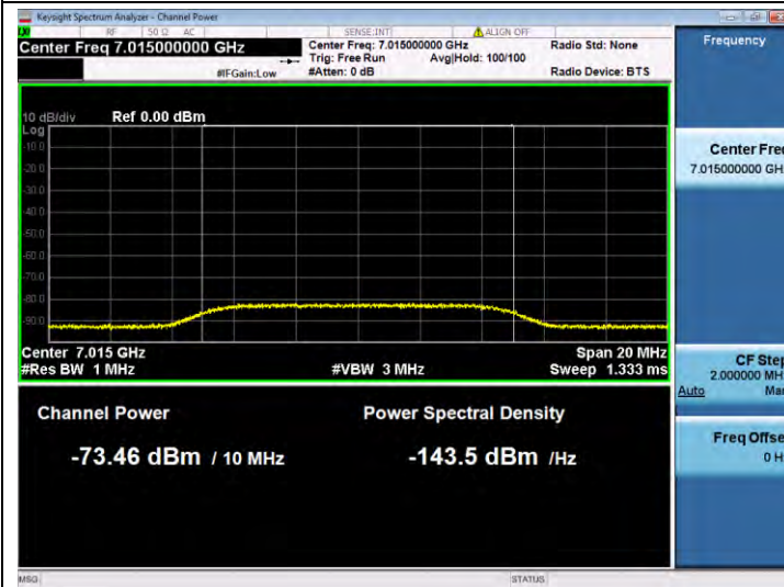
11AX20SISO-Ant 1-7015-Center-7015-Minimal
