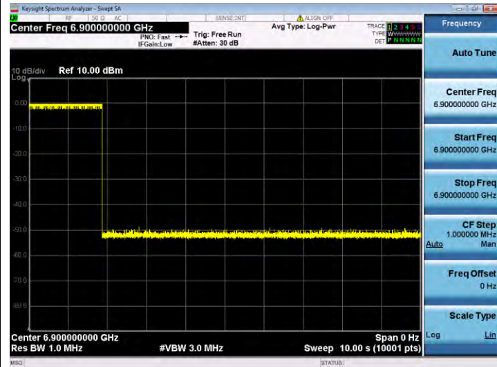
11AX160SISO-Ant 1-6825-Center-6900-Minimal
