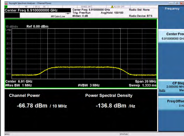
11AX160SISO-Ant 1-6985-Center-6910-Minimal
