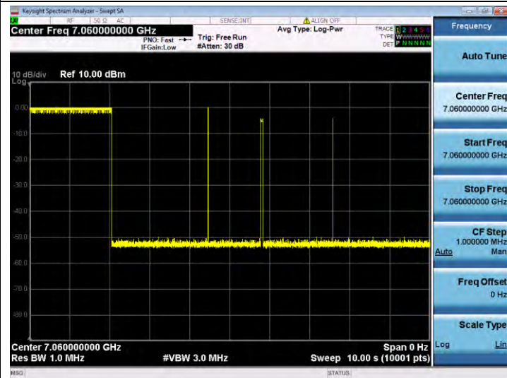
11AX160SISO-Ant 1-6985-Center-7060-Minimal
