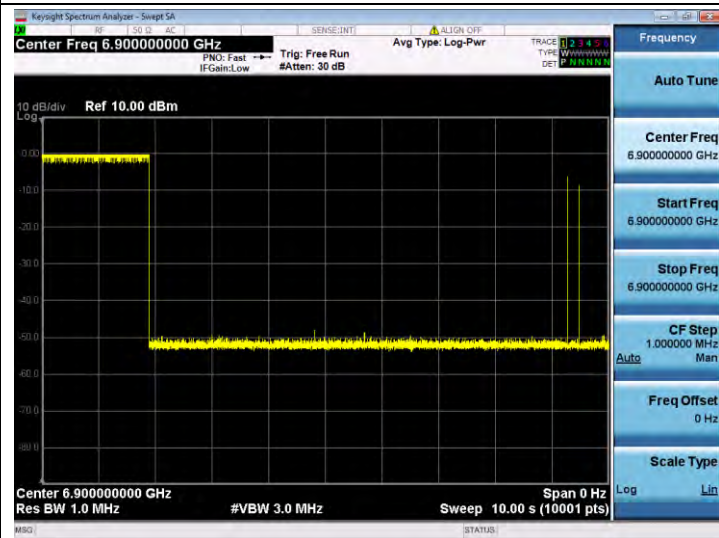
11AX160SISO-Ant 1-6825-Center-6900-Minimal
