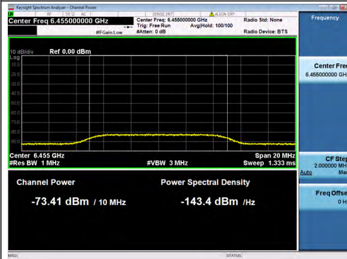
11AX20SISO-Ant 1-6455-Center-6455-Minimal
