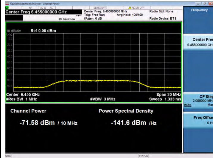
11AX20SISO-Ant 1-6455-Center-6455-Minimal
