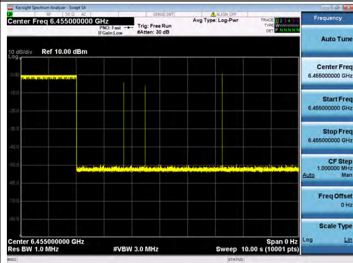
11AX20SISO-Ant 1-6455-Center-6455-Minimal
