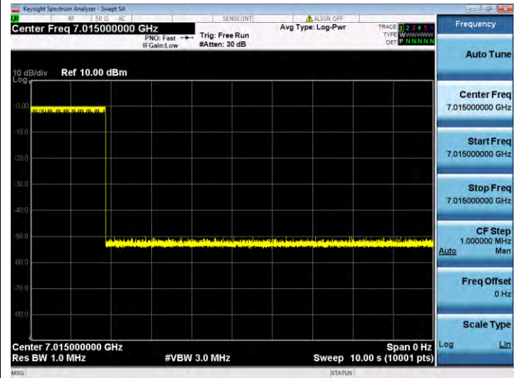
11AX20SISO-Ant 1-7015-Center-7015-Minimal
