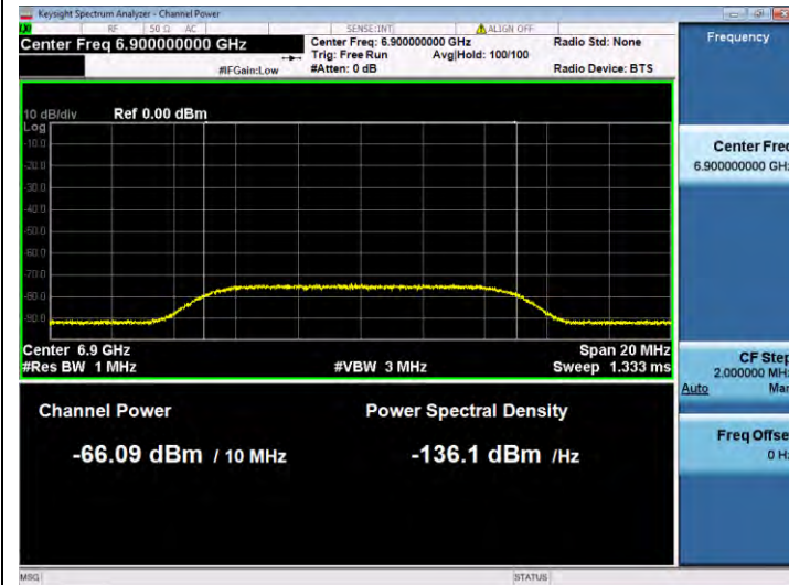
11AX160SISO-Ant 1-6825-Center-6900-Minimal
