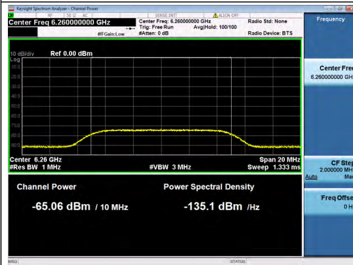
11AX160SISO-Ant 1-6185-Center-6260-Minimal
