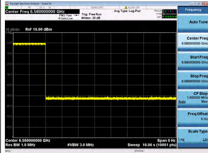
11AX160SISO-Ant 1-6505-Center-6580-Minimal
