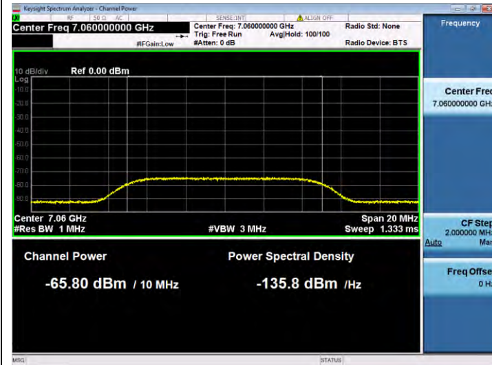
11AX160SISO-Ant 1-6985-Center-7060-Minimal
