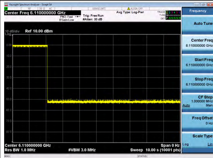
11AX160SISO-Ant 1-6185-Center-6110-Minimal
