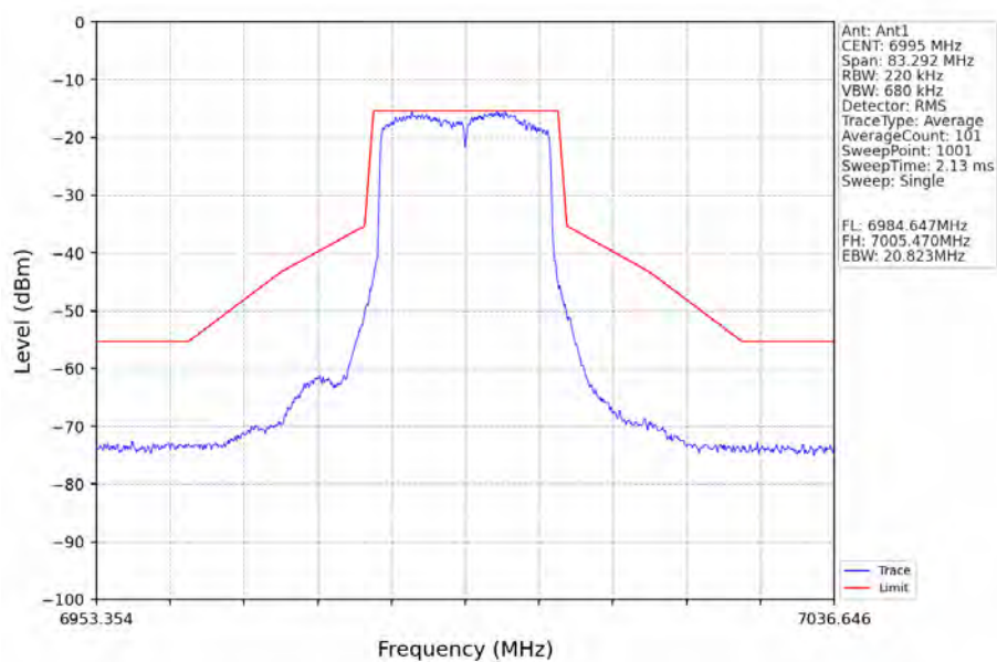
802.11ax(HEW20)_MCH_6995MHz_RU242_Left_Ant1_NTNV
