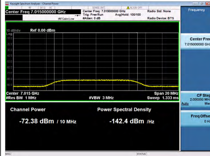
11AX20SISO-Ant 1-7015-Center-7015-Minimal
