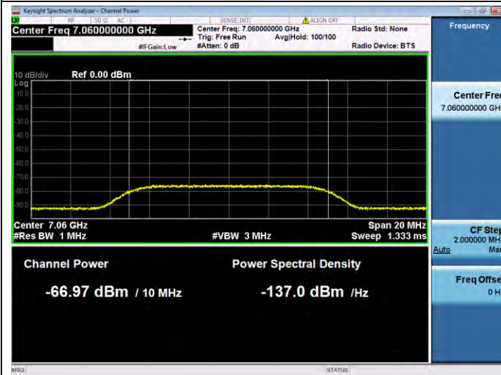
11AX160SISO-Ant 1-6985-Center-7060-Minimal
