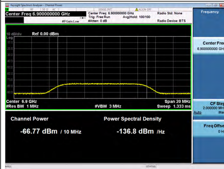
11AX160SISO-Ant 1-6825-Center-6900-Minimal
