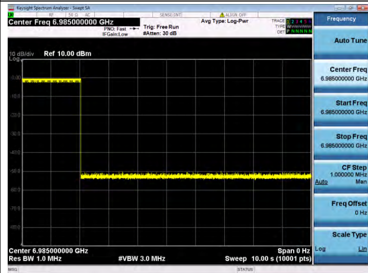
11AX160SISO-Ant 1-6985-Center-6985-Minimal
