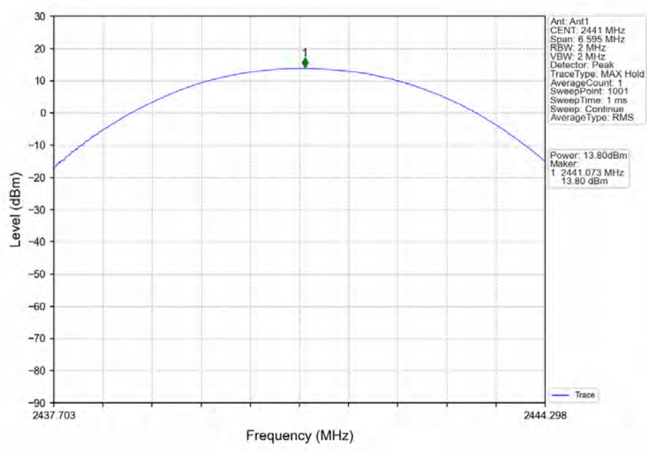
8DPSK_3DH5_MCH_2441MHz_Ant1_NTNV
