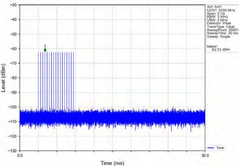
Signal Calibration_802.11ax(HEW160)_2A_5250MHz_RadarType3_Trial0
