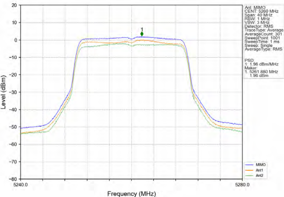
802.11ax(HEW20)_LCH_5260MHz_RU242_Left_MIMO_NTNV
