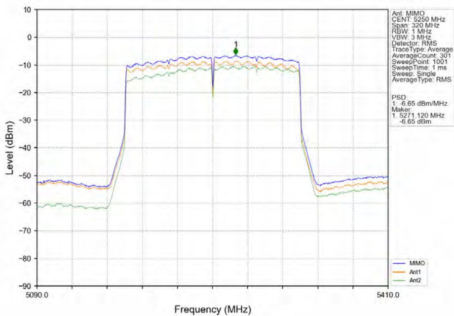
802.11ax(HEW160)_MCH_5250MHz_2xRU996_Left_MIMO_NTNV
