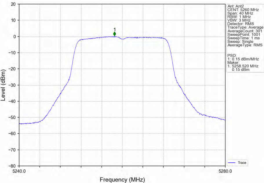
802.11ac(VHT20)_LCH_5260MHz_MIMO_NTNV
