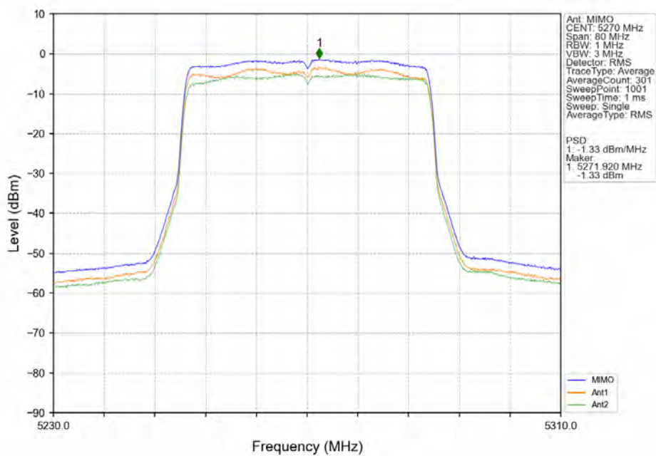
802.11ax(HEW40)_LCH_5270MHz_RU484_Left_MIMO_NTNV
