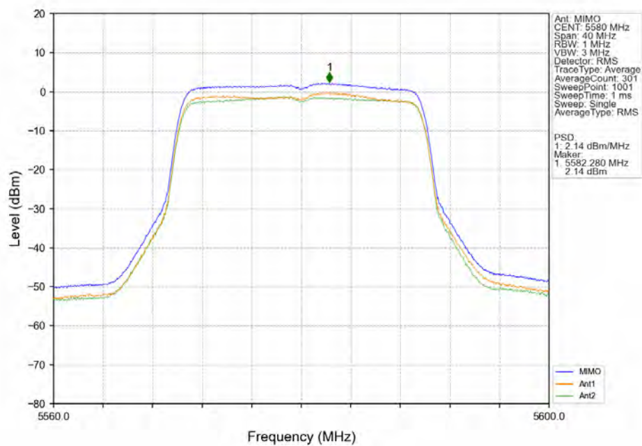
802.11ax(HEW20)_MCH_5580MHz_RU242_Left_MIMO_NTNV
