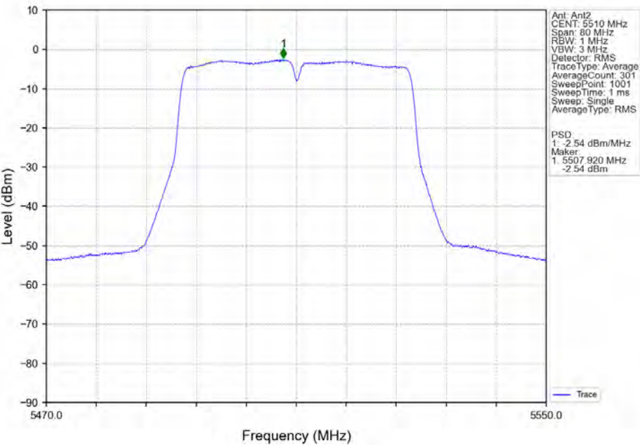
802.11n(HT40)_LCH_5510MHz_MIMO_NTNV
