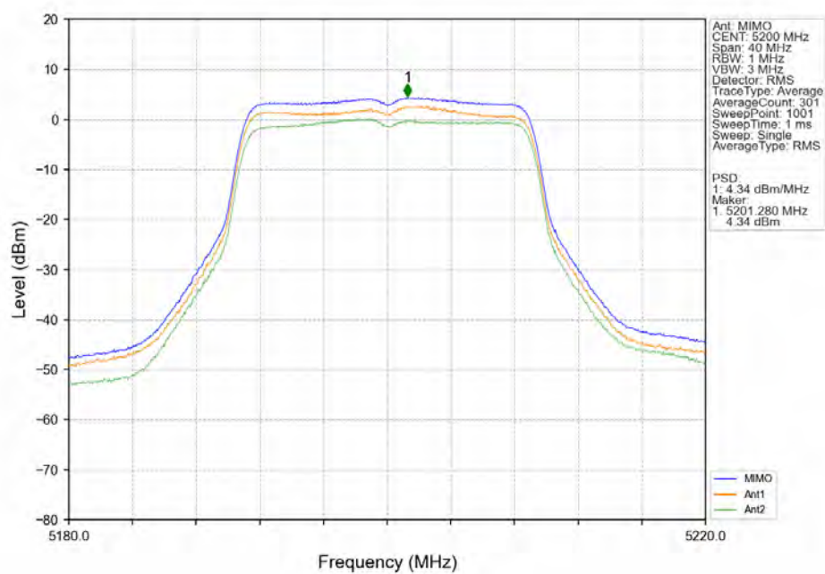
802.11ac(VHT20)_MCH_5200MHz_MIMO_NTNV
