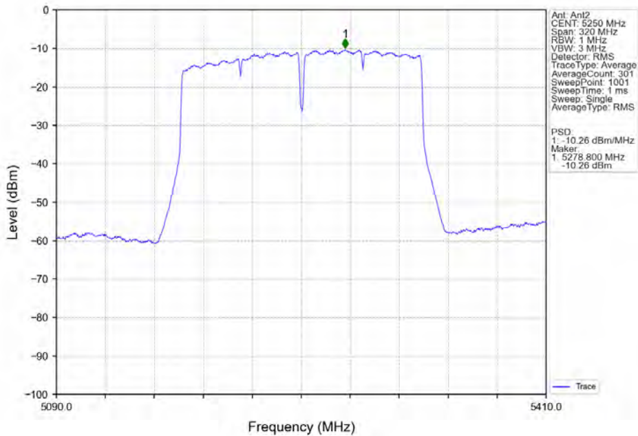
802.11ac(VHT160)_MCH_5250MHz_MIMO_NTNV
