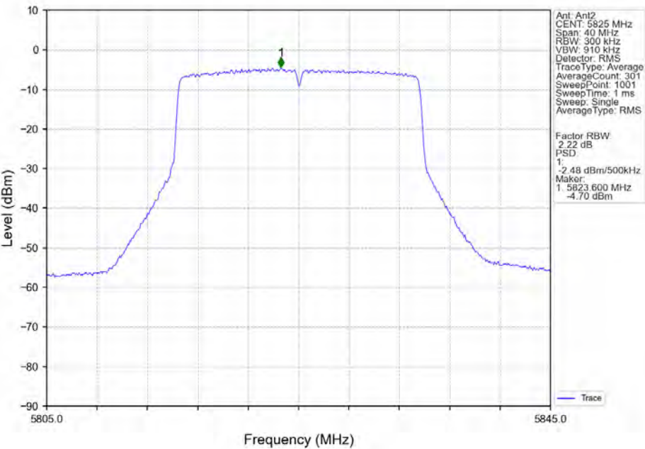
802.11ax(HEW20)_HCH_5825MHz_RU242_Left_MIMO_NTNV
