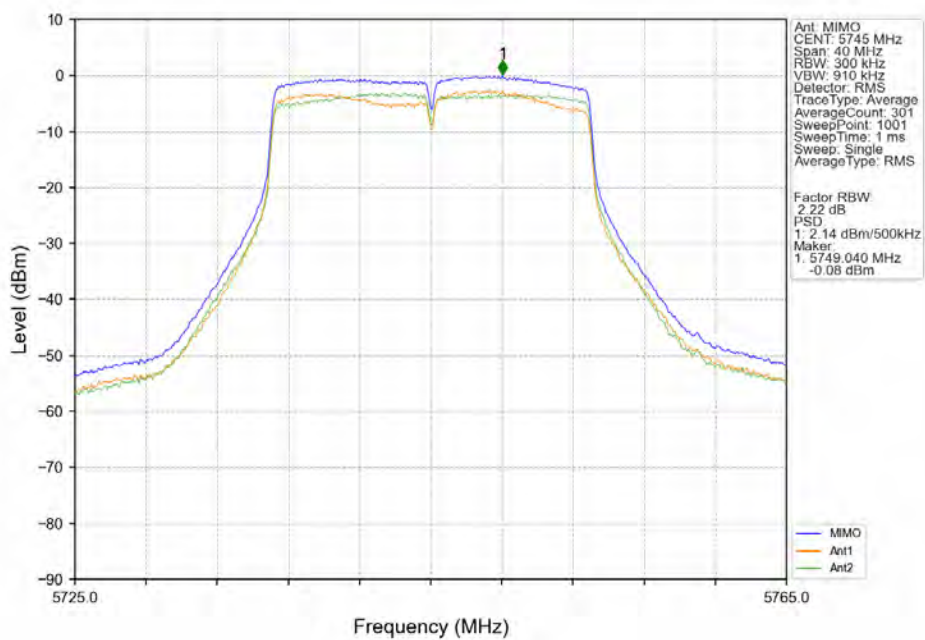
802.11ac(VHT20)_LCH_5745MHz_MIMO_NTNV
