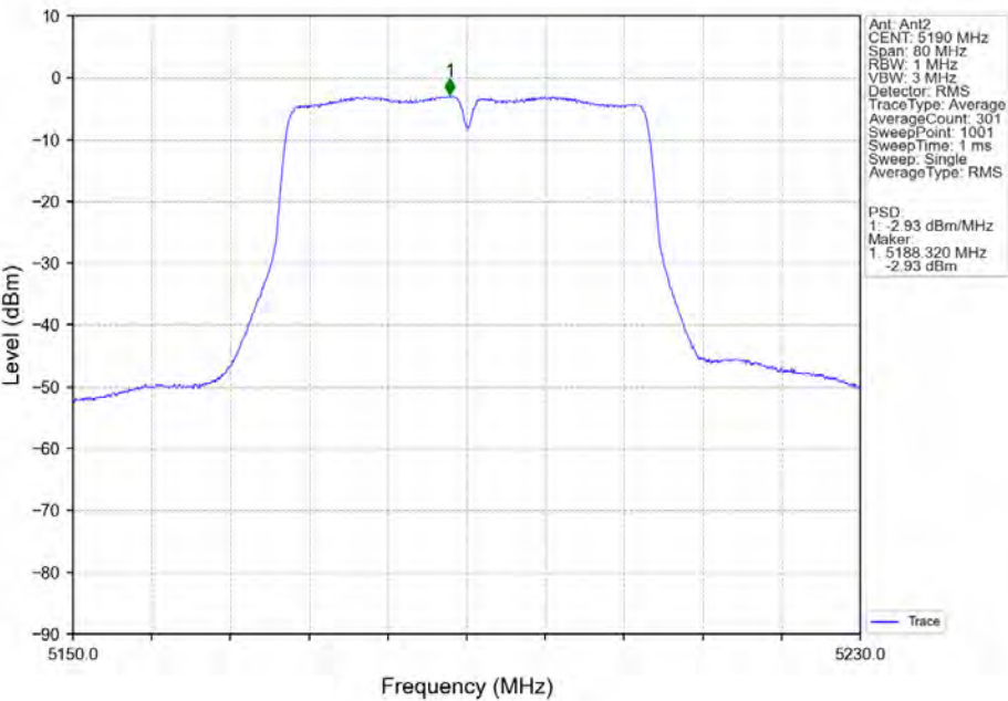
802.11ac(VHT40)_LCH_5190MHz_MIMO_NTNV
