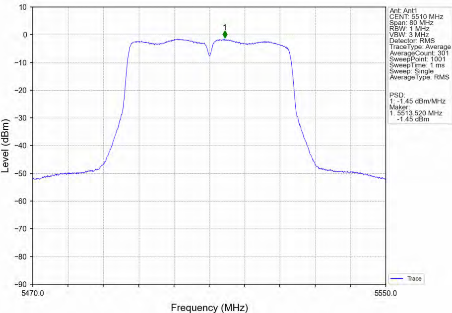
802.11ac(VHT40)_LCH_5510MHz_Ant1_NTNV
