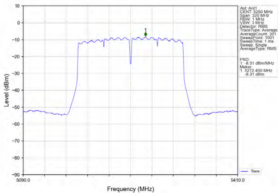
802.11ac(VHT160)_MCH_5250MHz_Ant1_NTNV
