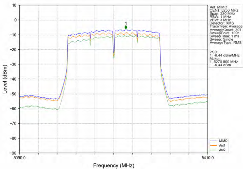
802.11ac(VHT160)_MCH_5250MHz_MIMO_NTNV
