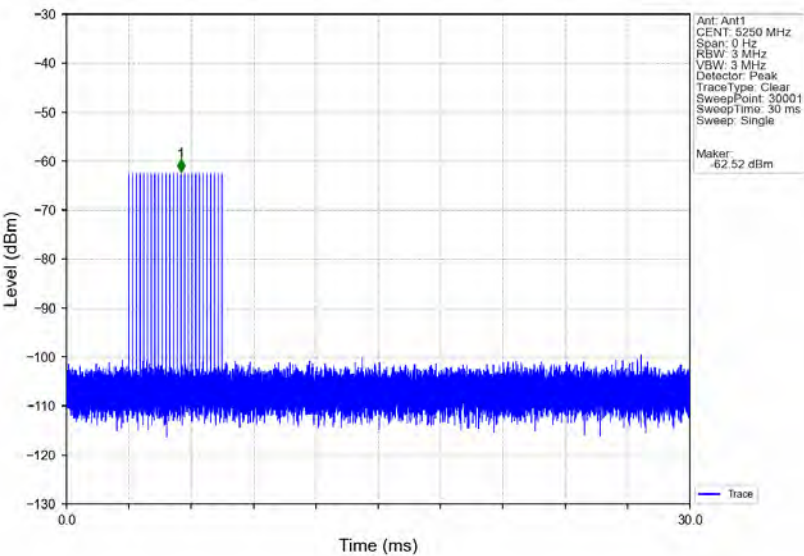
Signal Calibration_802.11ax(HEW160)_2A_5250MHz_RadarType3_Trial0
