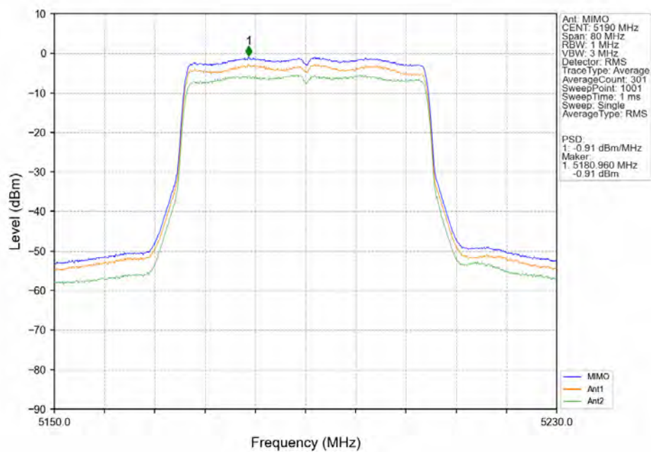
802.11ax(HEW40)_LCH_5190MHz_RU484_Left_MIMO_NTNV
