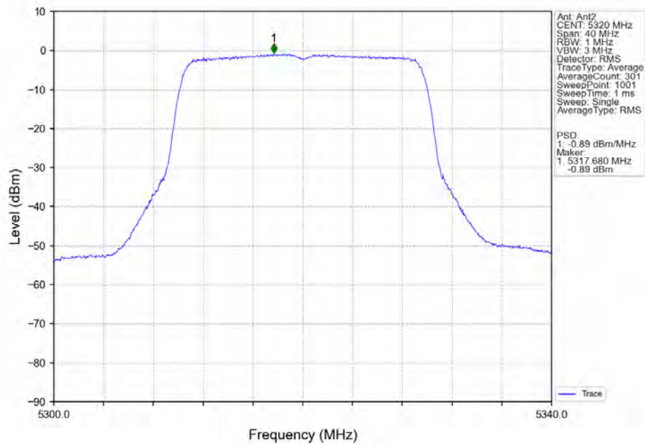
802.11ax(HEW20)_HCH_5320MHz_RU242_Left_MIMO_NTNV
