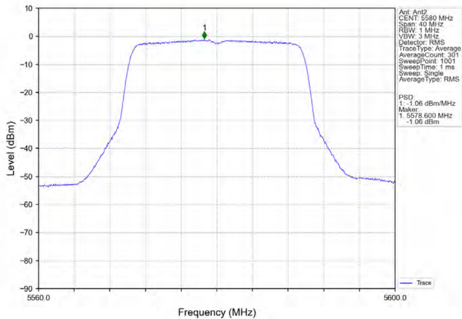
802.11ax(HEW20)_MCH_5580MHz_RU242_Left_MIMO_NTNV
