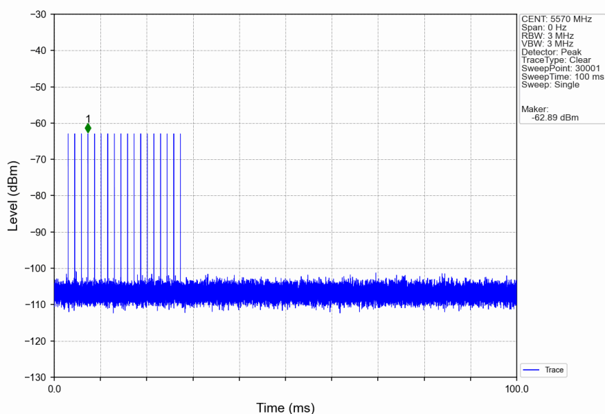
Signal Calibration_802.11ax(HEW160)_2C_5570MHz_RadarType1_Trial0
