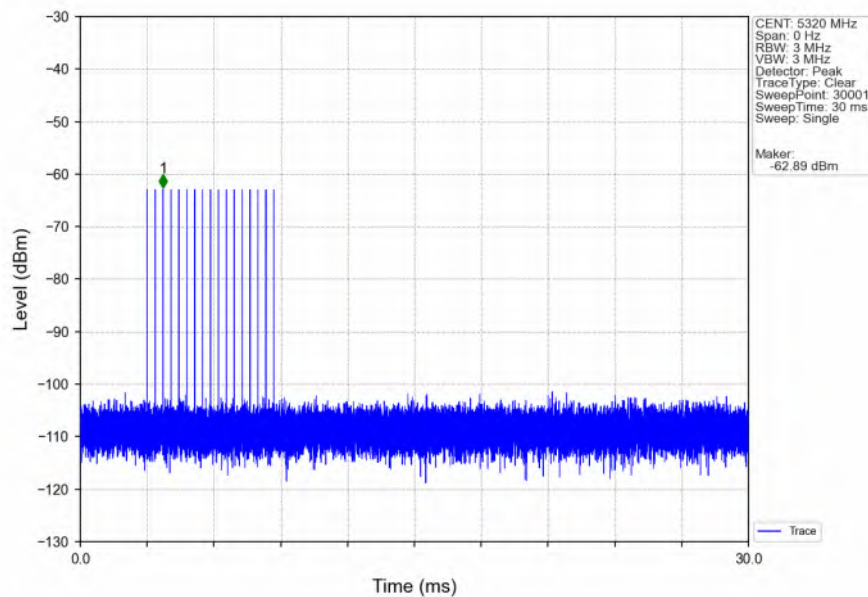
Signal Calibration_802.11ax(HEW20)_2A_5320MHz_RadarType3_Trial0
