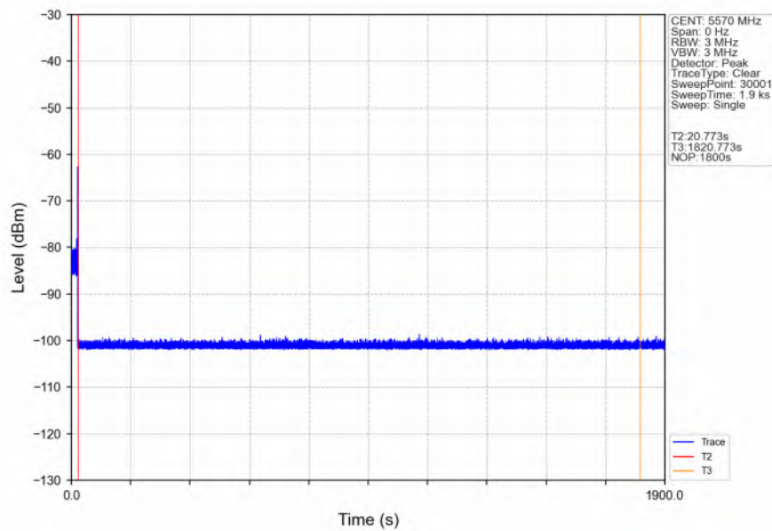
Non-Occupancy Period_802.11ax(HEW160)_2C_5570MHz
