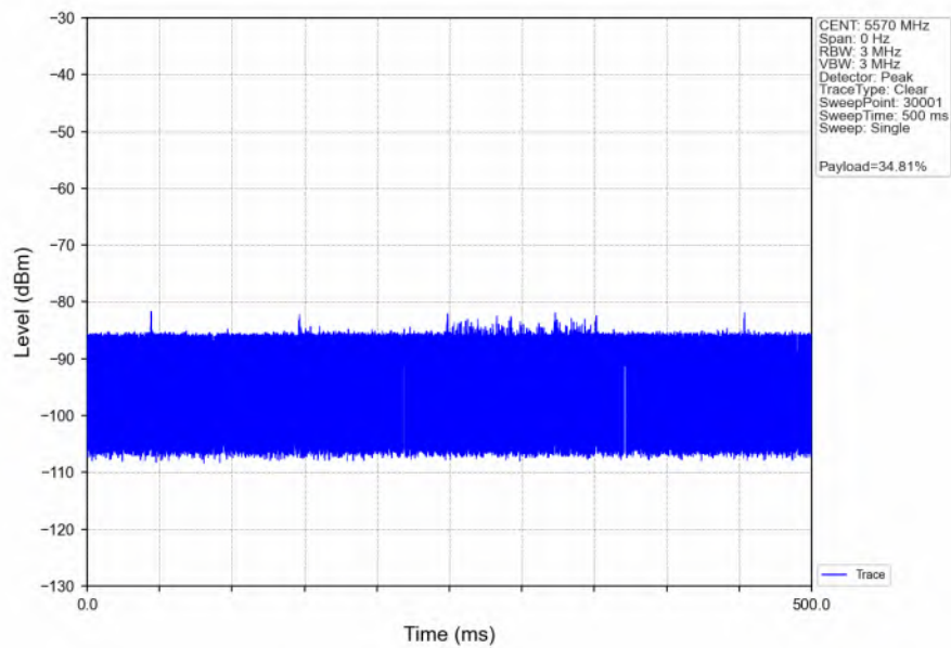
Channel Loading (Payload)_802.11ax(HEW160)_2C_5570MHz
