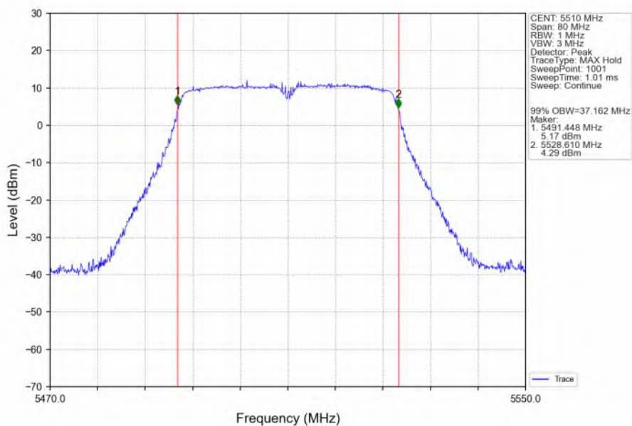
802.11ac(VHT40)_LCH_5510MHz_Ant6_NTNV
