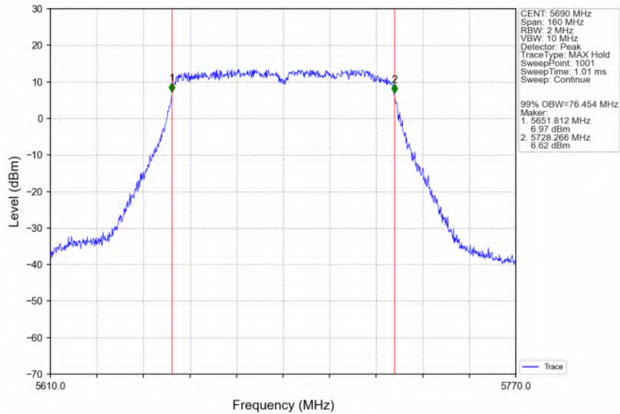
802.11ac(VHT80)_HCH_5690MHz_Ant6_NTNV
