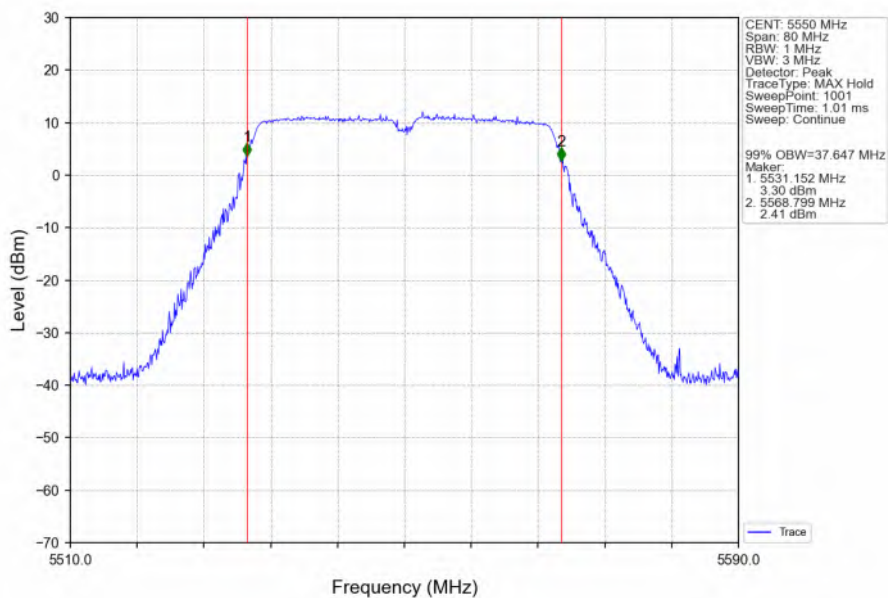
802.11ac(VHT40)_MCH_5550MHz_Ant6_NTNV
