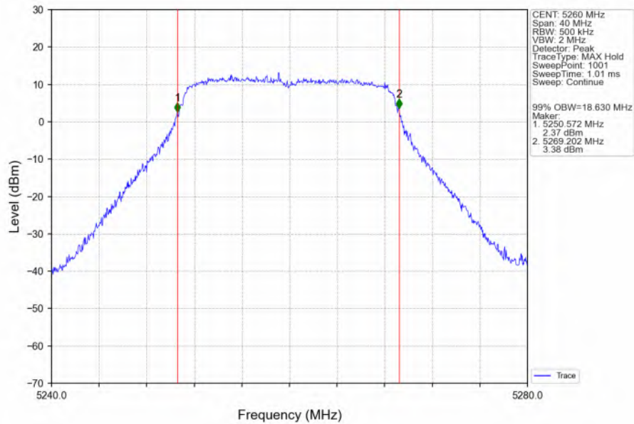
802.11ac(VHT20)_LCH_5260MHz_Ant6_NTNV
