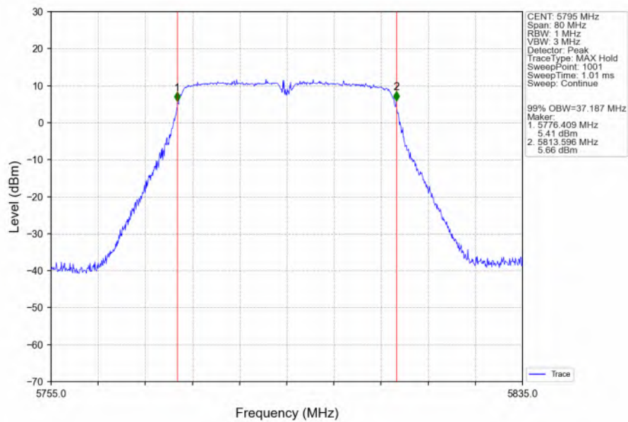
802.11ac(VHT40)_HCH_5795MHz_Ant6_NTNV
