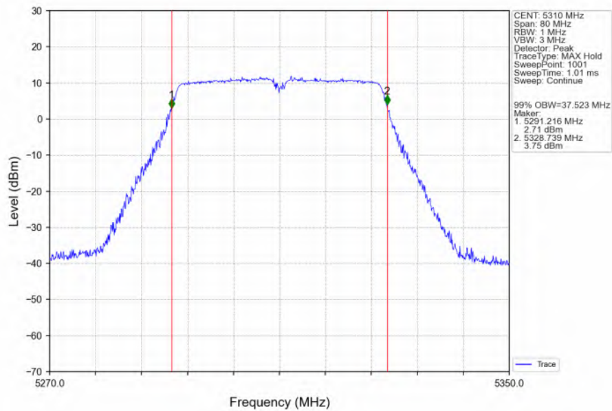
802.11ac(VHT40)_HCH_5310MHz_Ant6_NTNV
