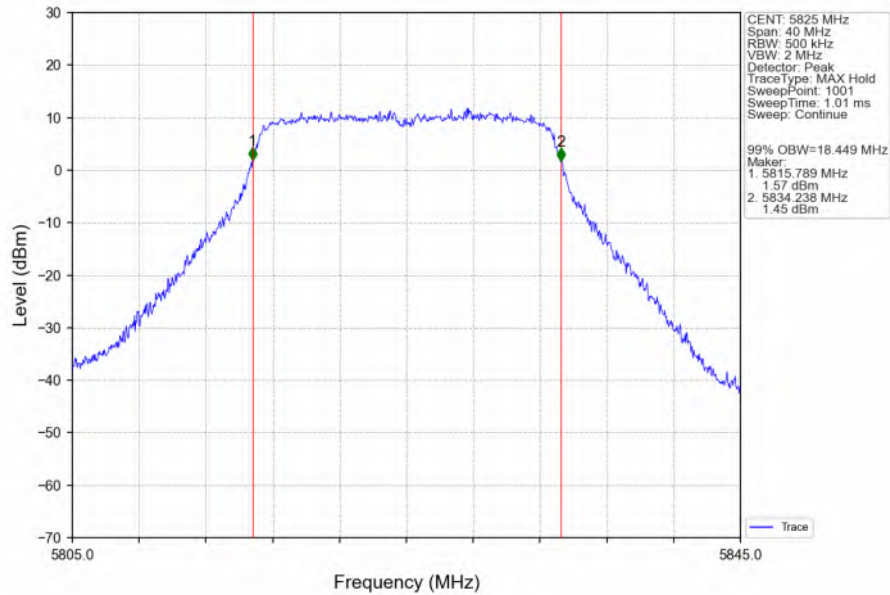
802.11ac(VHT20)_HCH_5825MHz_Ant6_NTNV
