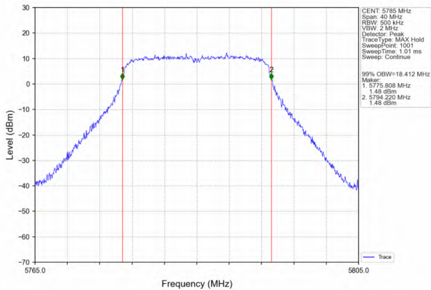
802.11ac(VHT20)_MCH_5785MHz_Ant6_NTNV
