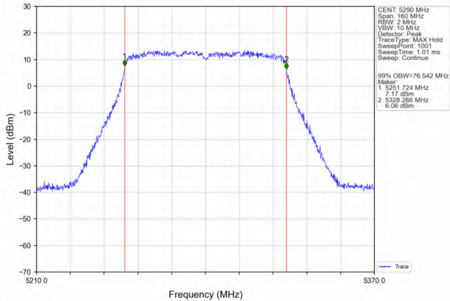
802.11ac(VHT80)_MCH_5290MHz_Ant6_NTNV
