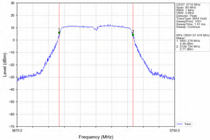
802.11ac(VHT40)_HCH_5710MHz_Ant6_NTNV
