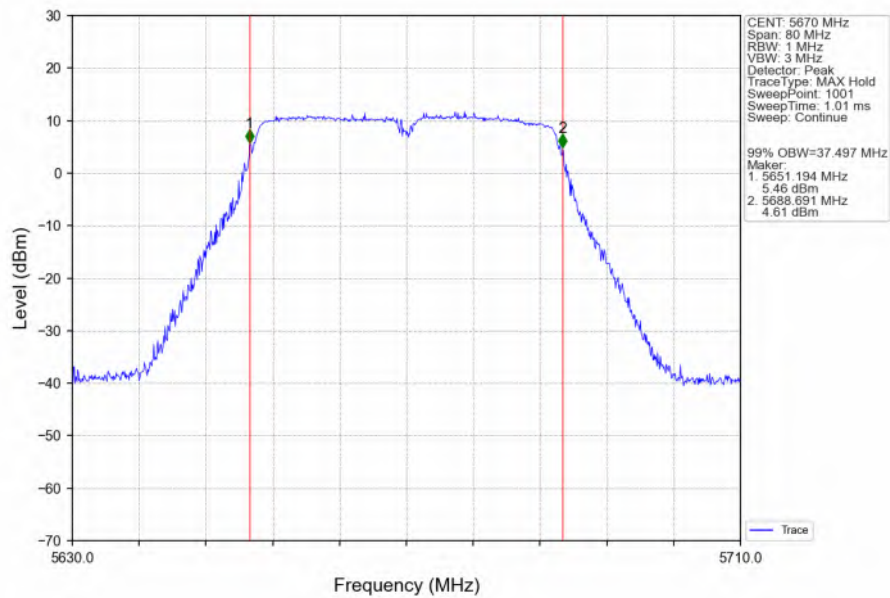
802.11ac(VHT40)_HCH_5670MHz_Ant6_NTNV
