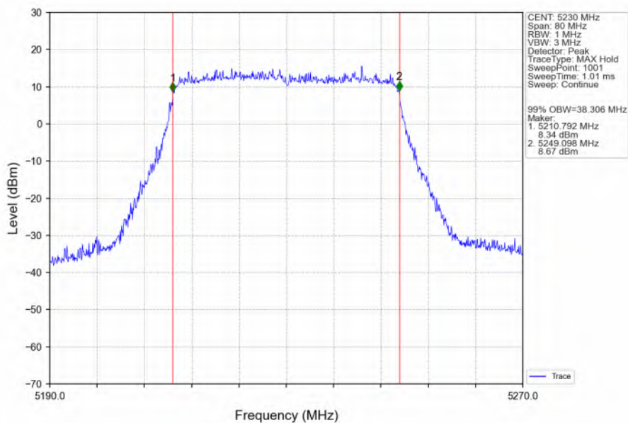
802.11ax(HEW40)_HCH_5230MHz_SU_ / _Ant6_NTNV
