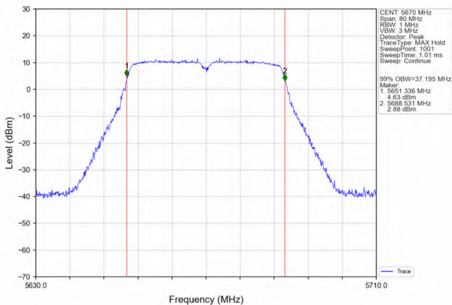
802.11n(HT40)_HCH_5670MHz_Ant6_NTNV
