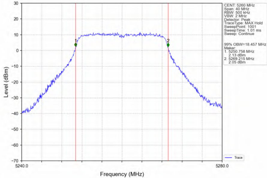
802.11ac(VHT20)_LCH_5260MHz_Ant6_NTNV
