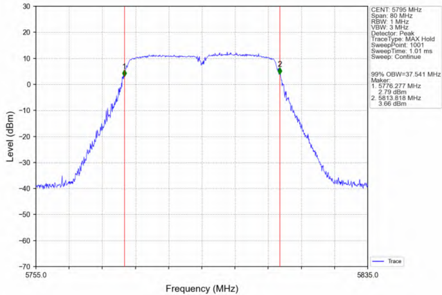
802.11ac(VHT40)_HCH_5795MHz_Ant6_NTNV
