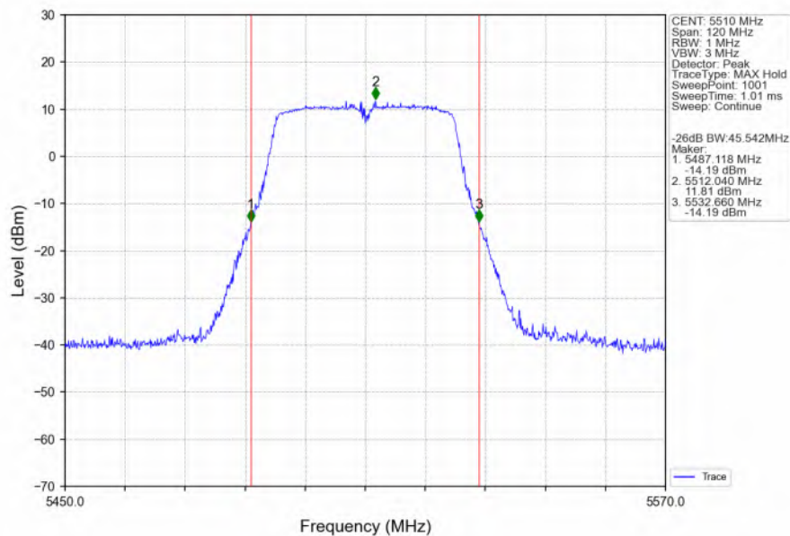
802.11ac(VHT40)_LCH_5510MHz_Ant6_NTNV
