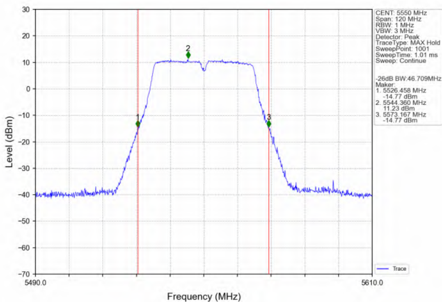
802.11n(HT40)_MCH_5550MHz_Ant6_NTNV
