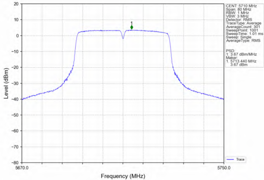
802.11ac(VHT40)_HCH_5710MHz_MIMO_NTNV
