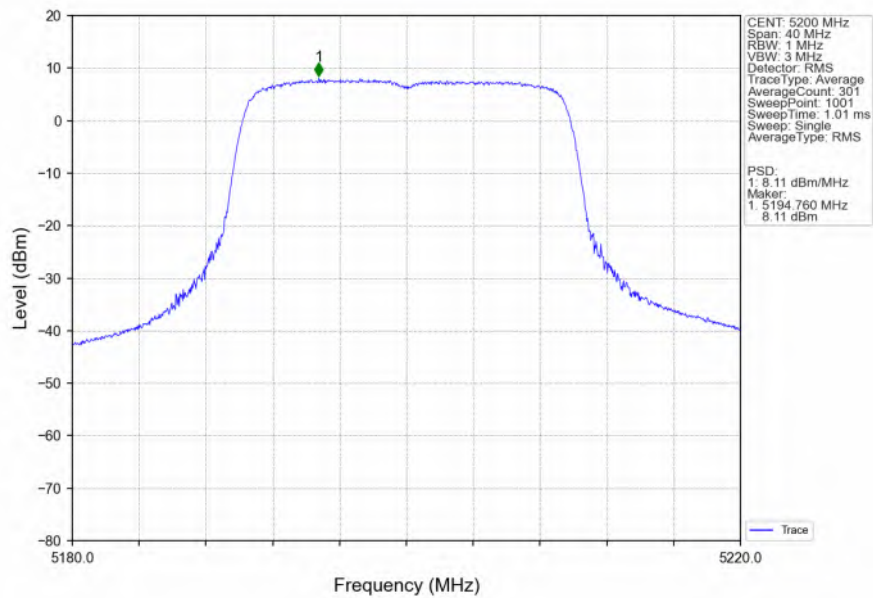
802.11ax(HEW20)_MCH_5200MHz_SU_/_Ant6_NTNV
