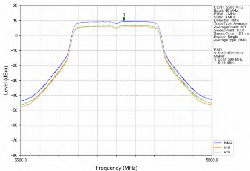
802.11ac(VHT20)_MCH_5580MHz_MIMO_NTNV
