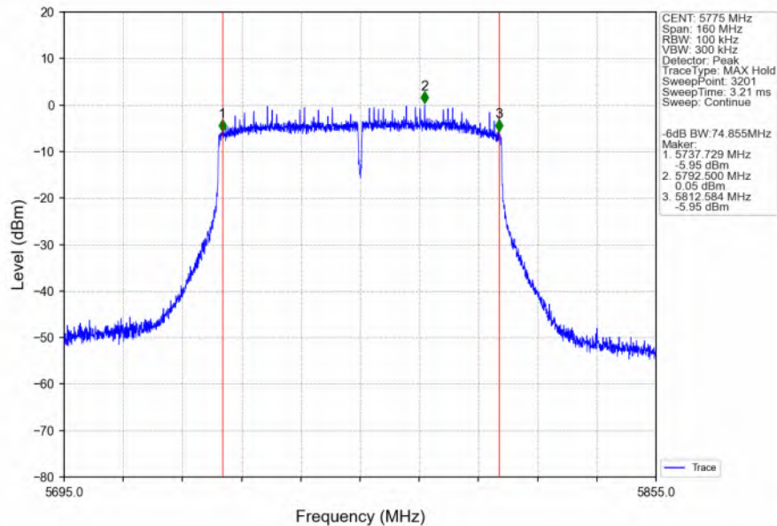
802.11ac(VHT80)_MCH_5775MHz_Ant6_NTNV
