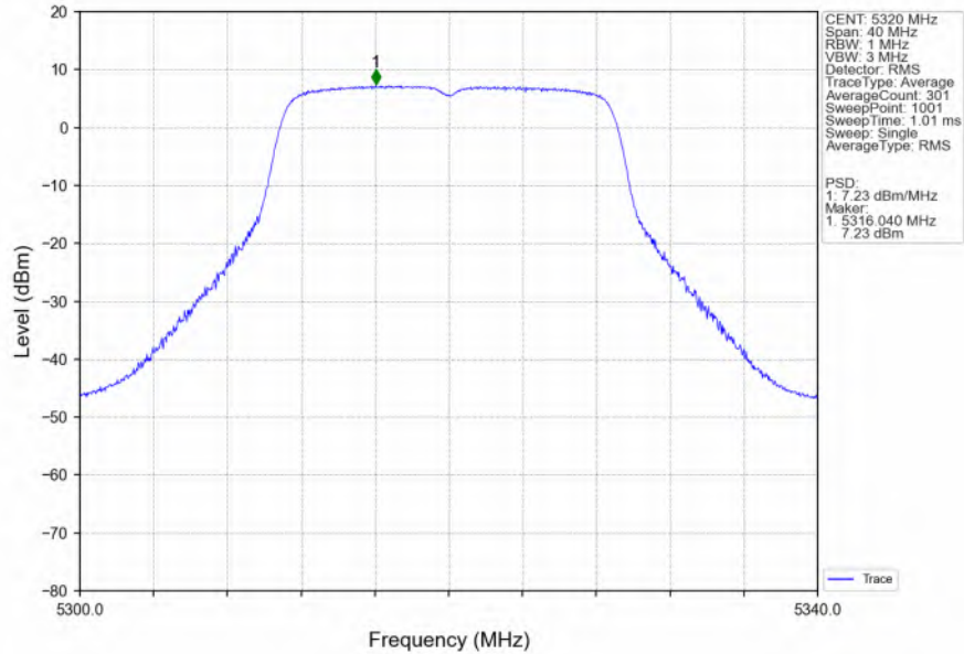
802.11ac(VHT20)_HCH_5320MHz_MIMO_NTNV
