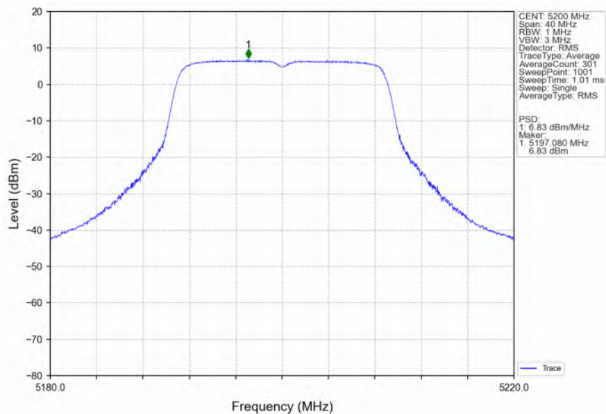
802.11n(HT20)_MCH_5200MHz_Ant5_NTNV
