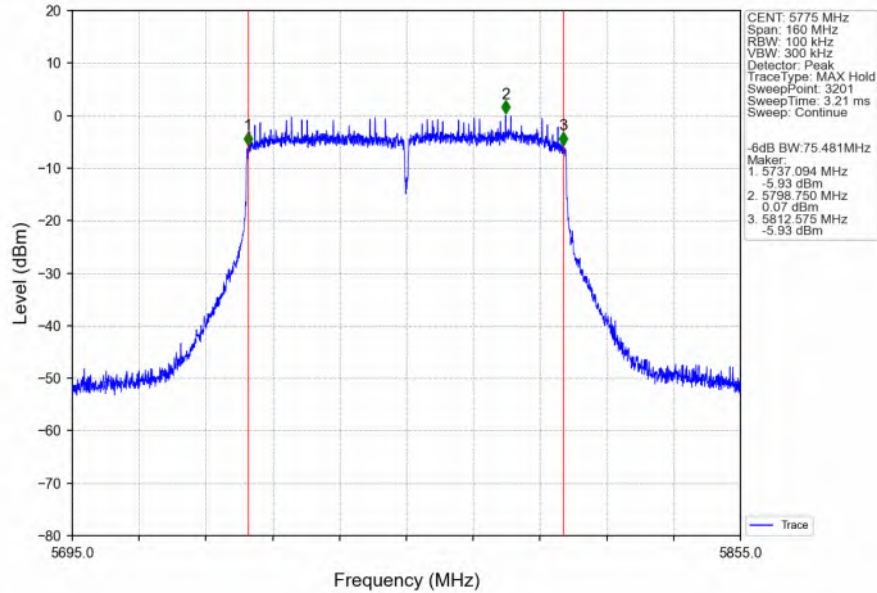
802.11ac(VHT80)_MCH_5775MHz_Ant6_NTNV
