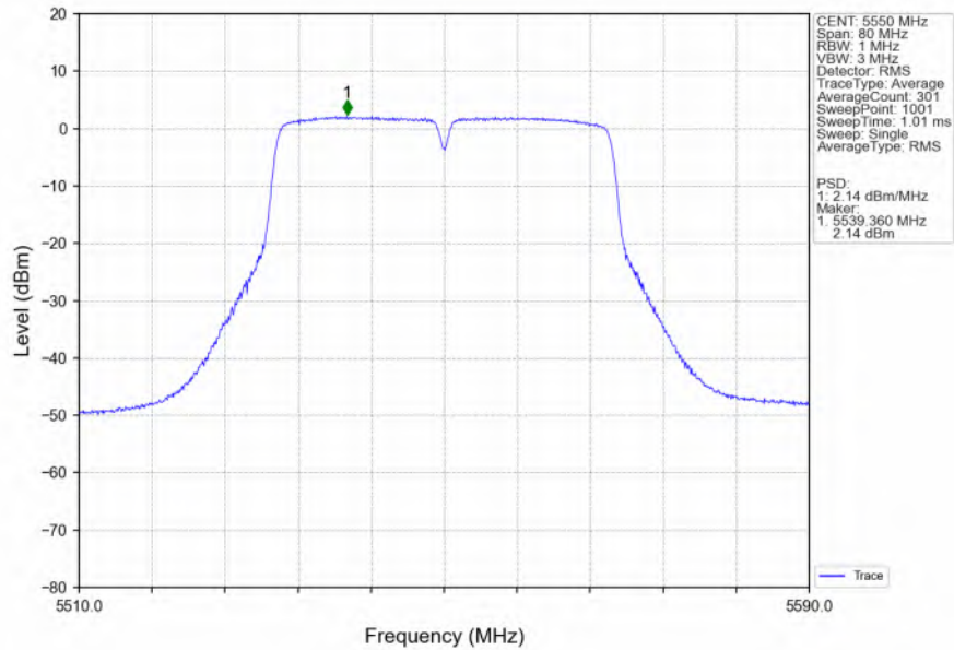
802.11ac(VHT40)_MCH_5550MHz_MIMO_NTNV
