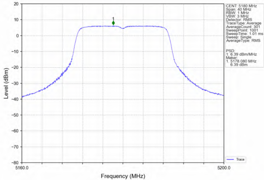
802.11ac(VHT20)_LCH_5180MHz_Ant6_NTNV
