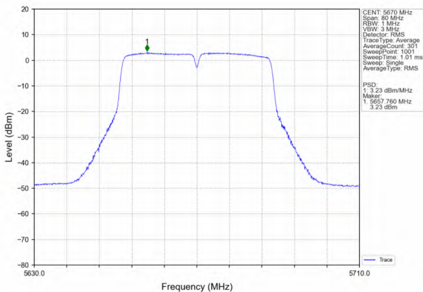
802.11n(HT40)_HCH_5670MHz_Ant6_NTNV
