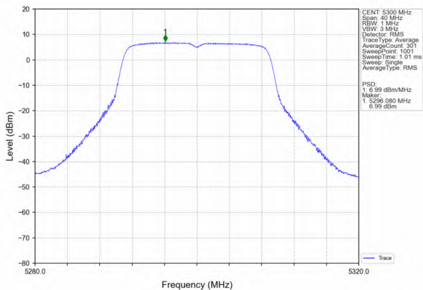
802.11ac(VHT20)_MCH_5300MHz_Ant6_NTNV
