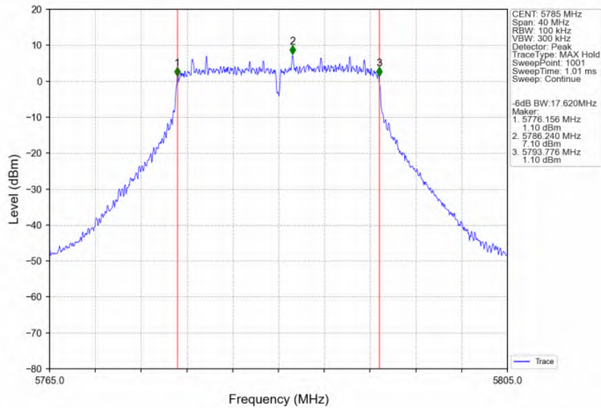
802.11n(HT20)_MCH_5785MHz_Ant6_NTNV
