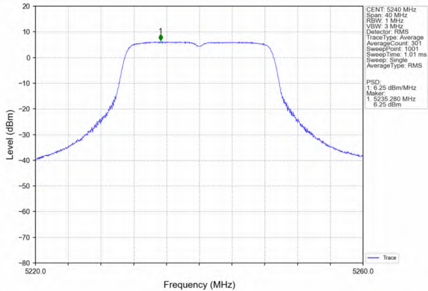
802.11ac(VHT20)_HCH_5240MHz_Ant6_NTNV
