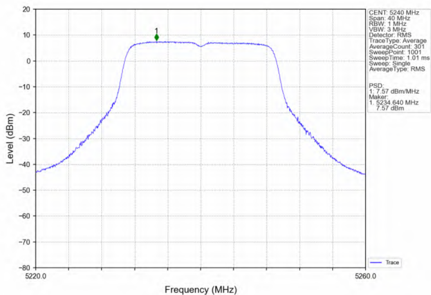
802.11n(HT20)_HCH_5240MHz_Ant6_NTNV
