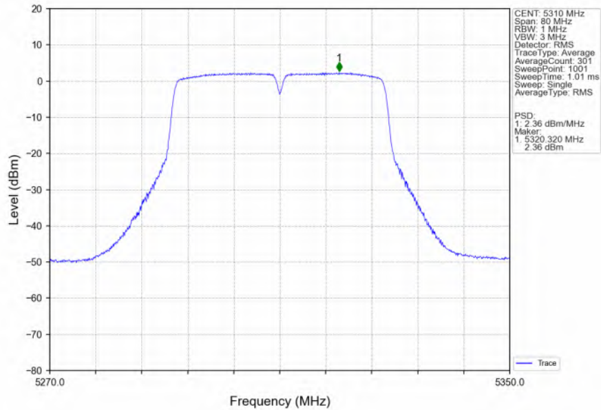
802.11ac(VHT40)_HCH_5310MHz_MIMO_NTNV
