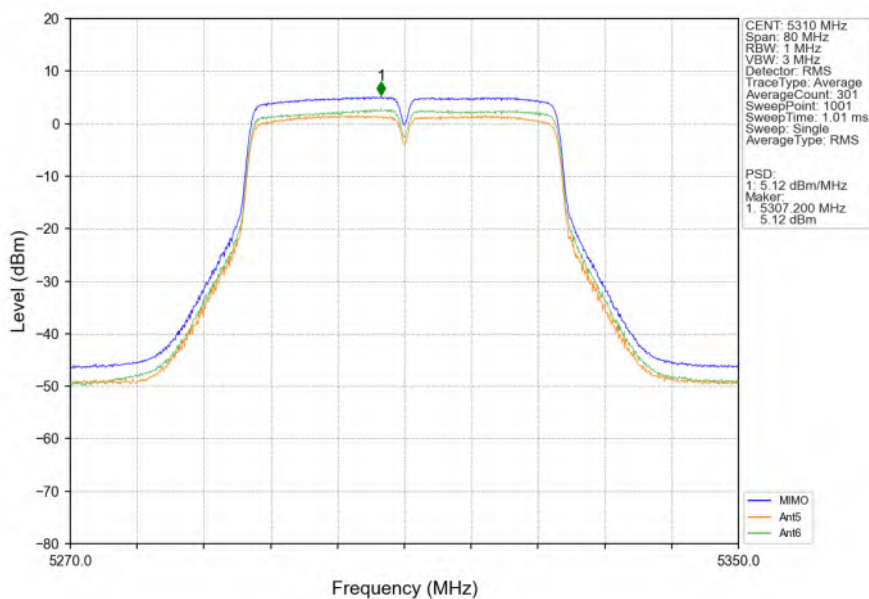
802.11n(HT40)_HCH_5310MHz_MIMO_NTNV
