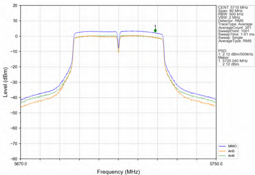
802.11ac(VHT40)_HCH_5710MHz_MIMO_NTNV
