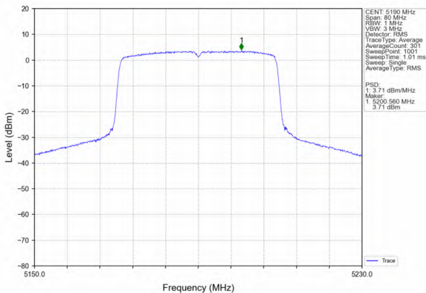
802.11ax(HEW40)_LCH_5190MHz_SU_/_MIMO_NTNV
