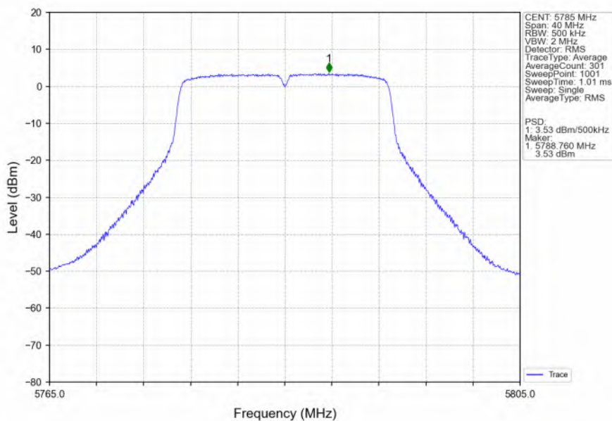
802.11ac(VHT20)_MCH_5785MHz_Ant6_NTNV
