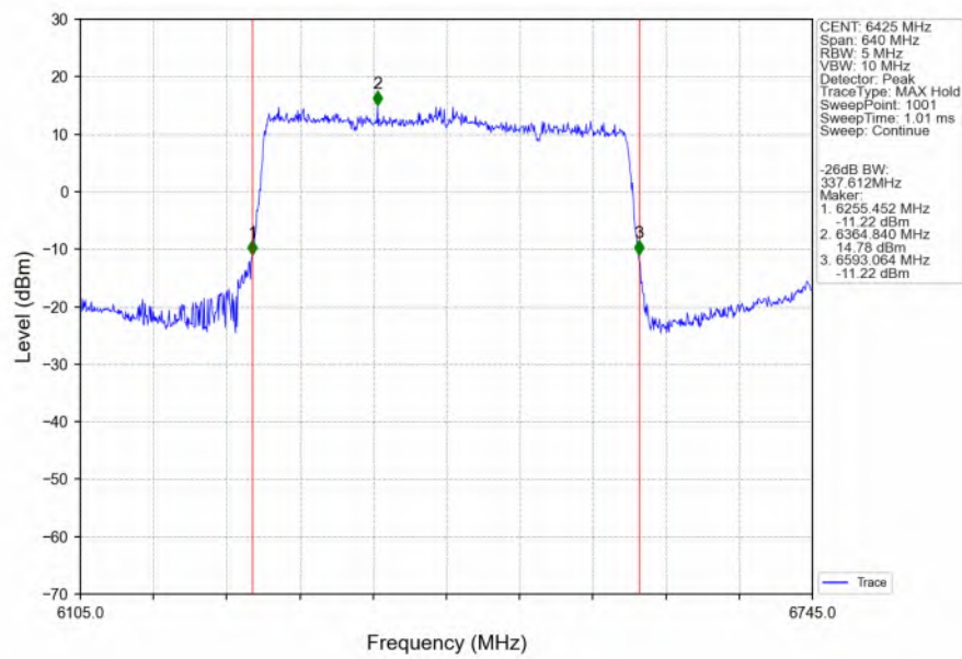
802.11be(EHT320)_MCH_6425MHz_SU_/_Ant1_NTNV
