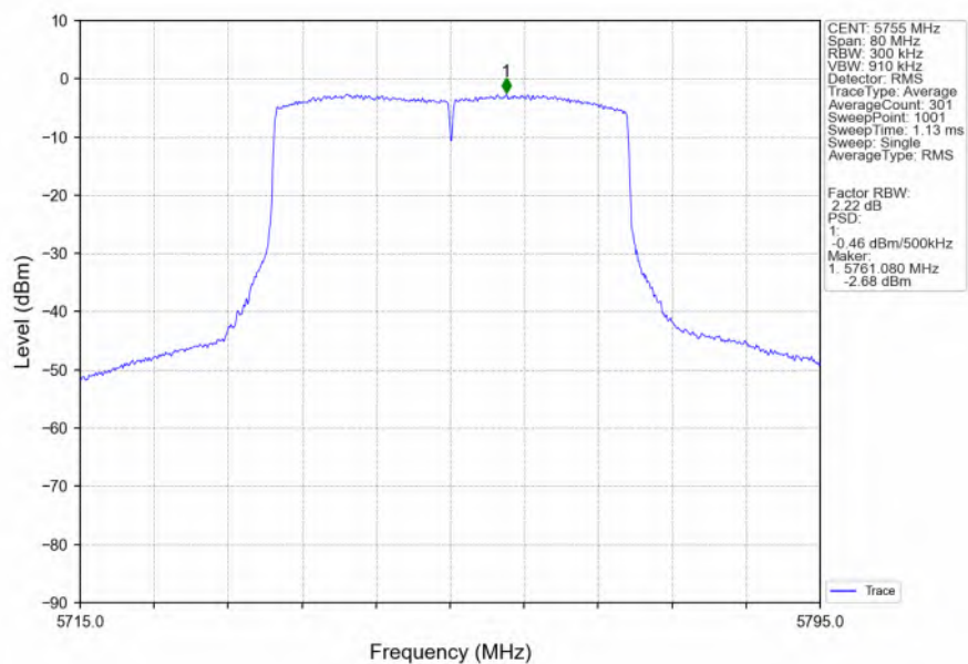
802.11ax(HEW40)_LCH_5755MHz_SU_ / _Ant6_NTNV
