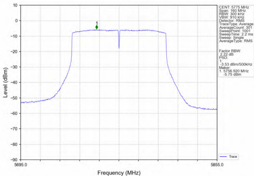
802.11ac(VHT80)_MCH_5775MHz_Ant6_NTNV
