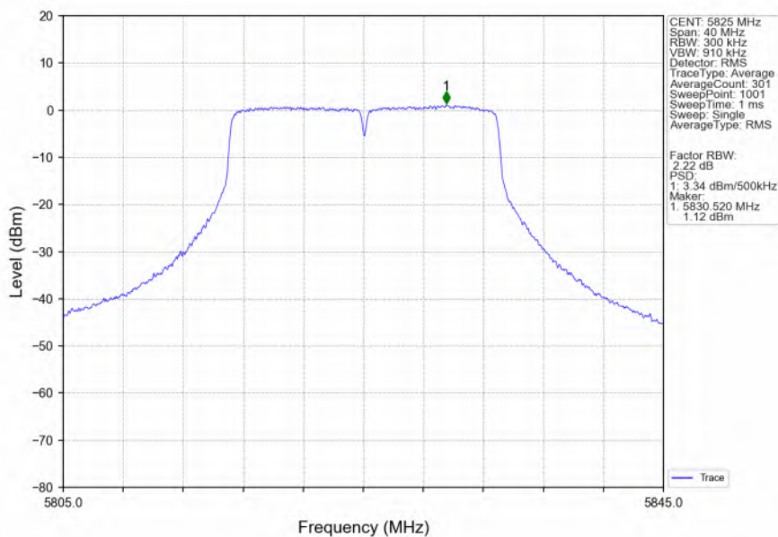
802.11ac(VHT20)_HCH_5825MHz_MIMO_NTNV
