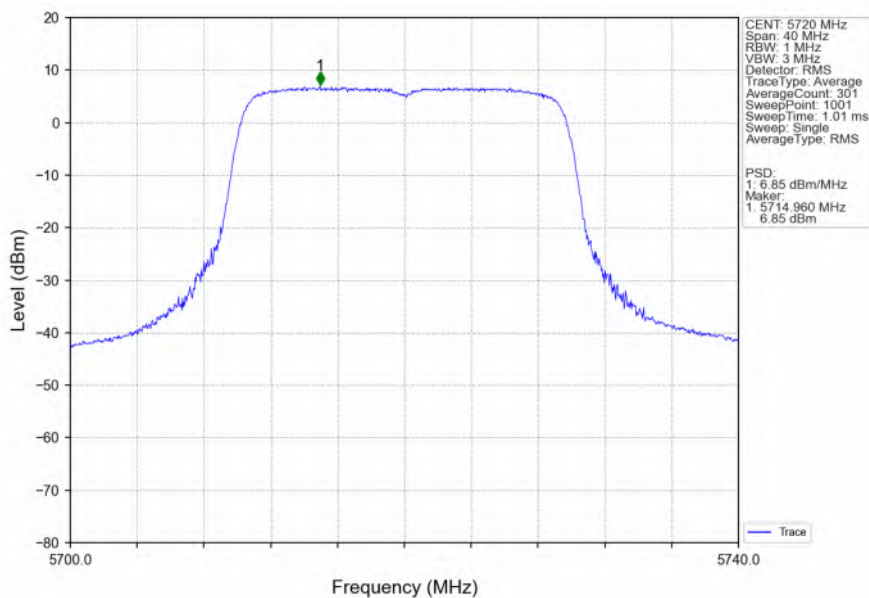
802.11ax(HEW20)_HCH_5720MHz_SU_/_MIMO_NTNV
