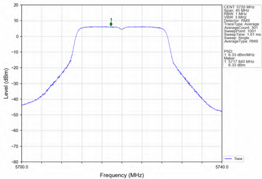
802.11ac(VHT20)_HCH_5720MHz_MIMO_NTNV
