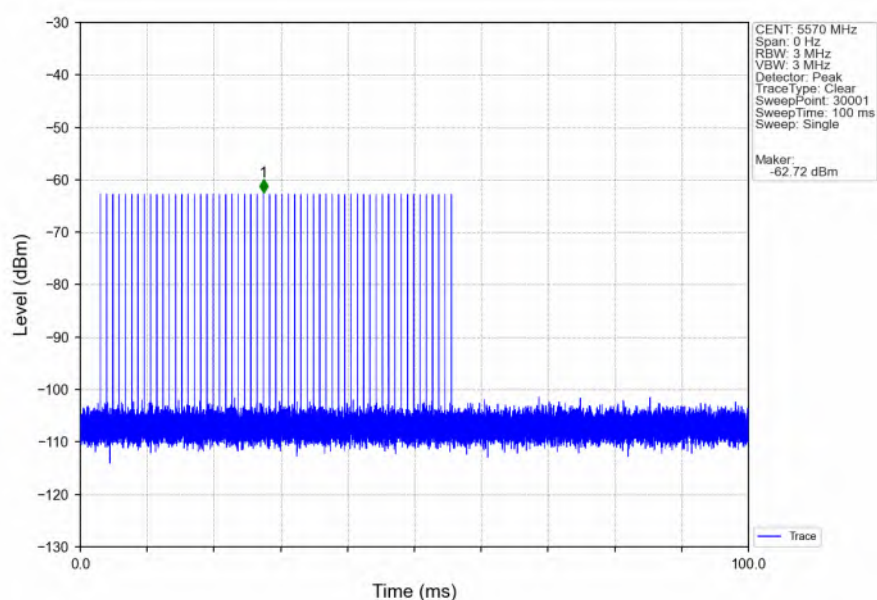
Signal Calibration_802.11be(EHT160)_2C_5570MHz_RadarType1_Trial0
