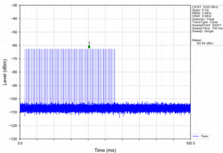
Signal Calibration_802.11be(EHT20)_2A_5320MHz_RadarType1_Trial0
