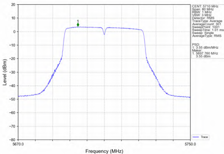
802.11ac(VHT40)_HCH_5710MHz_MIMO_NTNV
