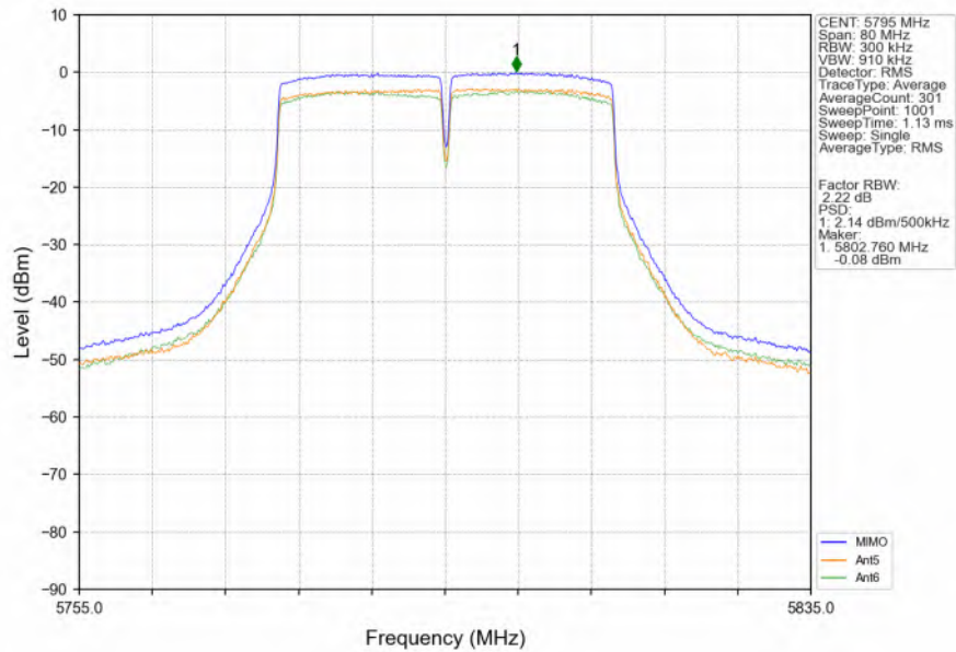
802.11ac(VHT40)_HCH_5795MHz_MIMO_NTNV
