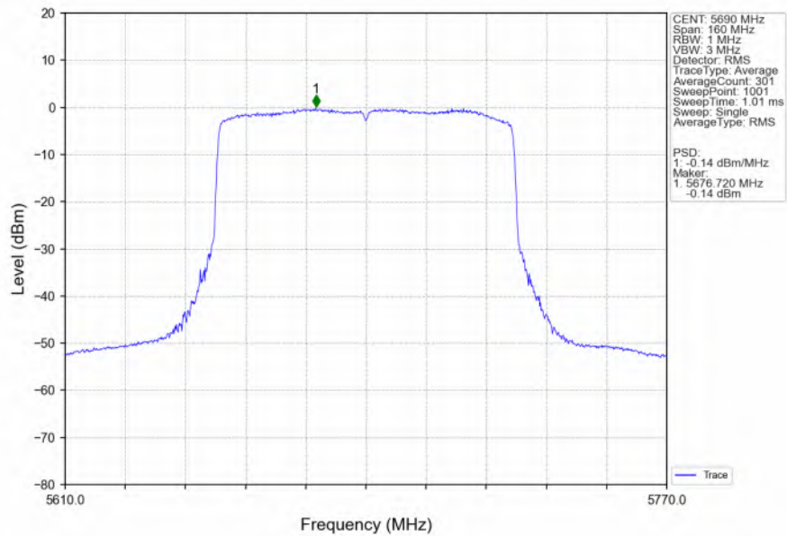
802.11ax(HEW80)_HCH_5690MHz_SU_ / _Ant6_NTNV
