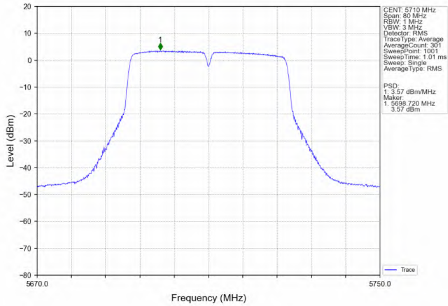
802.11n(HT40)_HCH_5710MHz_MIMO_NTNV
