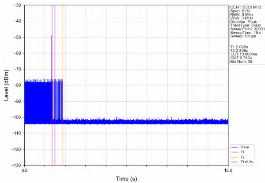
Channel Move Time and Closing Transmission Time_802.11be(EHT20)_2A_5320MHz
