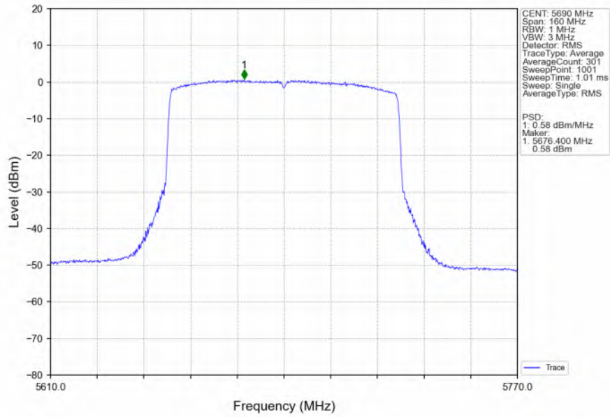
802.11ax(HEW80)_HCH_5690MHz_SU_/_MIMO_NTNV
