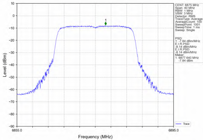
802.11ax(HEW20)_HCH_6875MHz_SU / Ant2_NTNV
