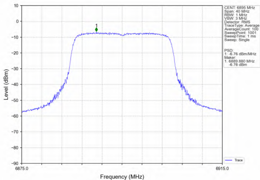
802.11ax(HEW20)_LCH_6895MHz_SU_ / Ant2_NTNV
