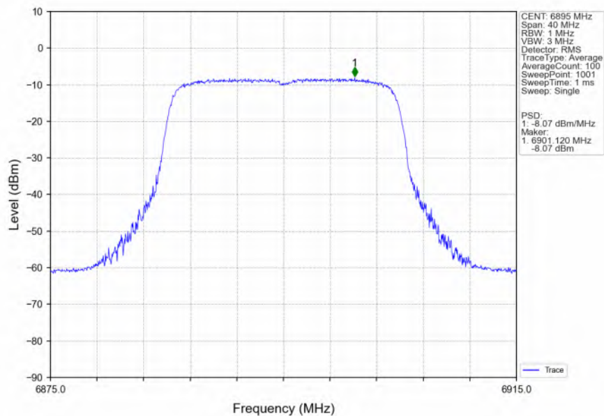
802.11ax(HEW20)_LCH_6895MHz_SU_ / Ant2_NTNV
