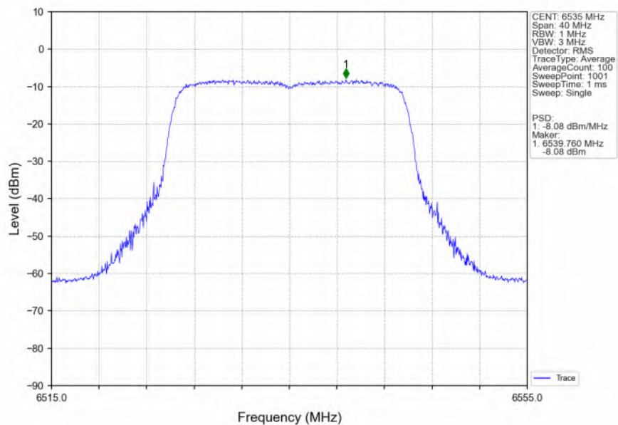
802.11ax(HEW20)_LCH_6535MHz_SU_ / Ant2_NTNV
