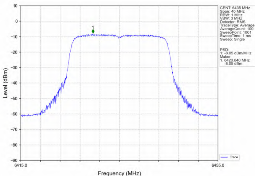
802.11ax(HEW20)_LCH_6435MHz_SU_ / Ant2_NTNV
