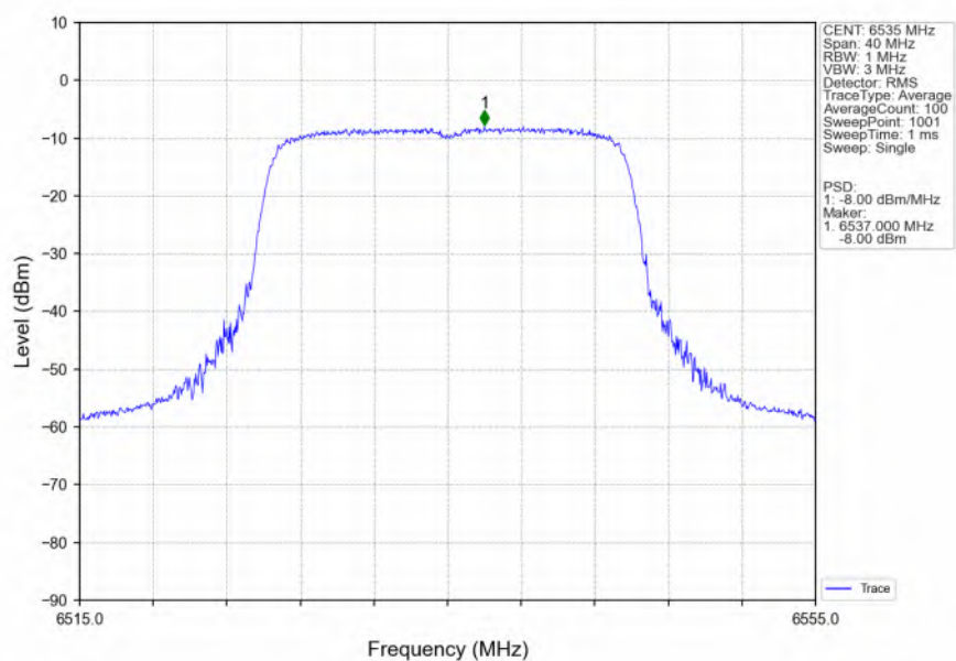
802.11ax(HEW20)_LCH_6535MHz_SU_ / Ant2_NTNV
