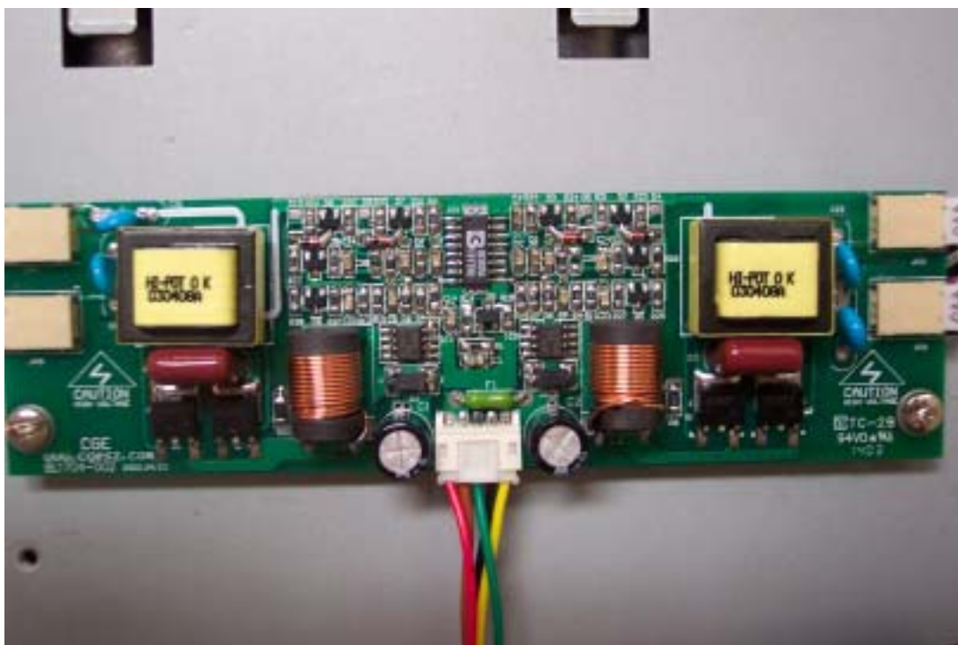
(Inverter)
