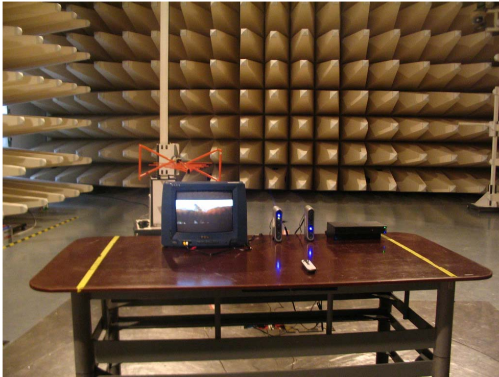
Radiated Emission:
