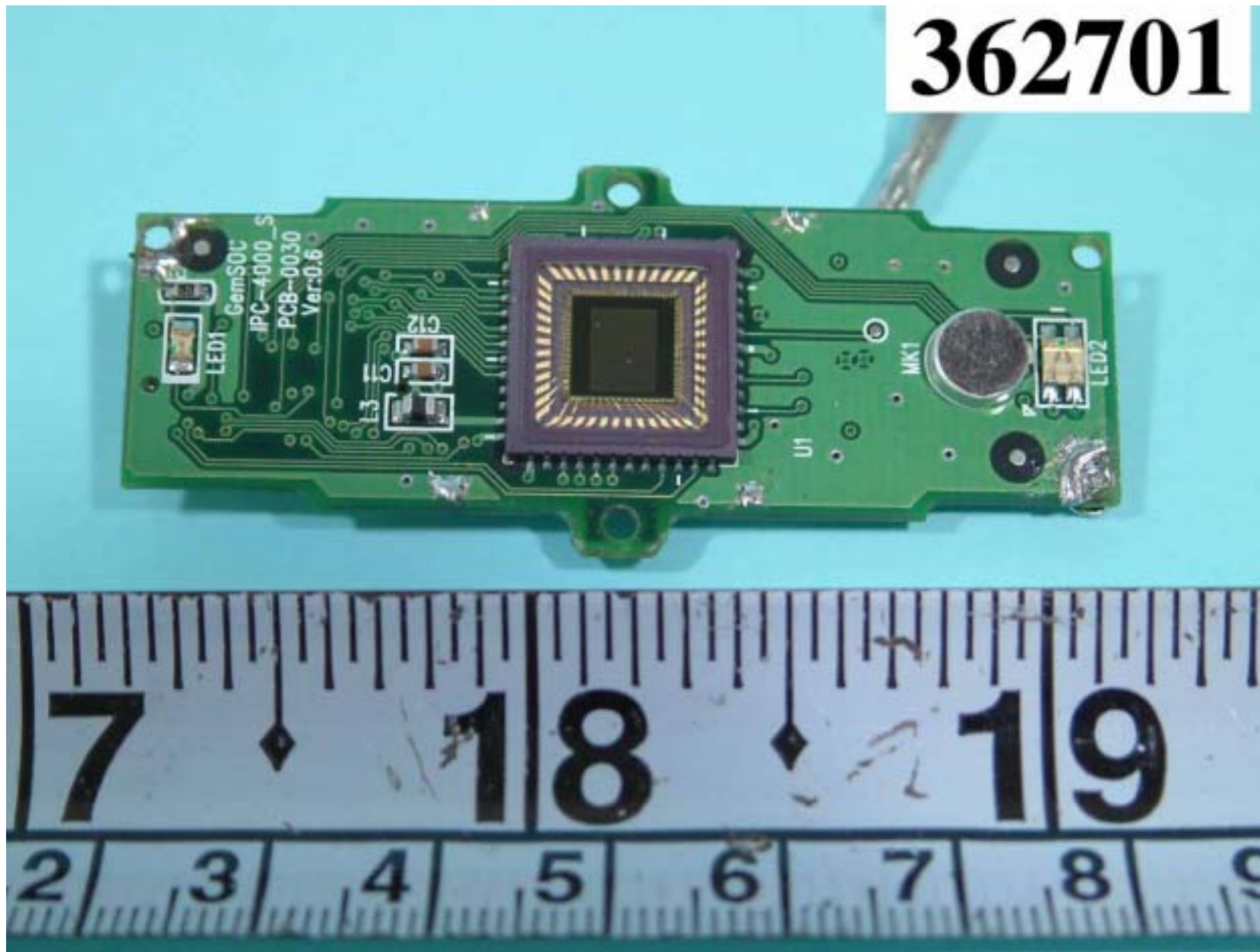
Front side of main board of camera
