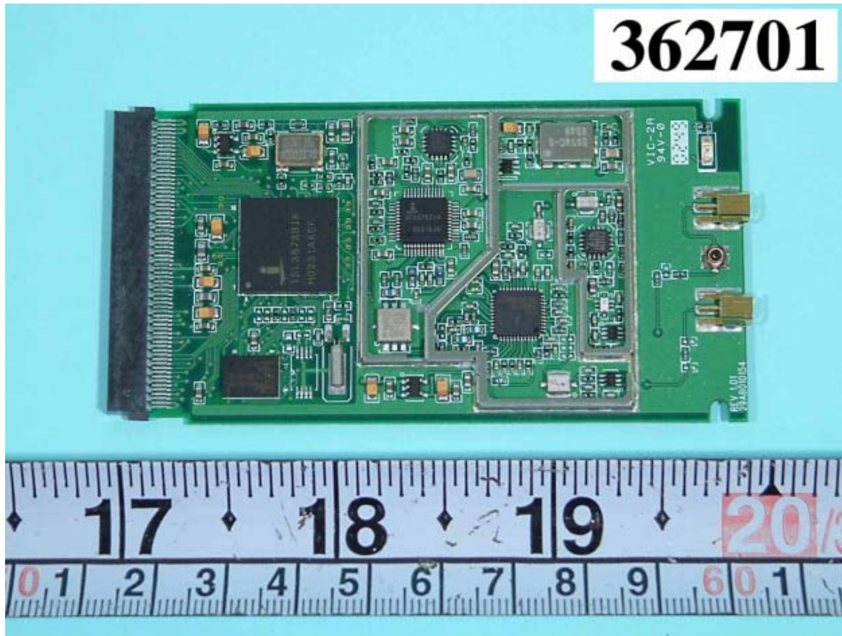
Front side of main board of RF module
