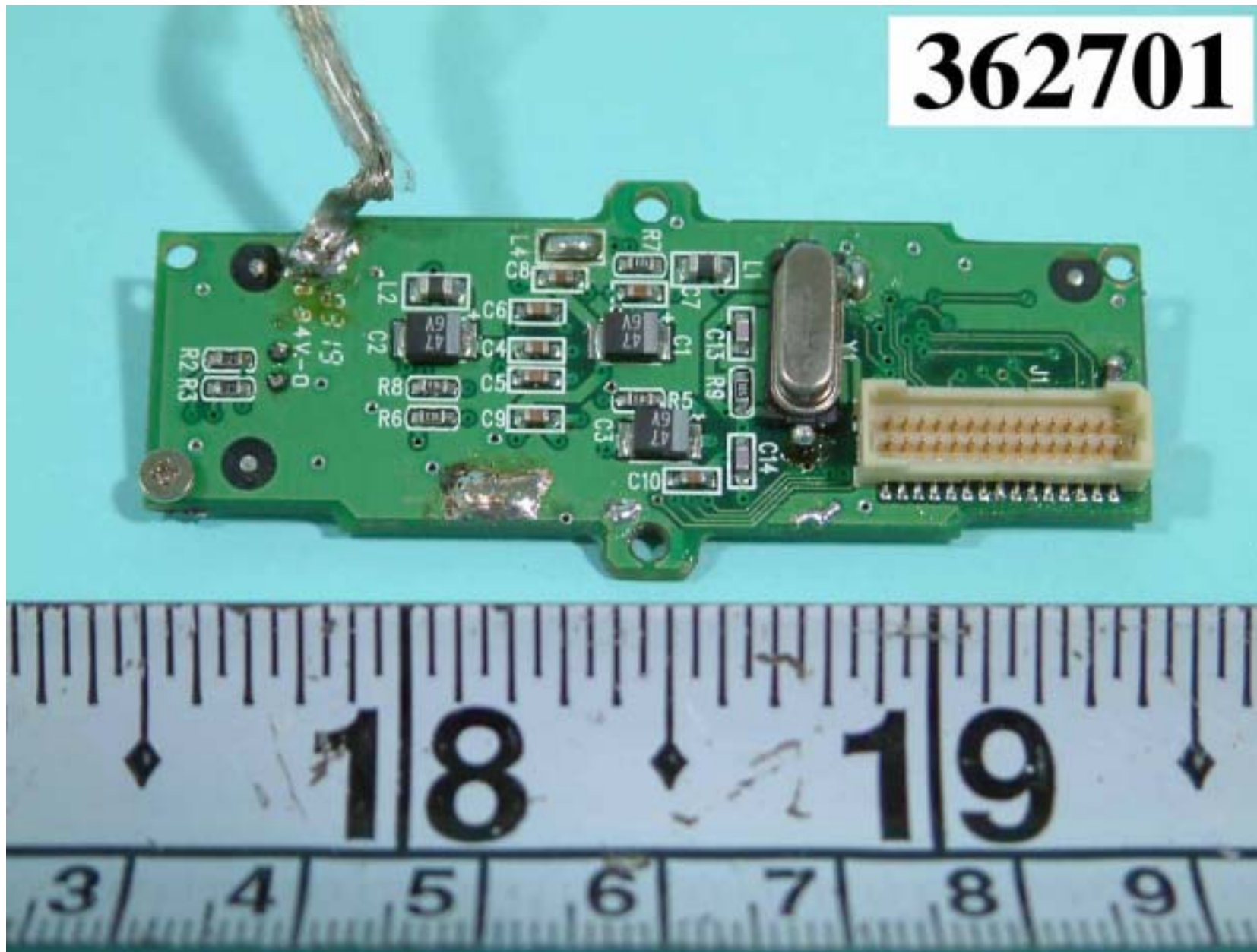
Rear side of main board of camera
