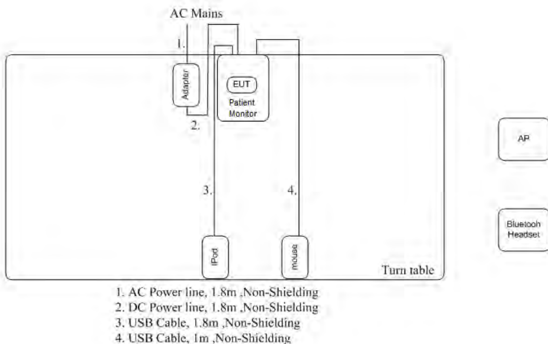
Test Setup Diagram –Radiated Test (below 1GHz)
