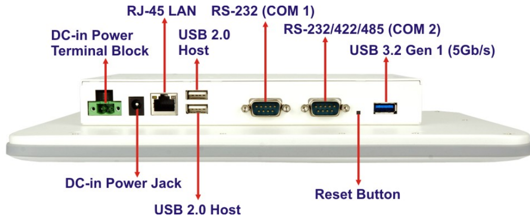
Figure 1-4: Bottom Panel
