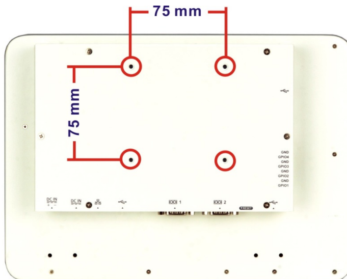
Figure 1-5: Rear Panel
