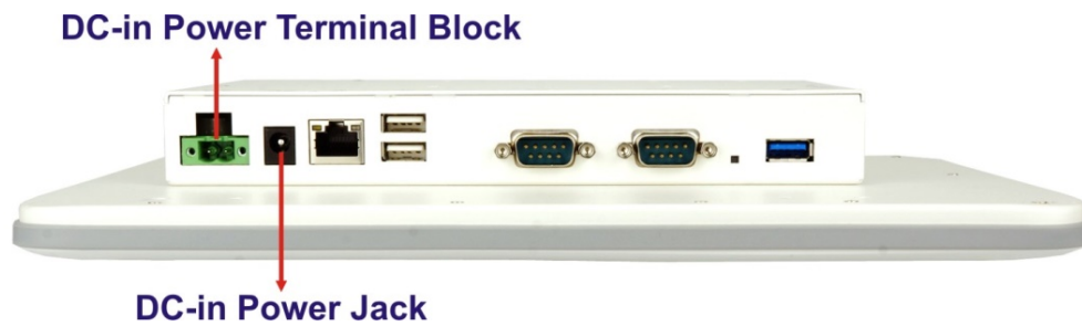
Figure 3-12: Power Connectors
