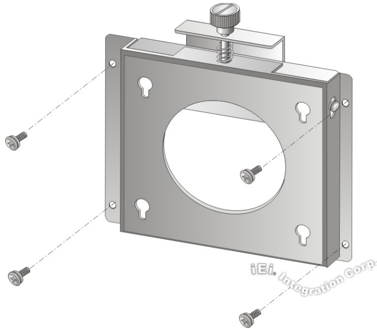
Figure 3-6: Wall-mounting Bracket
