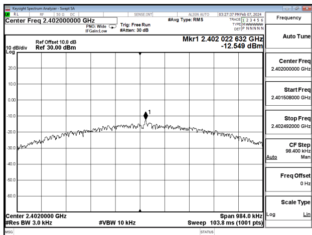
PSD_BLE 1M_MidCH20-2442MHz
