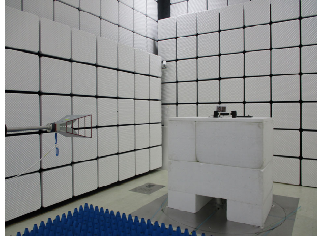
Part_15.247_WLAN_Radiated_Setup
