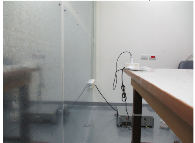
Part_15.247_WLAN_Conduction_Setup
