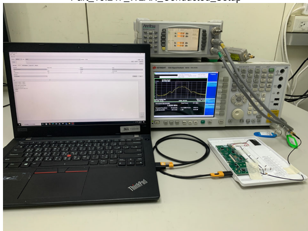
Part_15.247_WLAN_Conducted_Setup
