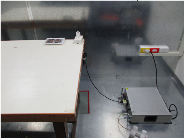
Part_15.247_LE_Conduction_Setup
