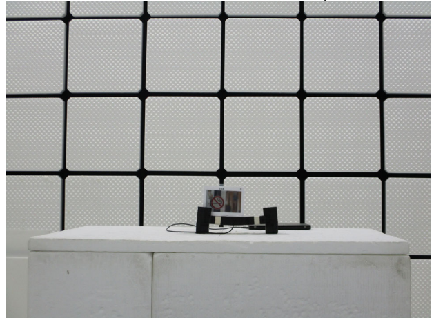
Part_15.247_WLAN_Radiated_Setup
