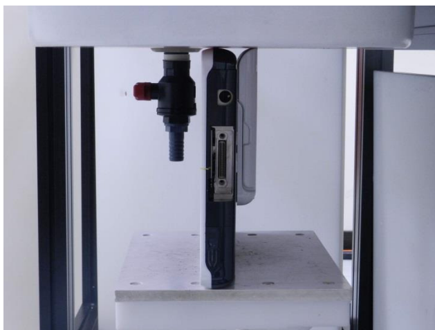
Edge 1 with stand, Test Separation 0 mm
