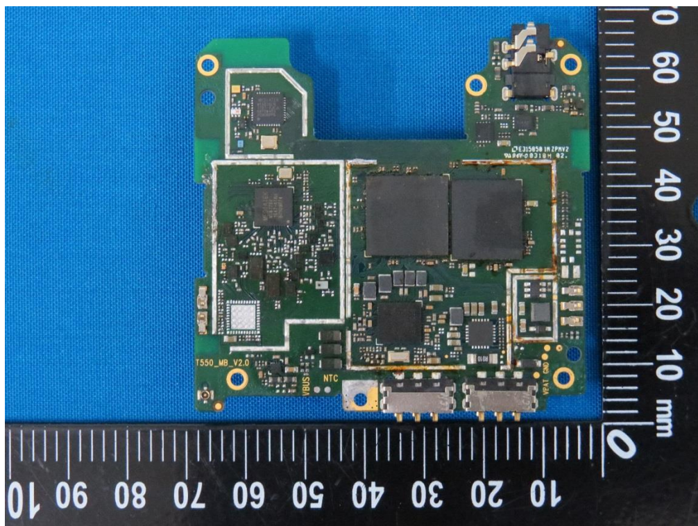
EUT- Main Board Uncover View
