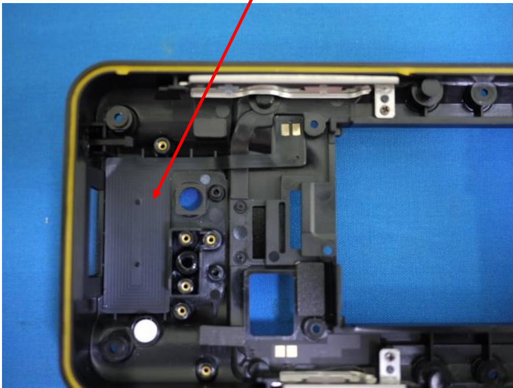
NFC PCB Antenna – Top View
