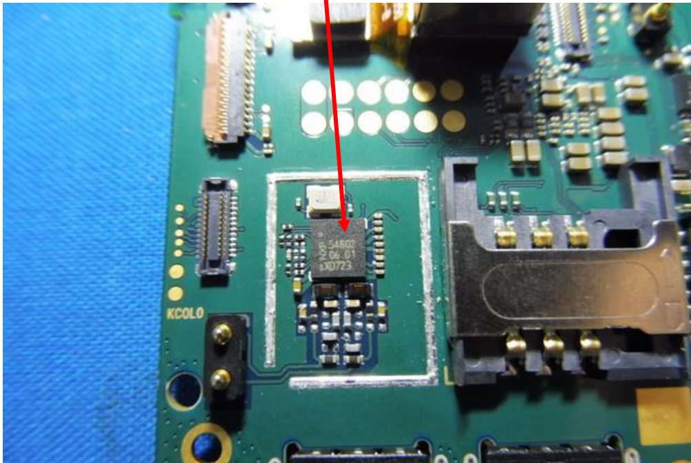
NFC RF Chip IC – Top View
