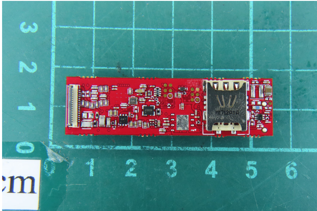
(39) EUT Photo
