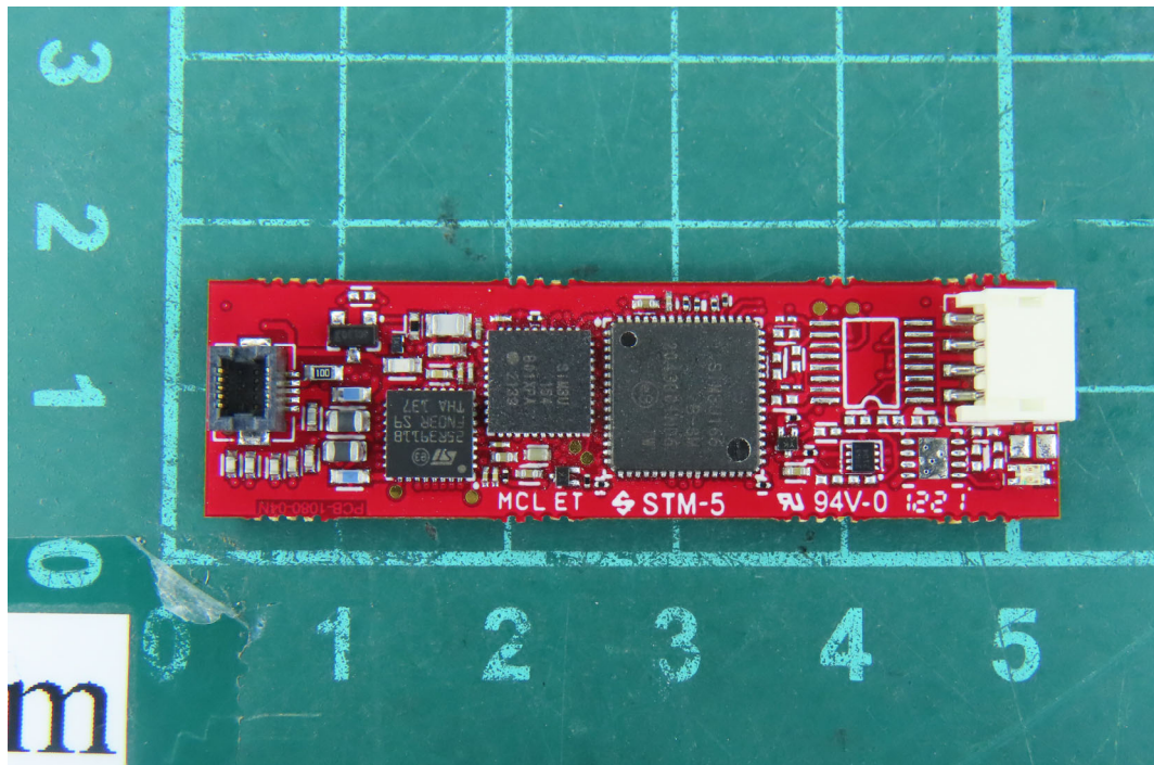
(38) EUT Photo
