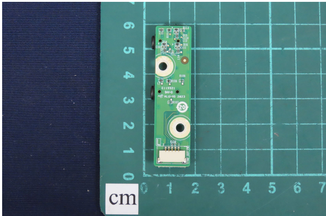
(68) EUT Photo
