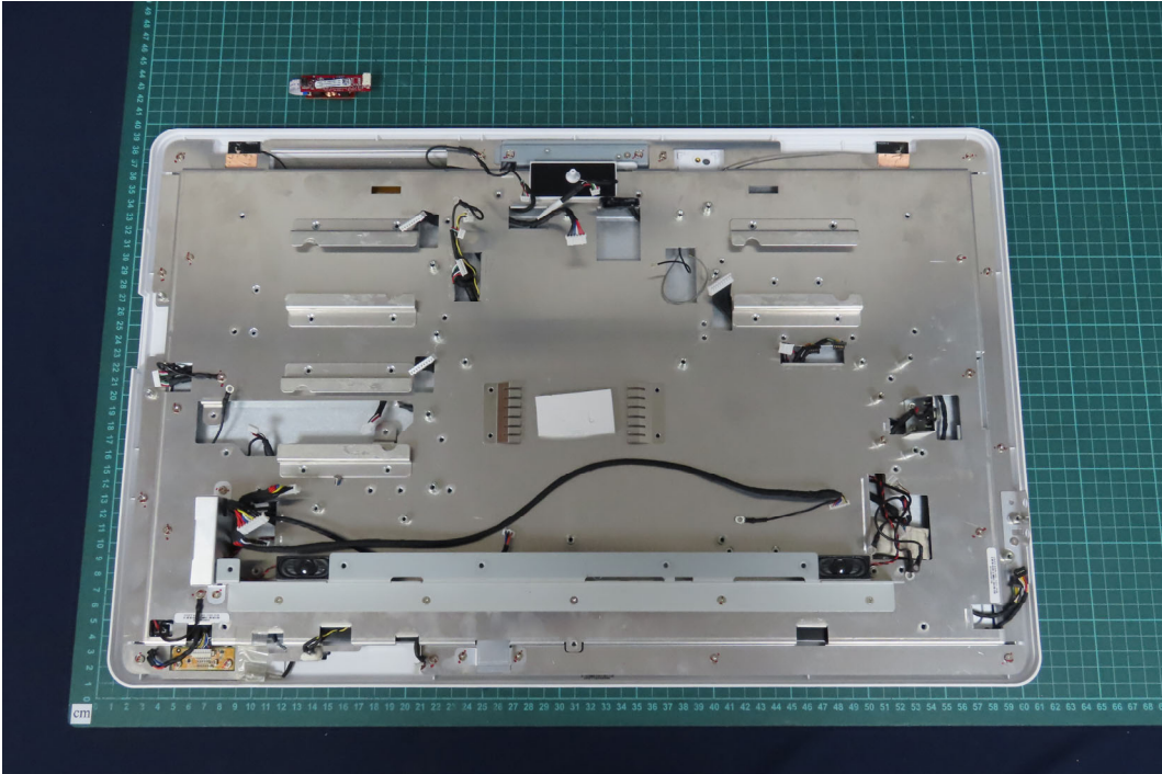
(76) EUT Photo
