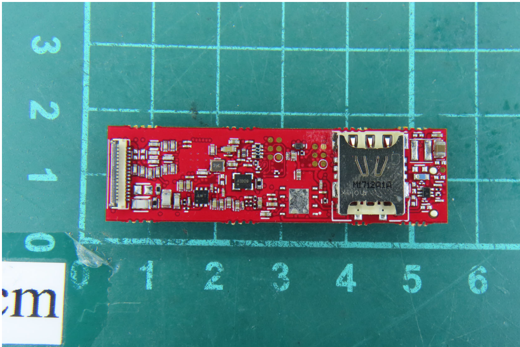
(80) EUT Photo
