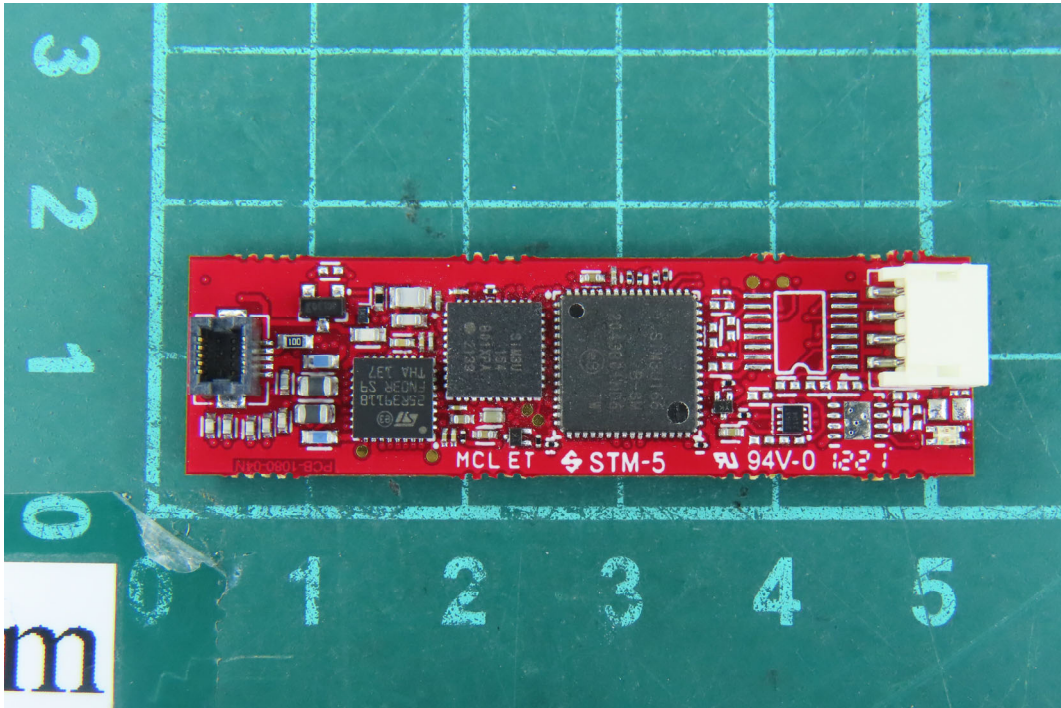
(79) EUT Photo
