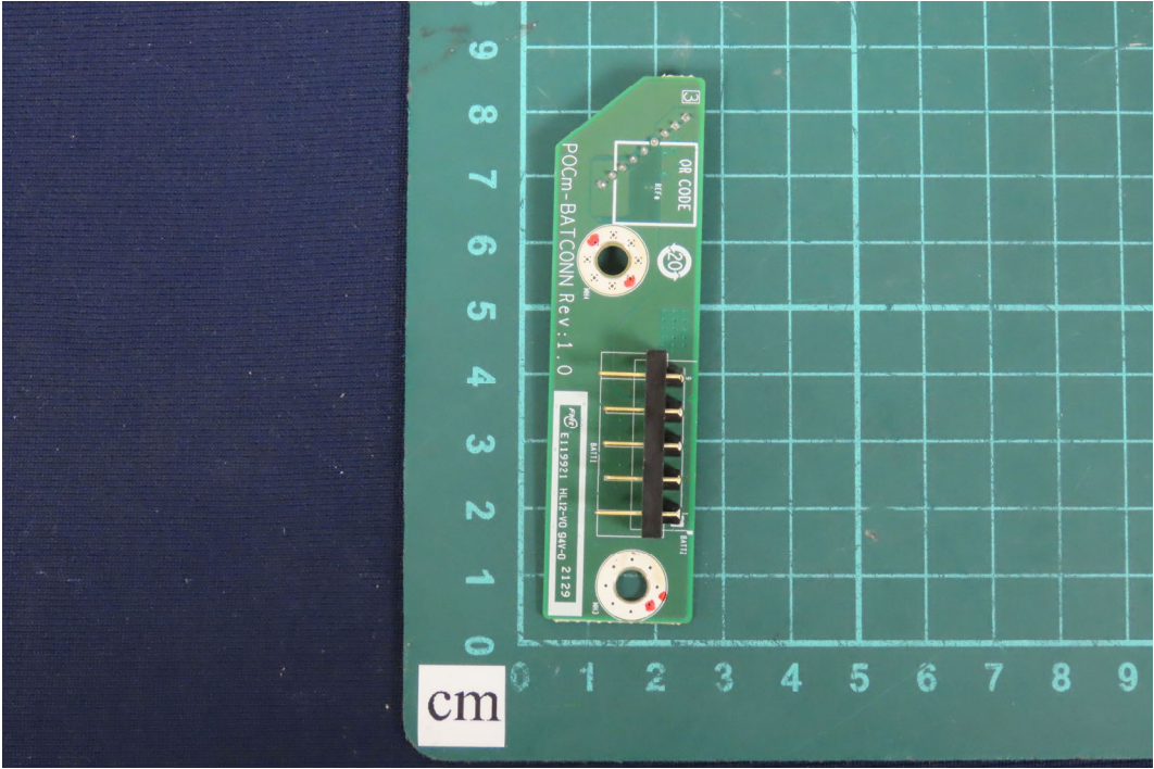
(100)EUT Photo
