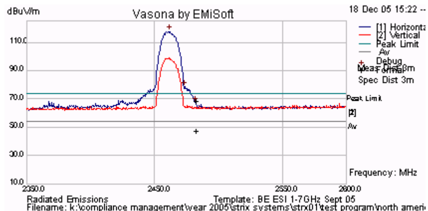
Plot 68 Channel 11 – Upper Band Edge, Peak Emission = 117.57 dBμV/m
