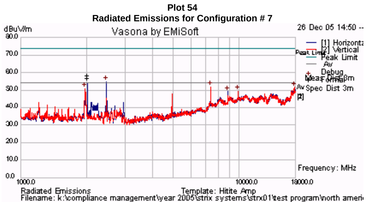
Freq. (MHz) Pol. (H/V) Raw Reading (dBμV/m) Correction Factor (dB) Corrected Field Strength (dBμV/m) Limit (dBμV/m) Margin (dB) 2016.087 H 59.44 -5.65 53.79 54 -0.21
