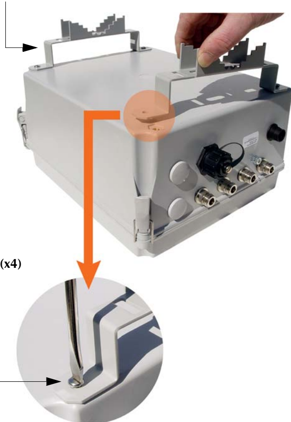
Mounting Brackets (x2)
