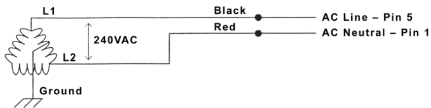
240 VAC Three Phase (two wire service - Delta)
