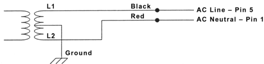
240 VAC Single Phase (two wire service)
