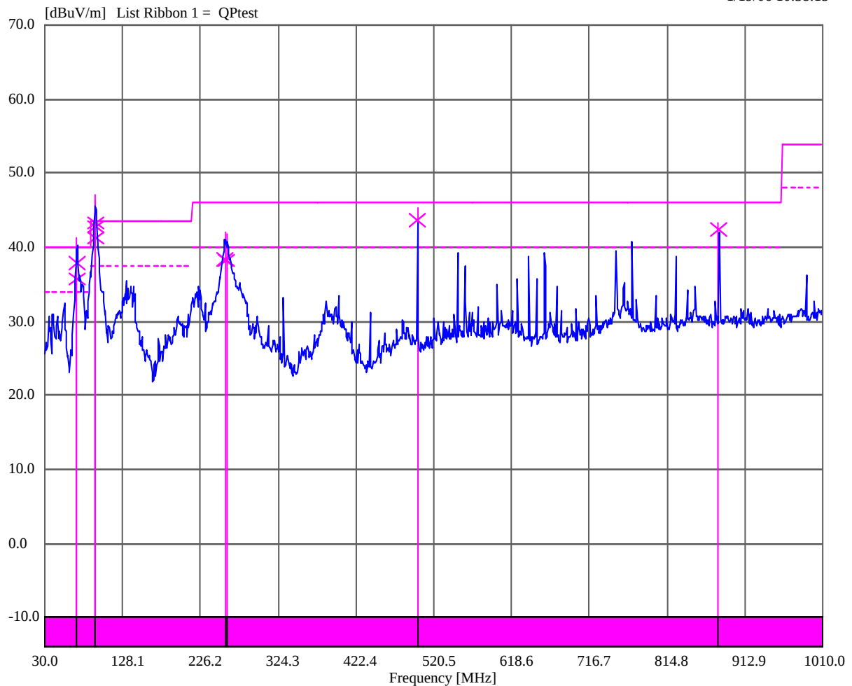
Plot 31 Radiated Spurious Emissions 30 MHz to 1 GHz
