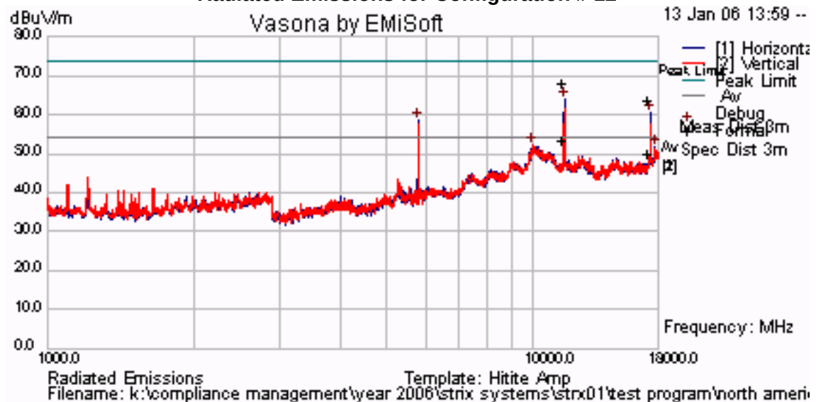
Plot 59 Radiated Emissions for Configuration # 12
